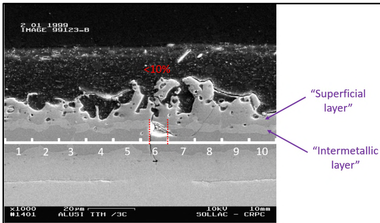
Cornette, Figure 22 (Section view)
