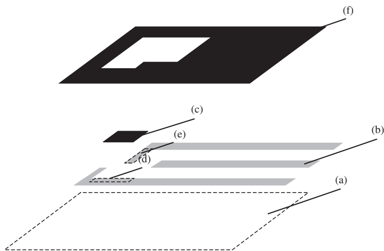
Figure 1. Components of the in-house screen-printed electrode: (a) substrate, (b) Ag/AgCl conducting paths, (c) carbon working electrode, (d) Ag/AgCl auxiliary electrode, (e) Ag/AgCl reference electrode, and (f) insulation layer. (Working electrode area: 9 mm 2 ).
