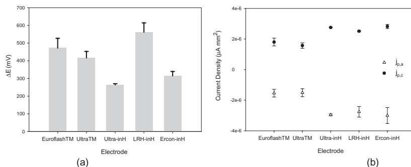
Figure 3. (a) Cyclic voltammetric peak separations ( \Delta E_p ) and (b) anodic and cathodic peak current densities for 1 \times 10^{-3} M ferri/ferrocyanide and 1 M KCl for each of the screen-printed electrodes ( n=3 ).
