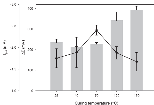
Figure 6. Mean cyclic voltammetric peak separations ( n=4 ) (bar) and mean anodic peak currents ( n=4 ) (line) for 1 \times 10^{-3} M ferrocyanide and 1 M KCl for varying curing temperatures of the Ultra™ ink on the Ultra-inH electrode. A curing temperature of 70°C showed optimal voltammetric performance for \Delta E_p and i_{p,a} values.
