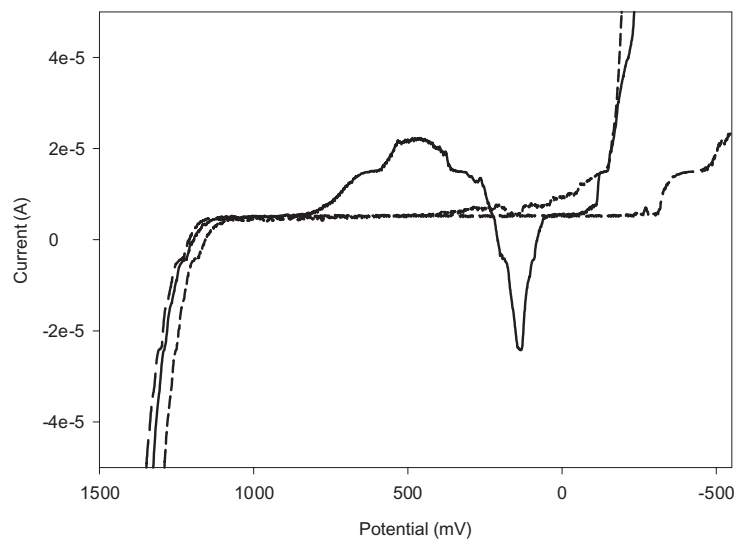
Figure 5. Linear sweep voltammograms in degassed PBS buffer (pH 6.8). Electrodes used were (solid line) LRH-inH, (long dash) Ultra-inH, and (short dash) Ercon-inH.
