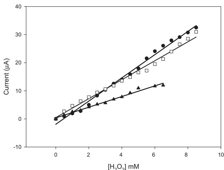
Figure 4. Amperometric sensor responses for successive additions of 0.5 mM hydrogen peroxide to a solution containing 2 mg/mL horseradish peroxidase. Electrodes used were (●) Ultra-inH, (□) Ercon-inH, and (▲) LRH-inH. Electrodes held at -100 mV vs. Ag/AgCl wire electrode.
