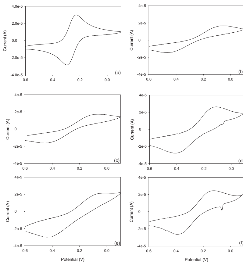
Figure 2. Cyclic voltammograms for different electrodes in 1 \times 10^{-3} M ferri/ferrocyanide and 1 M KCl supporting electrolyte. (a) Glassy carbon, (b) Euroflash™, (c) Ultra™, (d) Ercon-inH, (e) LRH-inH, and (f) Ultra-inH. The commercial electrodes ((b), (c)) showed very poor reversibility. Using the in-house design, ((d), (e), (f)) reversibility improved, with the Ultra-inH exhibiting the best behavior.
