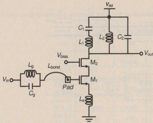
Fig. 11. Concurrent dual-band CMOS LNA (biasing circuitry not shown).
