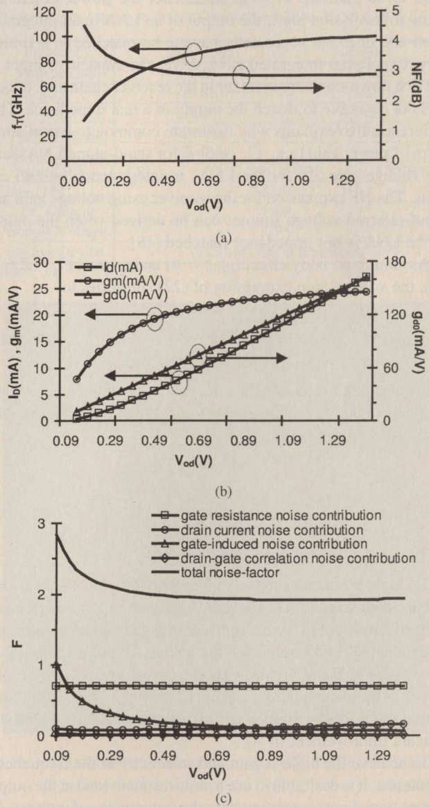
Fig. 9. (a) NF, f_T of a 20 \times 2.5 \mu\text{m}/0.18 \mu\text{m} CMOS transistor. (b) I_D , g_m , g_{d0} of the transistor. (c) Different noise contributions to the total NF from (16b) (NF numbers at 5.8 GHz).
