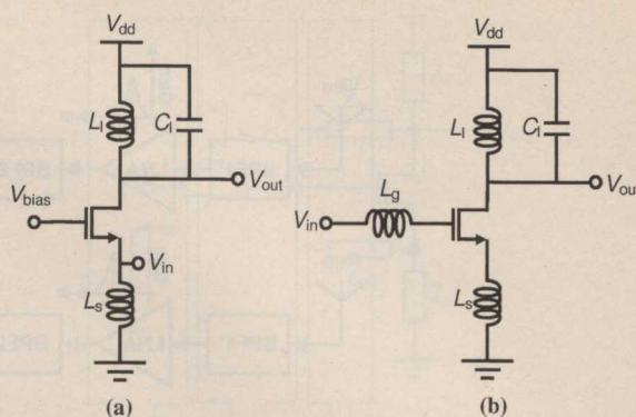
Fig. 1. Commonly used single-band CMOS LNAs. (a) Common-gate. (b) Common-source with inductive degeneration.
