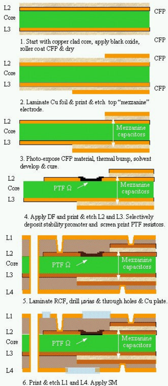
Figure 2 – EP Technology Process Flow with CFP Features Include: CFP Mezzanine Layer Capacitors, PTF Resistors, HDI Dielectric Capacitors and Inductors
