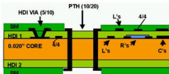
Figure 7 - Schematic Cross Section of RF Module Substrate Construction, with Feature Dimensions Shown in Mils
