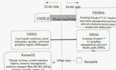
Figure 26. The relative code distribution in Windows 95
