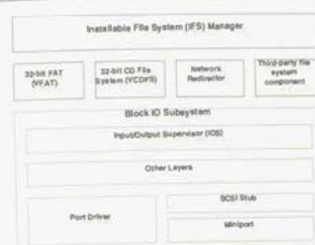
Figure 28. The file system architecture
