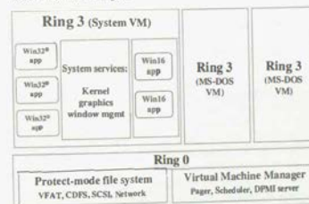
Figure 27. The integrated architecture of Windows 95, which supports running MS-DOS-based, Win16-based, and Win32-based applications
