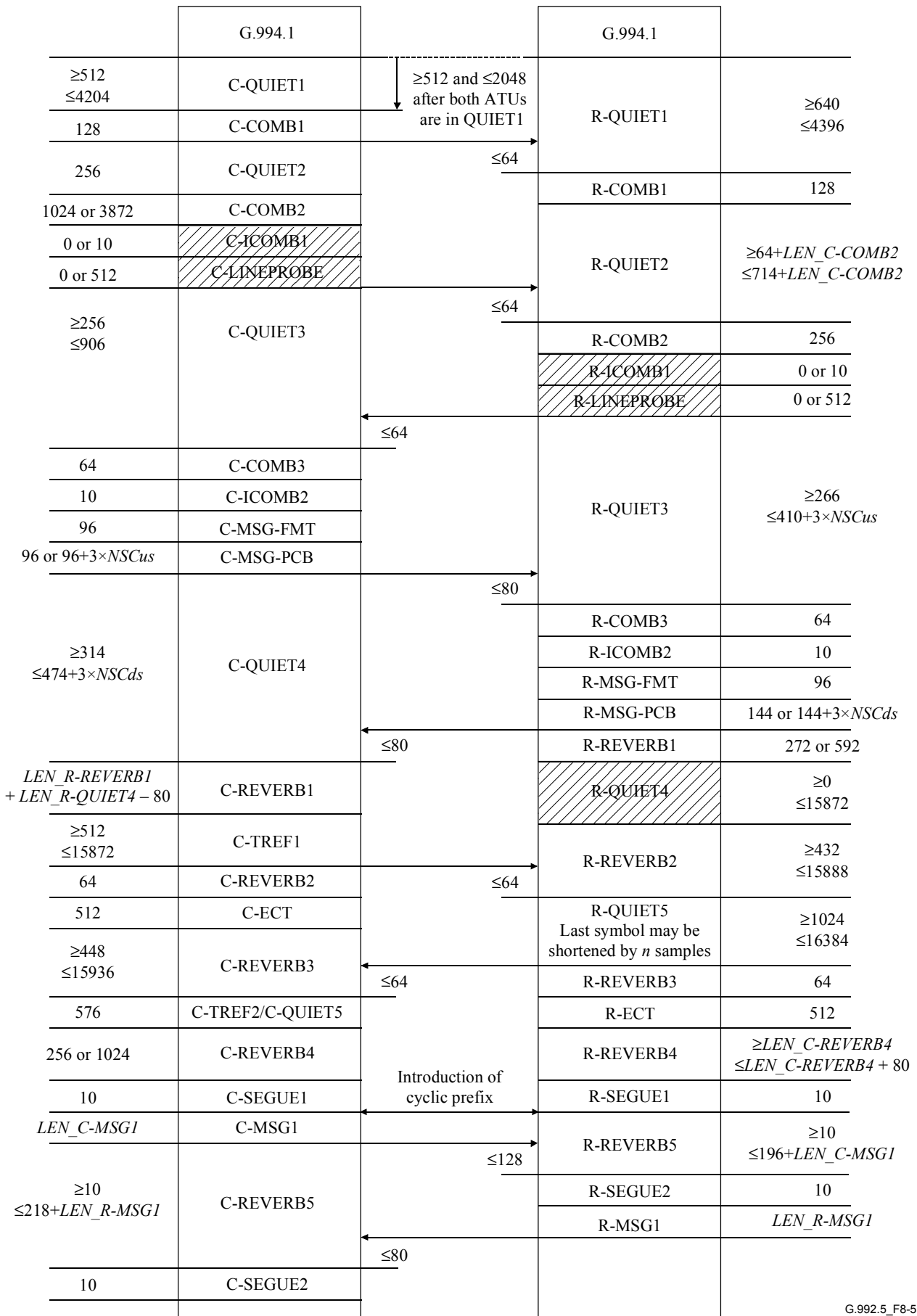
Figure 8-5/G.992.5 – Timing diagram of the initialization procedure (part 1)
