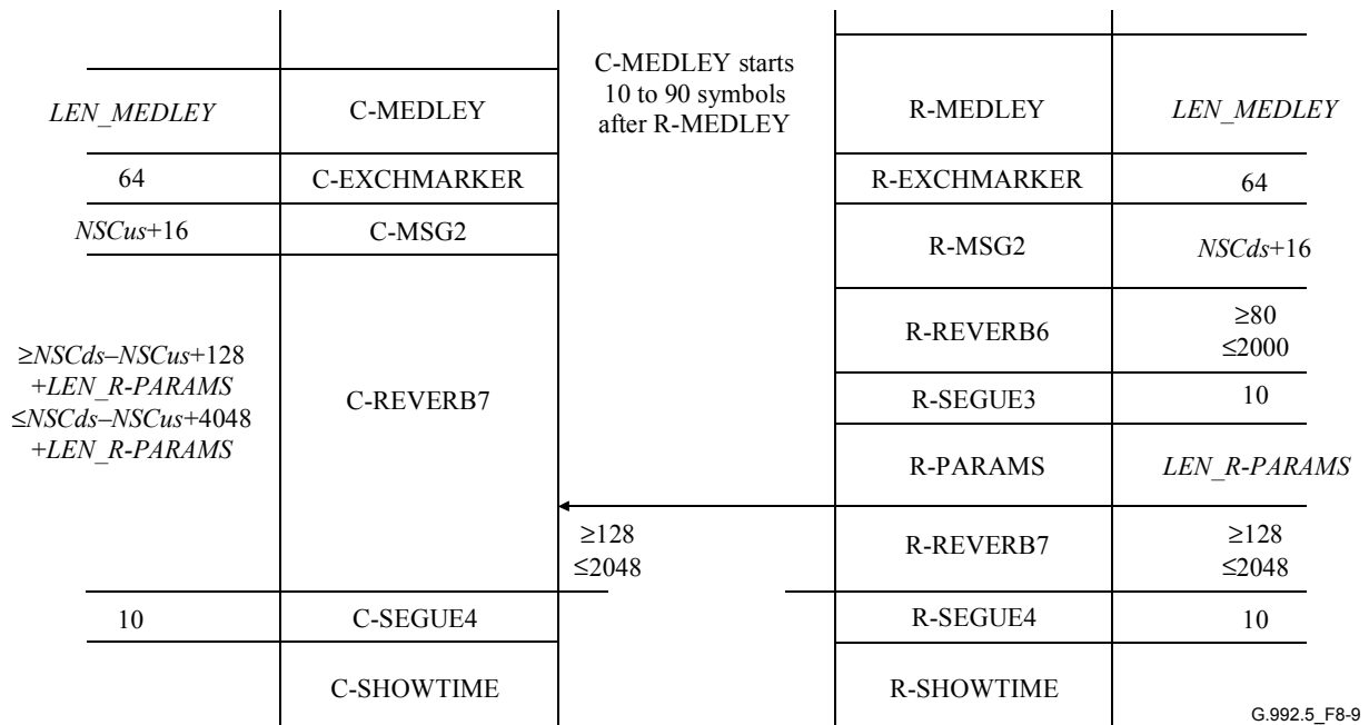
Figure 8-9/G.992.5 – Timing diagram of the initialization procedure (part 2) without C-PARAMS and with R-PARAMS states
