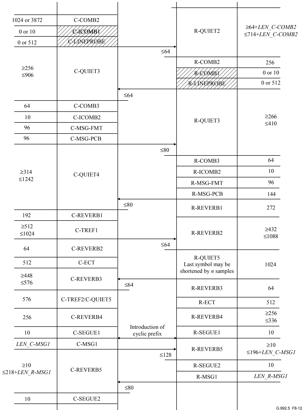
Figure 8-12/G.992.5 – Timing diagram of the short initialization procedure (part 1)
