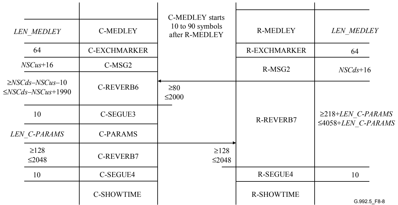
Figure 8-8/G.992.5 – Timing diagram of the initialization procedure (part 2) with C-PARAMS and without R-PARAMS states
