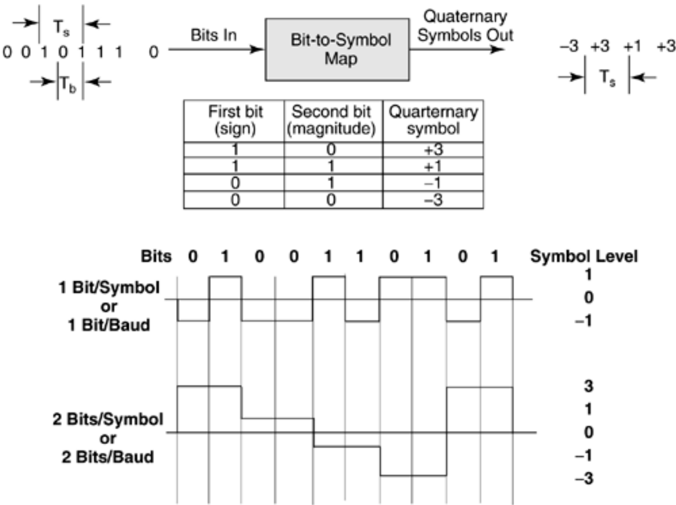
Figure 4.8. Bit-to-symbol mapping in 2B1Q HDSL.
