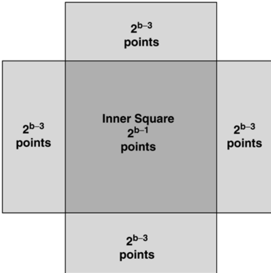
Figure 2.9. General QAM cross for b > 4 and odd.
