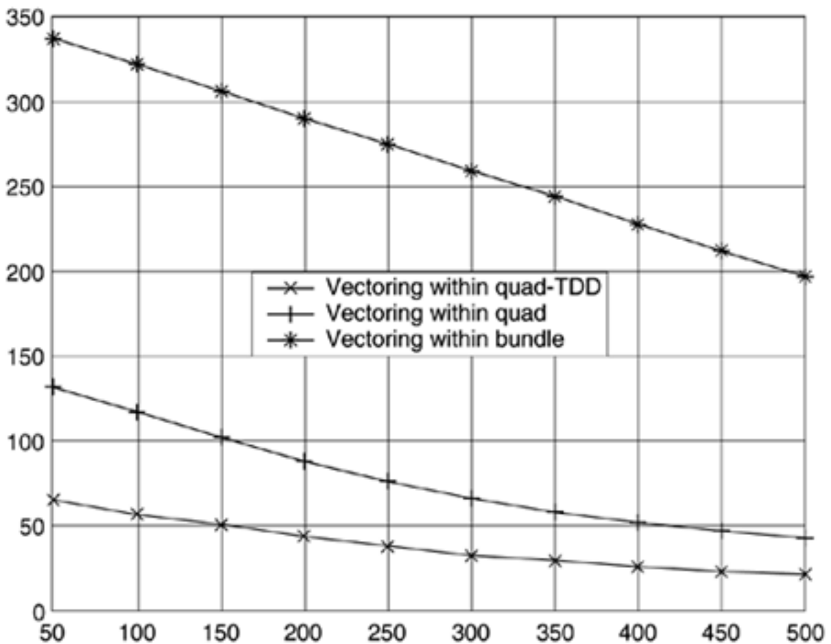
Figure 11.39. Longer line EFM/VDSL results with vectored DMT "symmetric transmission over full band.
