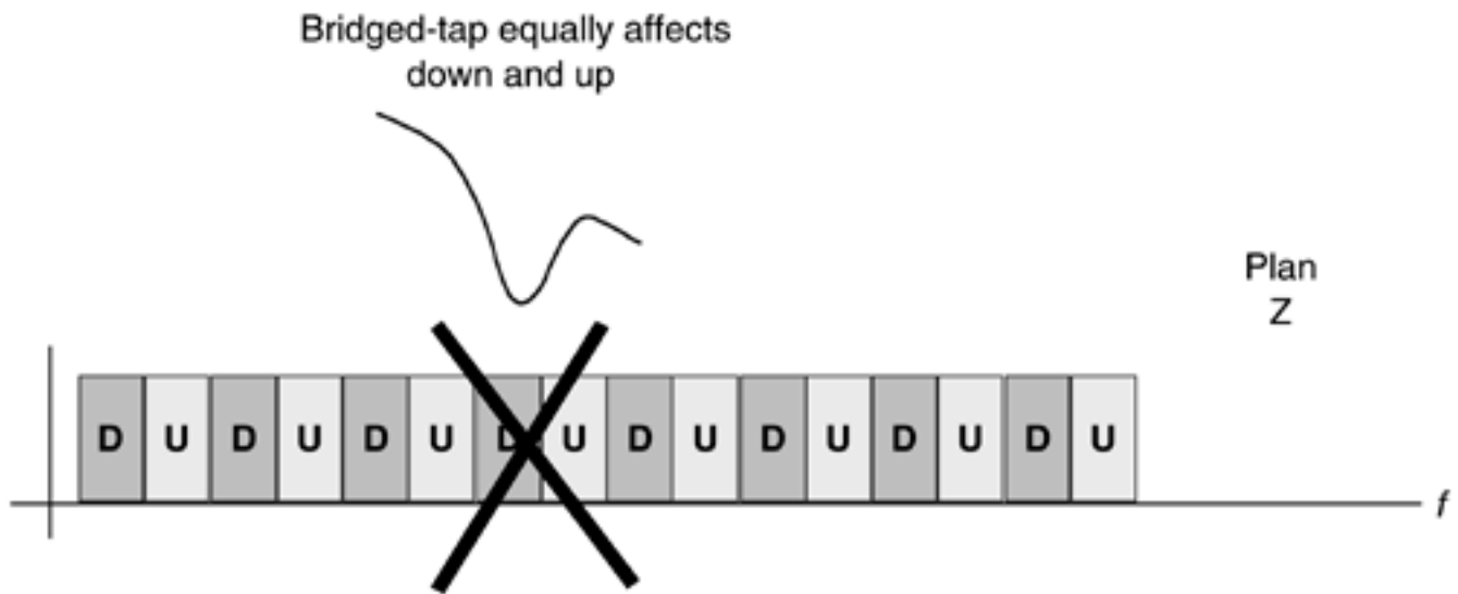
Figure 7.6. Optimal robust duplexing solution "the effect of bridged tap is shared between upstream and downstream.
