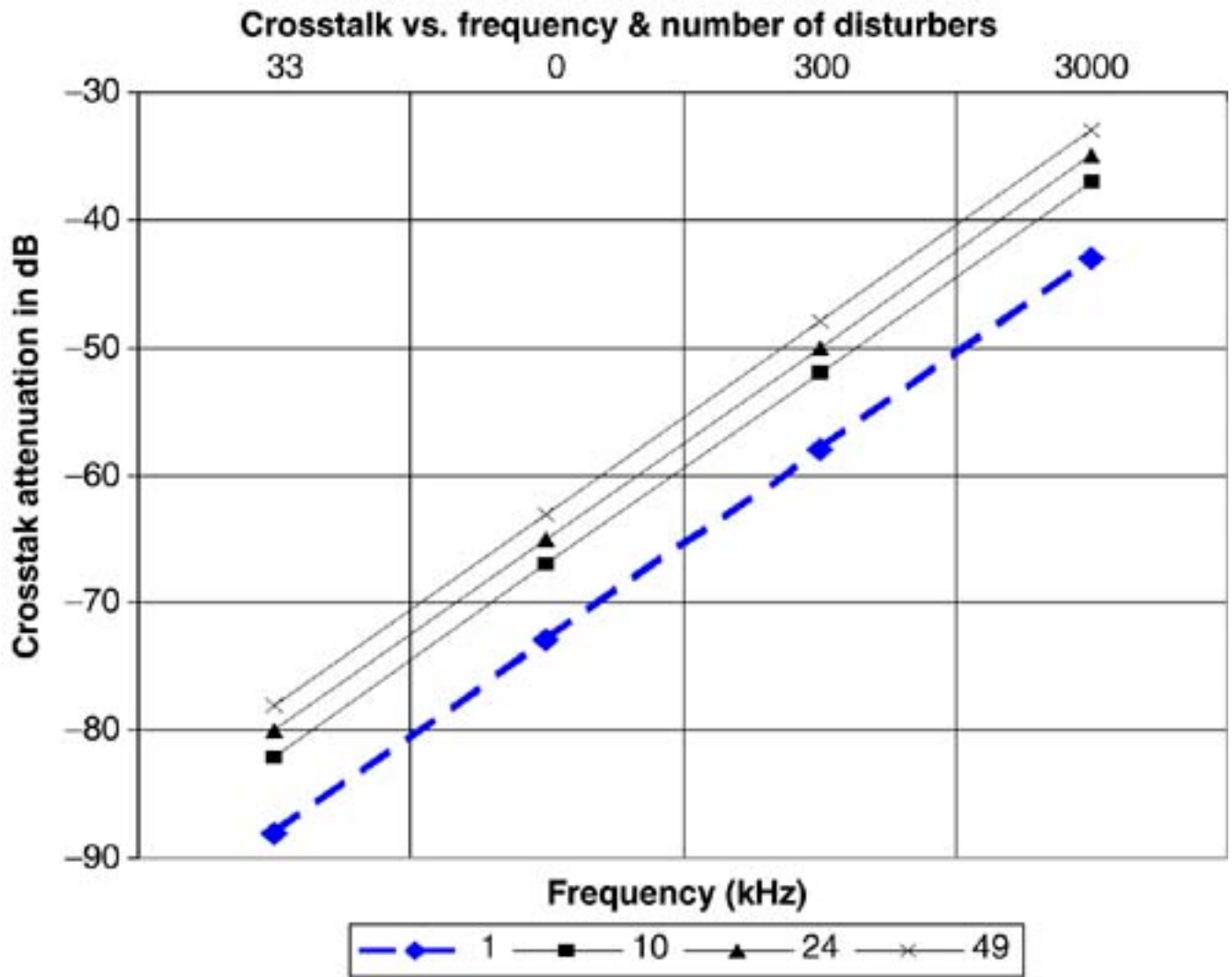
Figure 9.3. Plot of NEXT coupling versus frequency per number of disturbers.
