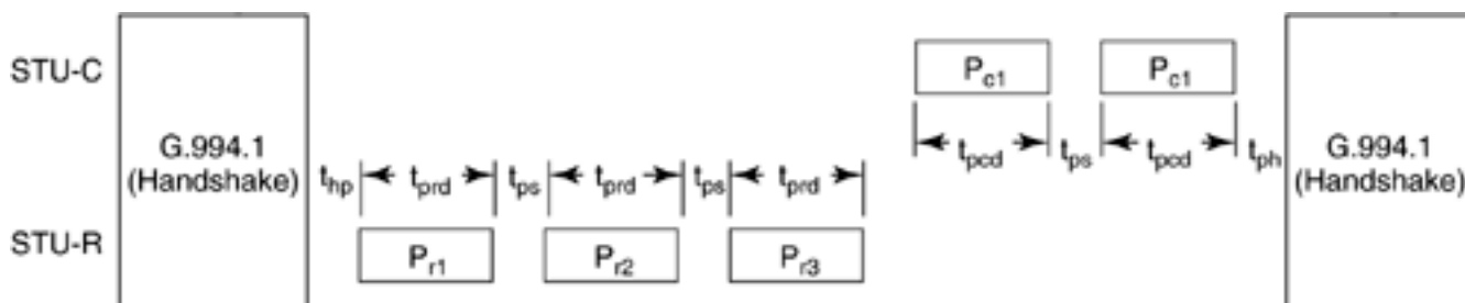
Figure 6.25. SHDSL preactivation sequence.
