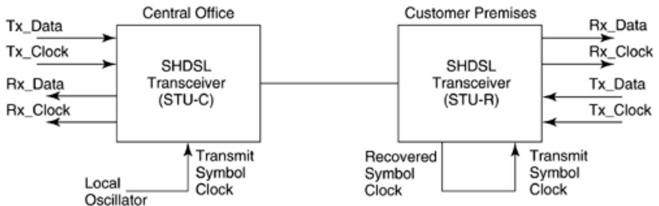
Figure 6.20. Plesiochronous timing mode.
