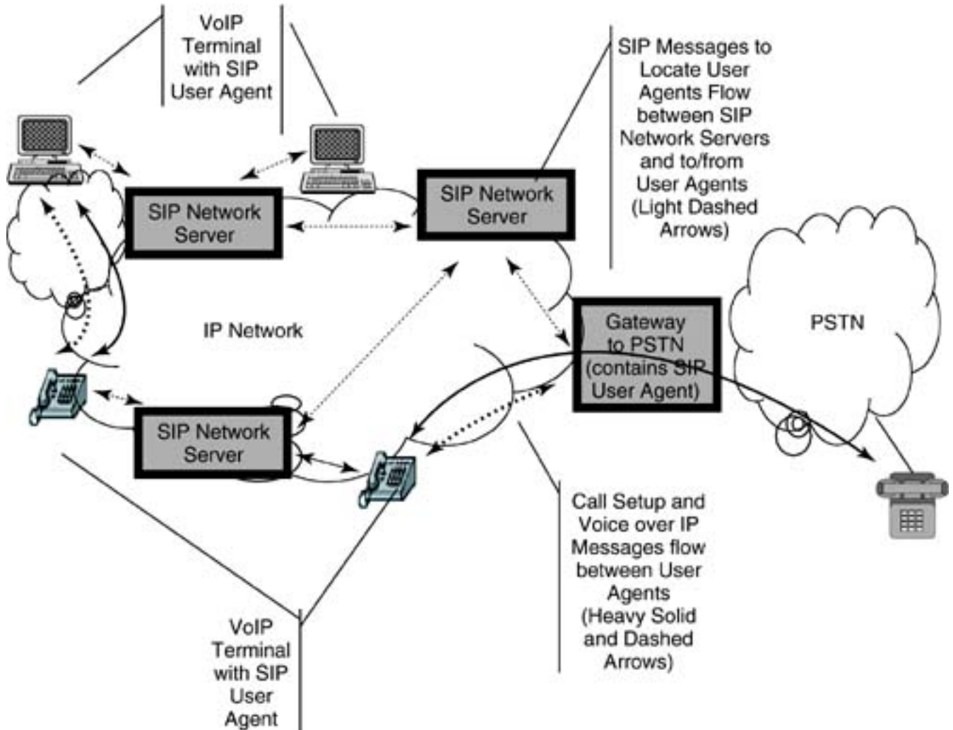
Figure 16.10. Overview of the SIP architecture.
