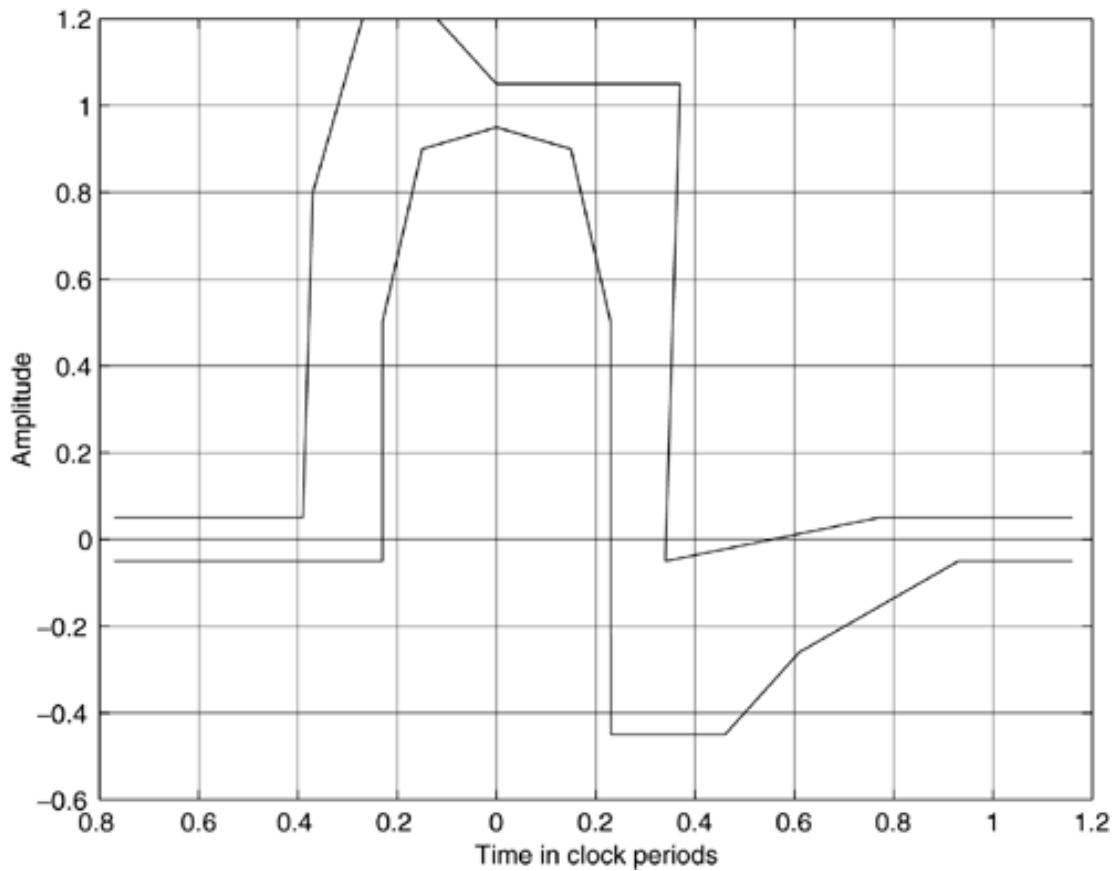
Figure 2.7. T1.403 "T1" pulse shape (basis function after 1-D operation in T1 alternate mark inversion (AMI), 1 = 648 ns).
