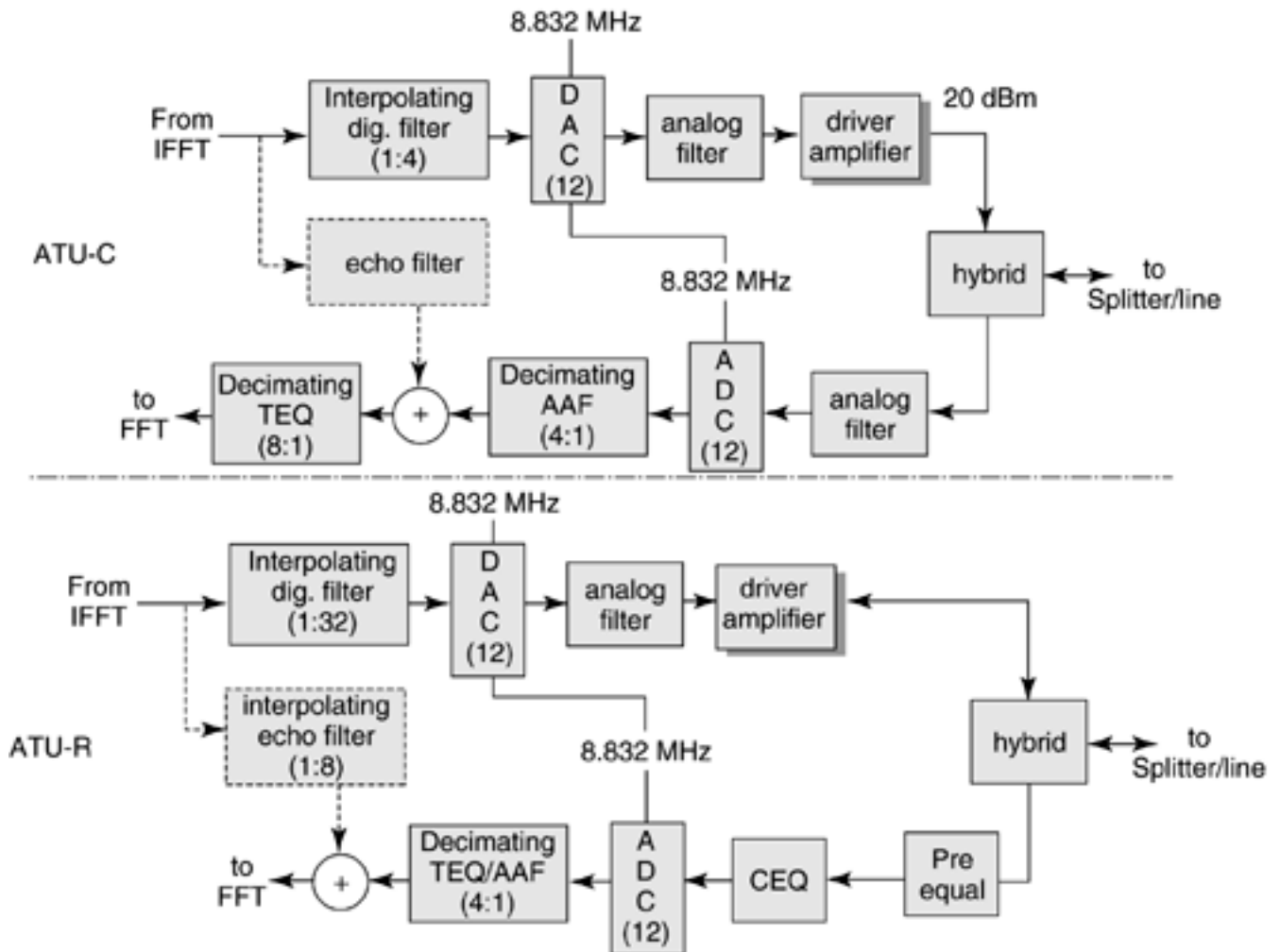
Figure 3.16. Analog front ends.
