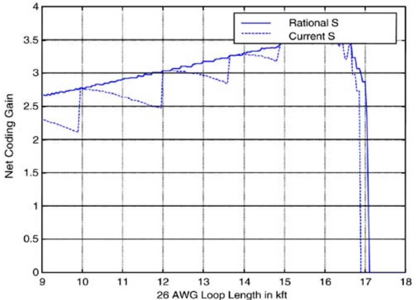
Figure 3.11. Net coding gain produced by new ADSL framing proposal (see [6]).
