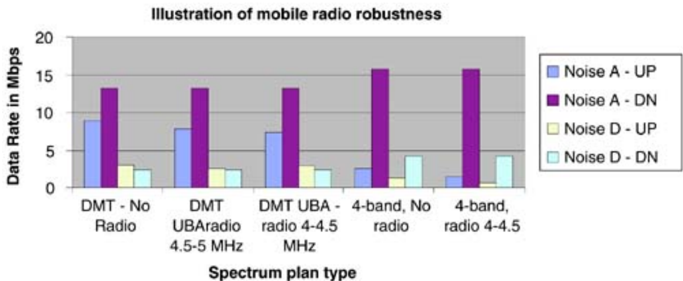
Figure 7.7. Illustration of mobile radio noise robustness for two plans with 1.1-km loop, 20 VDSL FEXT, noise A and D, .4 mm line.
