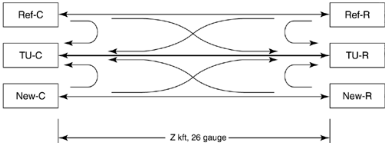
Figure 10.15. System model for evaluating crosstalk disturbance into basis system.
