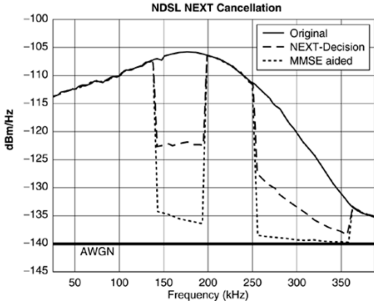
Figure 11.49. Illustration of reduction of HDSL NEXT into ADSL in the 150 to 200 kHz band that accrues to choosing X_2 to correspond to signals in the 250 to 350 kHz band. Effect of both decisions and no decisions with B_2 = 0 is shown.
