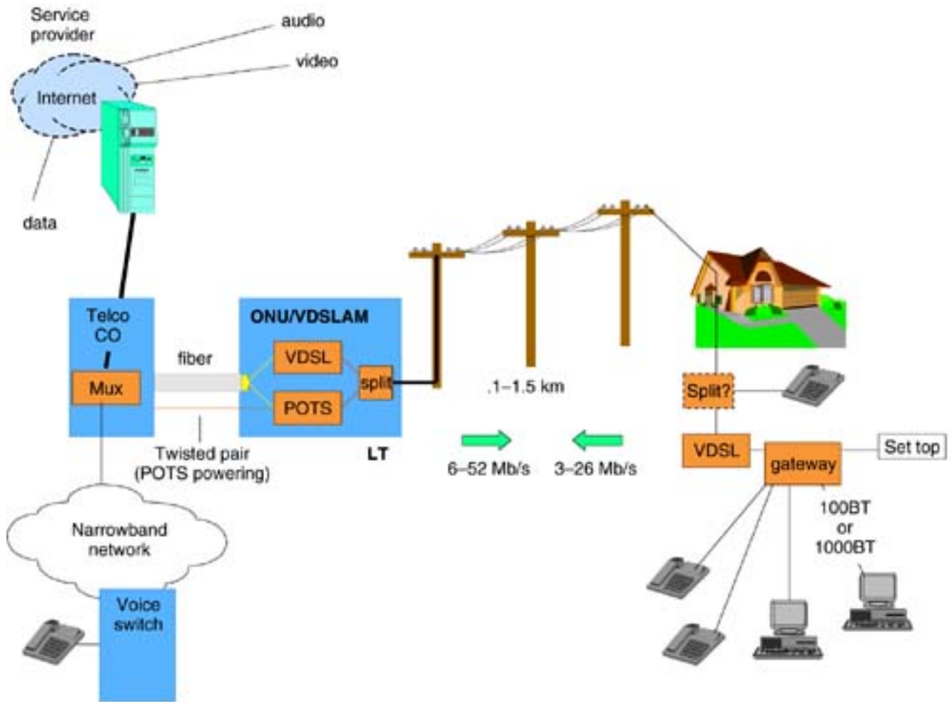
Figure 7.1. VDSL system architecture with ONU/fiber-loop-carrier system.
