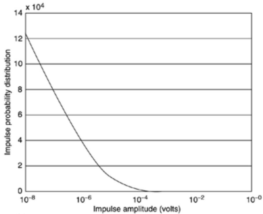
Figure 3.6. Exponential probability distribution for impulses.
