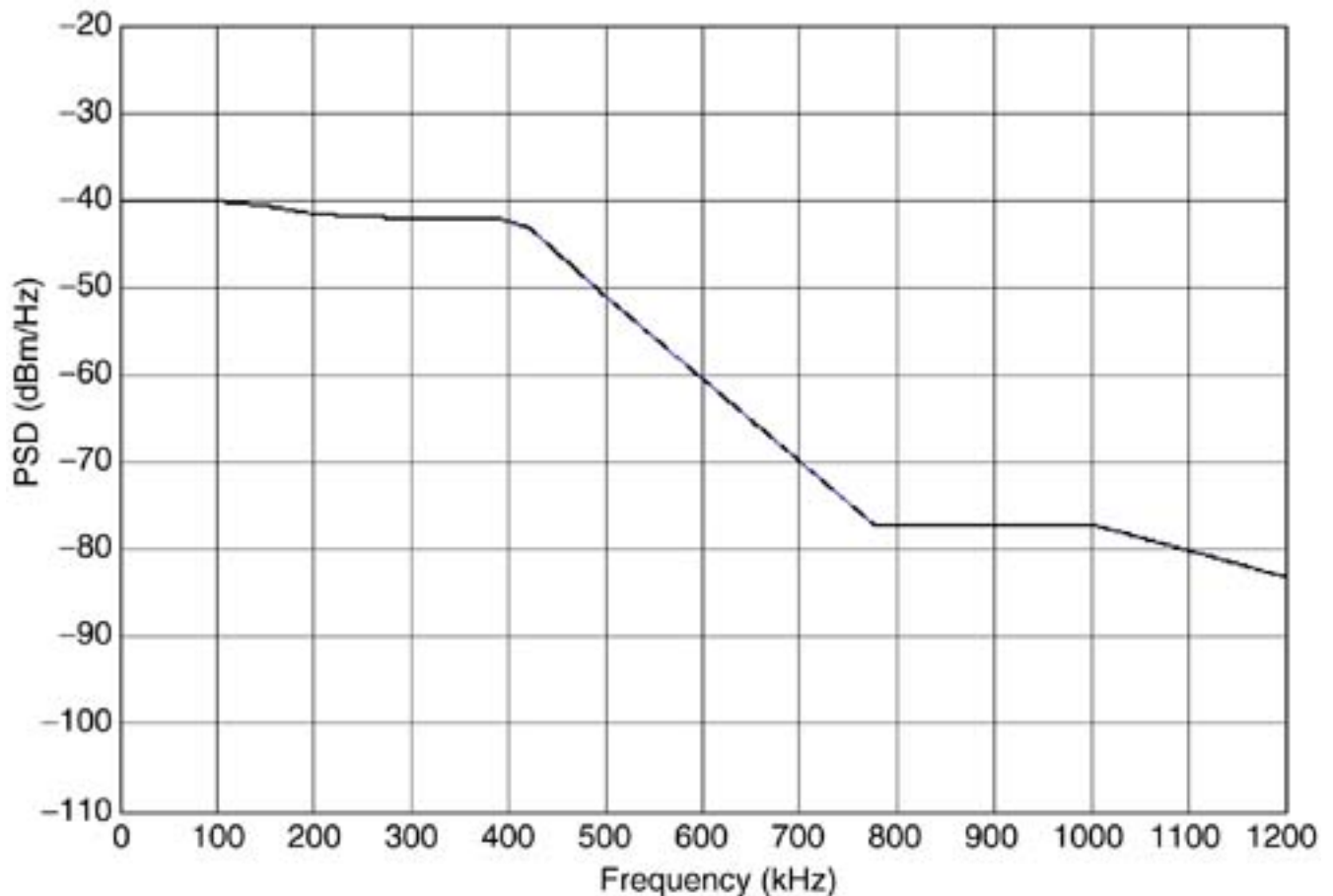
Figure 10.10. Spectrum Management Class 7 template plots.
