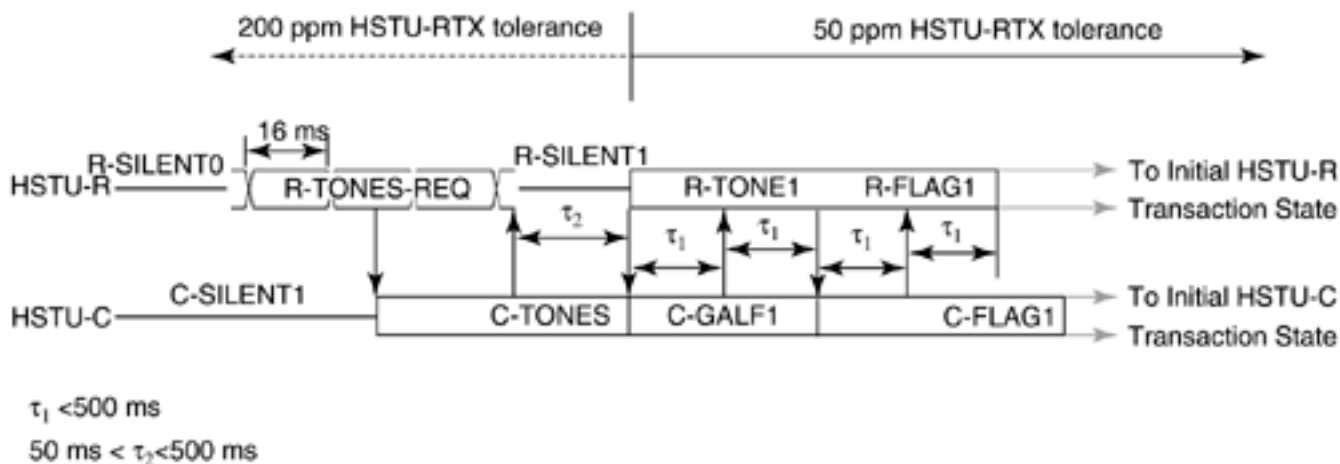
Figure 5.8. Customer premises initiated duplex start-up sequence (Figure 14/G.994.1[1]).
