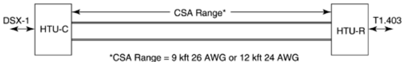
Figure 4.2. HDSL dual-duplex provisioning of T1 service.
