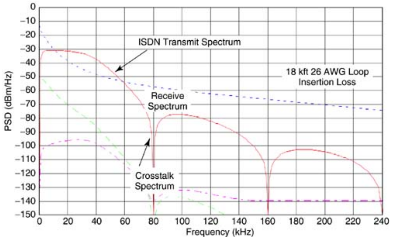
Figure 9.12. Spectral plots of ISDN reach with 49-SNEXT.
