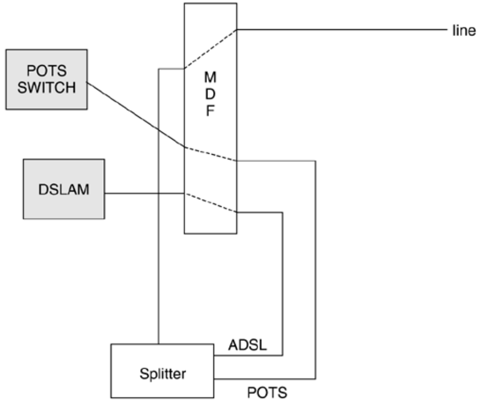
Figure 3.18. CO wiring configuration with splitters.
