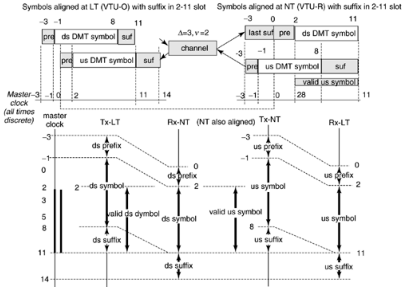
Figure 7.16. Illustration of cyclic suffix and LT timing advance.
