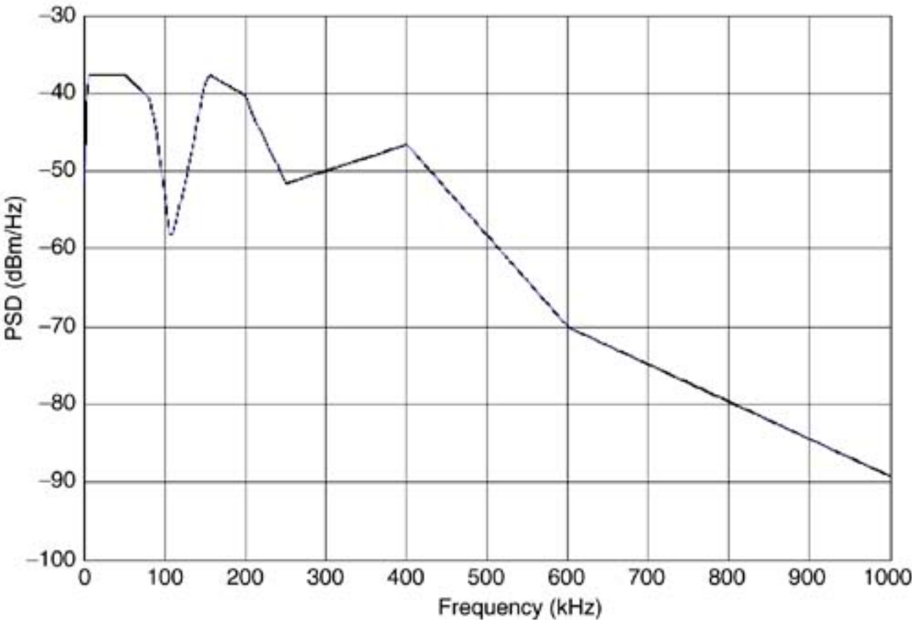
Figure 10.13. Plot of PSD template for HDSL4 downstream channel.
