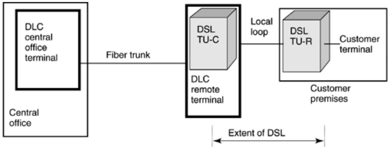
Figure 1.2. Digital Loop Carrier Reference Model
