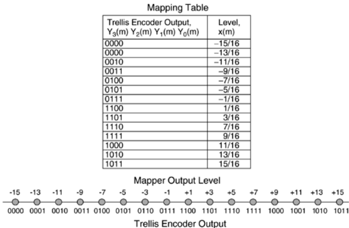
Figure 4.21. HDSL2 bit-to-symbol mapping.
