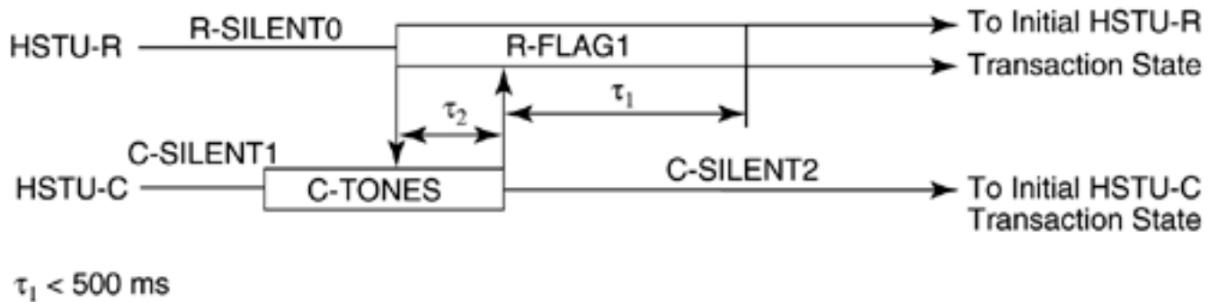
Figure 5.11. CO initiated half-duplex start-up sequence (Figure 17/G.994.1[1]).
