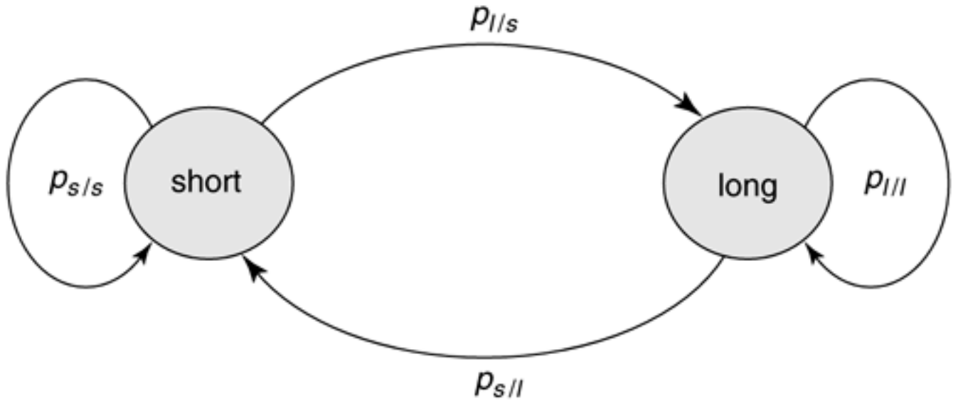
Figure 3.8. State transition diagram for interimpulse delay.
