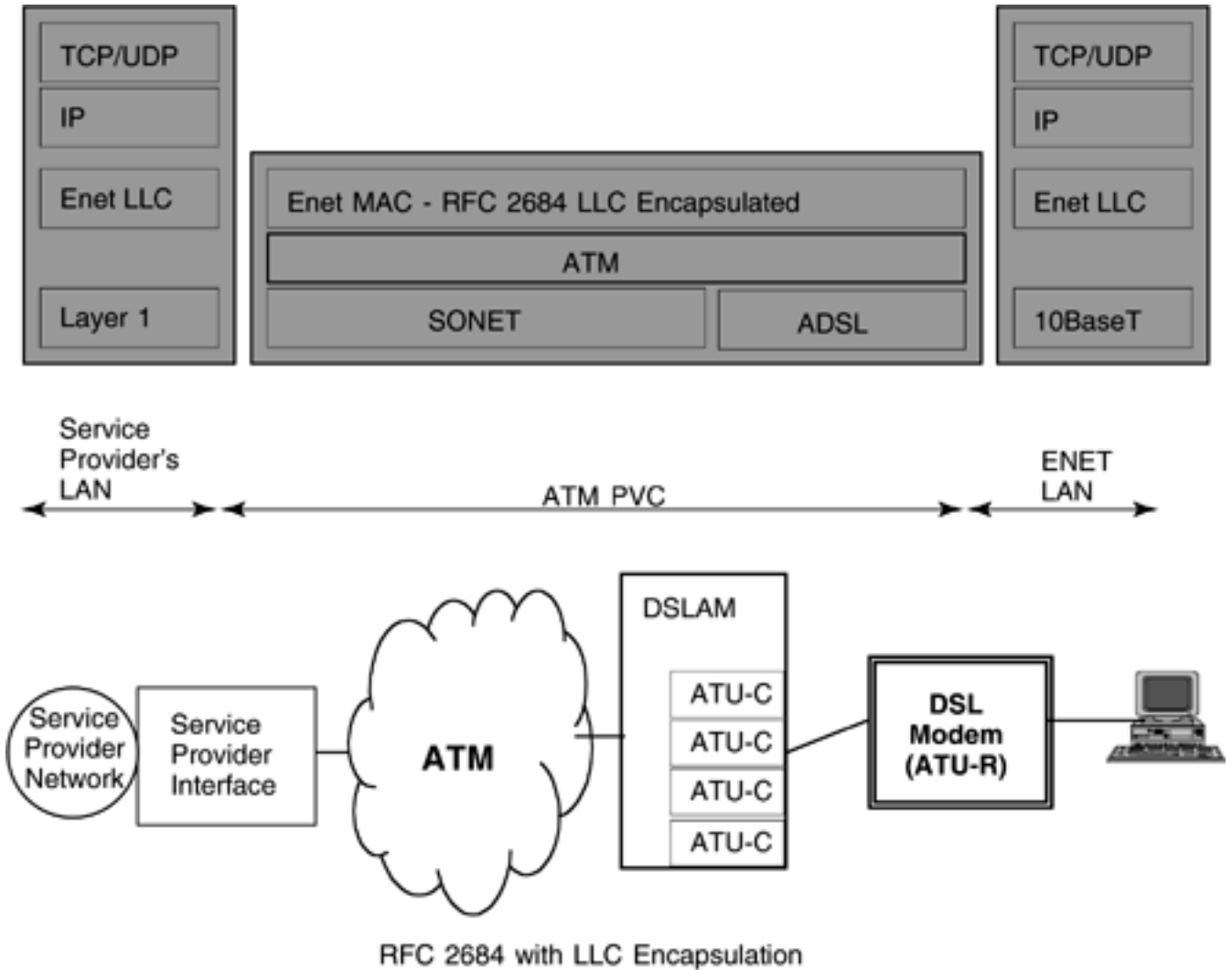
Figure 14.3. Bridged Ethernet directly transporting IP.
