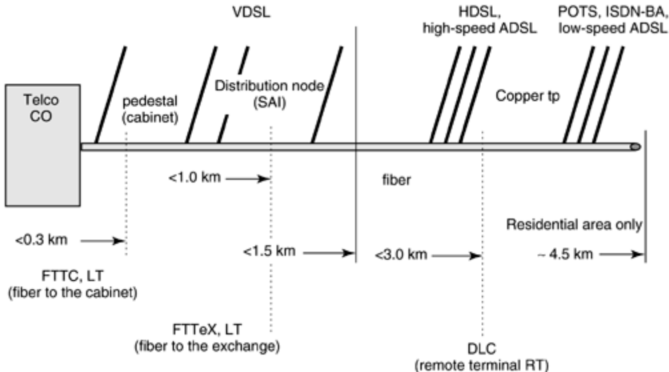
Figure 7.3. Illustration of intermediate points to which fiber (shaded line) may traverse.
