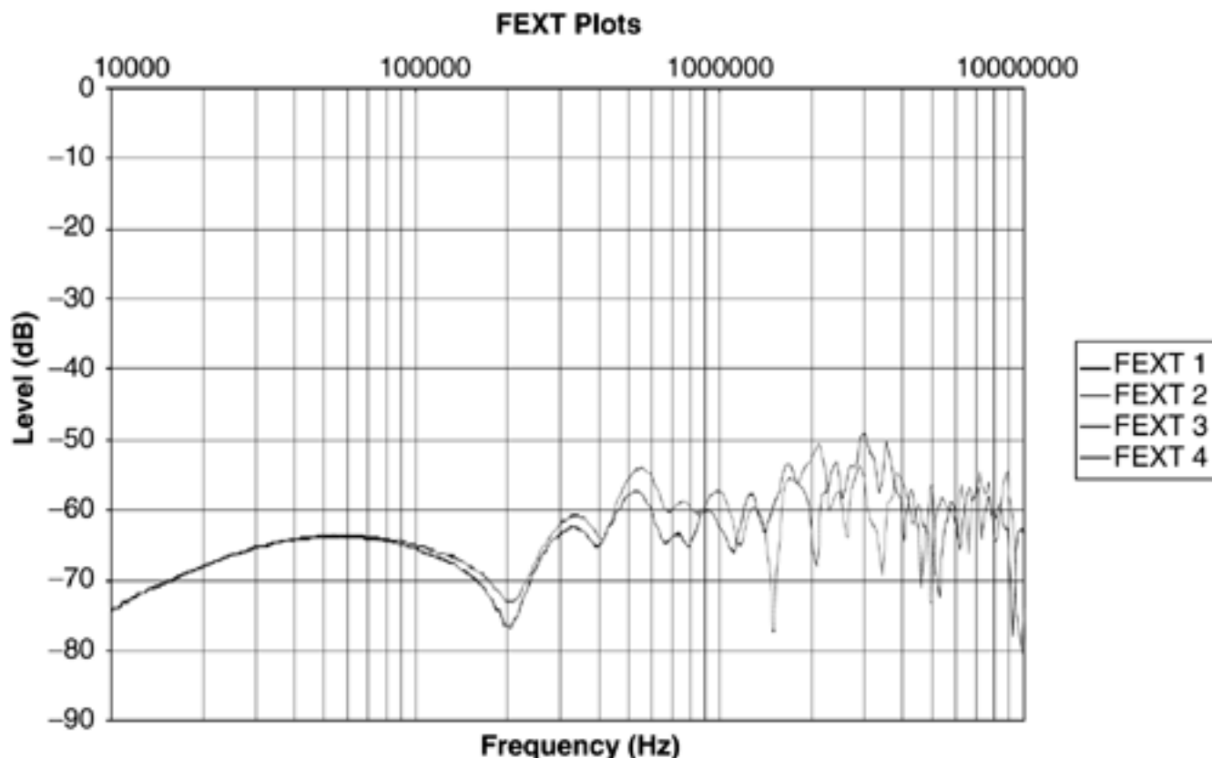
Figure 7.29. 500-meter example FEXT insertion loss functions. (Courtesy of John Cook of BTextact).
