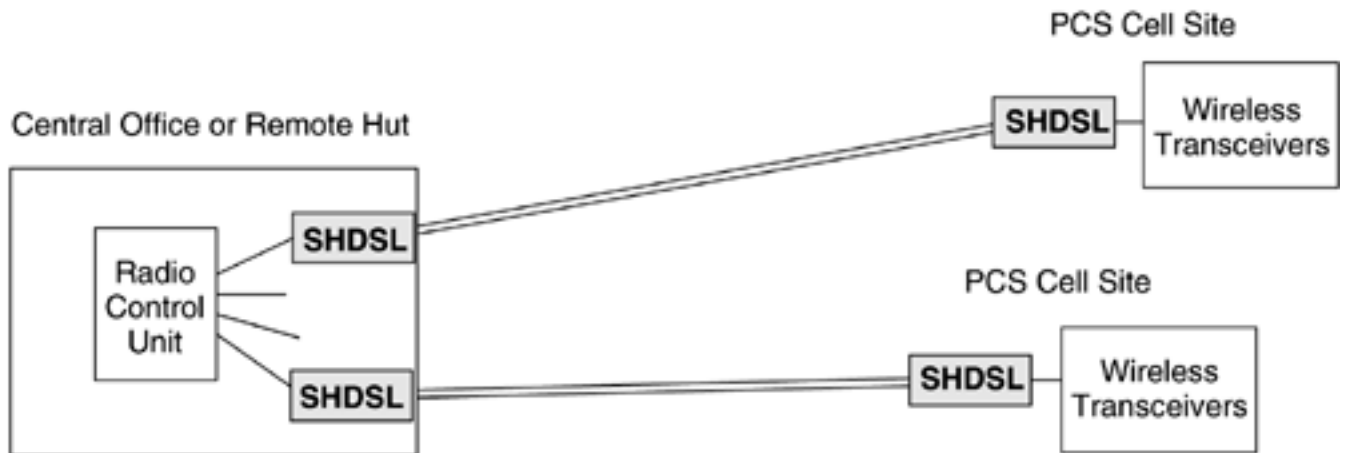
Figure 6.2. Transport application from wireless base station to central office.
