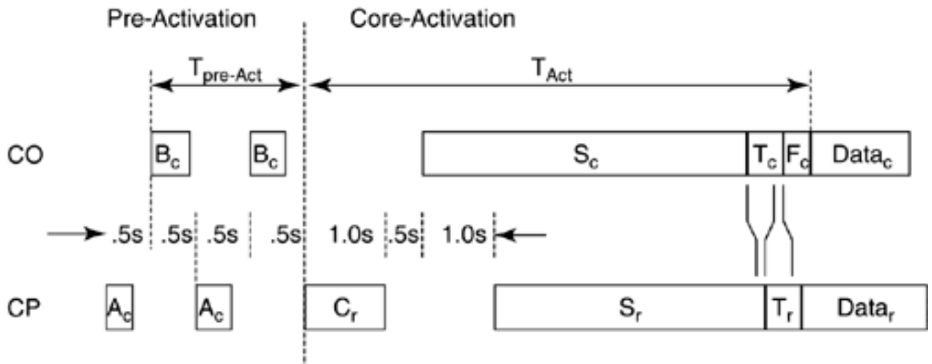
Figure 4.26. Initialization sequence timing diagram.
