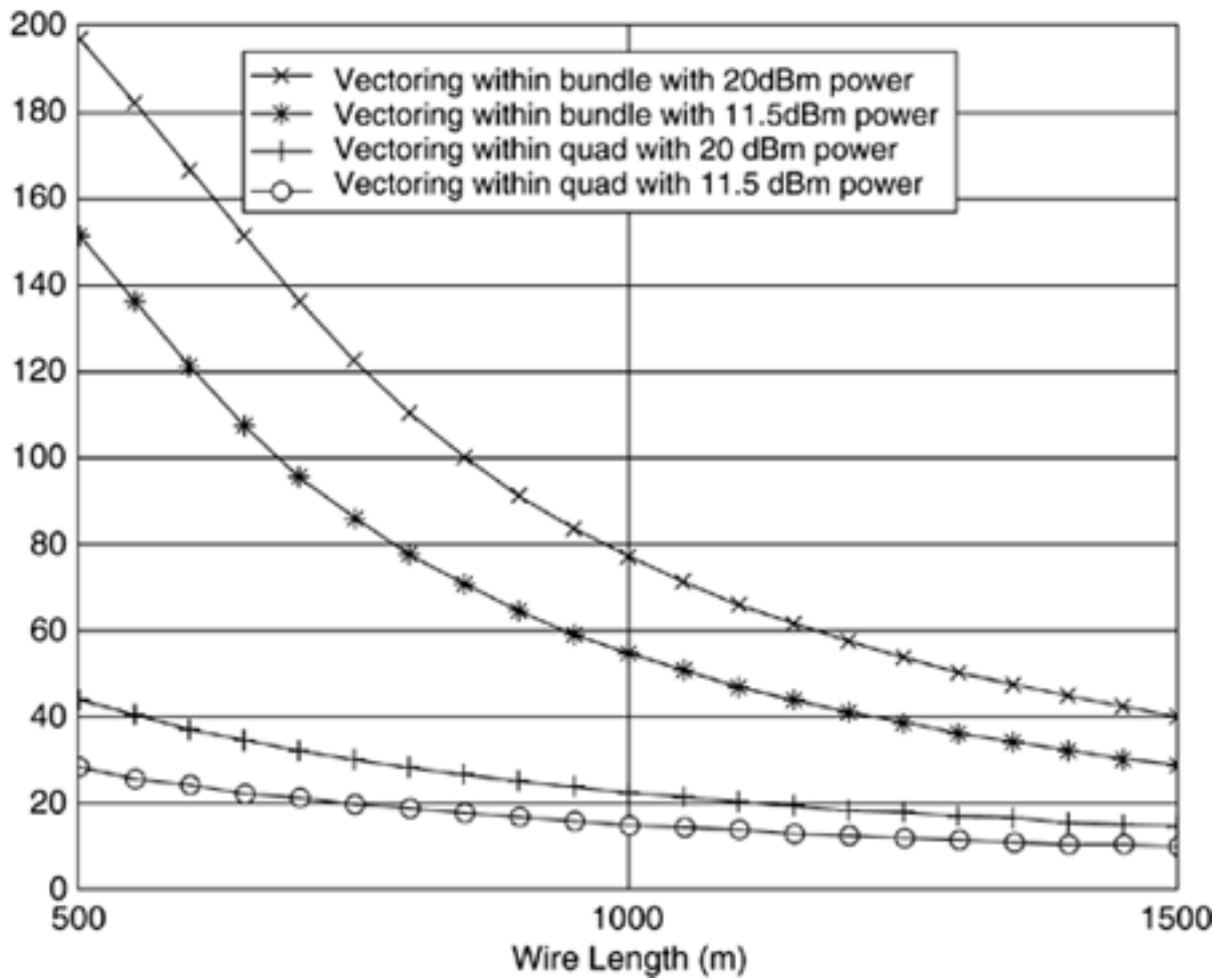
Figure 11.38. Short line EFM/VDSL results with vectored DMT "symmetric transmission over full band.
