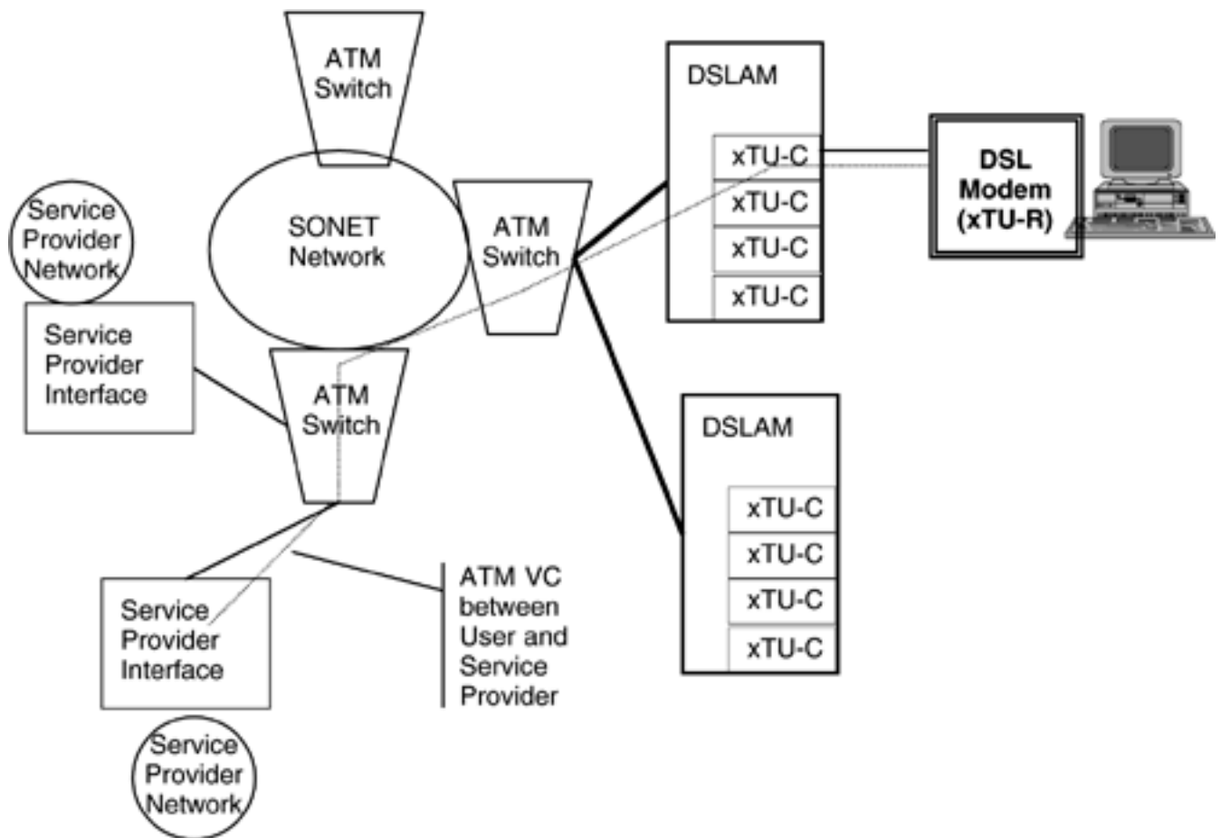
Figure 14.1. Overview of the use of ATM in DSL access architectures.
