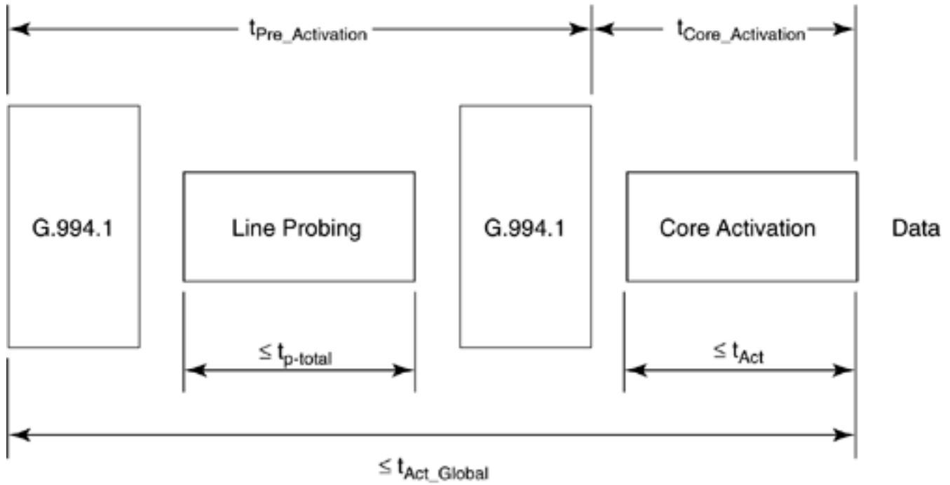
Figure 6.24. SHDSL total activation sequence.
