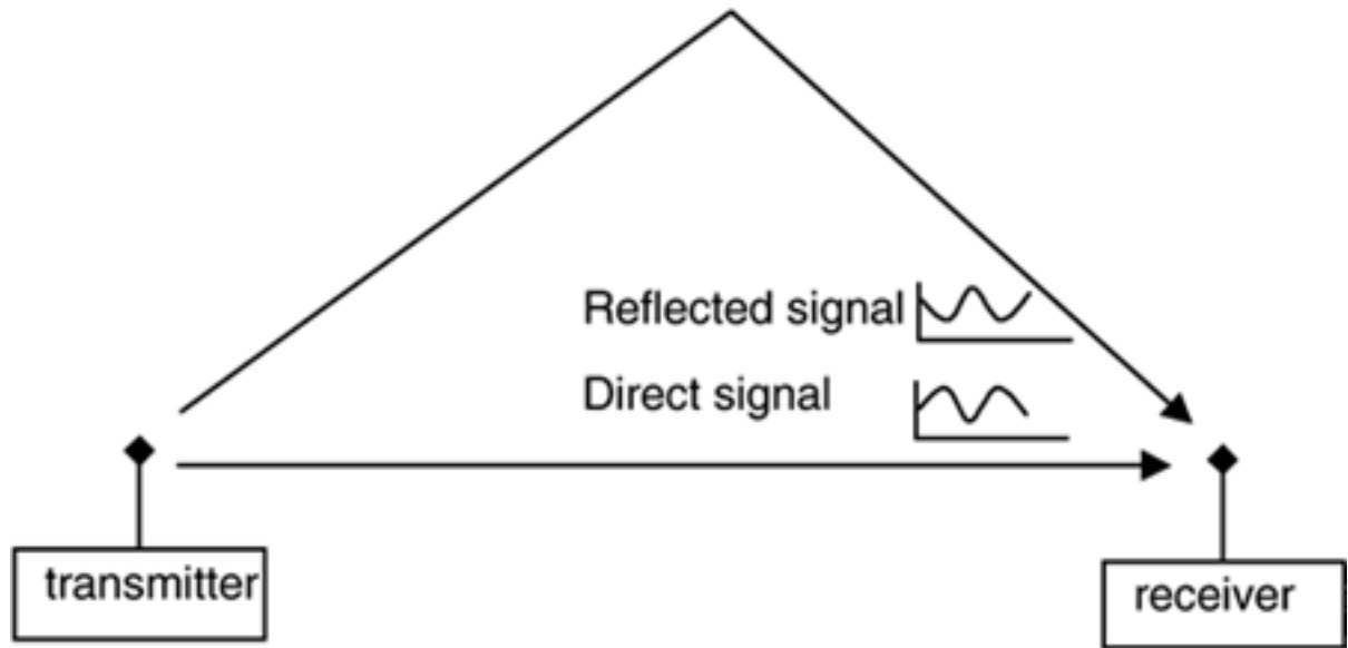
Figure 12.10. Multipath distortion.
