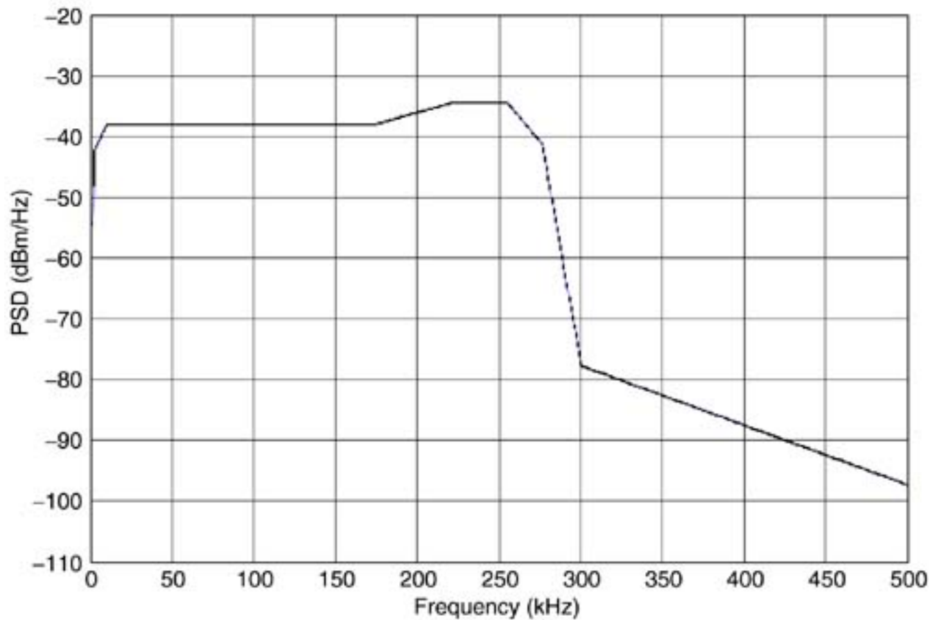
Figure 10.8. Spectrum Management Class 4 upstream template plot.
