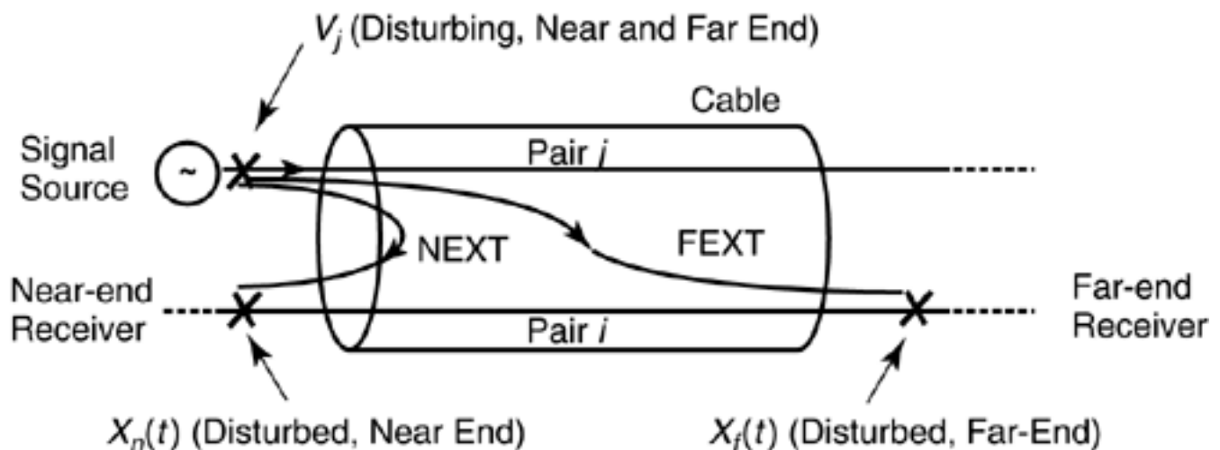
Figure 9.2. NEXT and FEXT in a multipair cable.
