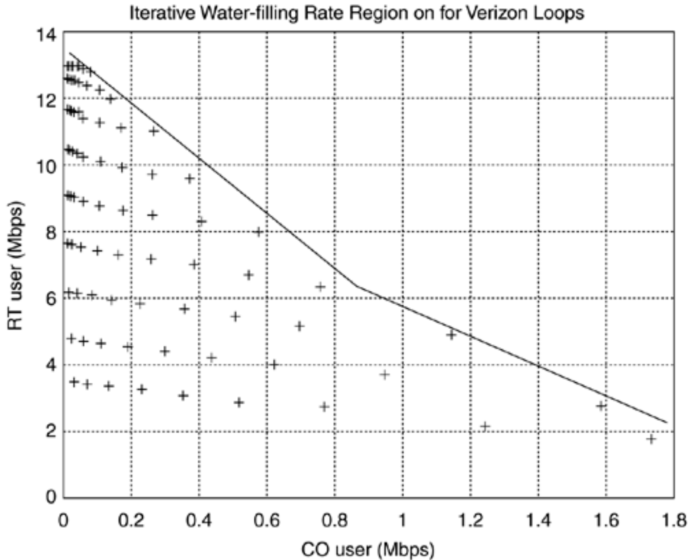
Figure 11.18. Fixed-margin iterative water-filling achievable rate region for Verizon experiment in [31].
