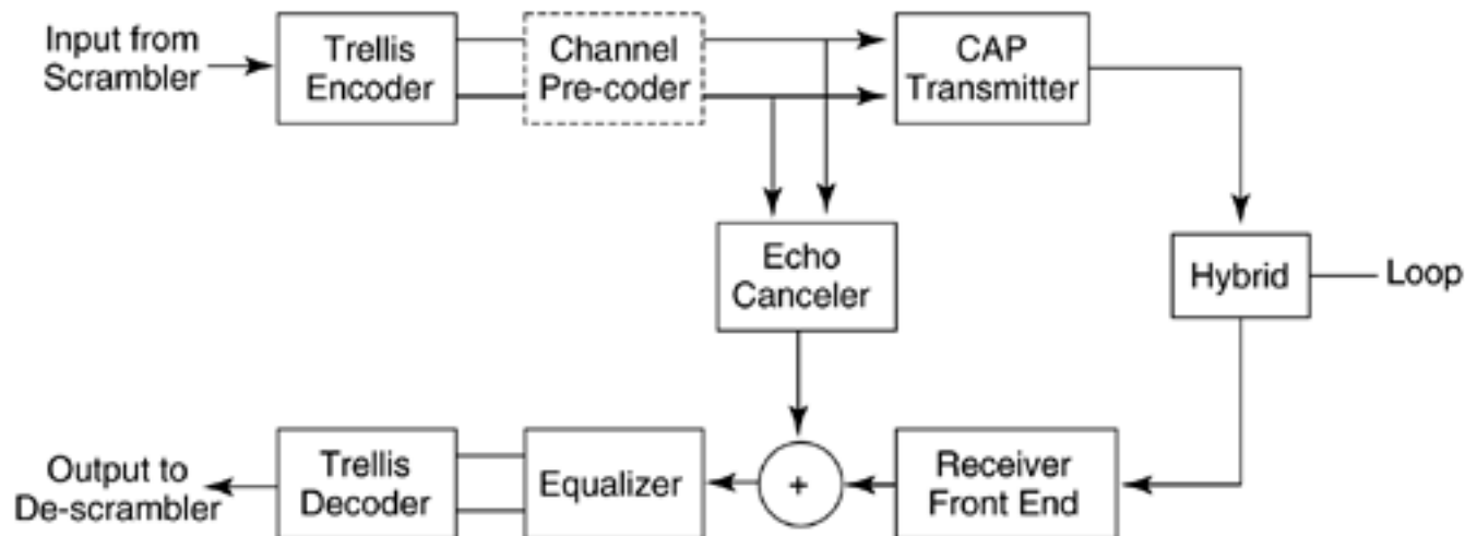
Figure 4.12. CAP-based HDSL transceiver functional block diagram.
