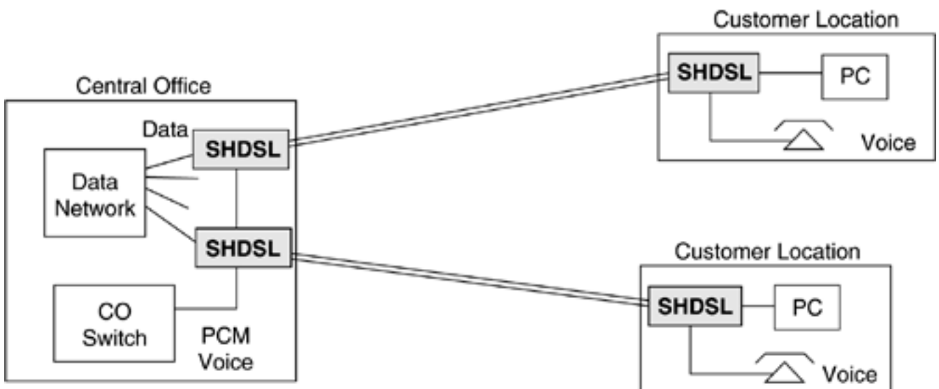
Figure 6.5. Work-at-home application "data plus PCM voice.
