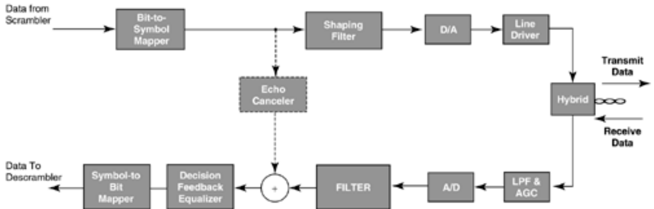
Figure 4.10. Functional block diagram of a 2B1Q HDSL transceiver.
