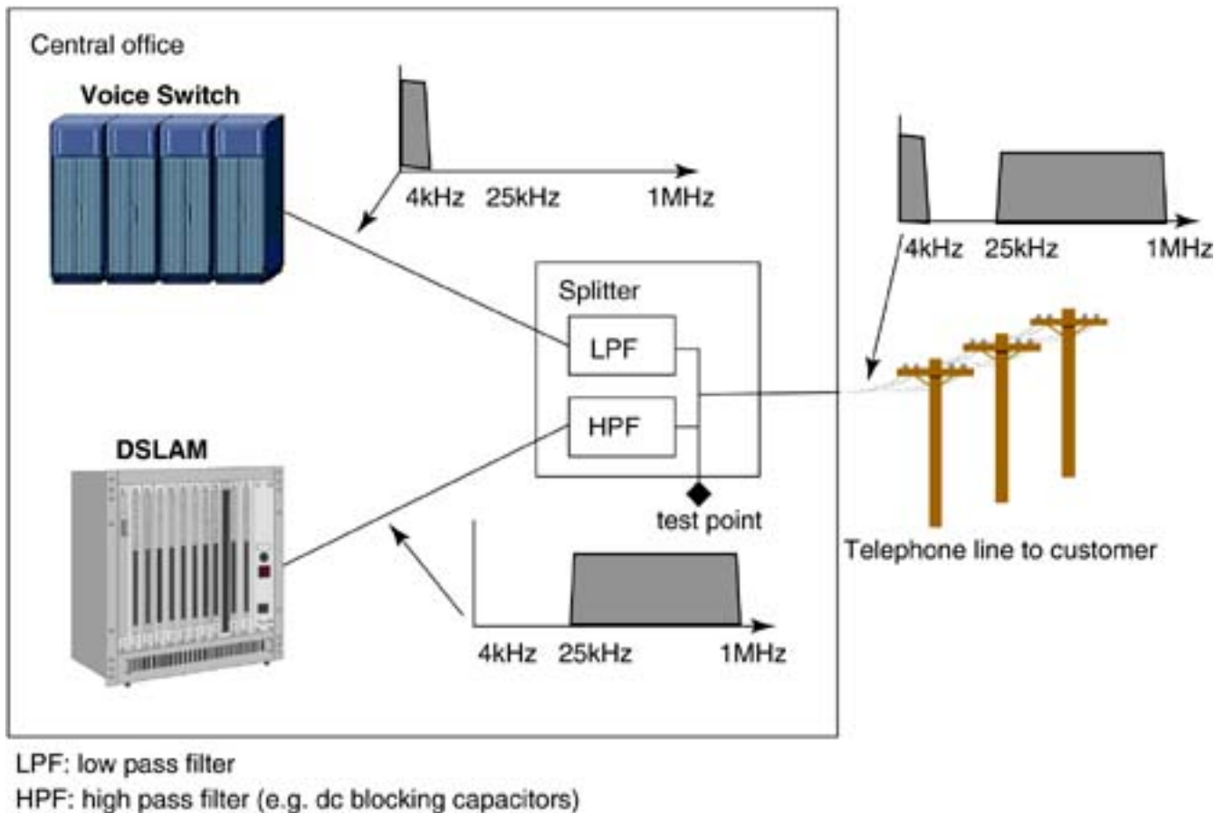
Figure 8.3. Line sharing splitter at network end of line.
