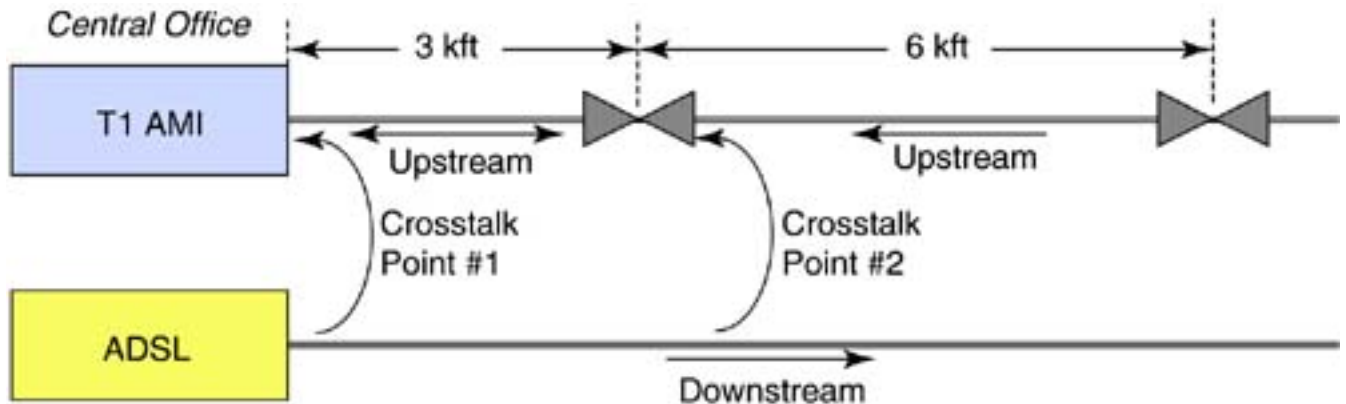
Figure 9.19. Crosstalk scenarios for DSLs into T1 AMI.
