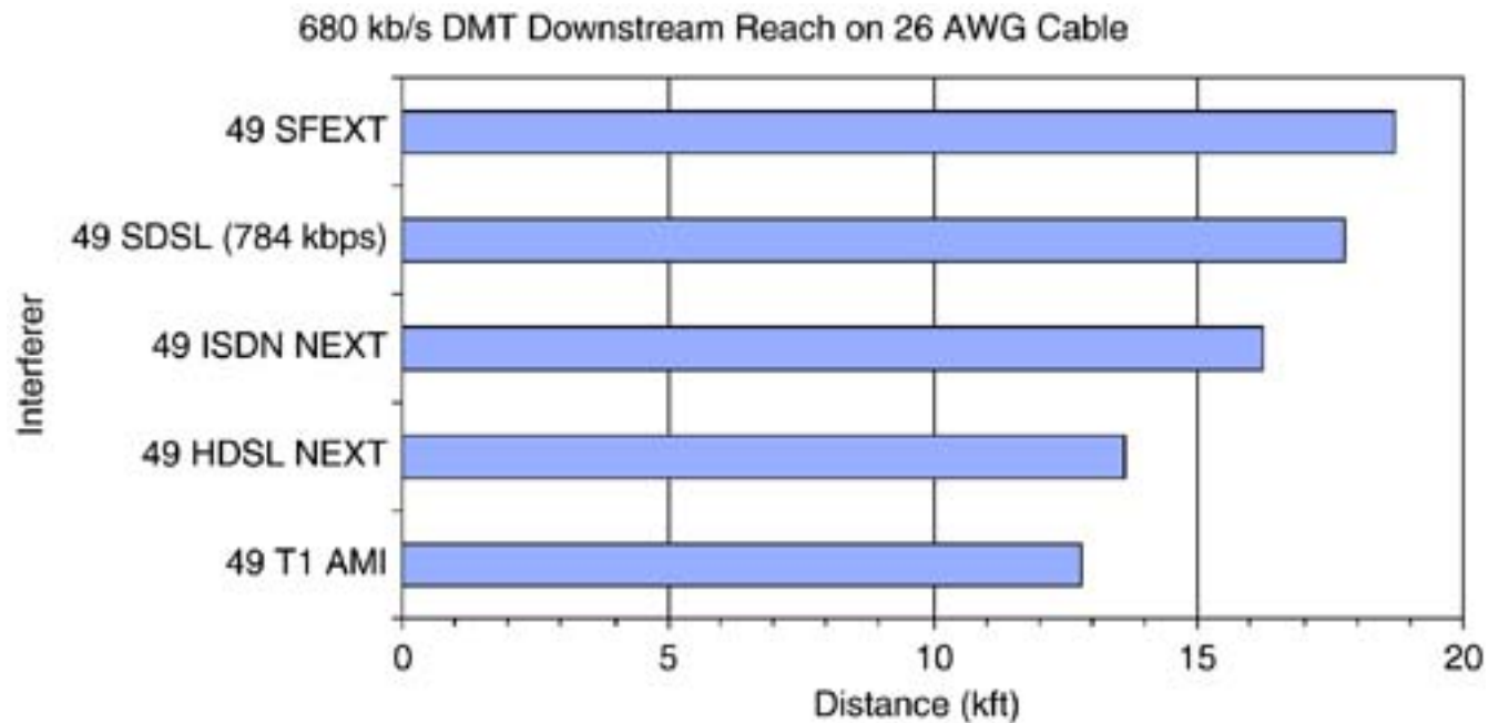
Figure 9.18. Downstream DMT spectral compatibility with other DSLs.
