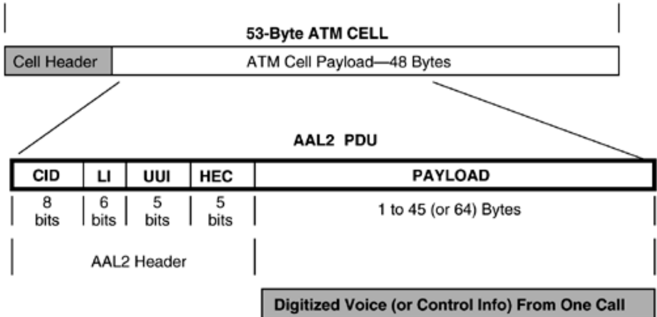
Figure 16.12. AAL2 cell structure.
