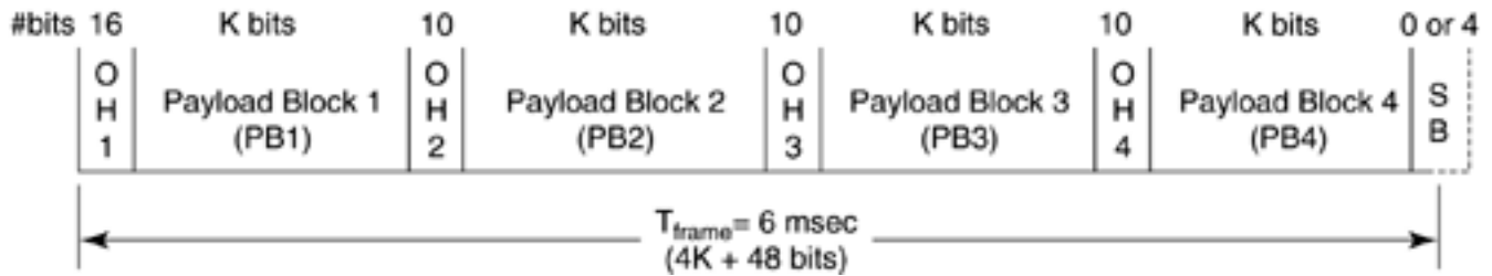
Figure 6.19. SHDSL core frame structure.
