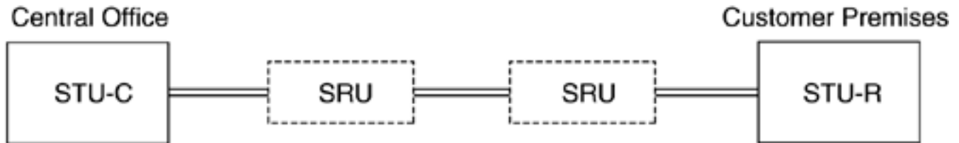
Figure 6.7. Reference model for deployment of SDHSL with repeaters.
