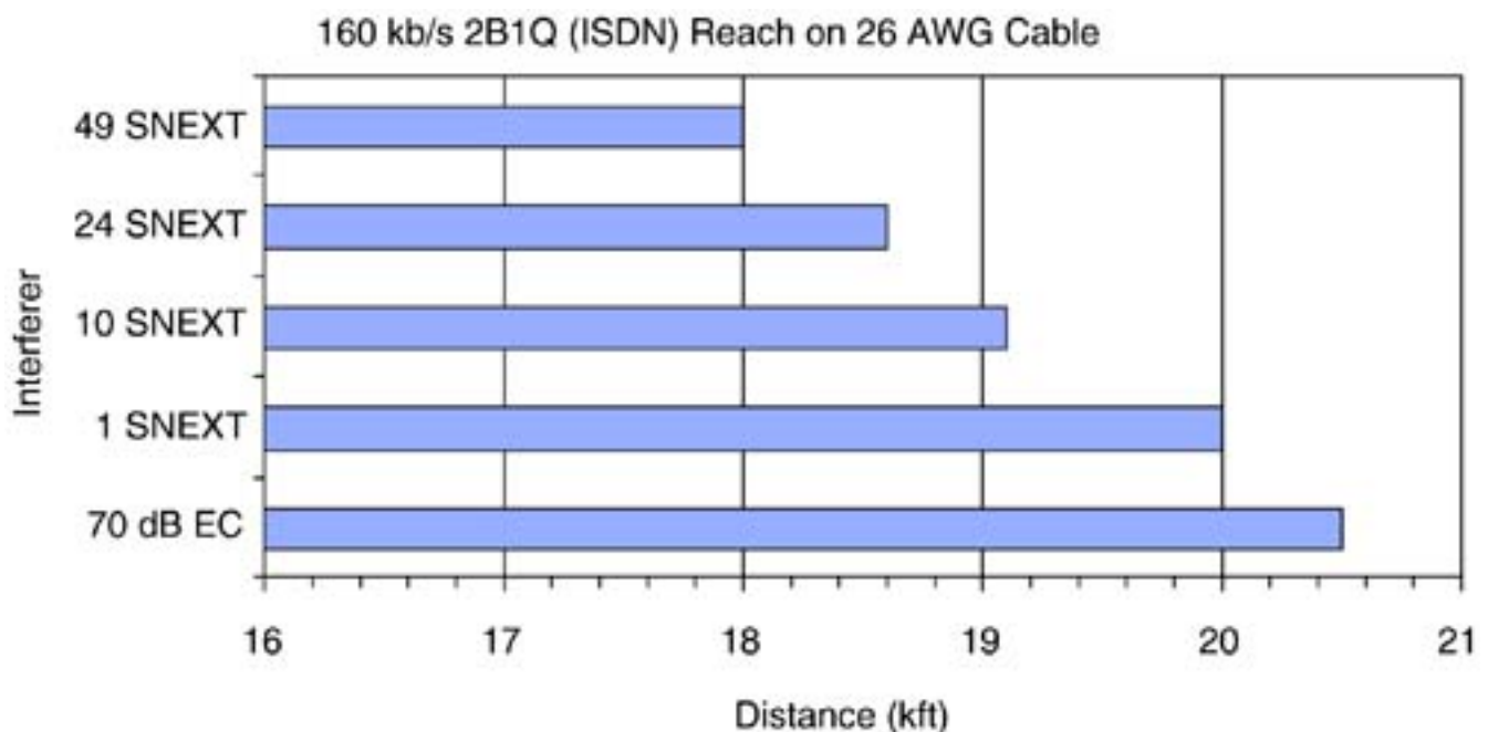
Figure 9.11. ISDN Reach as a function of SNEXT.
