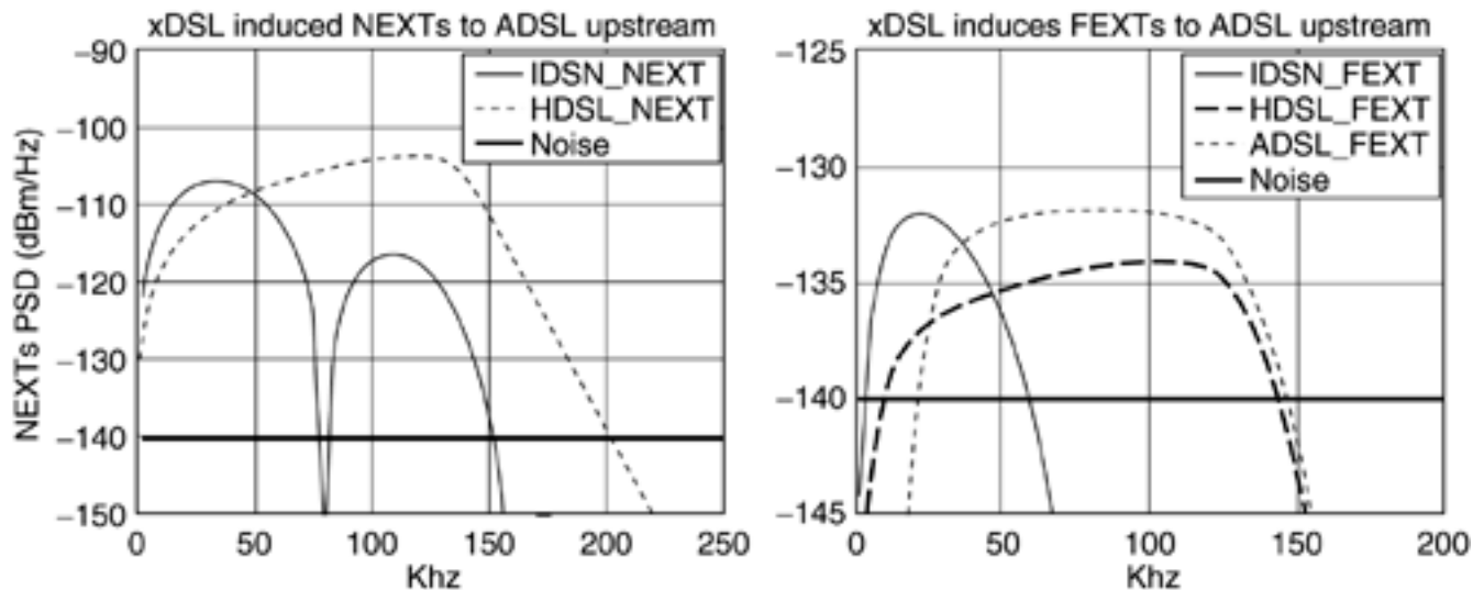
Figure 11.41. Crosstalk spectra into an upstream ADSL.
