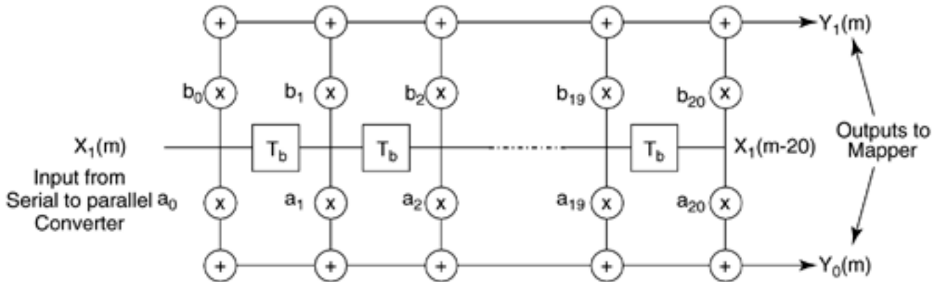
Figure 6.12. Convolutional encoder structure.
