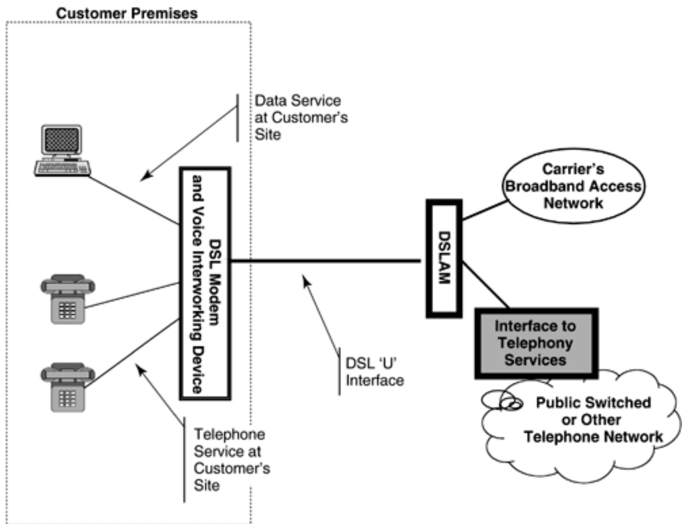
Figure 16.3. Generalized VoDSL architecture.
