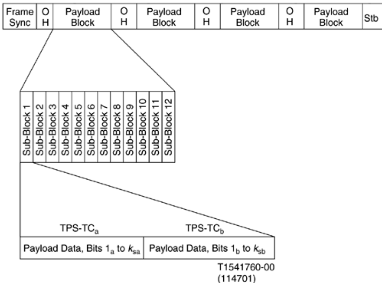
Figure 6.23. Dual bearer subchannel framing.
