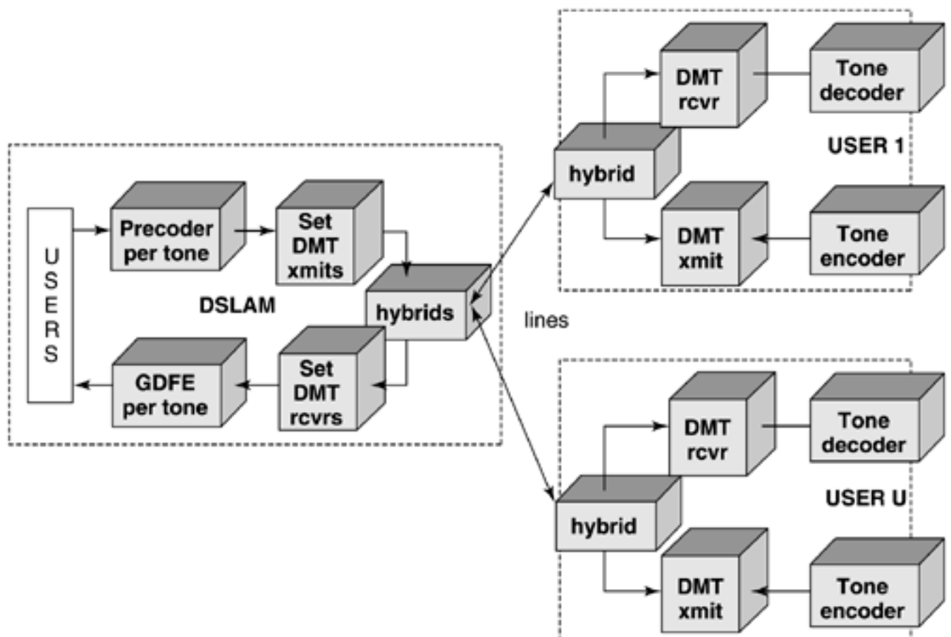
Figure 11.15. One-sided vectoring for DMT VDSL.
