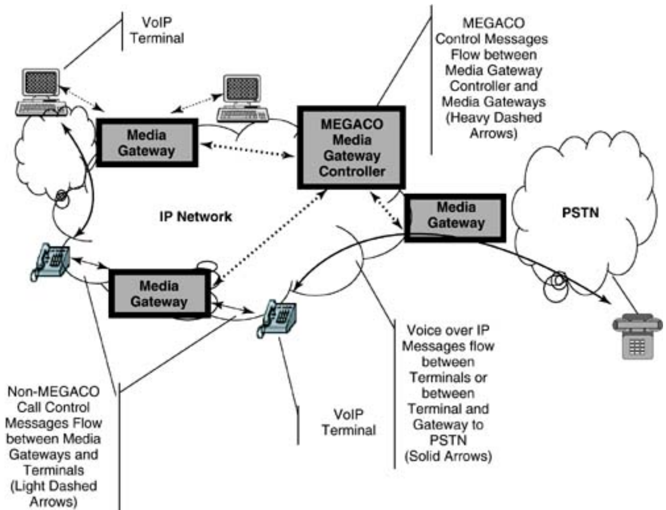
Figure 16.9. Overview of the MEGACO architecture.
