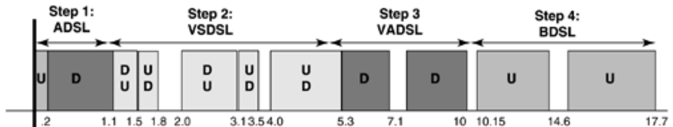
Figure 7.8. Possible VDSL rate progression and bandwidth use.
