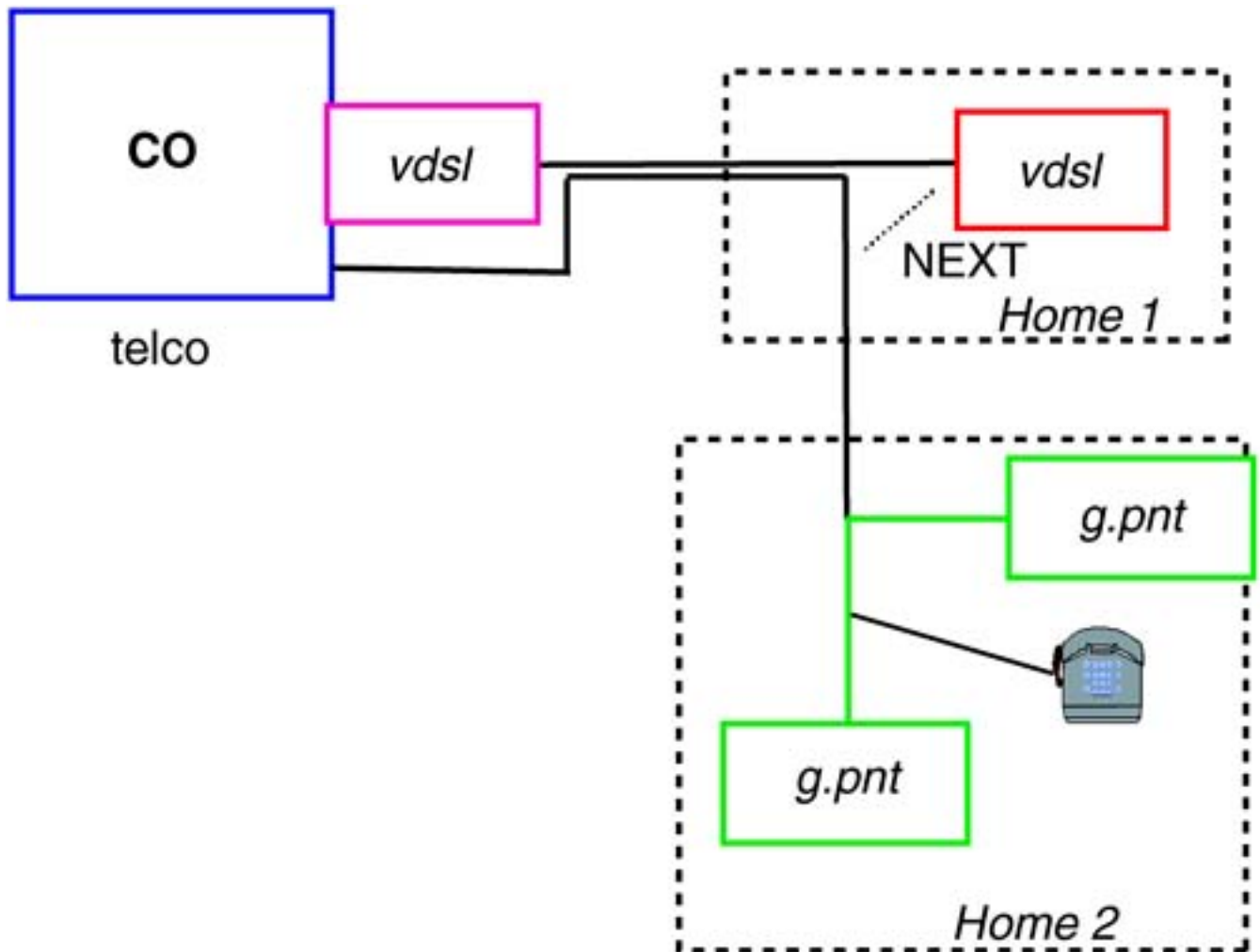
Figure 11.46(a). VDSL/G.pnt crosstalk problem.
