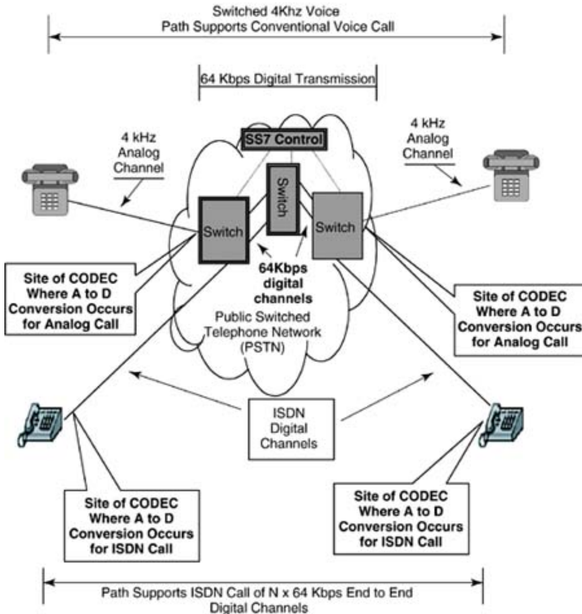
Figure 16.2. Overview of the PSTN carrying digitized telephony traffic.
