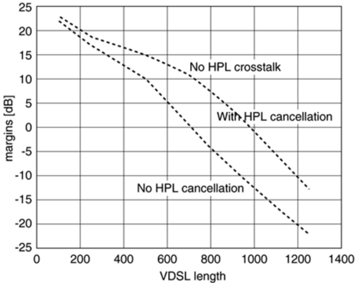
Figure 11.46(b). MUD ML detector for VDSL at 26 Mbps.
