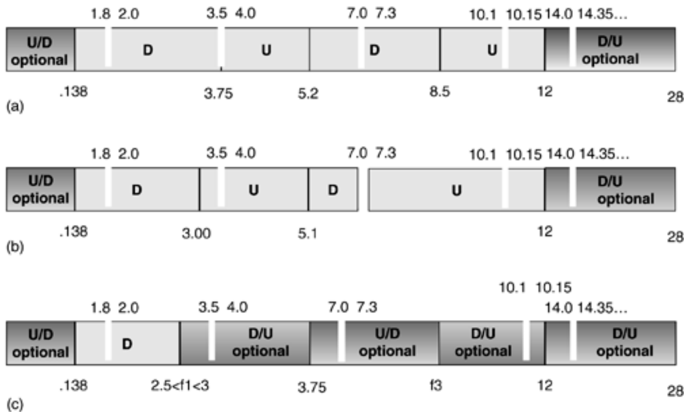
Figure 7.4. (a) Plan 998 "North American, United Kingdom, and Japan VDSL spectrum. (Additional radio bands notched when used at 18.068 "18.168, 21 "21.45, 24.89 "24.99 MHz). (b) Plan 997 "VDSL Spectrum for some European countries. (Same unshown notched bands as Figure 7.4(a). (c) International flexible VDSL Spectrum Plan (f1, f2, f3, f4 determined programmably).
