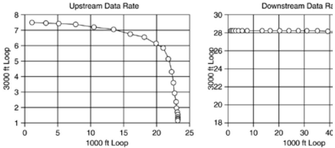
Figure 11.30. VDSL flexible upstream and downstream rate regions for 4 each of 1000 and 3000 ft loops in same binder with Level 0 distributed water-filling, but Level 1 control of up/down cut-off frequencies.
