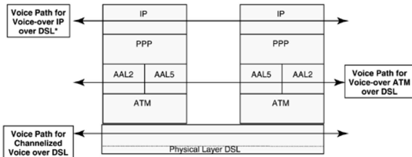
Figure 16.7. VoDSL architecture on the communications stack.
