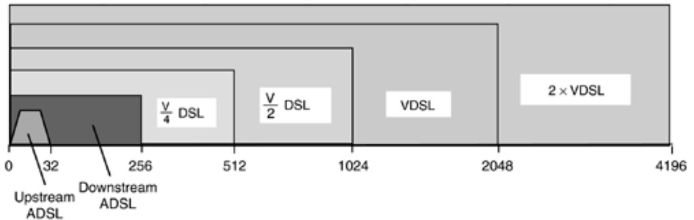
Figure 7.12. Interoperability diagram for standardized DMT modems of increasing speeds.
