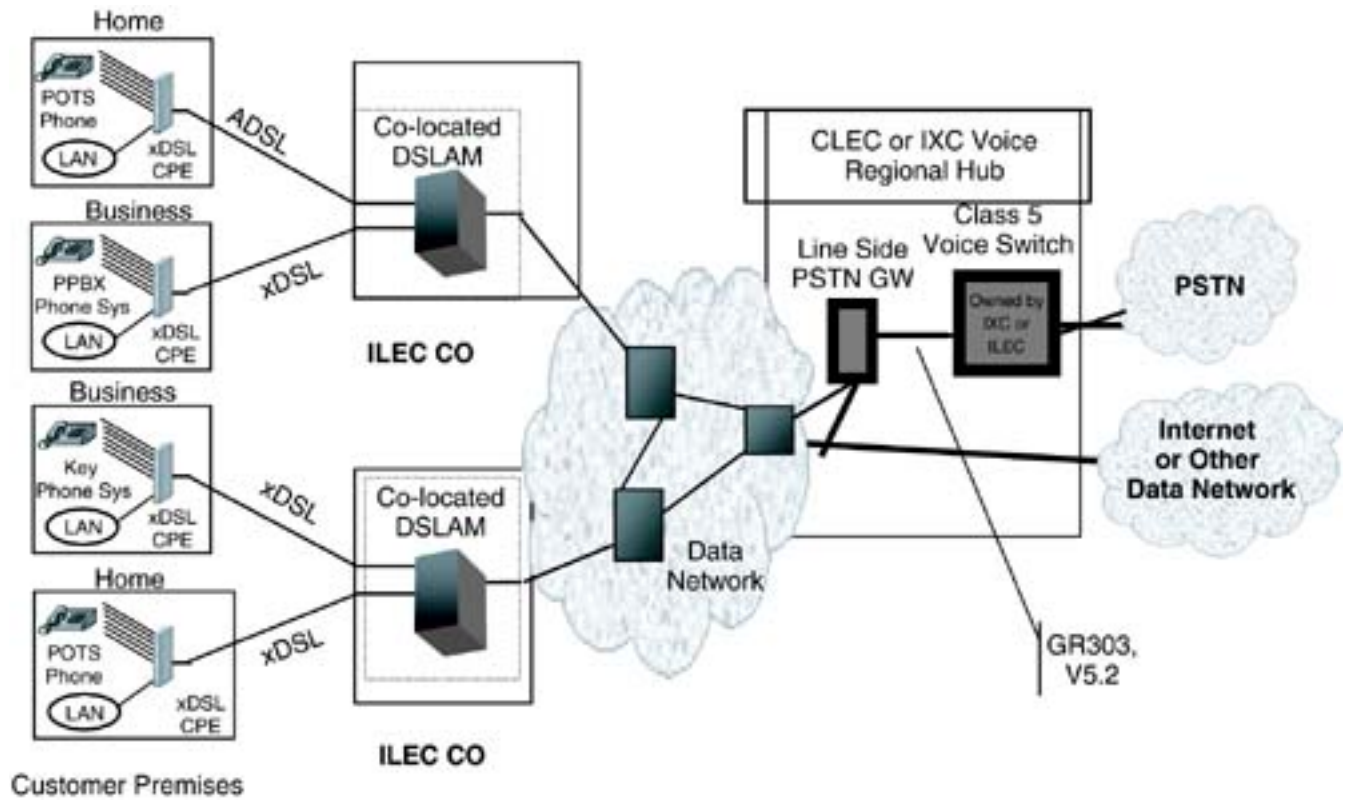
Figure 16.18. Loop extension architecture for CLEC.
