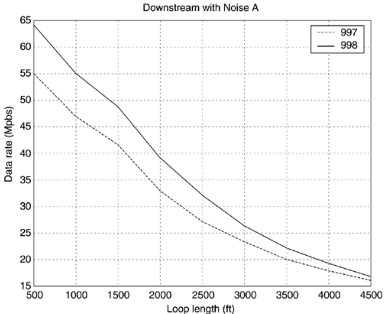
Figure 7.2(a). Downstream data rates for Frequency Plans 997 and 998 in draft standard DMT VDSL [17].
