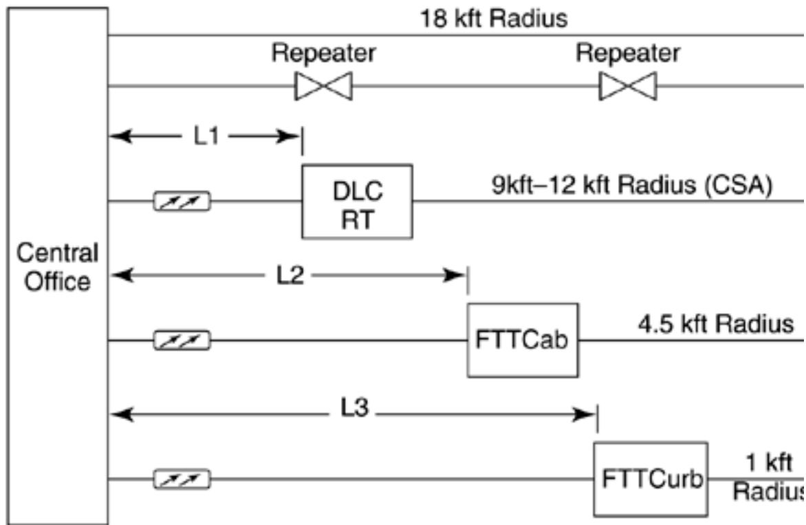
Figure 10.1. Deployment scenarios in the cable plant.
