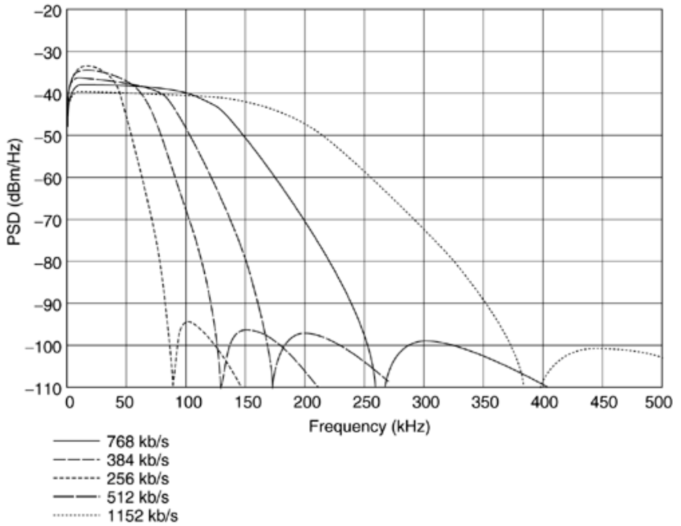
Figure 6.15. Nominal PAM PSDs without noise floor.
