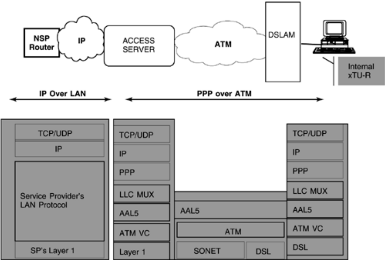
Figure 14.5. PPP over ATM stack.
