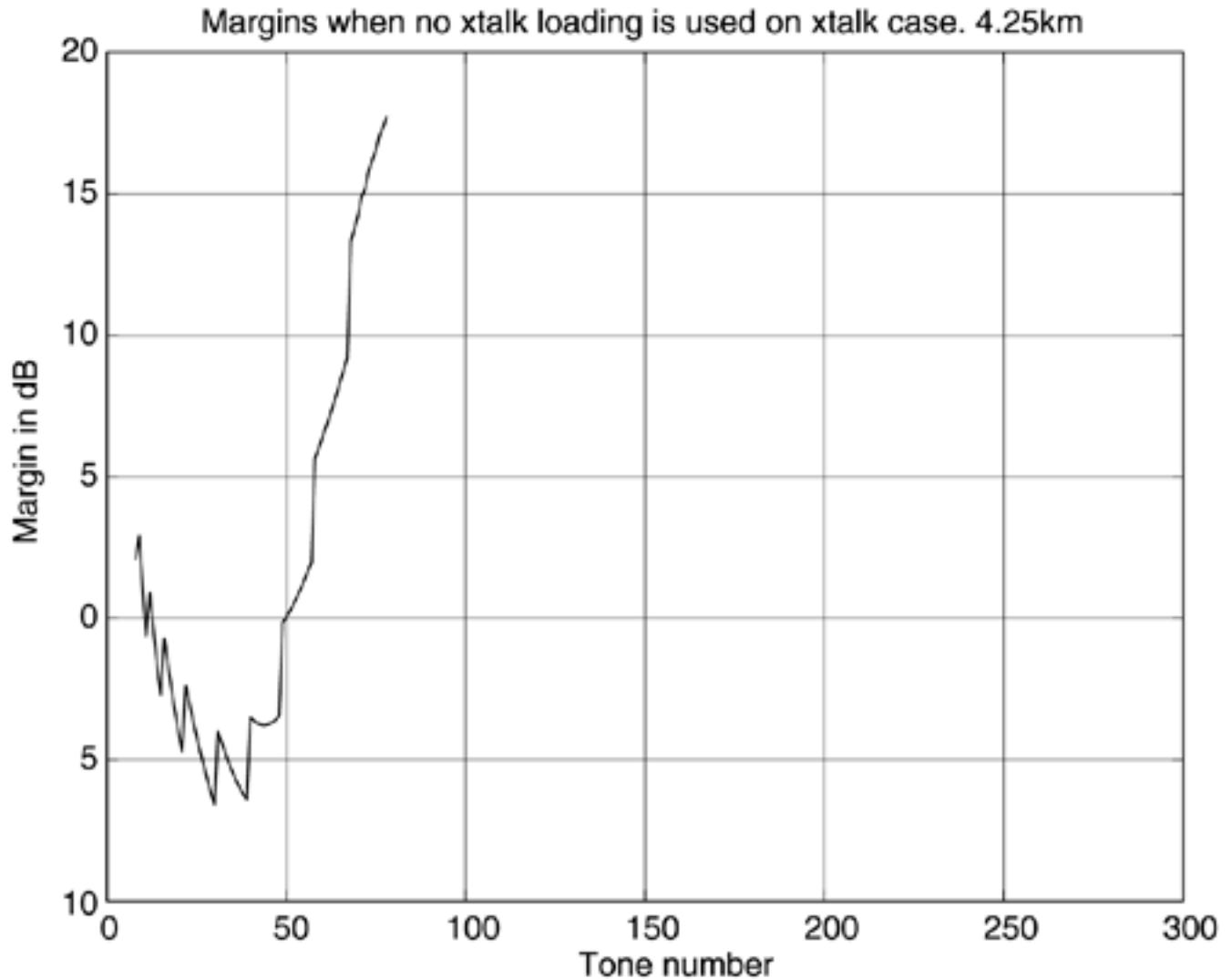
Figure 3.14. Margin for NO SWAPPING when the crosstalk is turned on.
