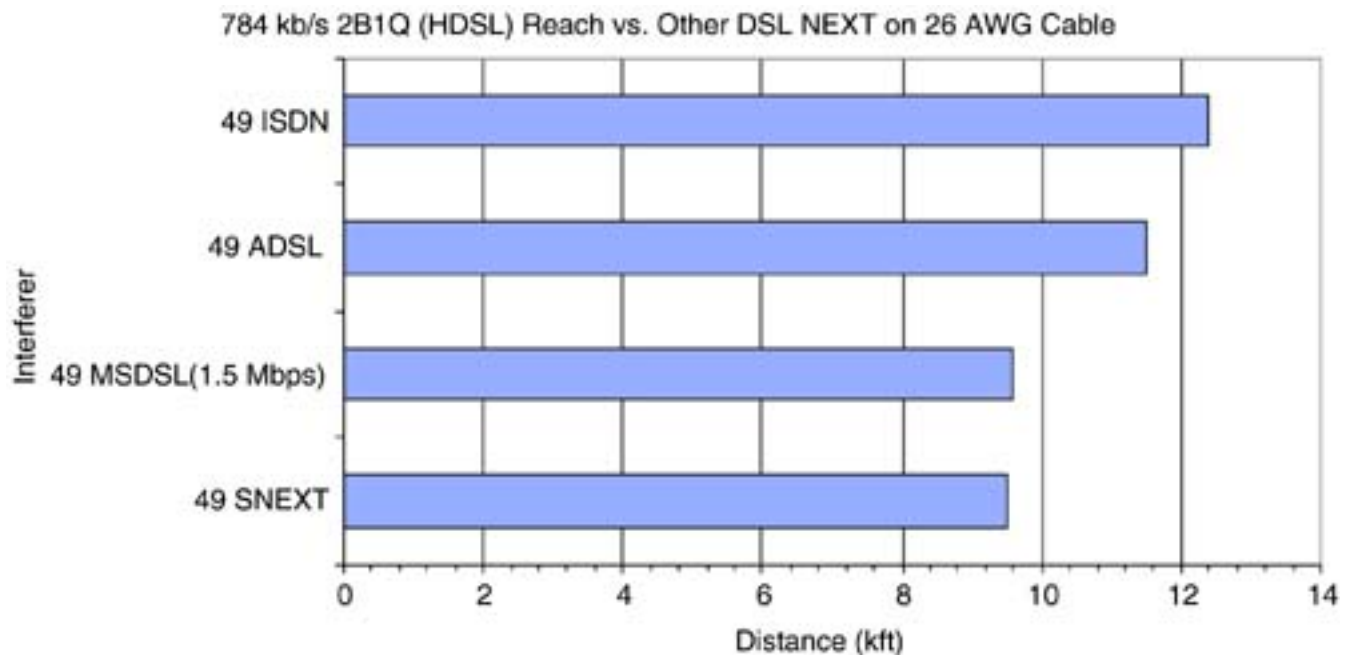
Figure 9.15. HDSL reach as a function of NEXT from other services.
