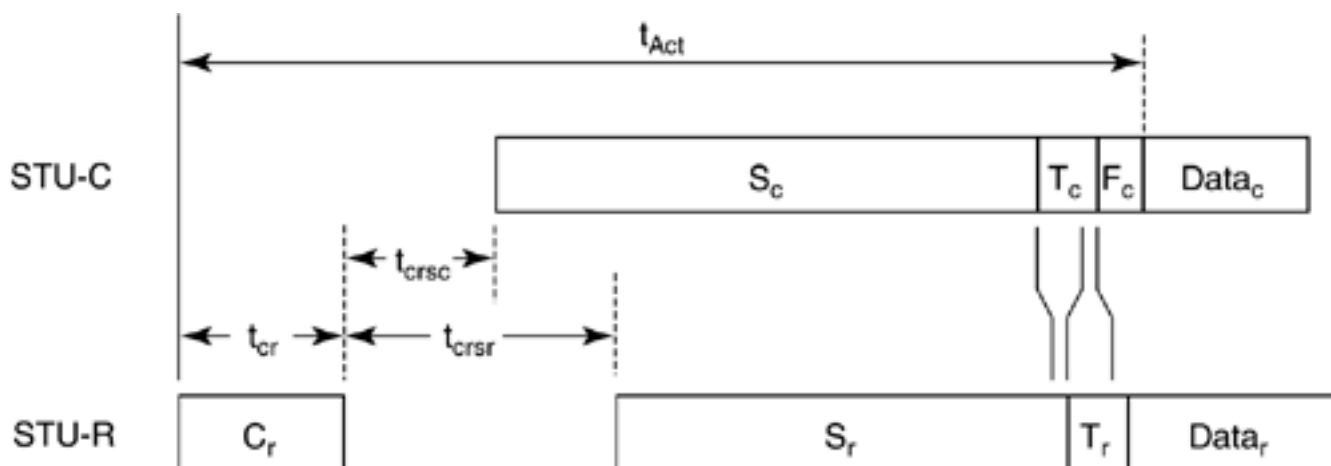
Figure 6.26. SHDSL core activation sequence.
