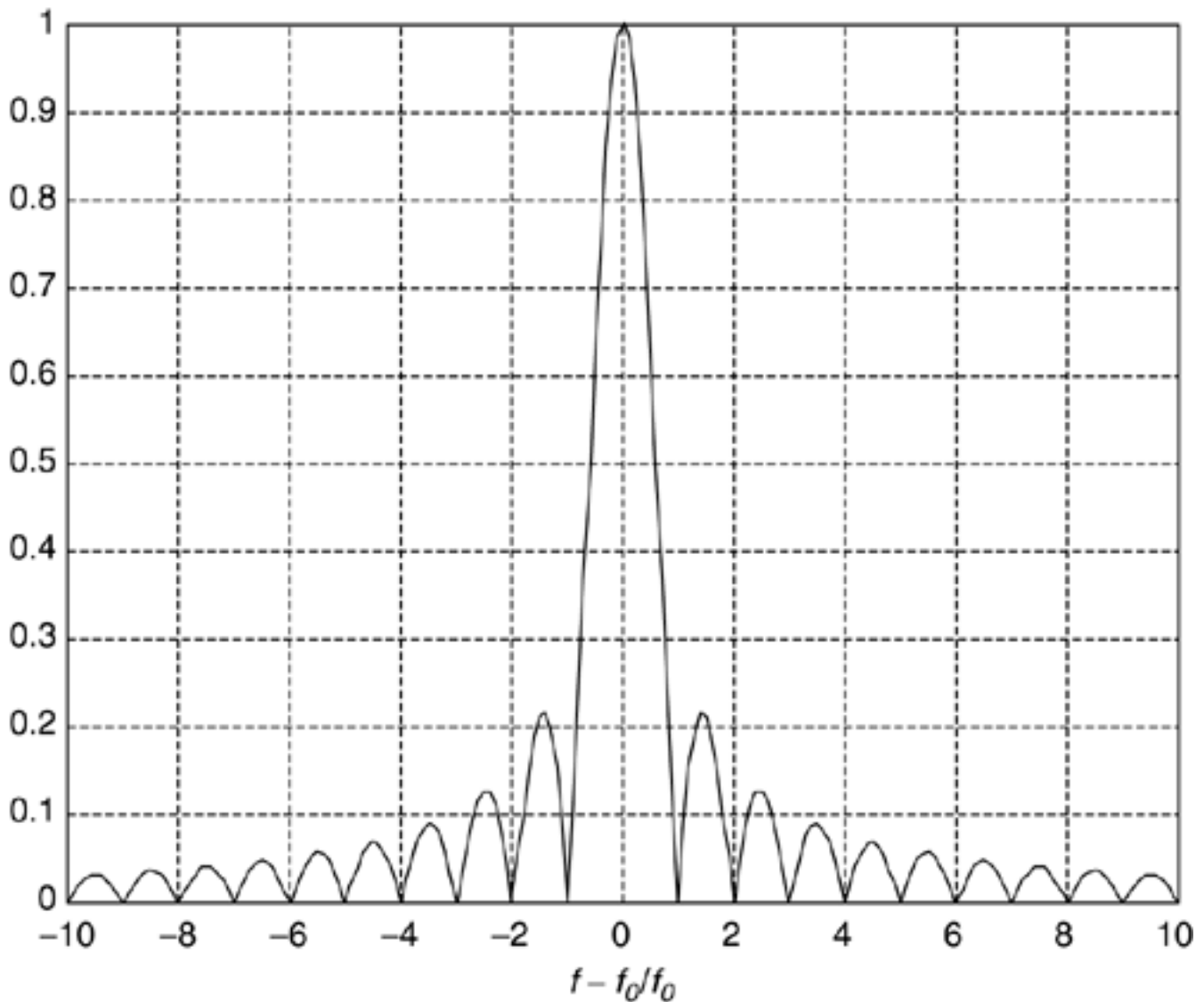
Figure 7.17. Magnitude of windowed sinusoid versus frequency. Note notches at DMT frequencies.
