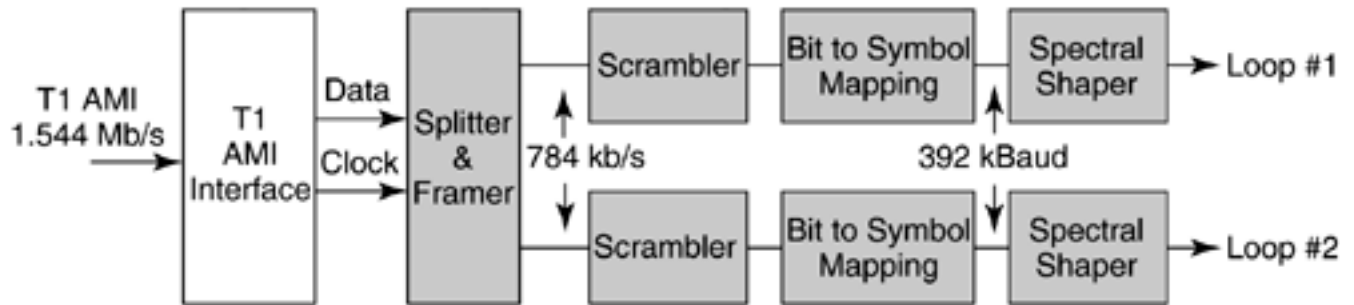
Figure 4.5. HDSL transmitter structure for lines #1 and #2.
