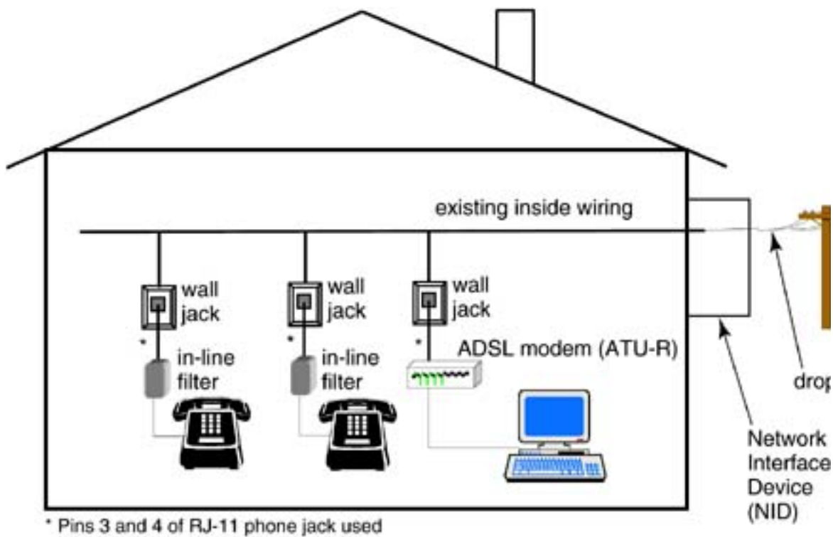
Figure 12.2. Splitterless customer premises configuration.
