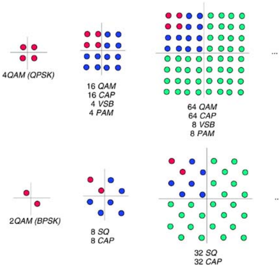
Figure 2.8. QAM/CAP square constellations.
