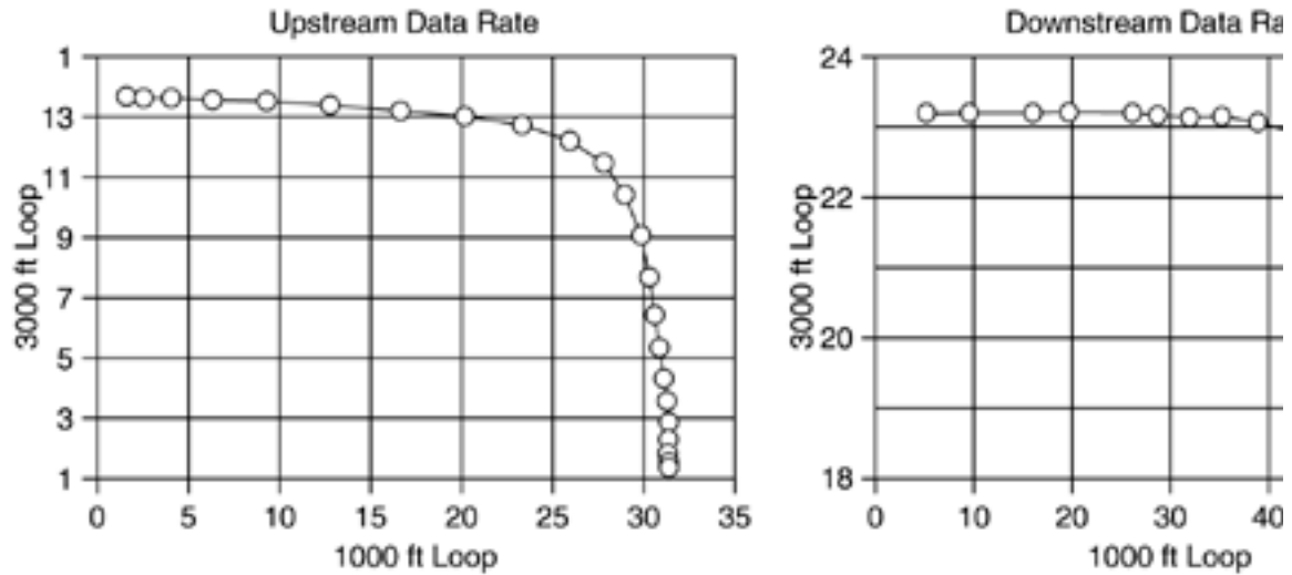
Figure 11.36. Vectored ADSL data rates versus range.
