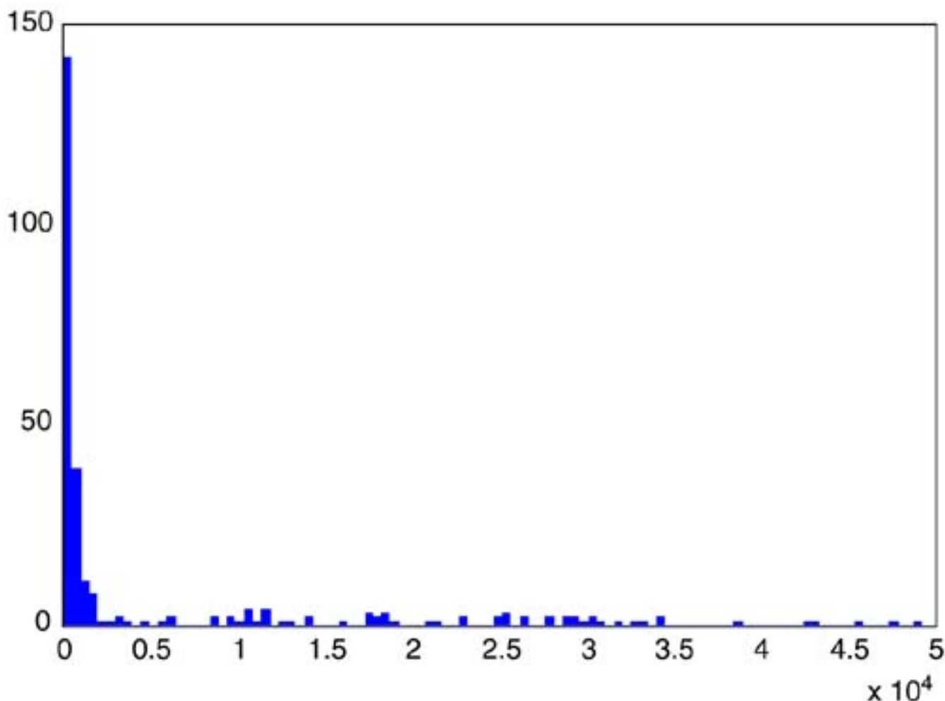
Figure 3.7. Impulse duration histogram (horizontal axis is \mu s, to 50 ms spanned ). Courtesy France Telecom [6].
