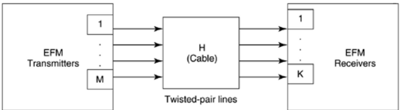
Figure 7.28. Matrix channel.
