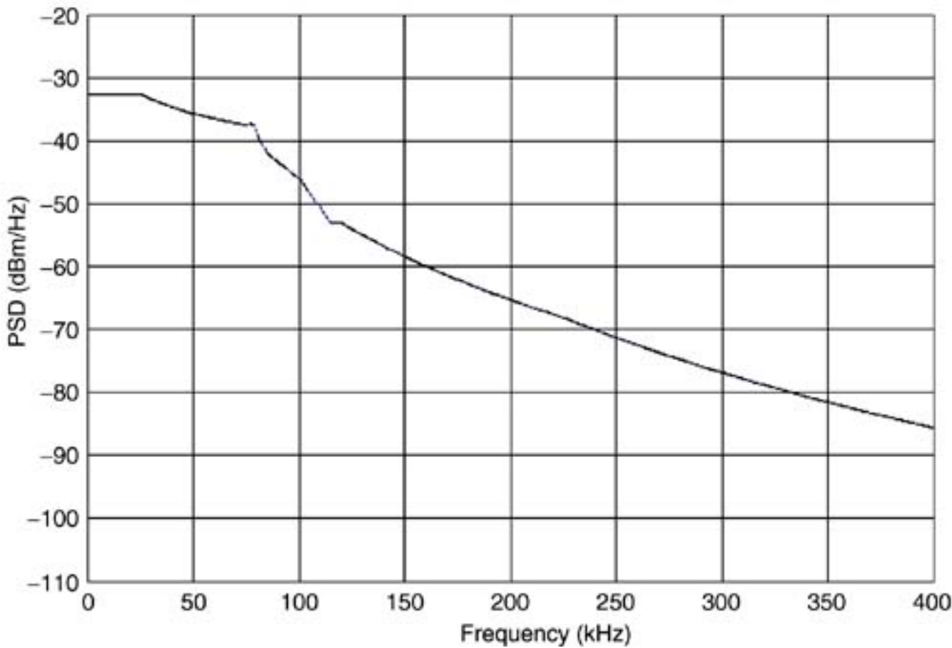
Figure 10.4. Spectrum management class 1 template plots.
