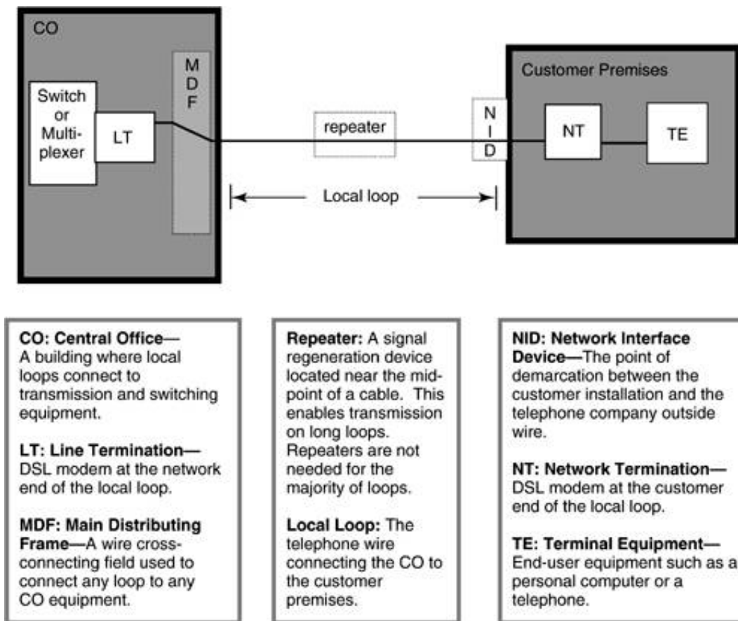
Figure 1.1. DSL Reference Model
