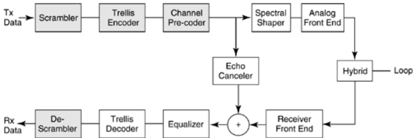
Figure 4.14. General transceiver functional block diagram for HDSL2.
