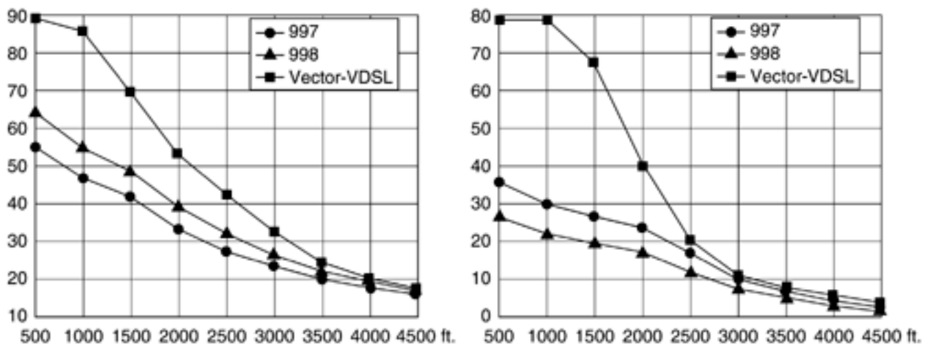
Figure 11.37. Vectored VDSL data rates versus range.
