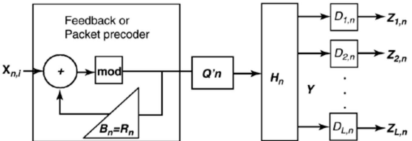
Figure 11.35. Exact illustration for one tone (n) of GDFE downstream vector receiver.
