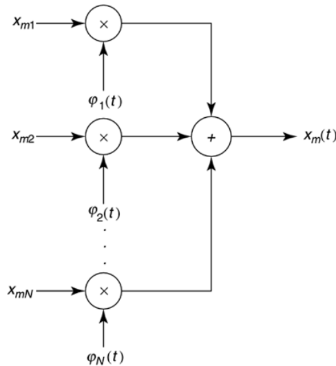
Figure 2.2. Linear modulator.
