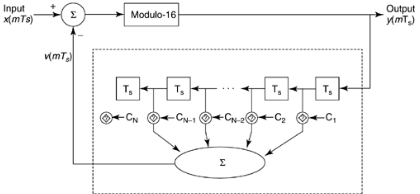
Figure 6.14. Channel precoder.
