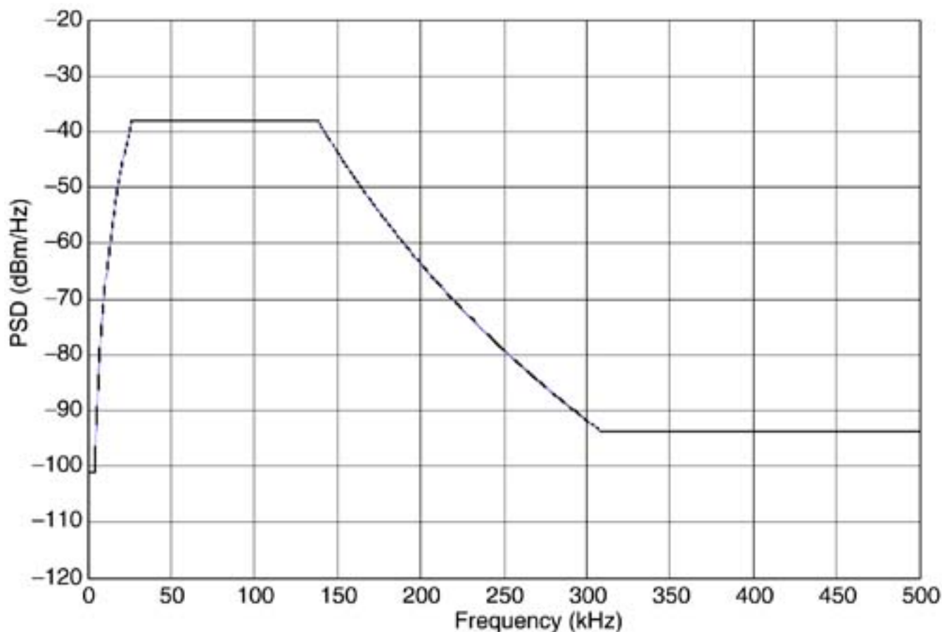
Figure 10.12. Spectrum Management Class 5 or Class 9 upstream template plots.
