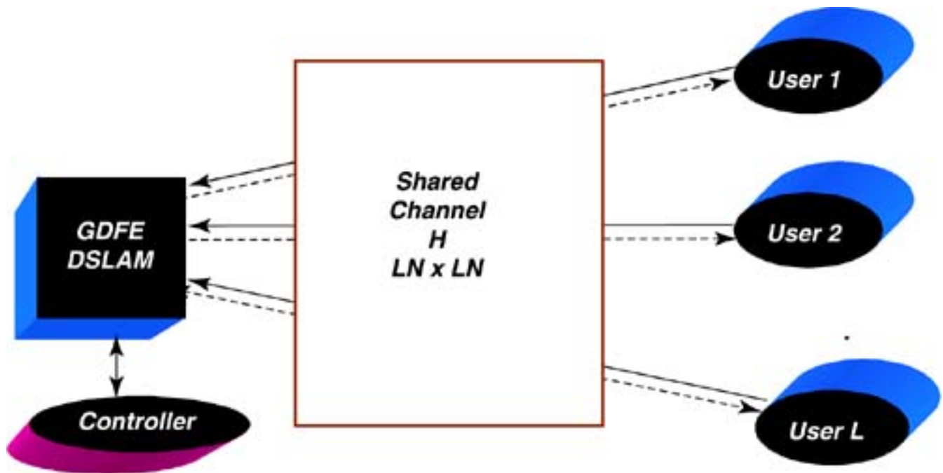
Figure 11.33. Vector multiple-access system for upstream DSL with coordinated reception but separated transmitters.
