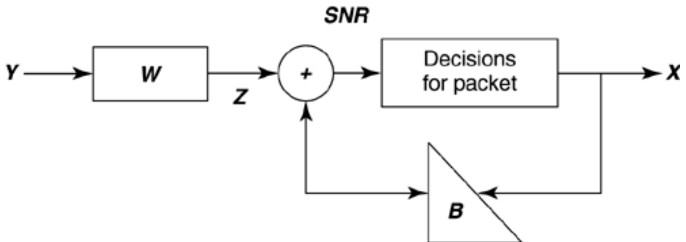
Figure 11.13. Generalized decision feedback equalization.
