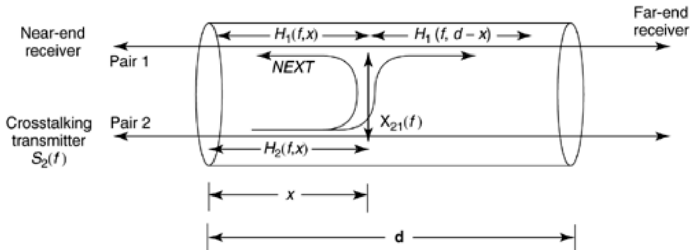
Figure 2.15. Illustration of crosstalk.
