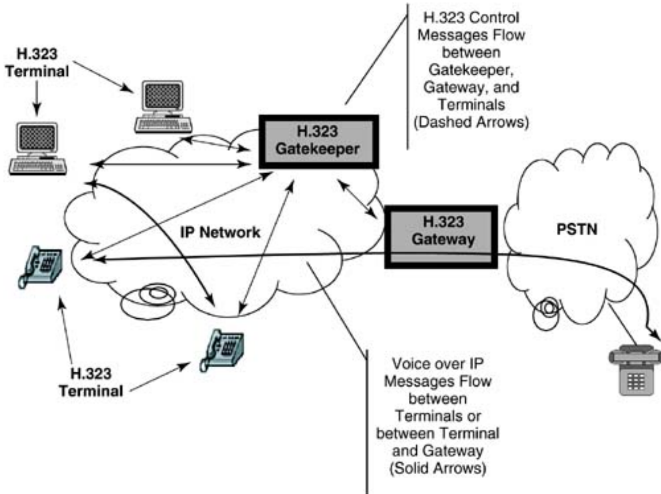
Figure 16.8. H.323 architecture for VoIP.
