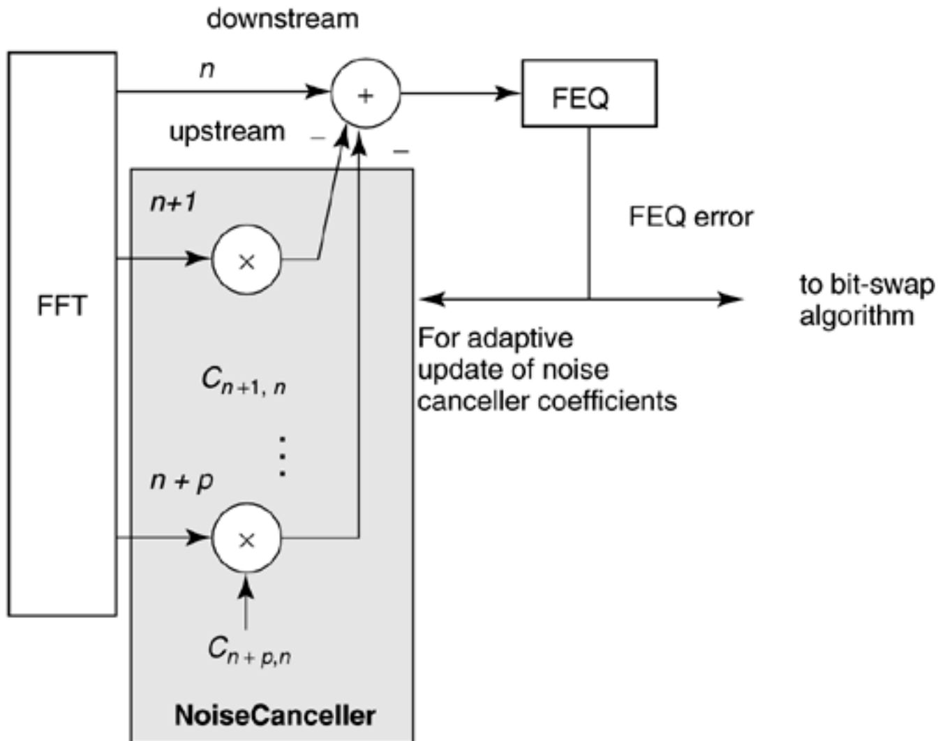
Figure 7.21. Adaptive noise canceller for elimination of VDSL self-NEXT in asynchronous VDSL operation. Shown for one upstream/downstream boundary tone (can be replicated for each up/down transition tone that has NEXT distortion with asynchronous VDSL NEXT). No canceler necessary if NEXT is synchronous.
