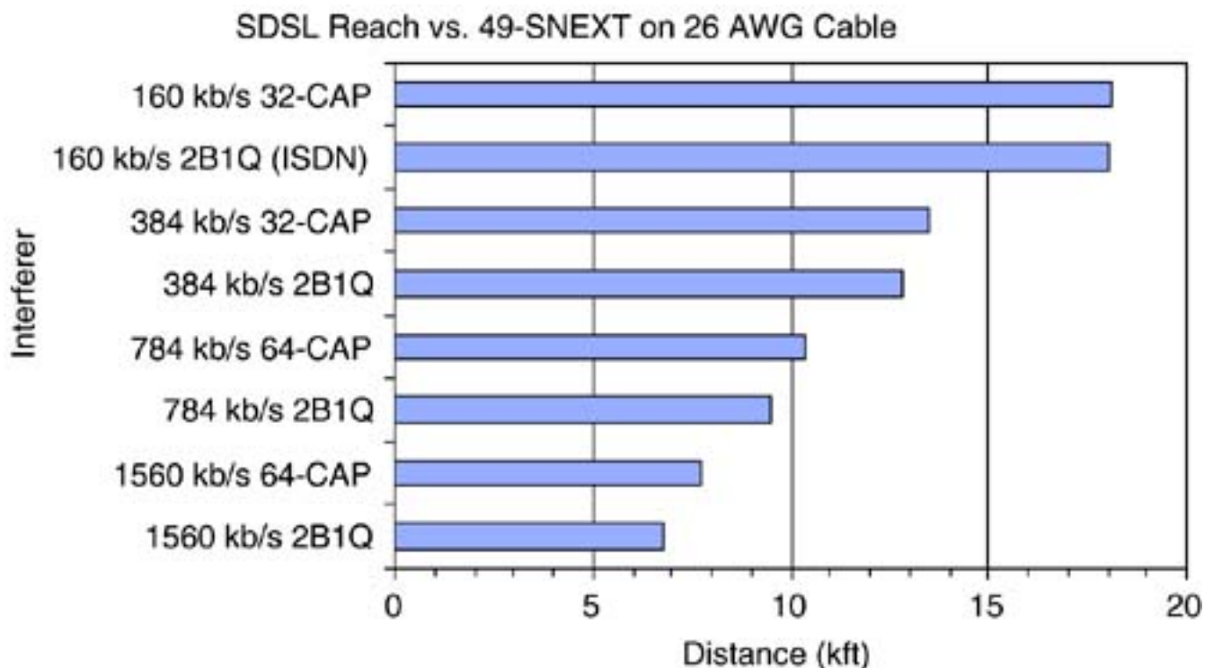
Figure 9.16. SDSL reach versus 49-SNEXT.
