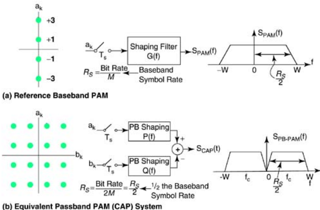
Figure 4.11. Example equivalent baseband and passband systems.
