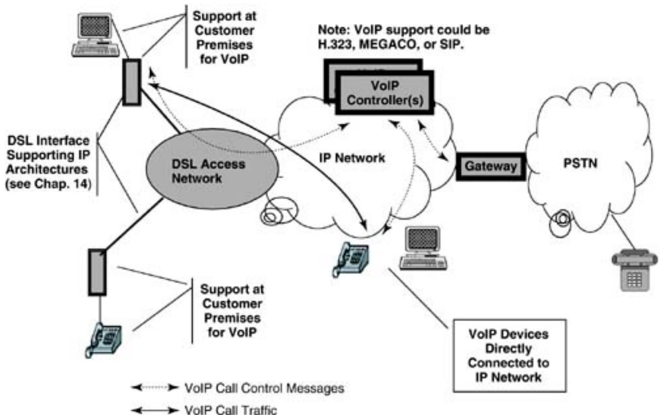
Figure 16.15. Access to packetized voice architectures.
