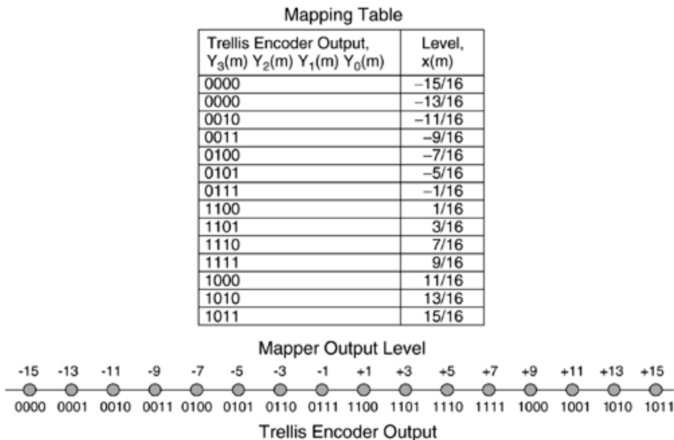
Figure 6.13. SHDSL bit-to-symbol mapping.
