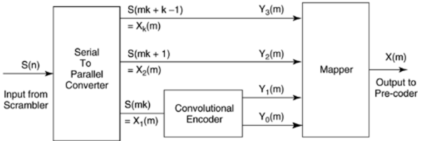
Figure 4.19. HDSL2 trellis encoder structure.
