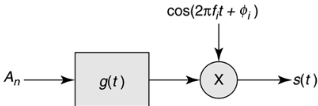
Figure 5.2. DPSK modulator block diagram.
