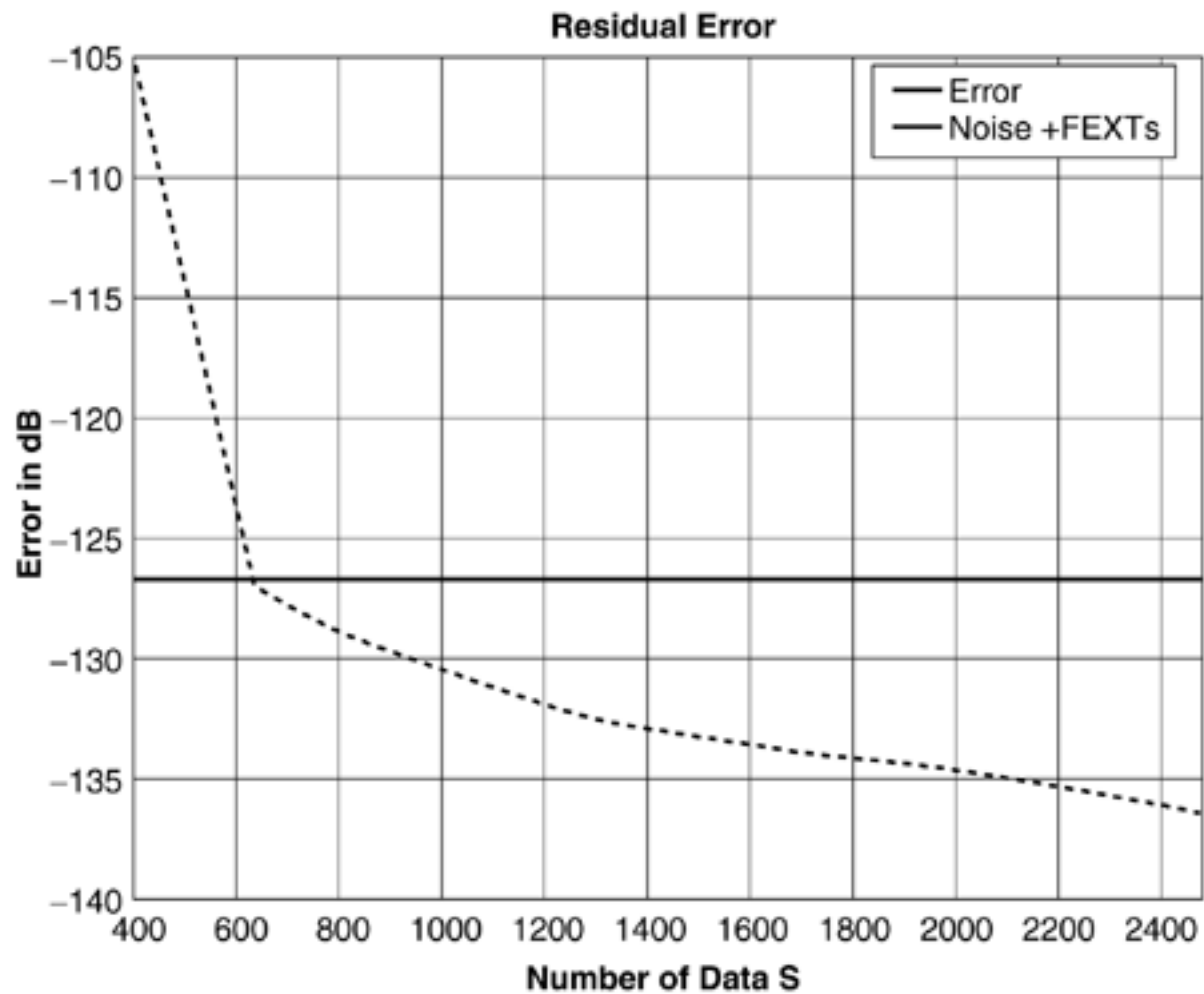
Figure 11.43. Estimation error for channel identification procedure.
