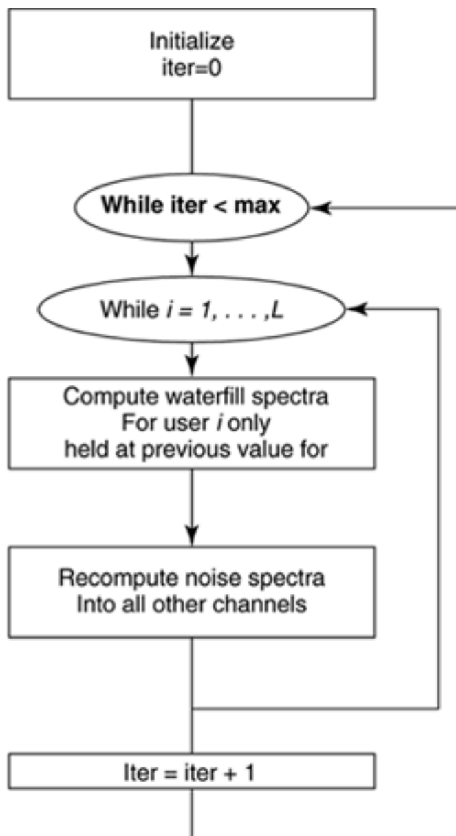
Figure 11.16. Iterative water-filling concept.
