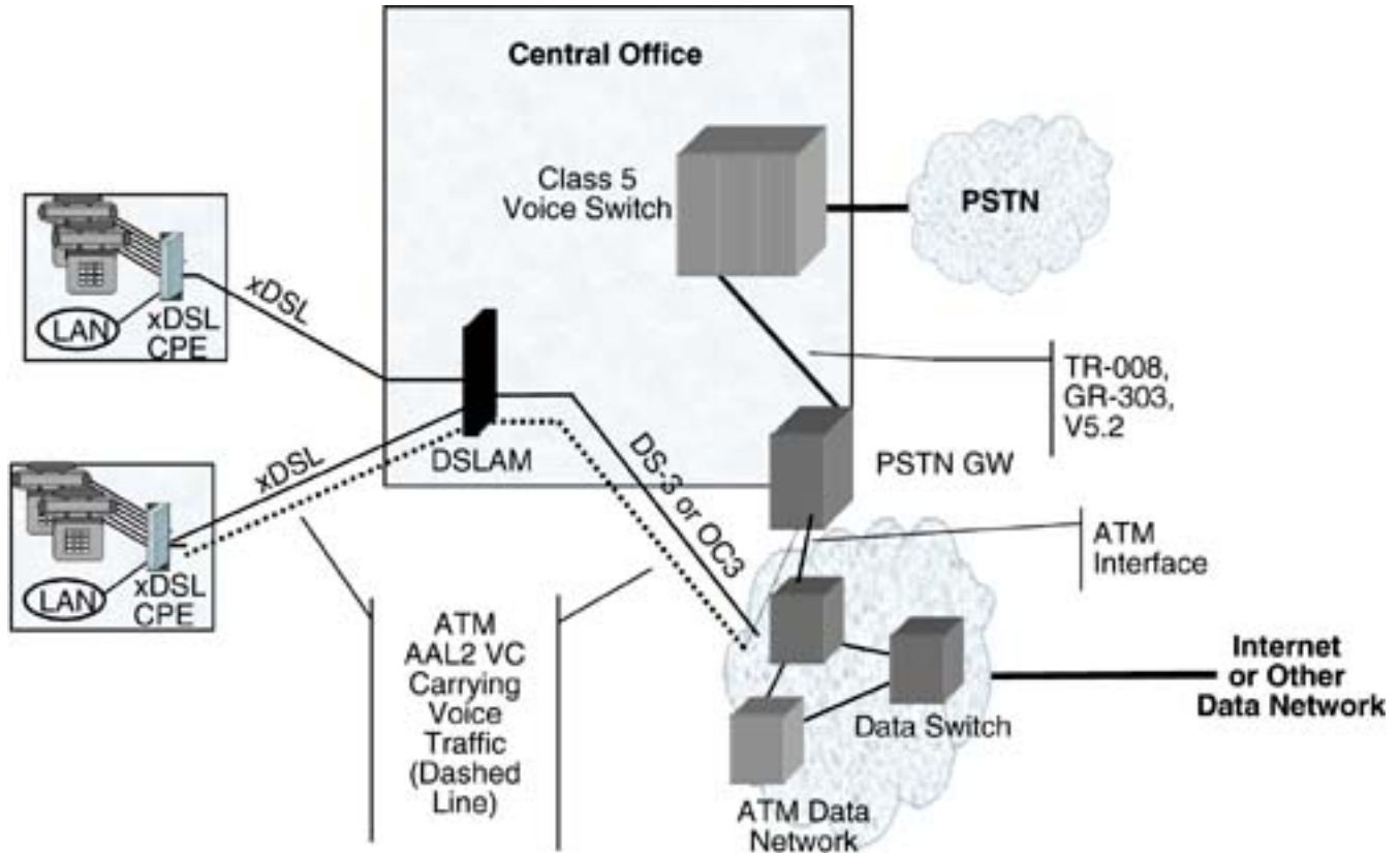
Figure 16.11. Overview of a VoATM architecture for DSL.
