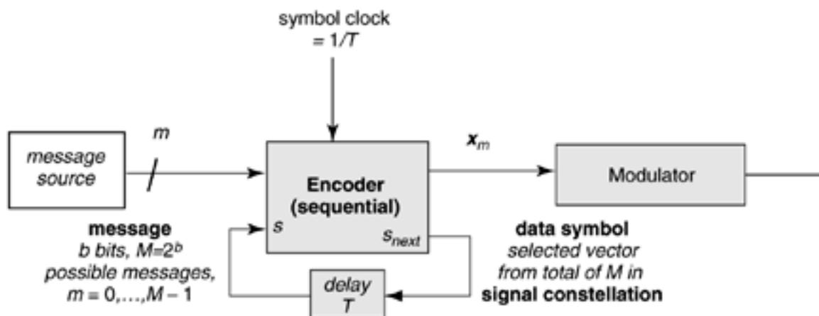
Figure 2.1. Transmitter of a digital transmission system.
