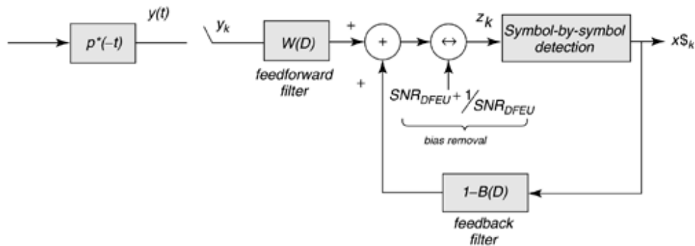
Figure 2.13. Decision-feedback equalization.
