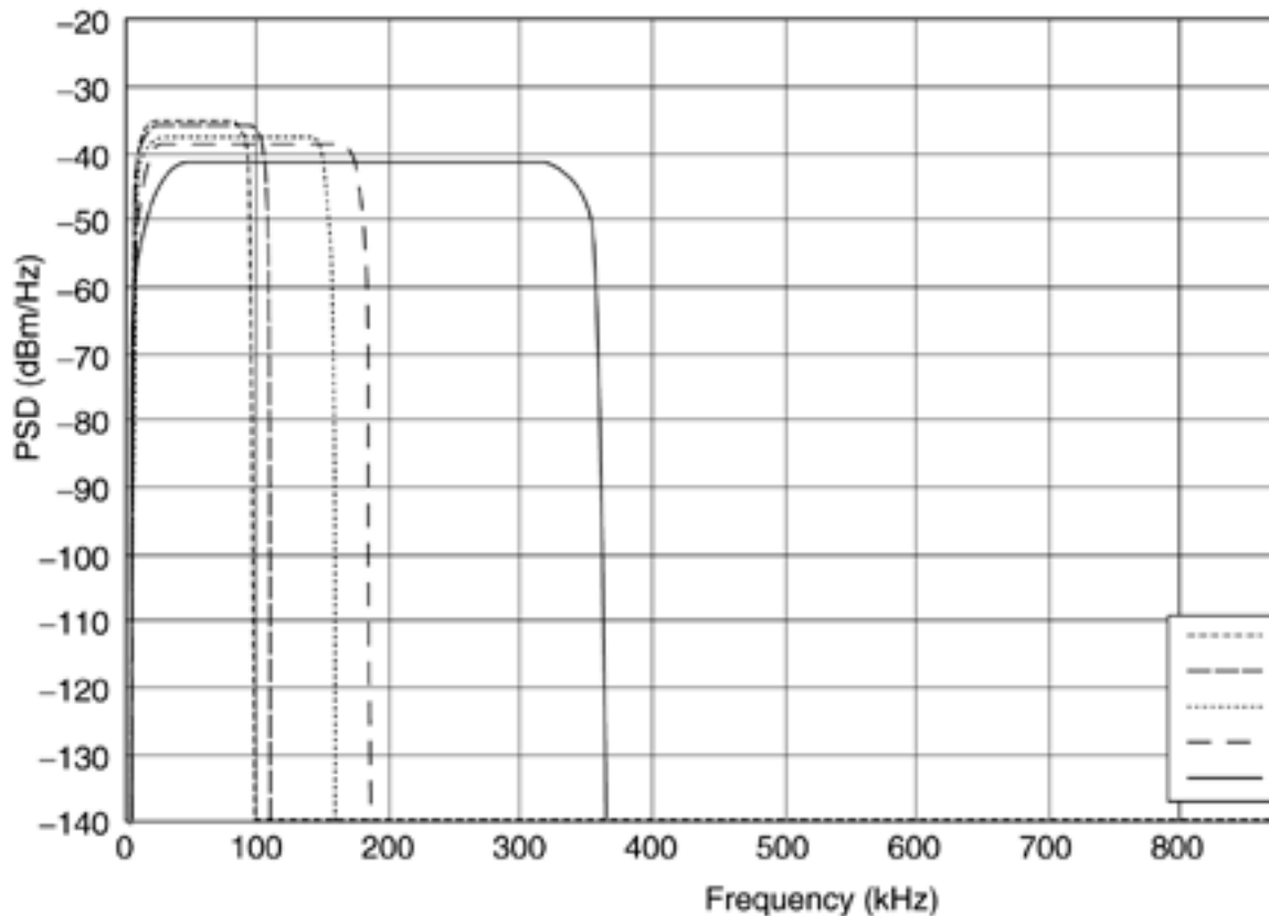
Figure 9.7. MSDSL transmit signal spectra.
