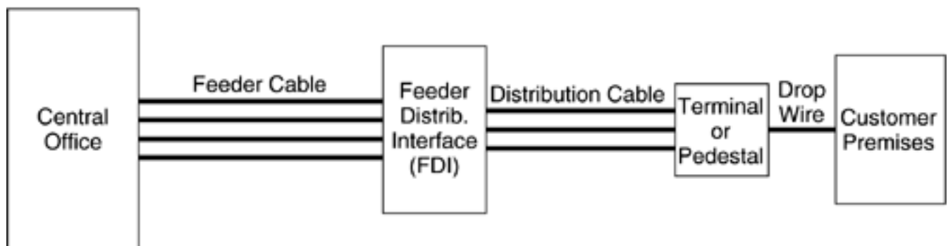
Figure 9.1. Architecture of the loop plant.
