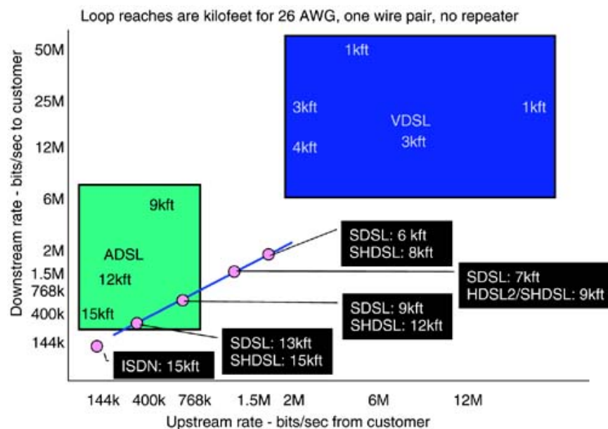
Figure 1.5. DSL Data Rates
