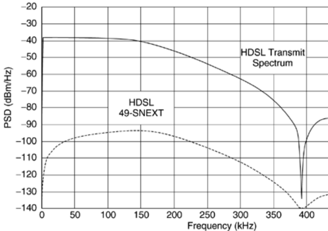
Figure 9.6. HDSL transmit signal and 49-NEXT spectra.
