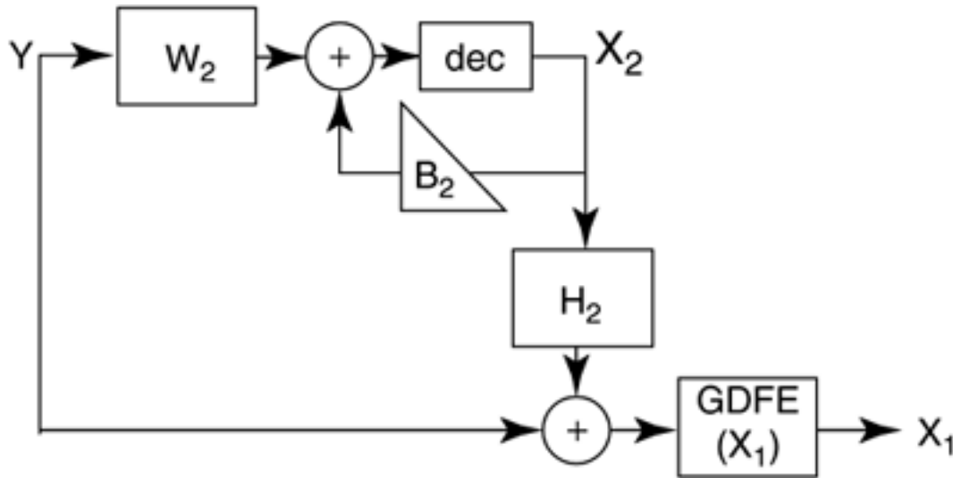
Figure 11.48. Simplified canceler configuration.
