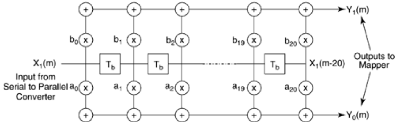
Figure 4.20. Convolutional encoder structure.
