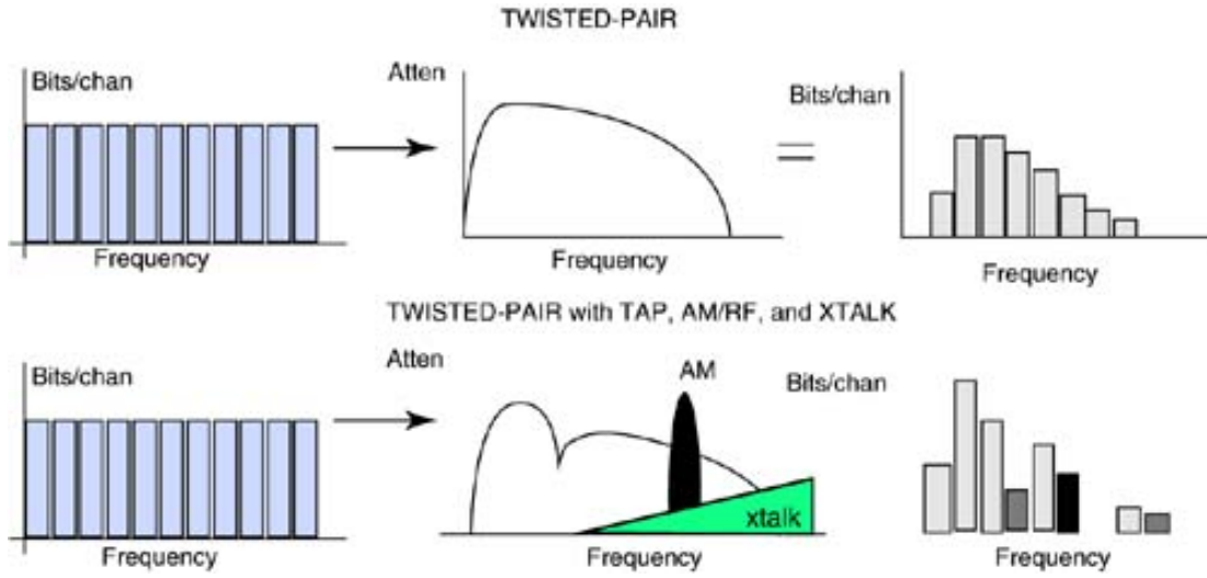
Figure 2.14. Basic multitone concept.
