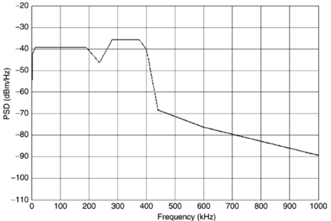
Figure 10.7. Spectrum Management Class 4 downstream template plot.
