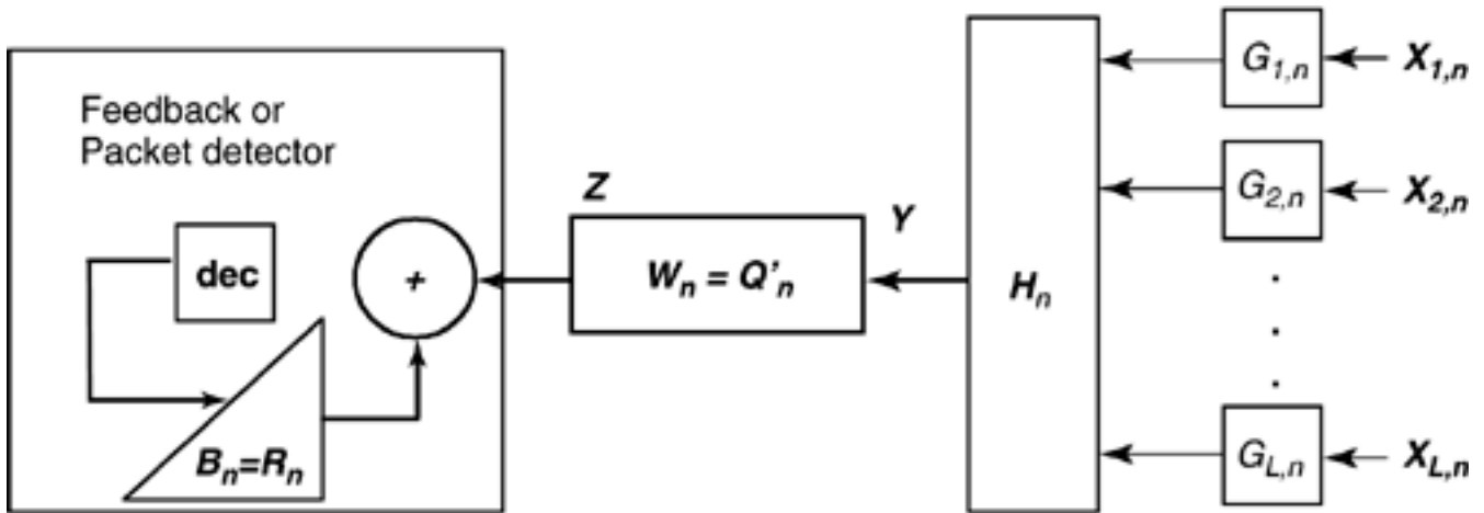
Figure 11.34. Exact illustration for one tone (n) of GDFE upstream vector receiver.
