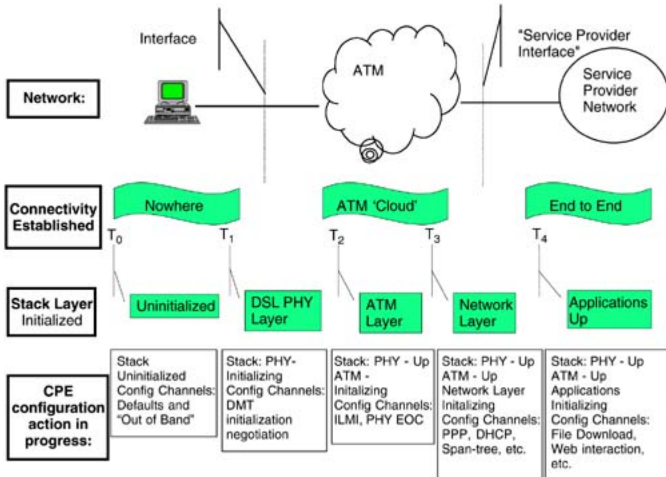
Figure 13.2. Progressive initialization of DSL CPE.
