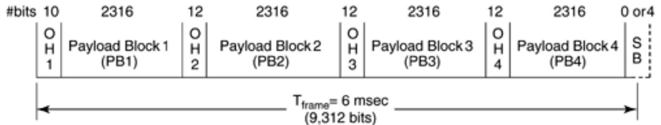
Figure 4.16. HDSL2 core frame structure.
