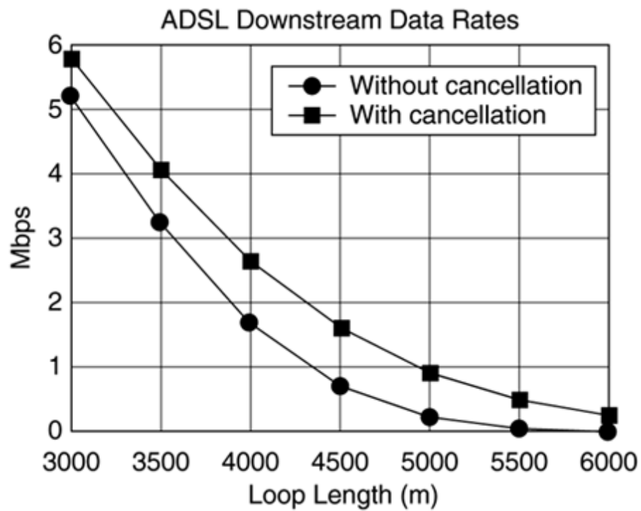
Figure 11.50. Illustration of rate/range improvement for situation illustrated in Figure 11.24.
