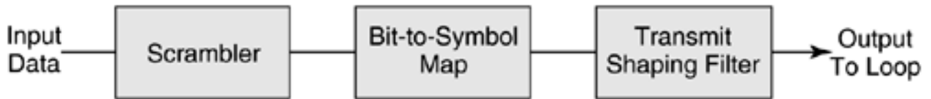
Figure 4.25. HDSL2 reference transmitter during startup.
