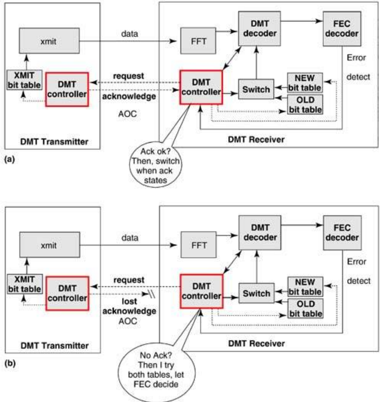
Figure 3.12. Illustration of functional and dysfunctional AOC. (a) Bit swap with AOC functioning properly. Receiver DMT controller switches to new bit table at time specified by AOC acknowledgment. (b) Bit swap with lost AOC acknowledgment. Receiver DMT controller tries both switch settings using the FEC decoder correct/errors detect to arbitrate.
