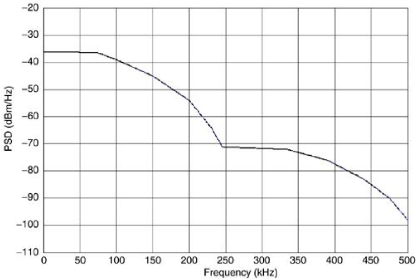
Figure 10.5. Spectrum Management Class 2 template plots.
