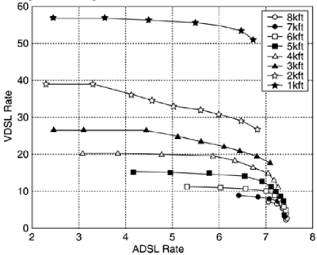
Figure 11.28(b). VDSL/ADSL with varying ADSL line length.
