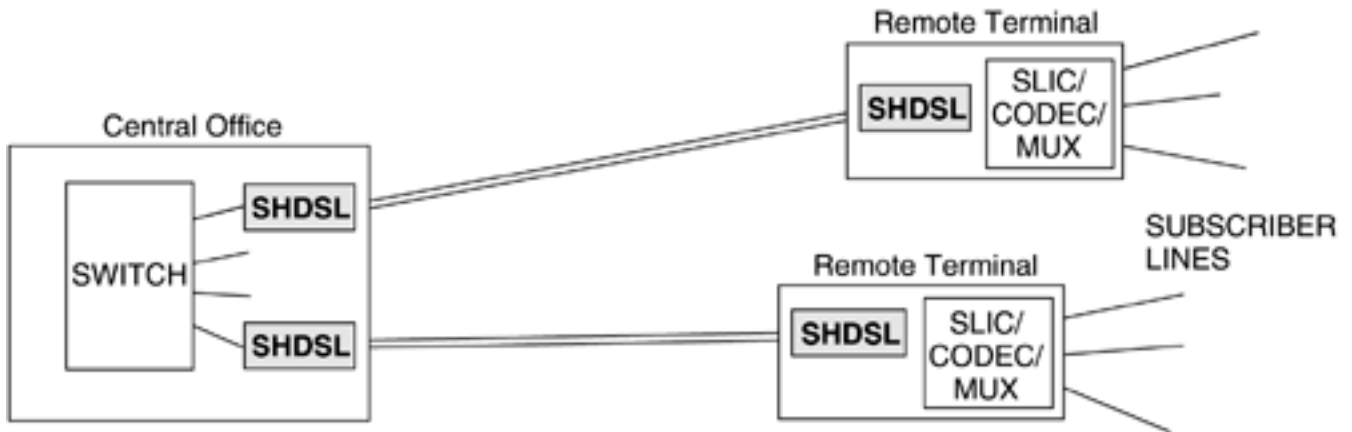
Figure 6.4. Provisioning of voice service using pair gain configuration.
