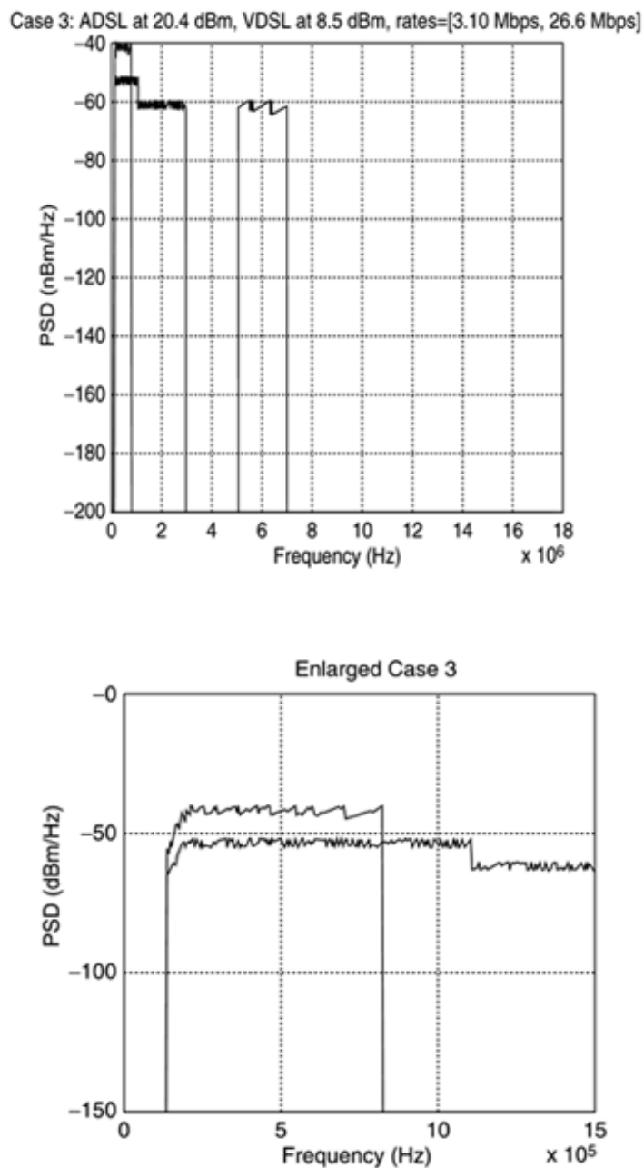
Figure 11.26. ADSL and VDSL spectra with full ADSL power, but low VDSL power (7.19, 16.2) Mbps.
