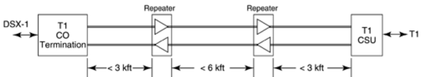
Figure 4.1. Conventional repeatered T1 AMI service provisioning.
