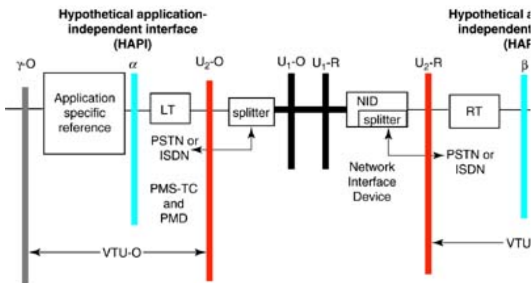
Figure 7.9. VDSL reference model from [15].
