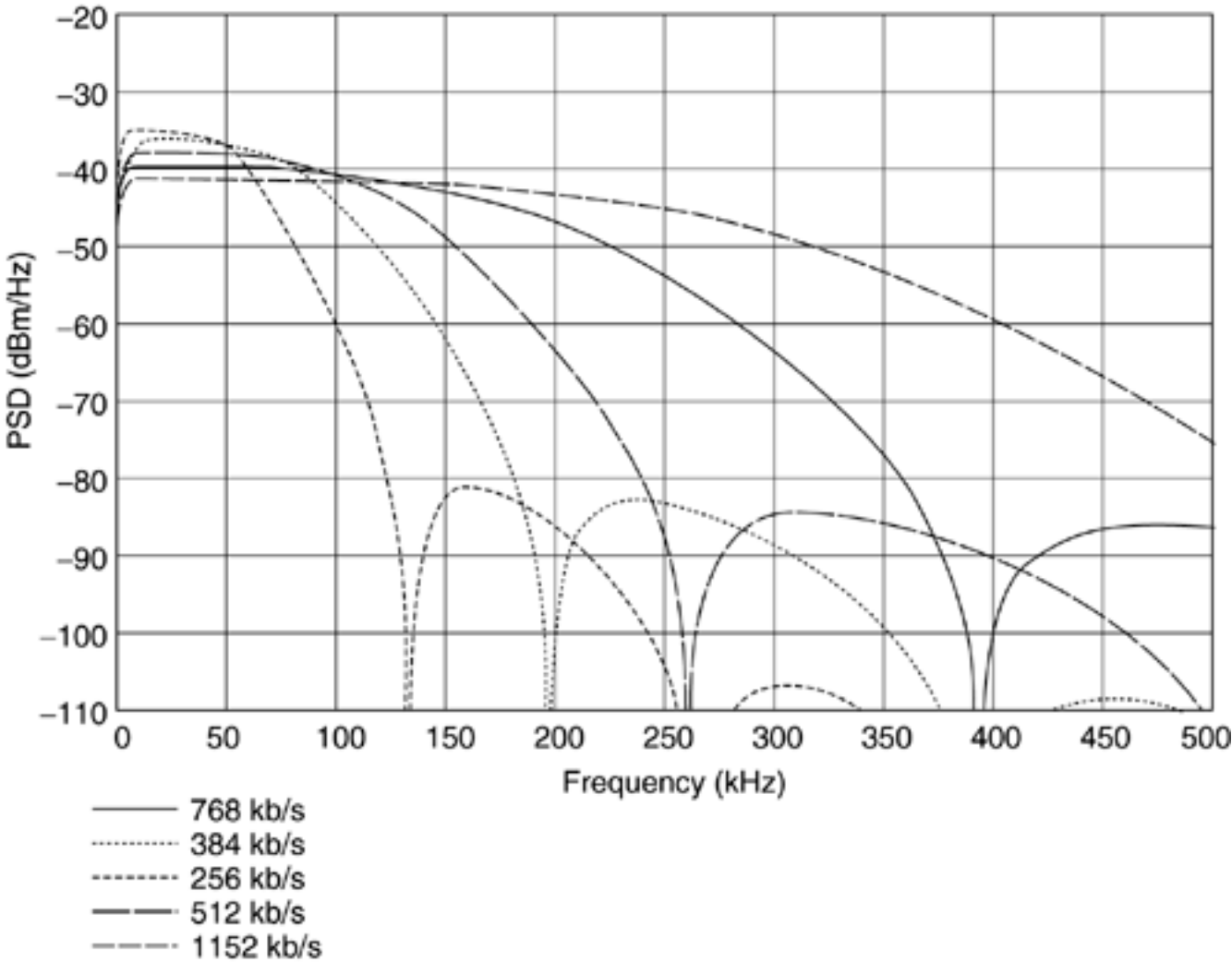
Figure 6.16. Nominal 2B1Q SDSL PSDs without noise floor.
