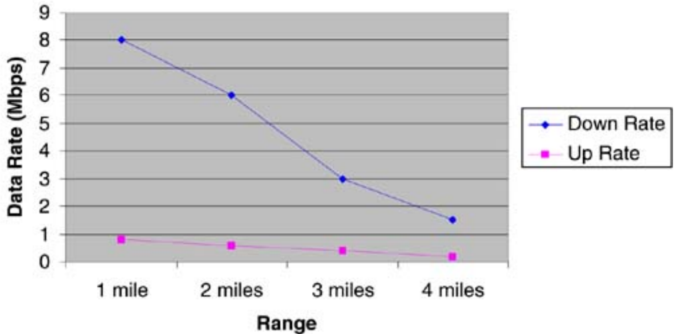
Figure 3.1. ADSL data rates.
