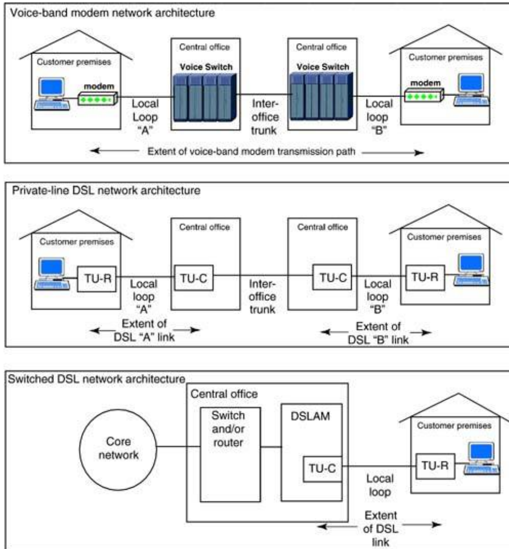
Figure 1.3. Comparative Network Architectures
