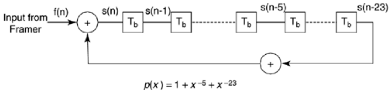
(a) Downstream channel scrambler
