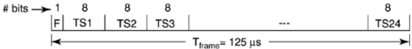
Figure 4.4. DS1 frame structure.
