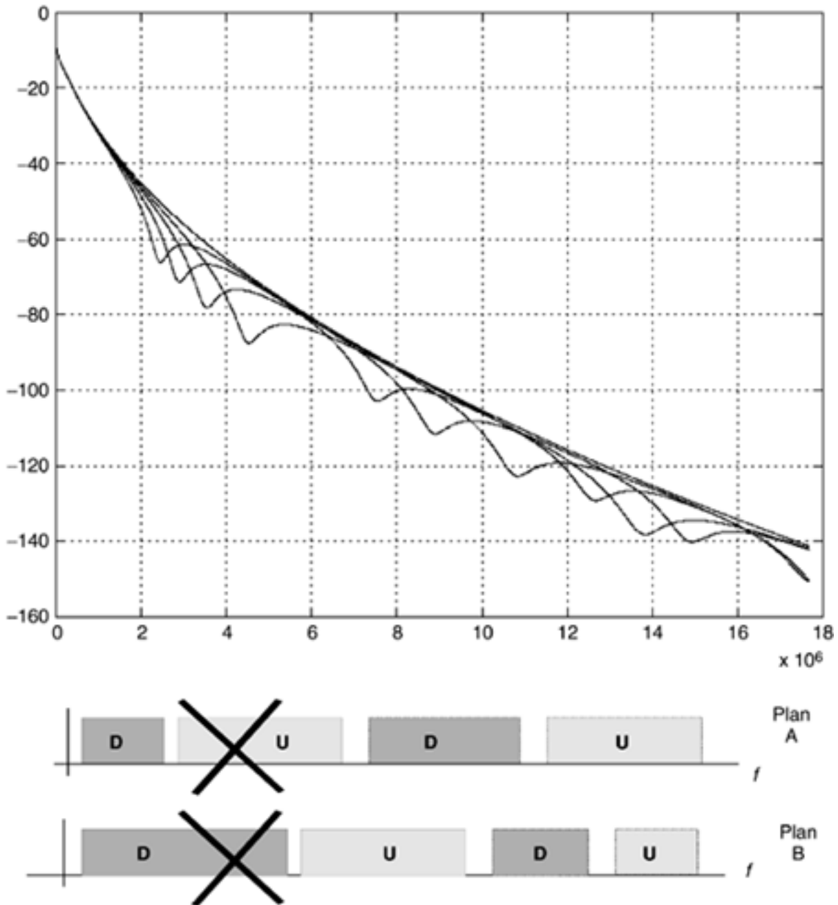
Figure 7.5. Illustration of robustness with bridged taps. The graph shows the insertion loss (in dB) of a 4050' loop with bridged-taps of length 66', 56', 46', and 36' (20 m, 17 m, 14 m, and 11 m respectively). Below the graph, two different frequency plans are shown. When plan A is used, only upstream transmission is affected. When plan B is used, only downstream transmission is affected. In both cases, symmetric service is disabled.
