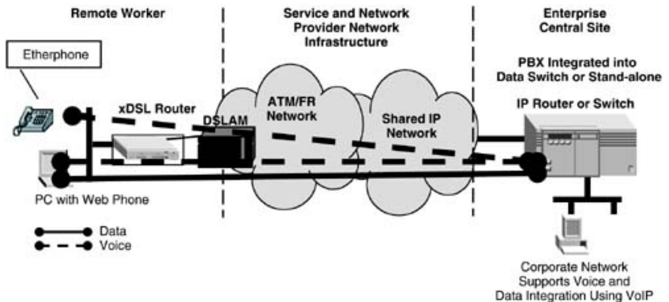
Figure 16.14. PBX extension architecture.
