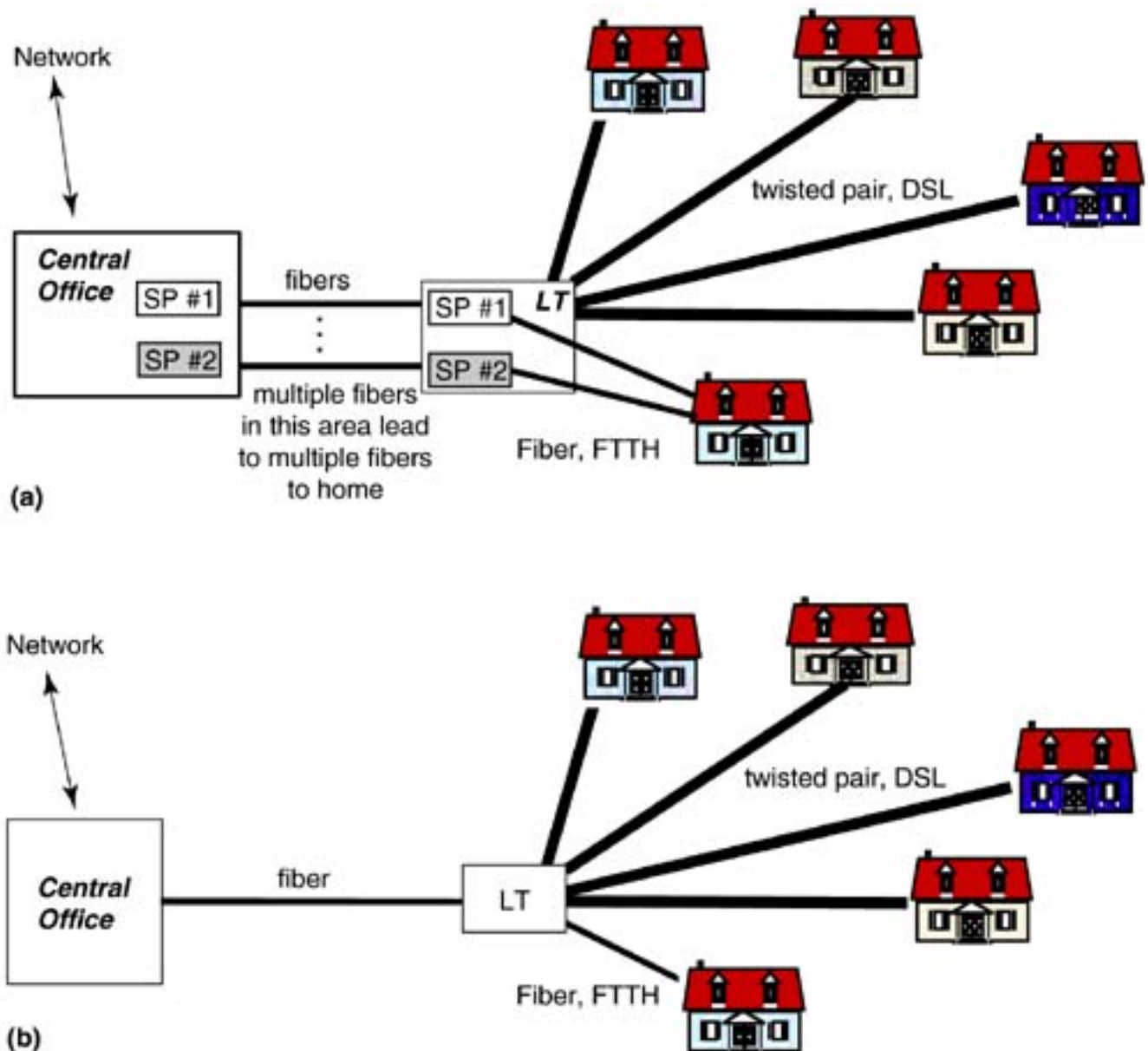
Figure 11.3. (a) Mutliple service provider, line-unbundled LT-based DSL; (b) Packet-unbundled DSL evolution.
