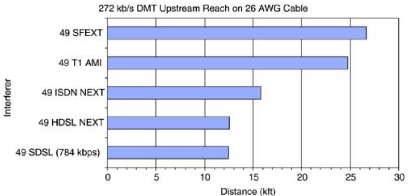
Figure 9.17. Upstream DMT spectral compatibility with other DSLs.
