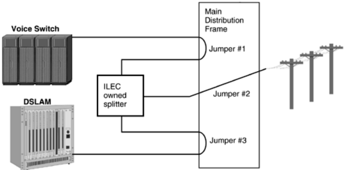
Figure 8.5. Central office configuration with ILEC-owned line sharing splitter.
