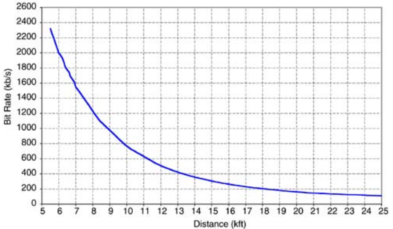
Figure 10.2. SDSL reach in the presence of 49 SNEXT.
