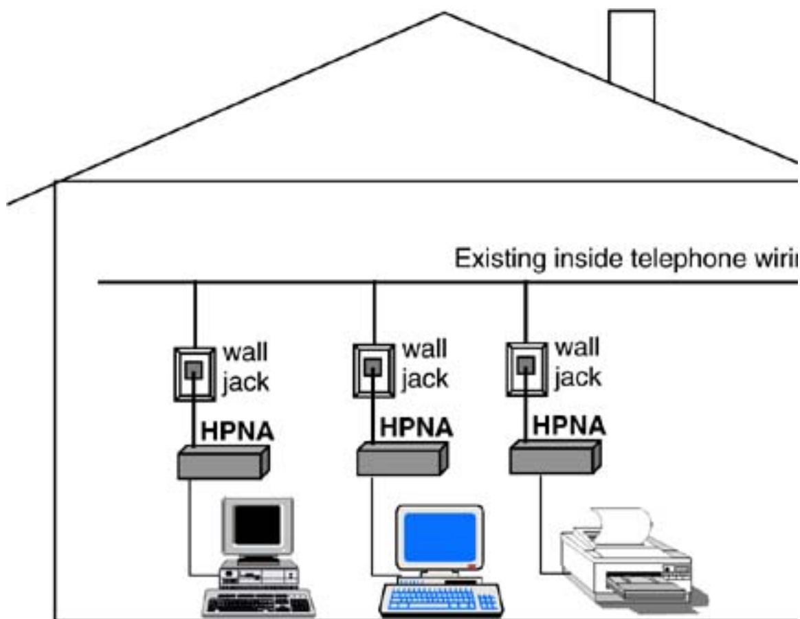
Figure 12.6. HomePNA configuration.
