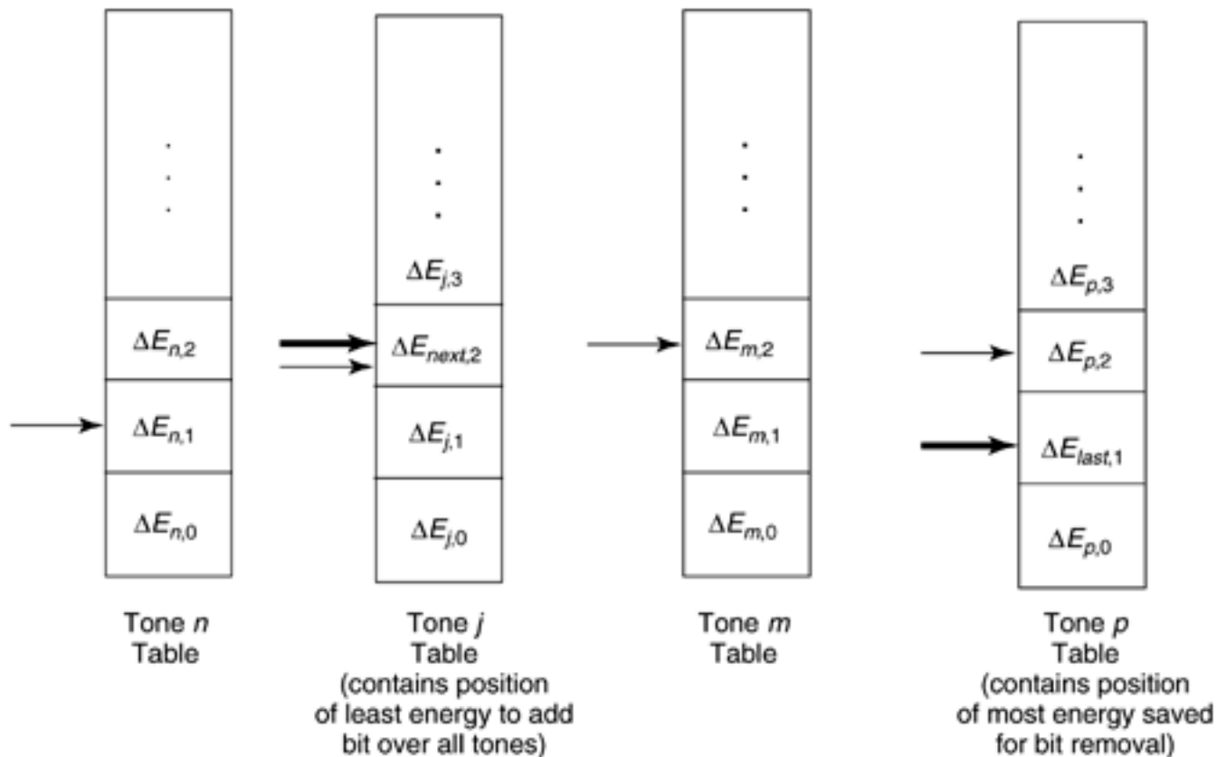
Figure 3.15. Bit-swapping table illustration. Light arrows indicate position to which energy for adding a bit to constellation on current tone is listed; heavy arrows indicate the positions of least cost and most saved energy over all tones.
