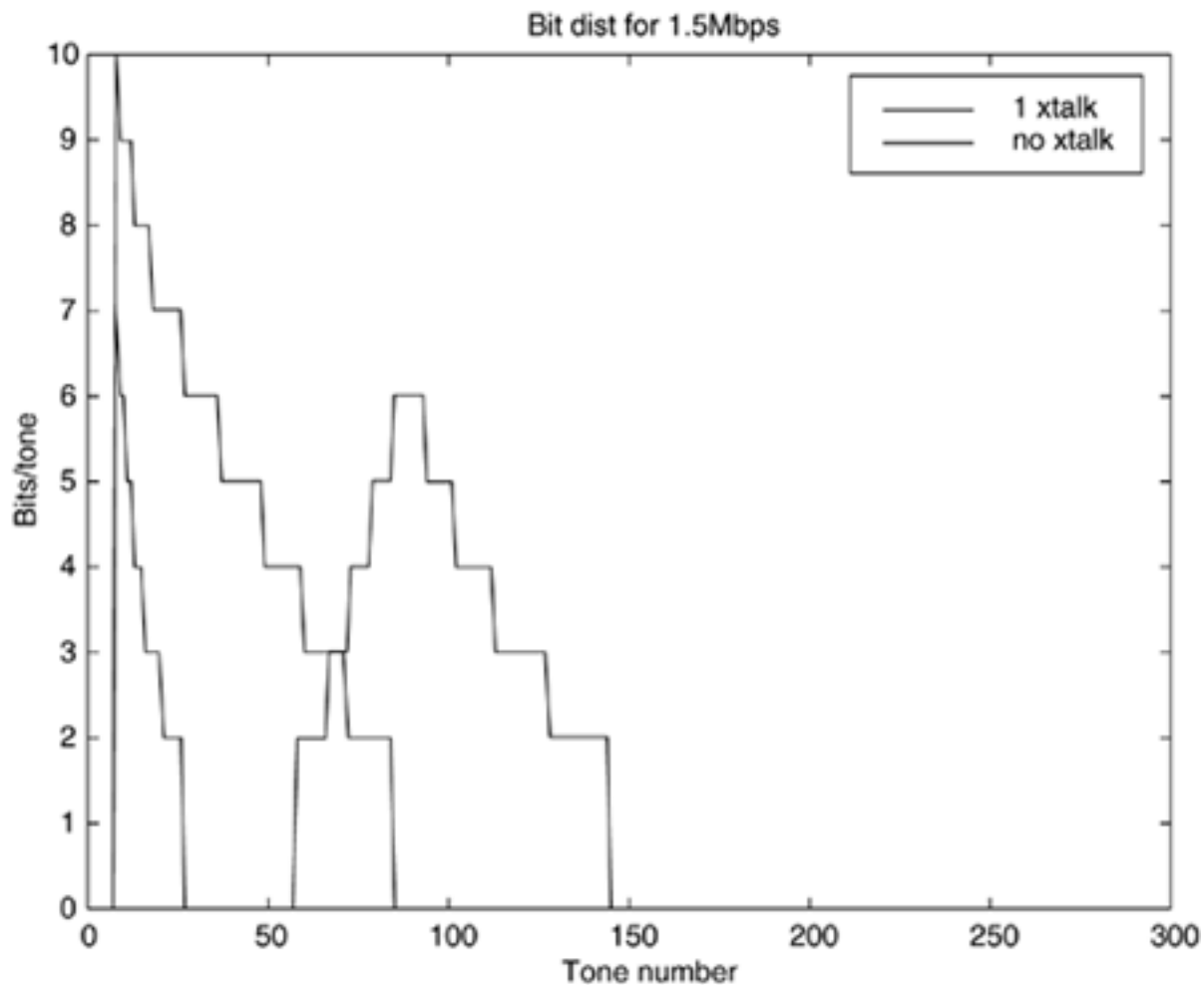
Figure 3.13. Optimized bit distributions for 0 crosstalkers and 1 crosstalker on 4.25 km 26-gauge twisted pair (xtalk is HDSL, background noise is “140 dBm/Hz).
