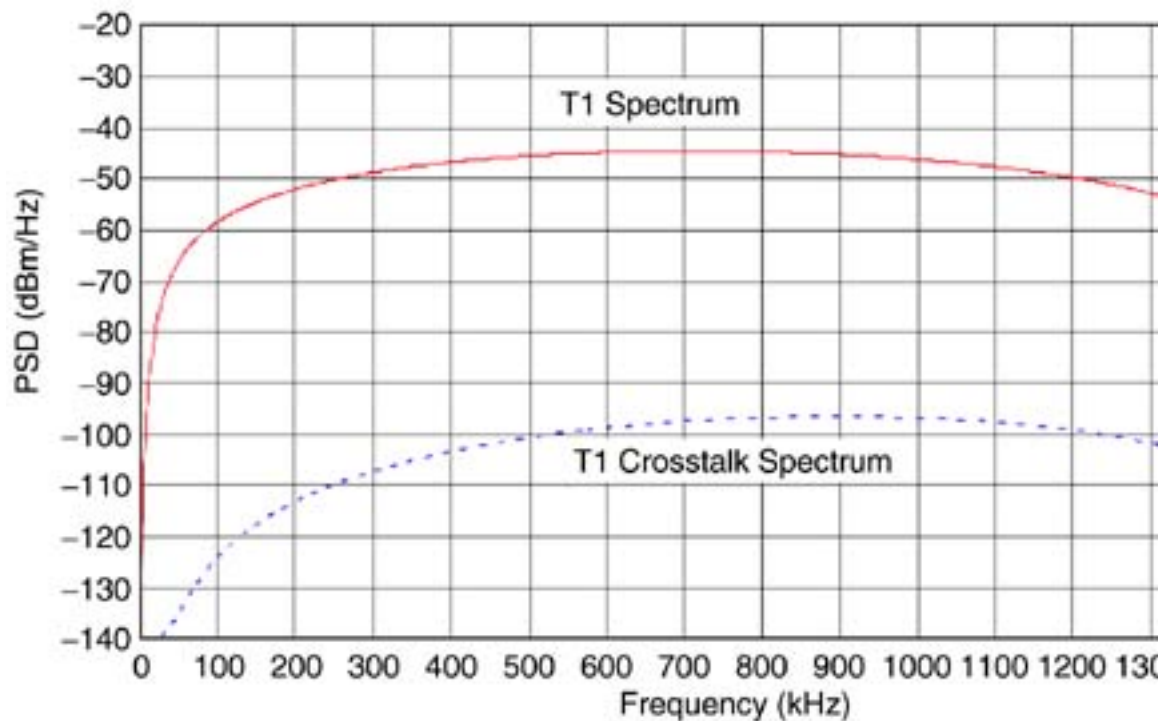
Figure 9.10. T1 AMI signal and crosstalk spectra.
