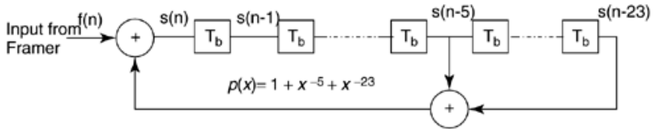
(a) Downstream Channel Scrambler
