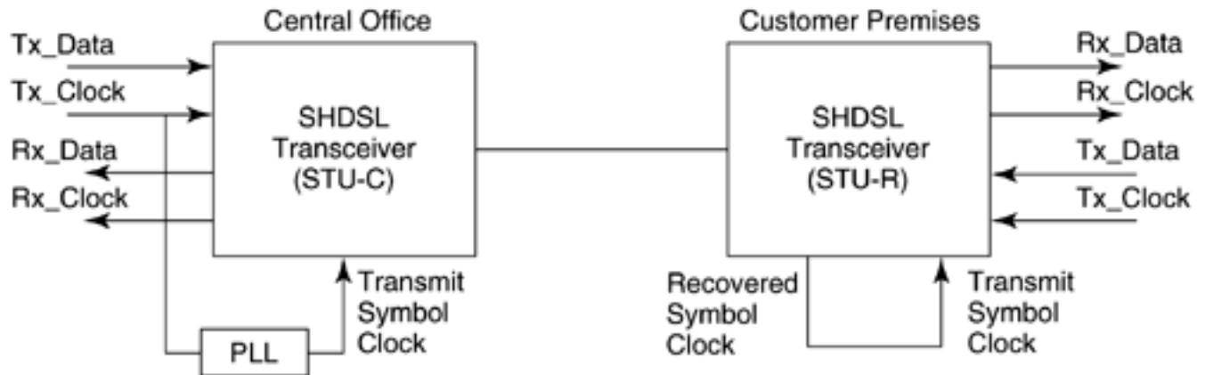
Figure 6.21. Synchronous timing mode.
