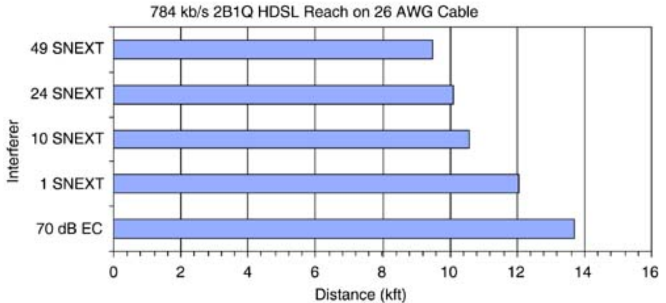
Figure 9.14. HDSL reach as a function of SNEXT.
