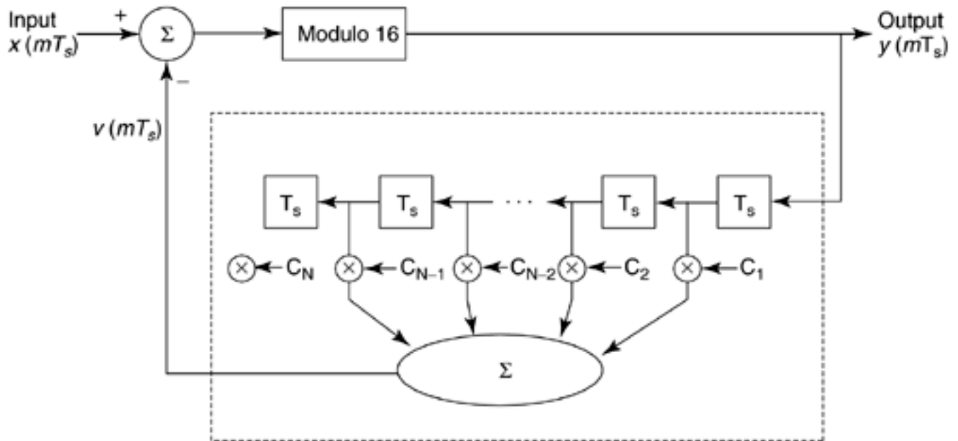
Figure 4.22. HDSL2 channel precoder.
