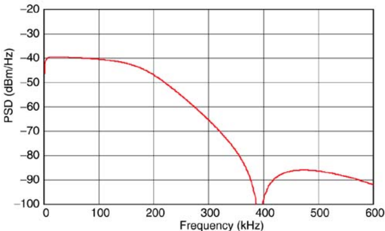
Figure 4.9. Nominal 2B1Q HDSL transmit PSD (784 kb/s) with 4th-order roll-off.
