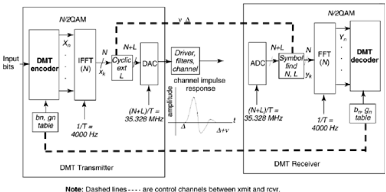
Figure 7.13. Basic DMT transmission system.
