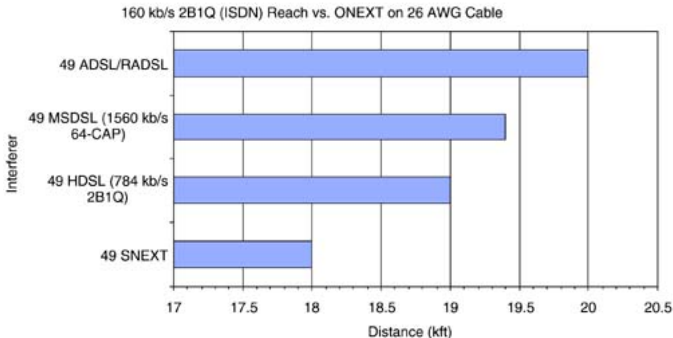
Figure 9.13. ISDN Reach as a function of other NEXT disturbers.
