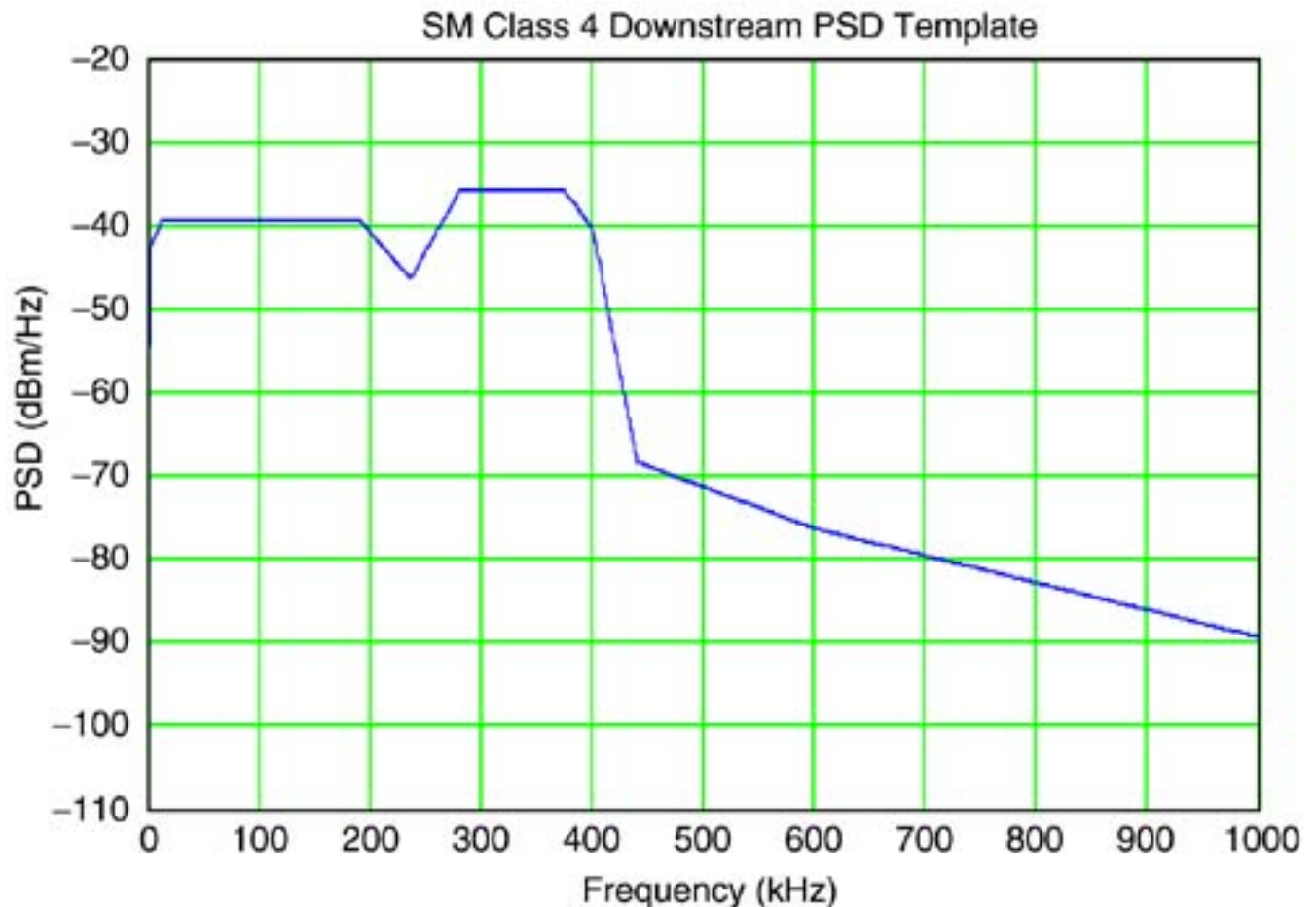
Figure 4.23. Downstream channel spectrum.
