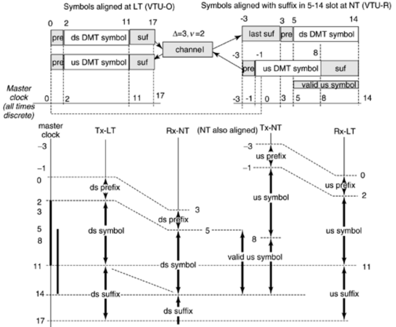
Figure 7.15. DMT symbol alignment at both LT and NT through use of suffix.
