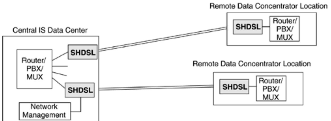
Figure 6.3. Campus private network application.
