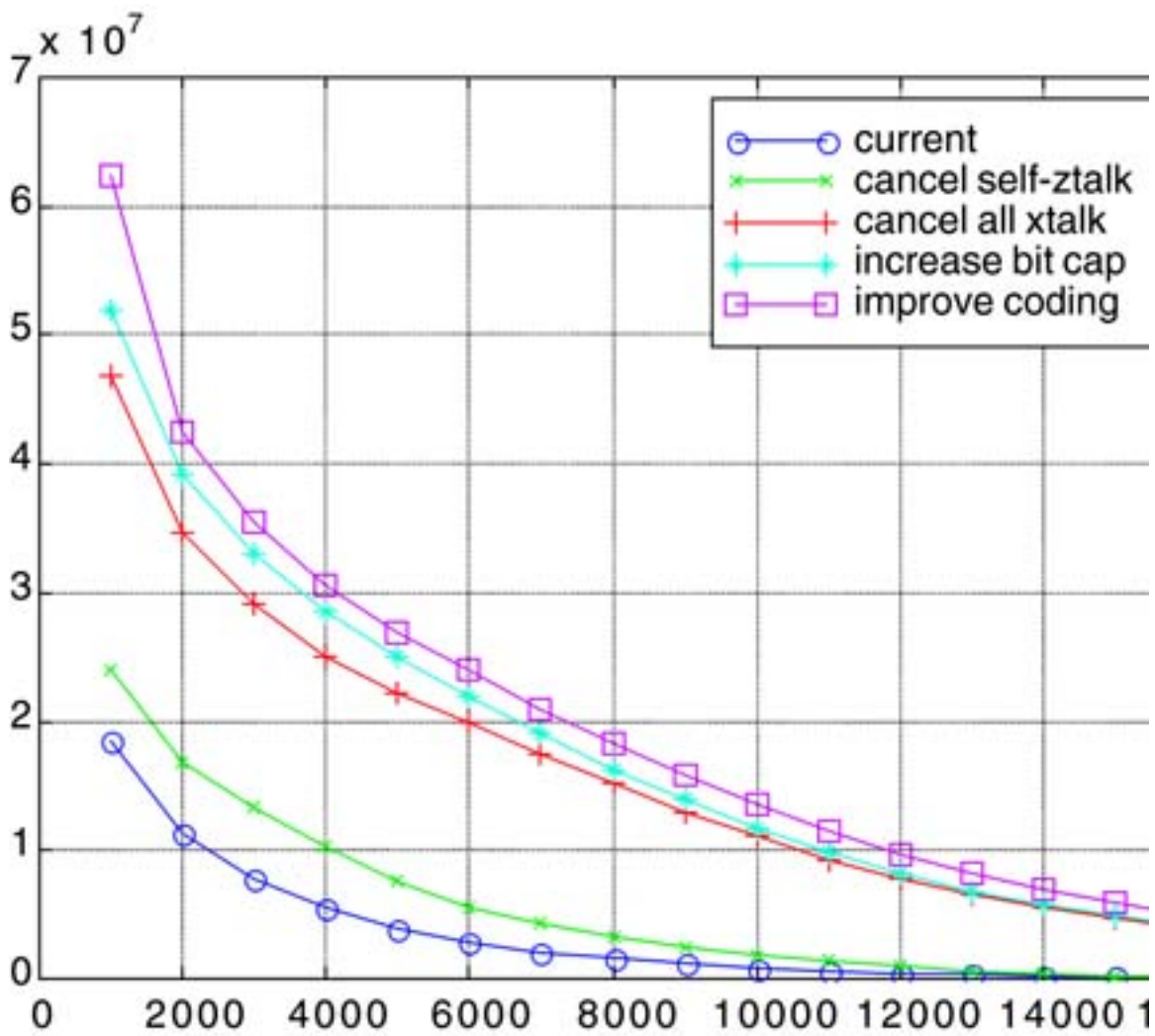
Figure 11.31 illustrates the trade-off versus line length as the loop length of VDSL instead varies with respect to the best-known (and not used because it cannot be implemented in the static-spectra-only QAM VDSL) reference-noise, spectrally shaped, power back-off methods of VDSL and the corresponding ADSL data rates.
