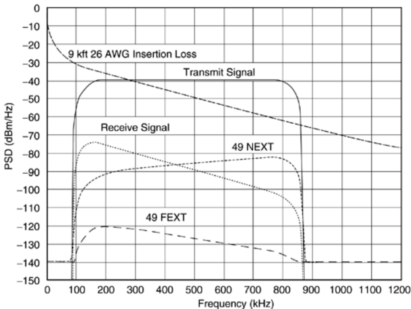
Figure 9.4. Comparison of NEXT and FEXT crosstalk levels.
