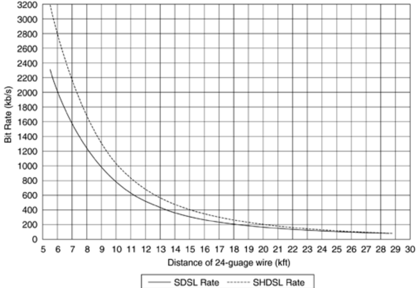
Figure 6.18. SHDSL and 2B1Q SDSL bit rates versus 24-gauge distance in presence of 49 SNEXT.
