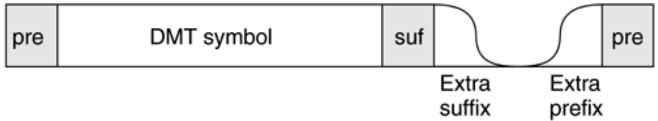
Figure 7.18. Illustration of windowing in extra suffix/prefix samplesmooth connection of blocks without affecting necessary properties for digital duplexing.
