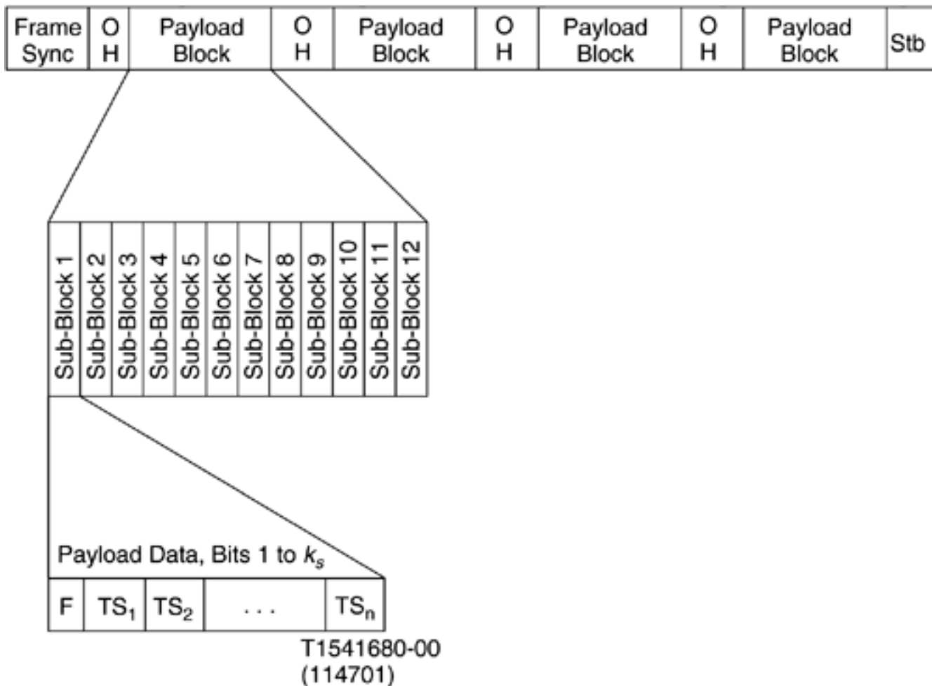
Figure 6.22. Fractional T1/E1 frame structure.
