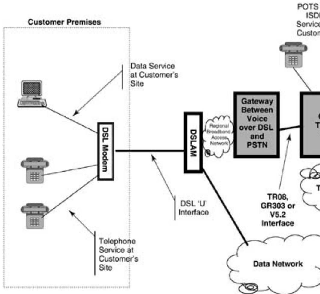
Figure 16.5. Use of TR-08, GR 303, and V5.2 to support VoDSL gateways.
