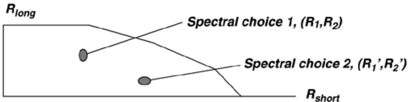
Figure 11.7. Illustration of rate regions for two DSL lines.
