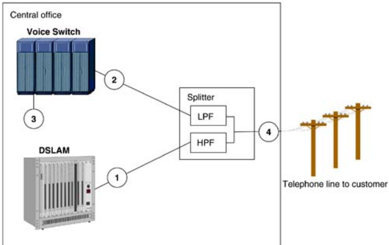
Figure 8.6. Potential locations for line testing systems.
