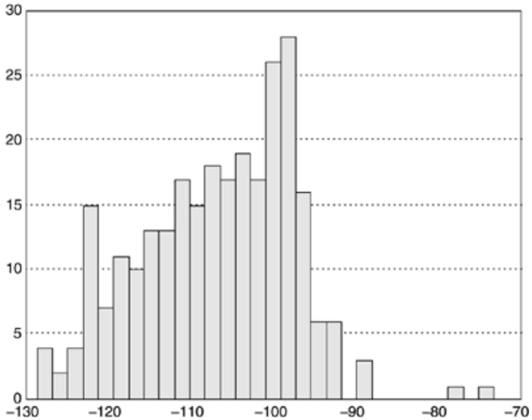
Figure 3.5. Impulse energy histogram (horizontal axis is dB in Watts/Hz). Courtesy France Telecom [6].
