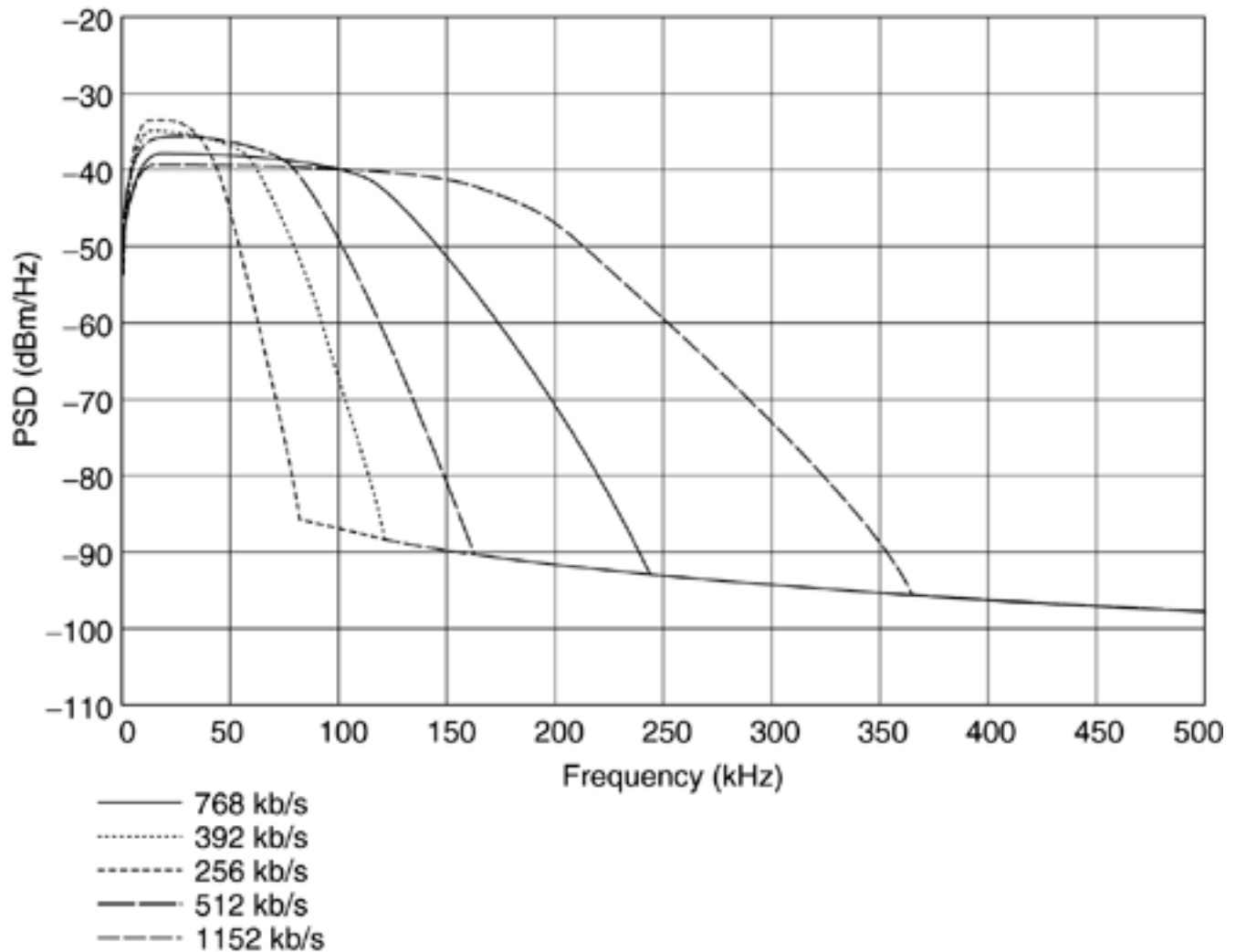
Figure 6.17. Nominal PAM PSDs with inclusion of out of band noise floor.
