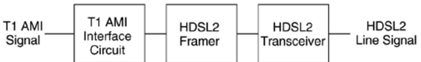
Figure 4.15. System reference model for and HDSL2 transceiver unit.
