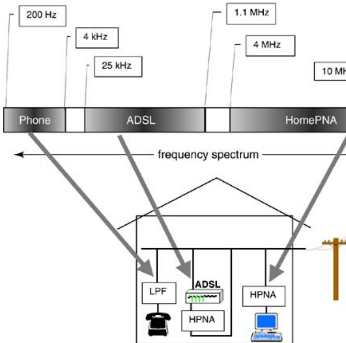
Figure 12.7. Frequency bands for phone, ADSL, and HomePNA.
