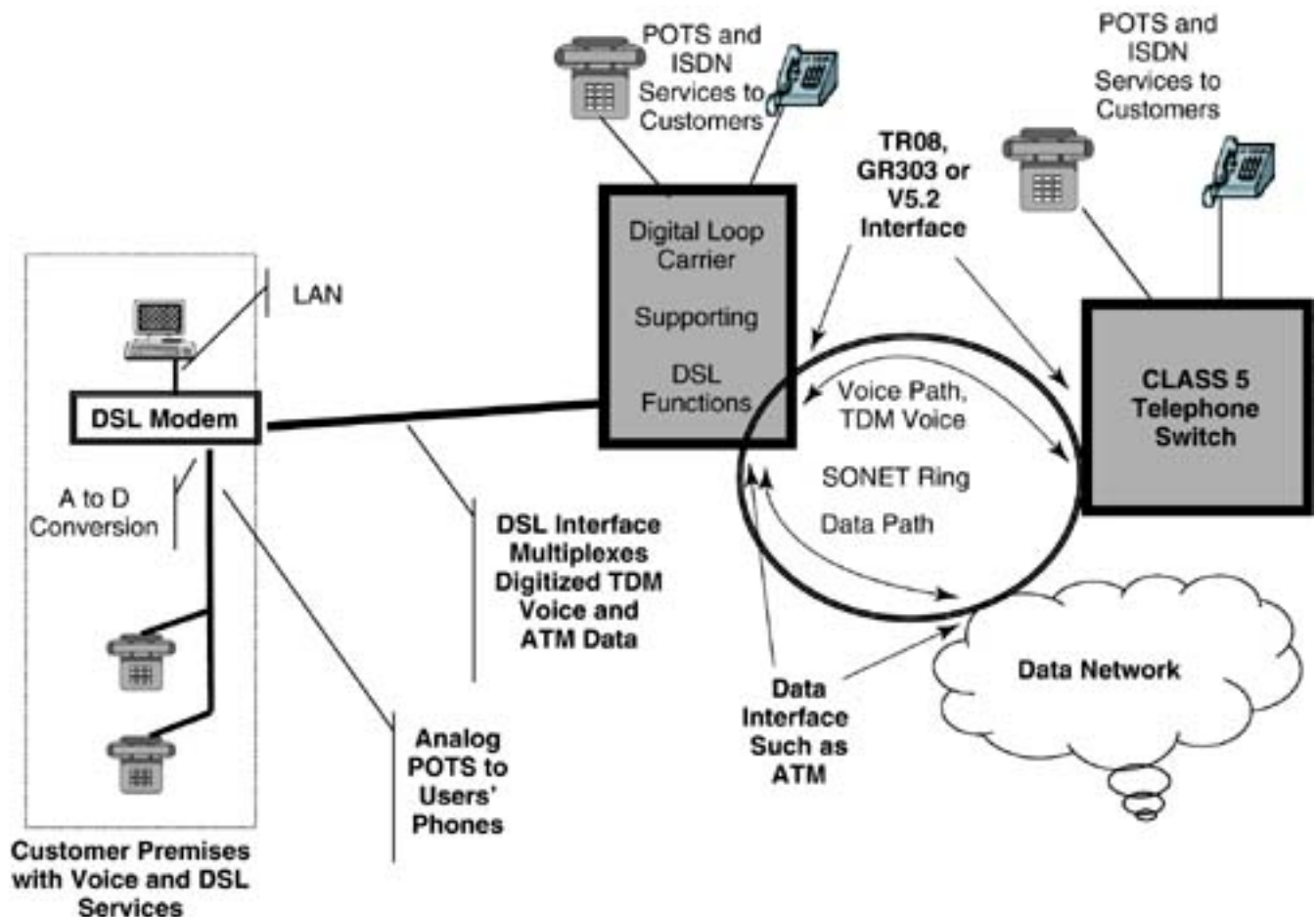
Figure 16.13. CVoDSL architecture.
