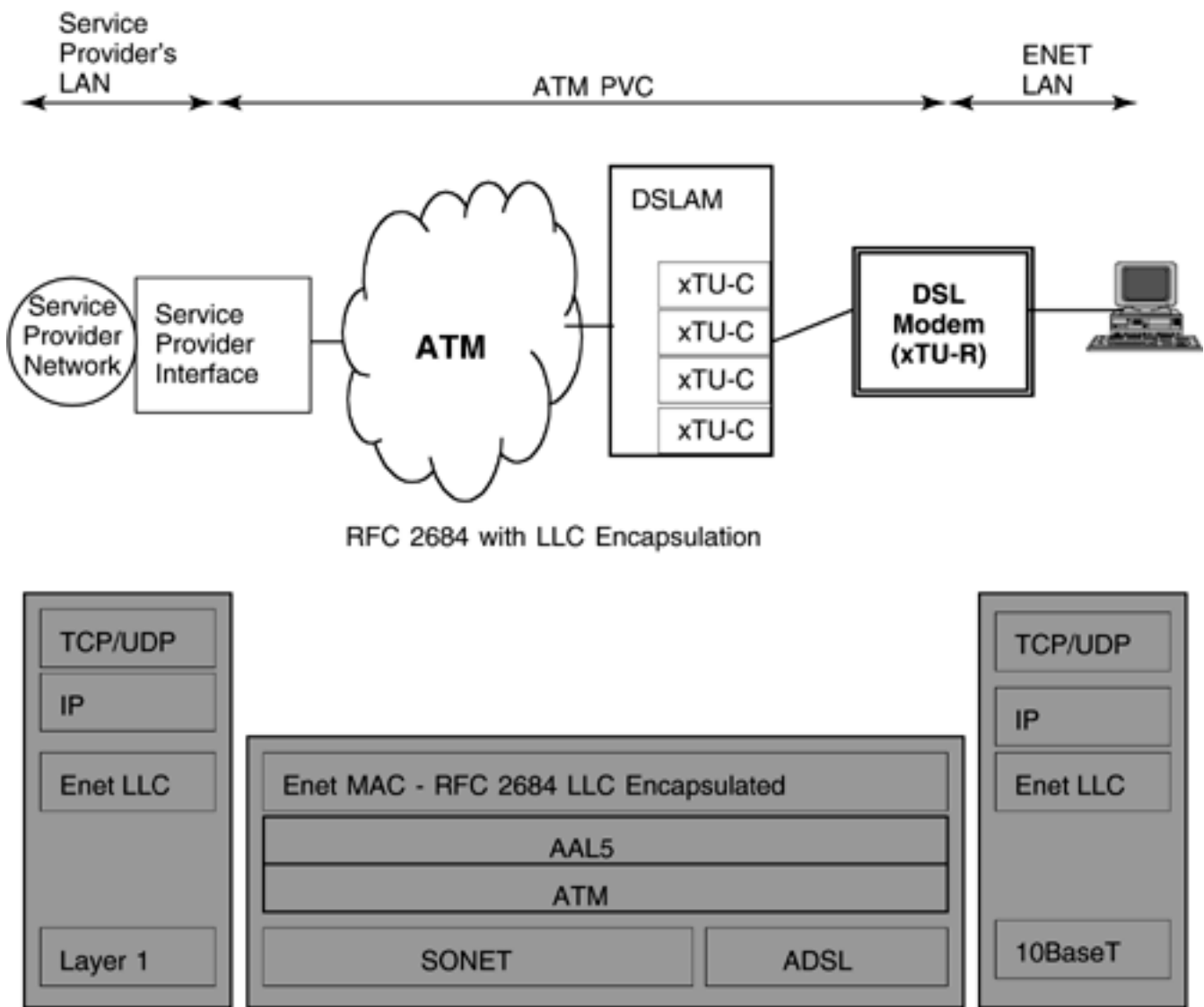
Figure 14.4. IP directly on AAL5.
