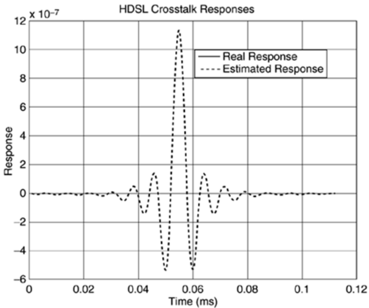
Figure 11.42. Cross-correlation for identification of offset between one of the HDSLs and the ADSL.
