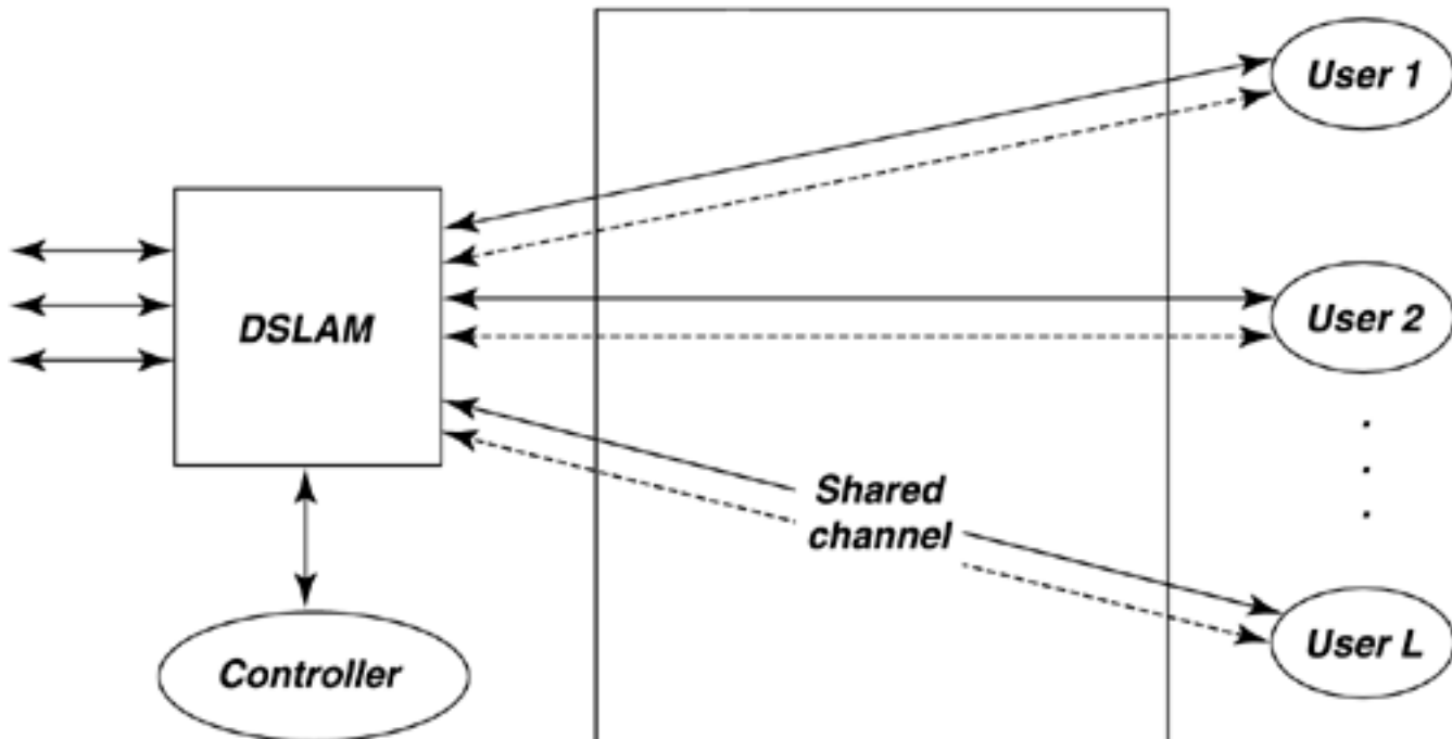
Figure 11.11. Level 2 two-sided coordination.
