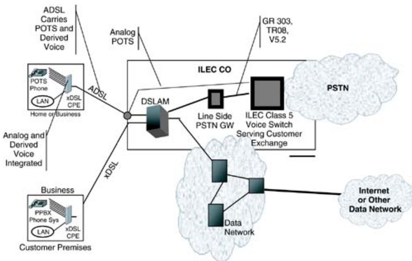
Figure 16.17. Loop extension architecture for an ILEC.
