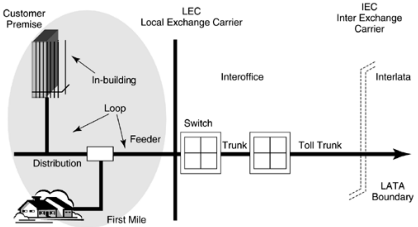
Figure 7.27. Ethernet in First Mile Illustration (shaded area is EFM interest). (Courtesy of H. Barass).
