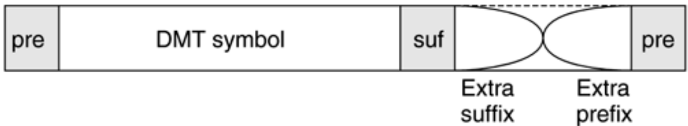
Figure 7.19. Illustration of overlapped windowing.
