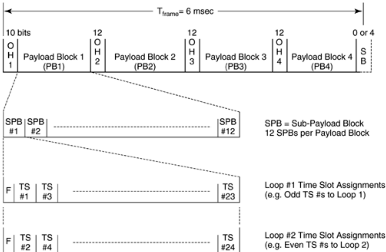
Figure 4.6. HDSL frame structure.
