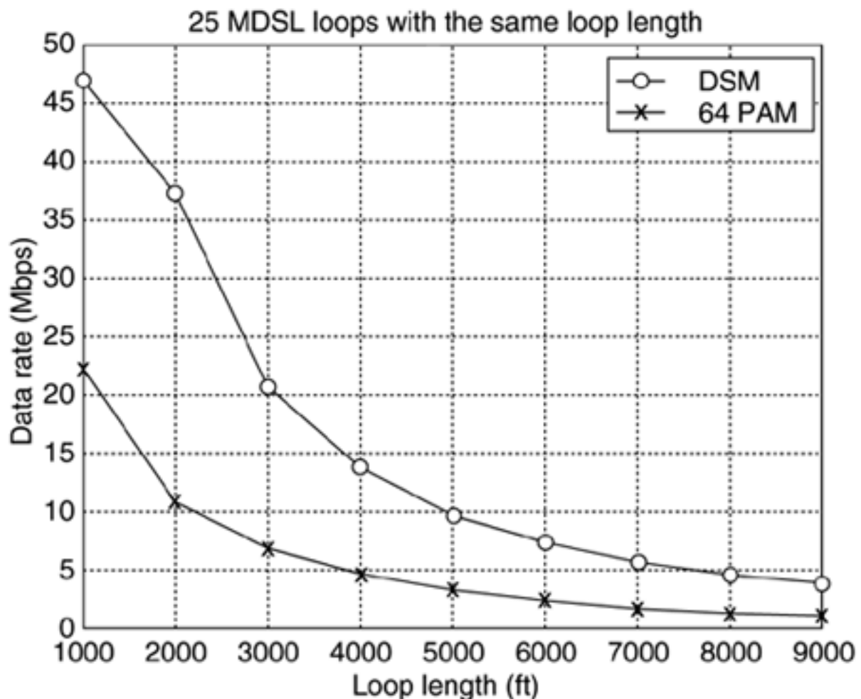
Figure 11.20. 10Mbps symmetric DSL (10MDSL) on a single-line with 25 lines all of same length. No coordination used.
