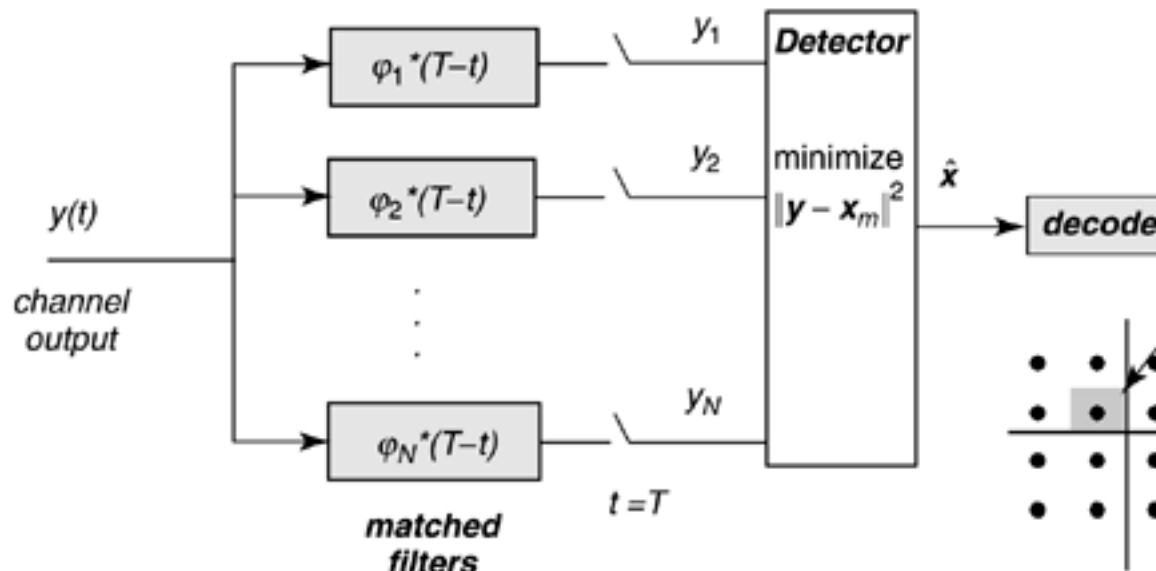
Figure 2.4. Demodulation, detection, and decoding.
