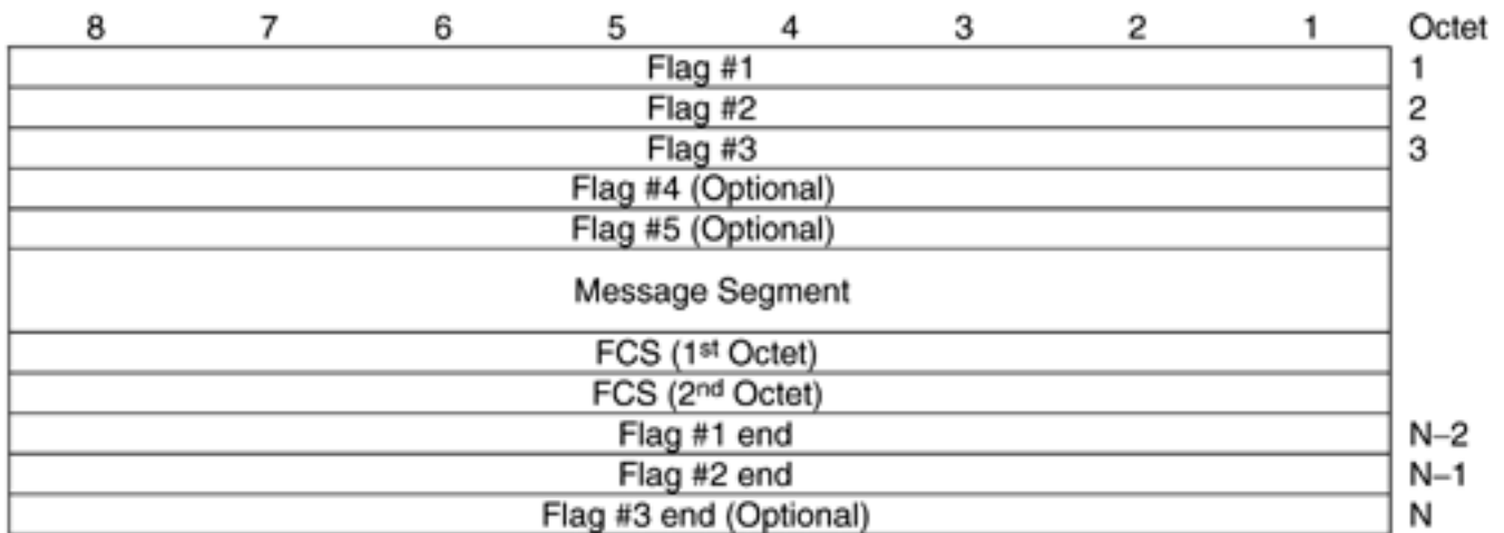
Figure 5.3. Message segment frame structure.
