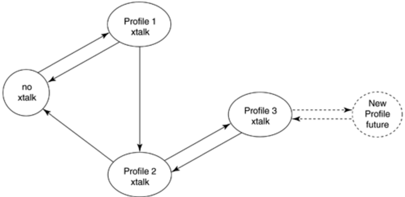
Figure 11.45. Profiling state machine.
