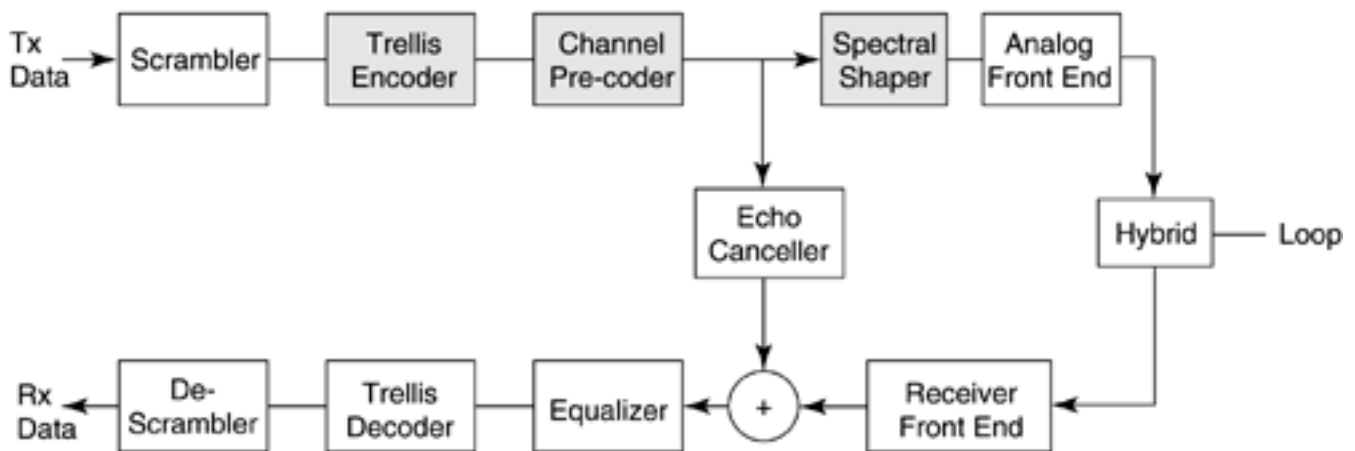
Figure 6.9. General transceiver functional block diagram for HDSL2.
