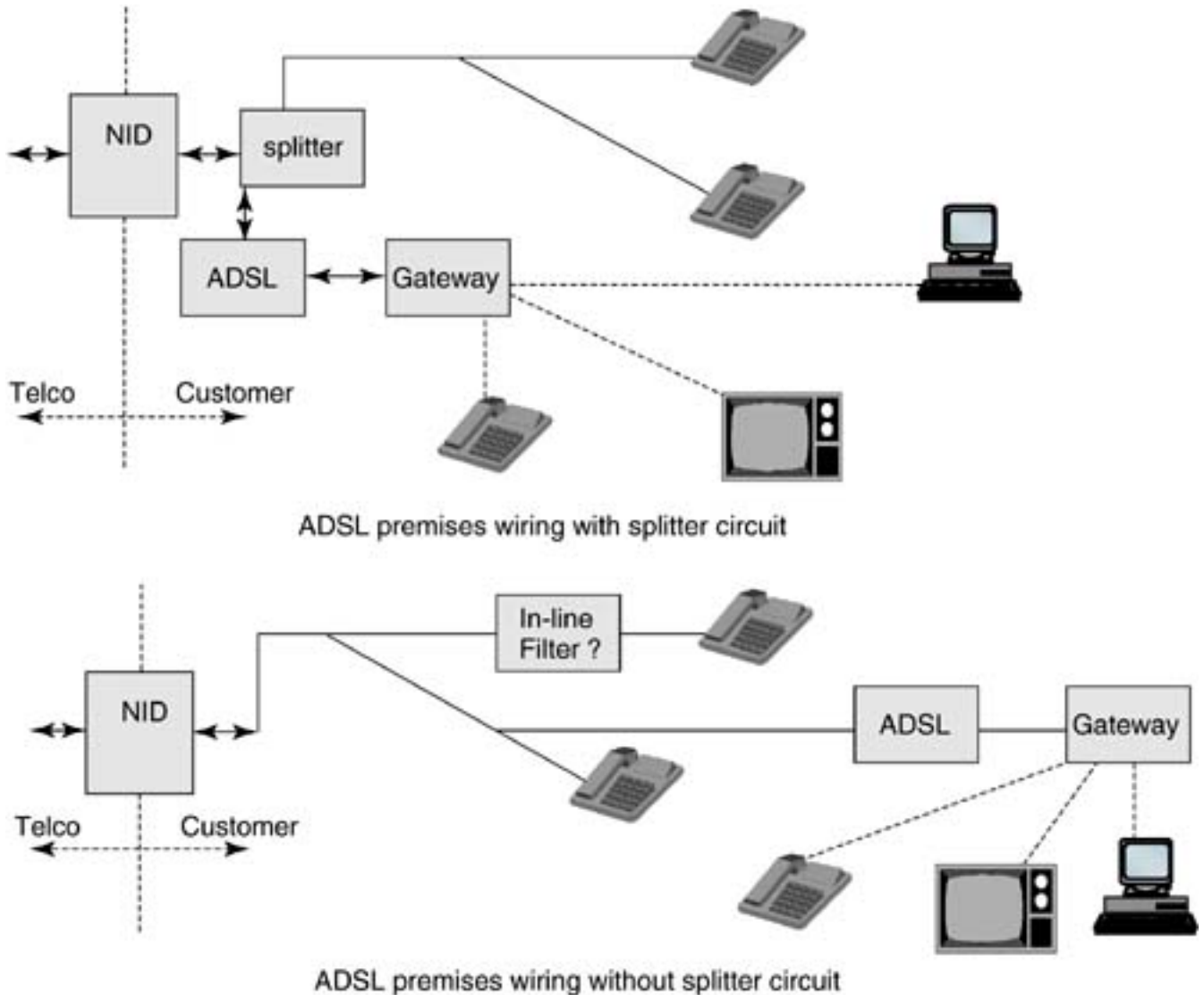
Figure 3.17. Customer premises wiring options.
