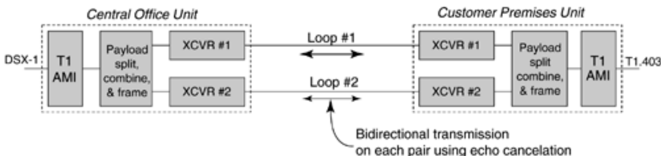
Figure 4.3. Dual-duplex architecture of HDSL.
