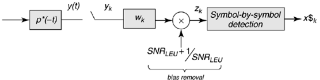
Figure 2.12. MMSE linear equalizer.
