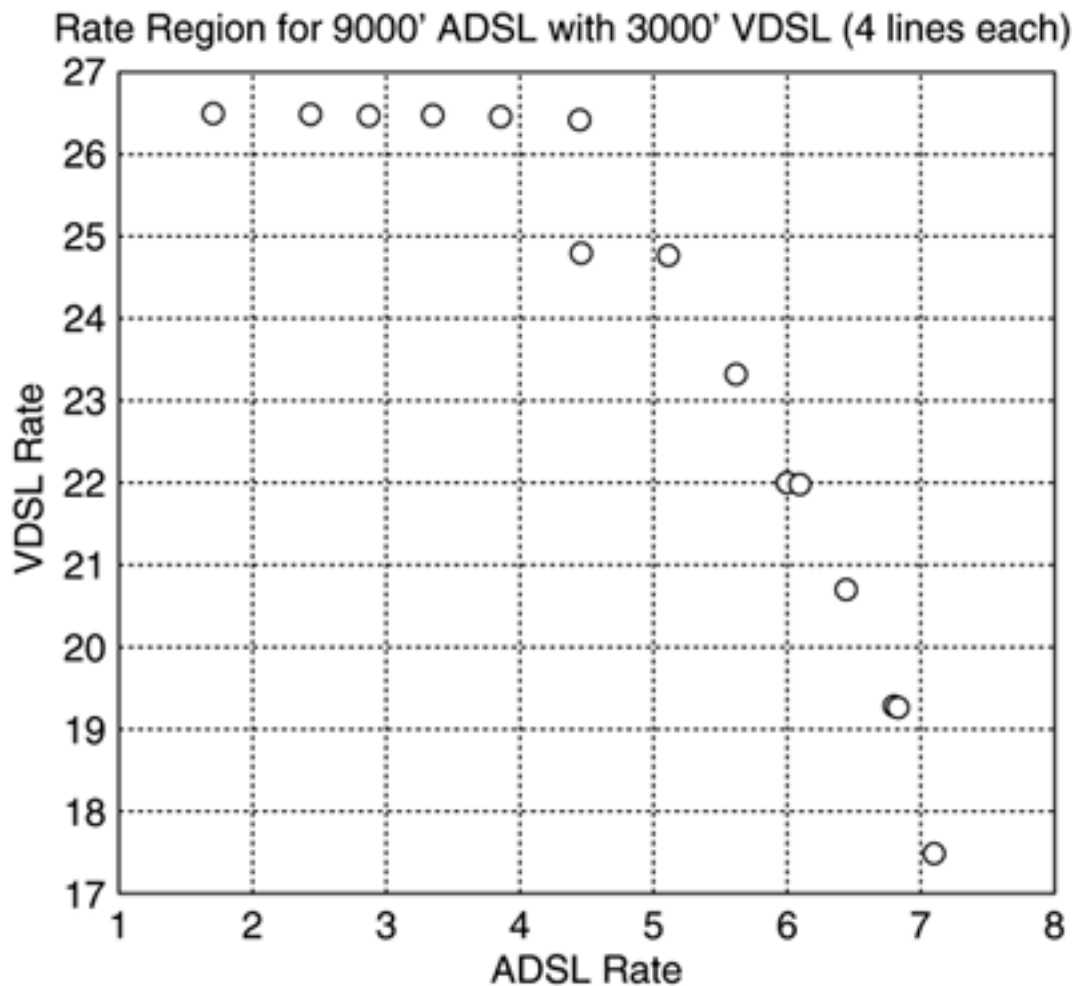
Figure 11.24. Rate region for ADSL and VDSL example.
