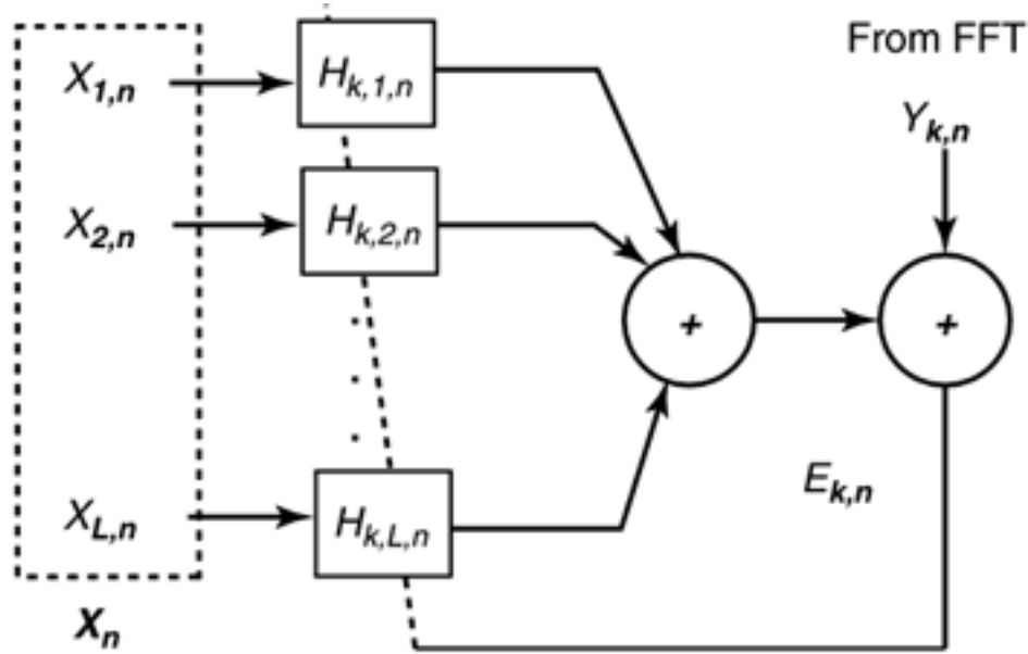
Figure 11.40. Adaptive channel (per tone) for L users.
