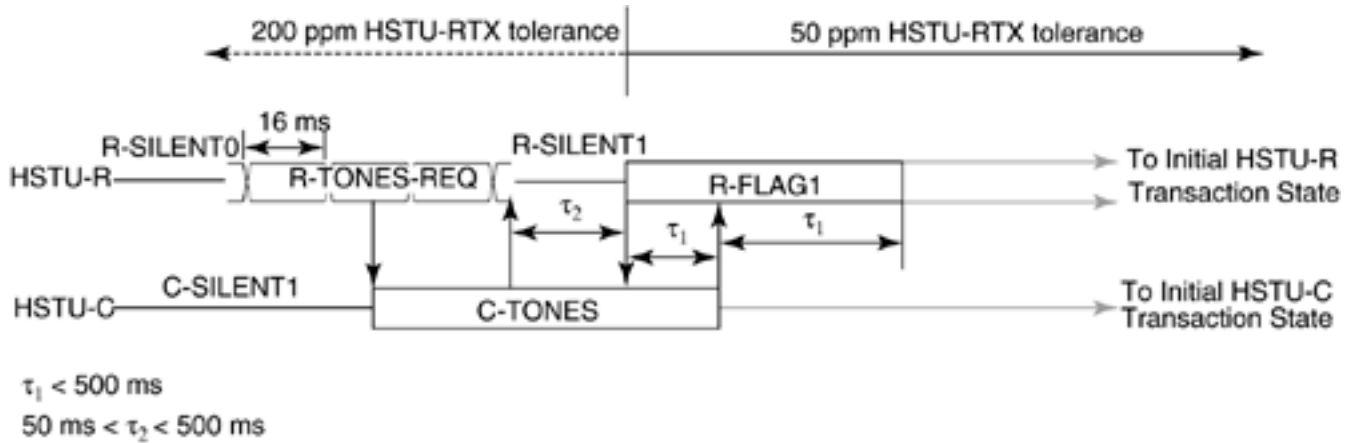
Figure 5.10. CP initiated half-duplex start-up sequence (Figure 16/G.994.1[1]).
