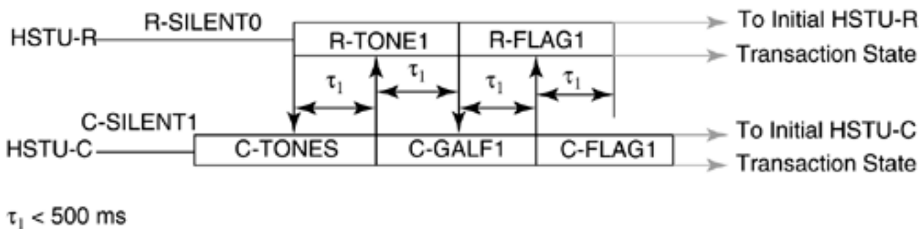
Figure 5.9. CO unit initiated duplex start-up (Figure 15/G.994.1[1]).
