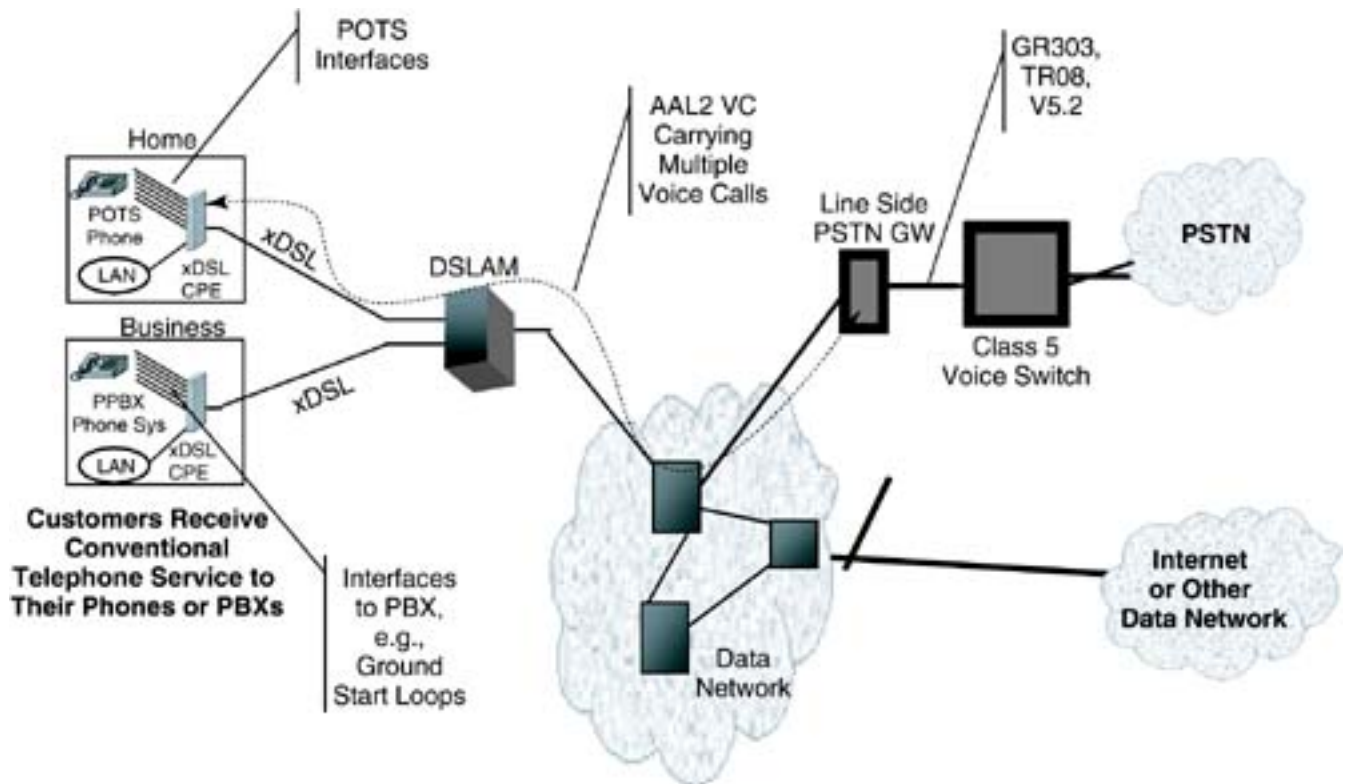
Figure 16.16. CLEC or IXE implementation of loop extension.
