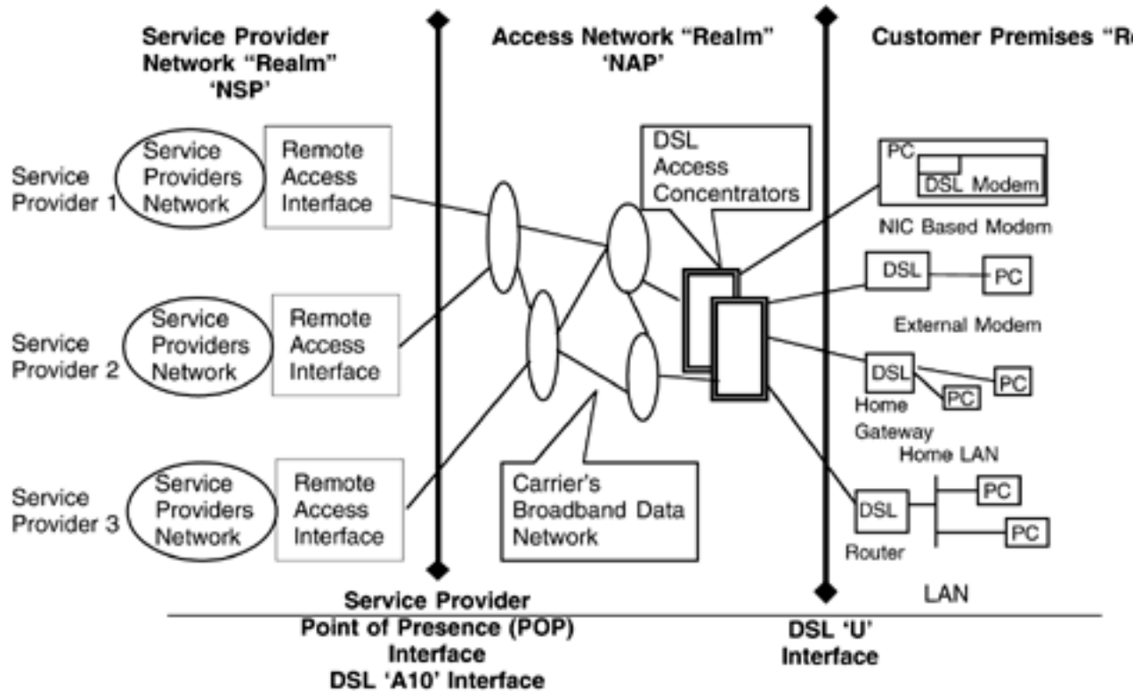
Figure 13.1. Division of realms of management control in a DSL network.
