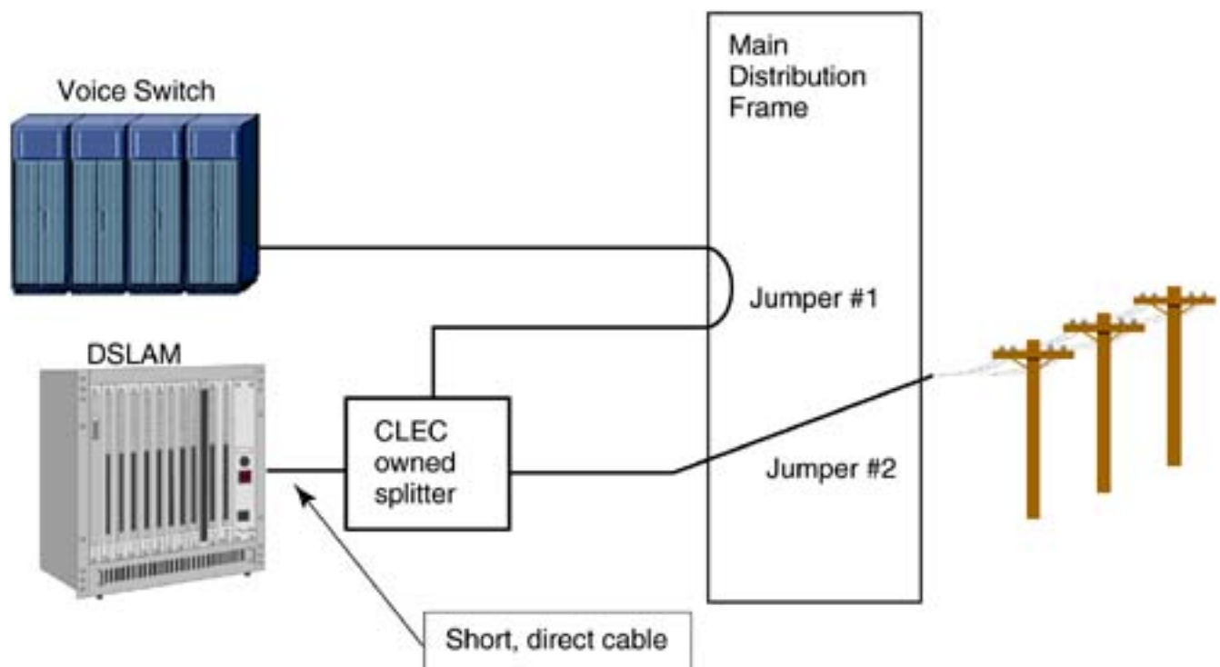
Figure 8.4. Central office configuration with CLEC-owned line sharing splitter.
