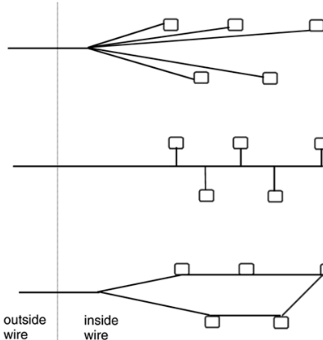
Figure 12.8. Home wiring topologies.
