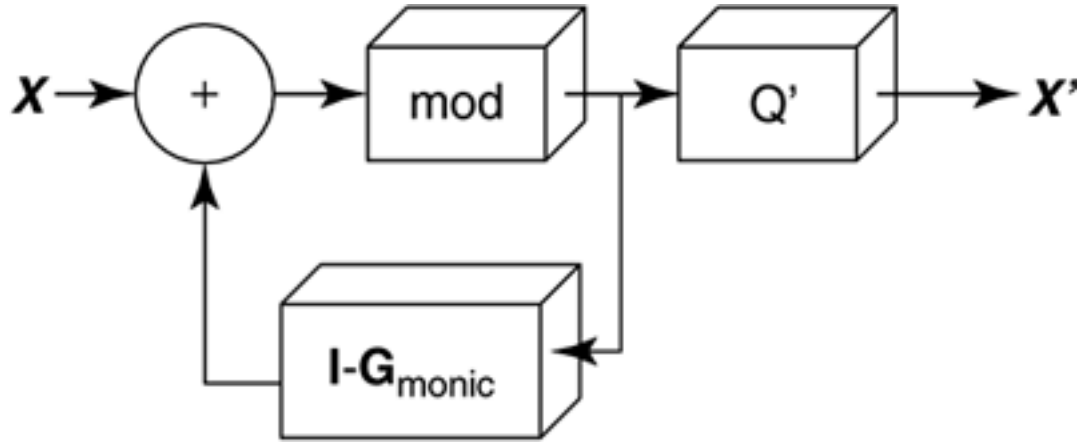
Figure 11.14. Ginis precoder "the channel output is HX' = DX where D is diagonal, so simply scaling by D^{-1} can be executed separately at each independent receiver.
