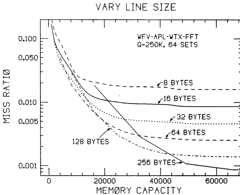
Figure 18. Miss ratios as a function of the line size and memory capacity.
