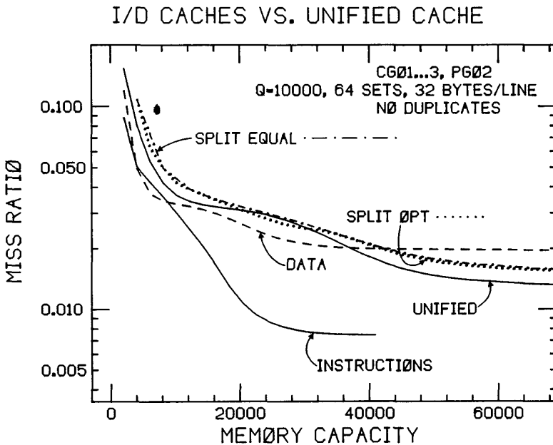
Figure 26. Miss ratio versus memory capacity for instruction/data cache and for unified cache.
