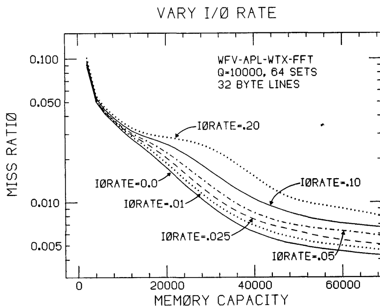
Figure 30. Miss ratio versus memory capacity while I/O occurs through cache.
