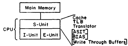
Figure 1. A typical CPU design and the S-unit.
