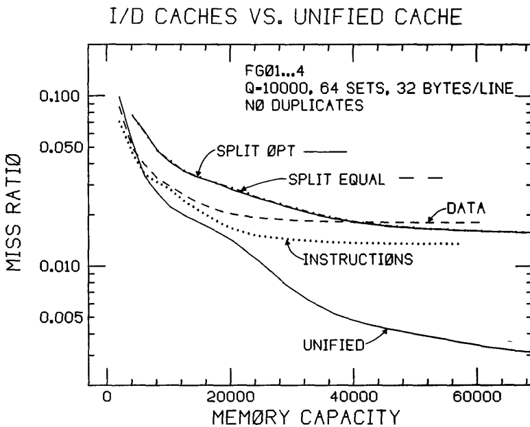
Figure 28. Miss ratio versus memory capacity for instruction/data cache and for unified cache
