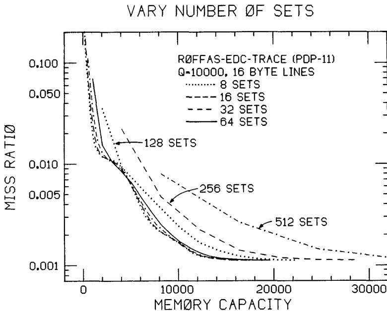
Figure 14. Miss ratios as a function of the number of sets and memory capacity.
