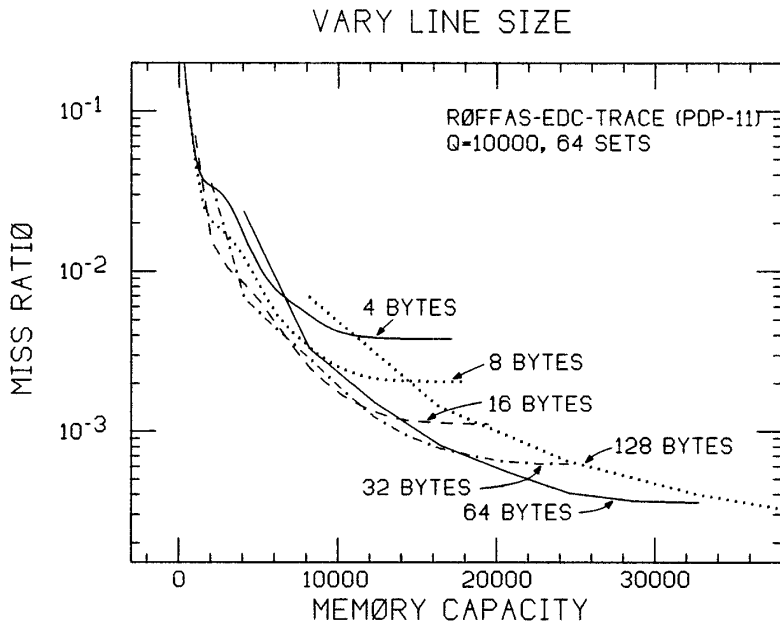
Figure 21. Miss ratios as a function of the line size and memory capacity.
