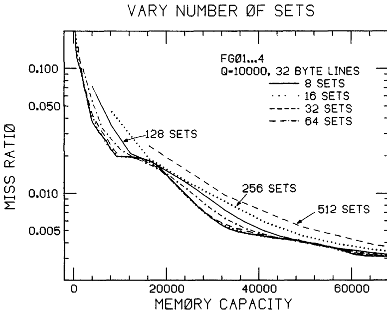
Figure 11. Miss ratios as a function of the number of sets and memory capacity
