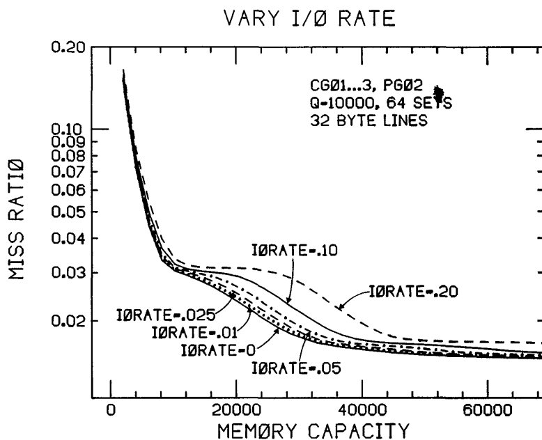
Figure 29. Miss ratio versus memory capacity while I/O occurs through cache at specified rate IORATE refers to fraction of all memory references due to I/O
