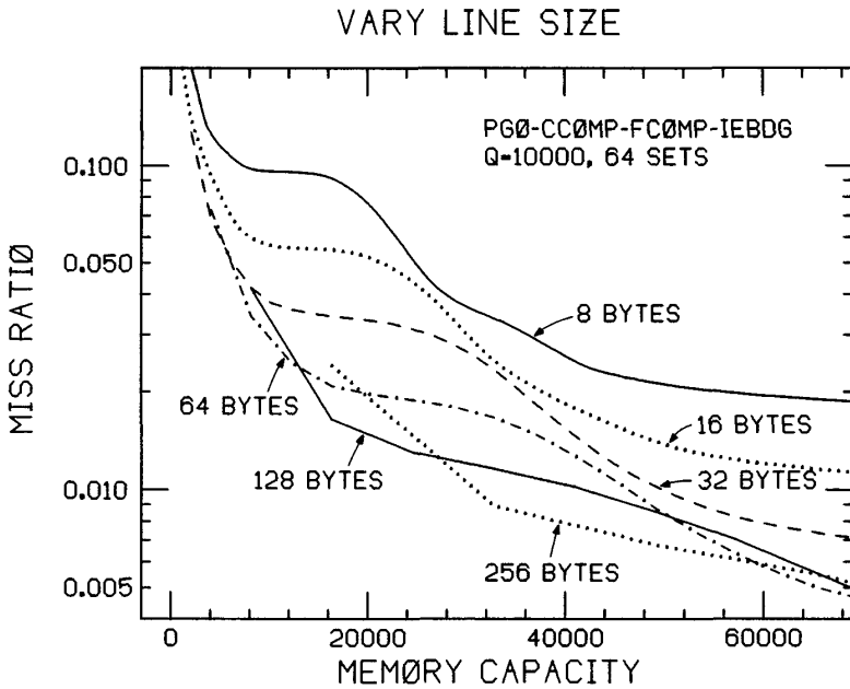
Figure 16. Miss ratios as a function of the line size and memory capacity.
