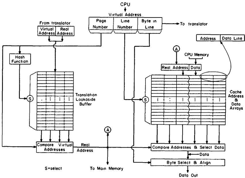
Figure 2. A typical cache and TLB design.
