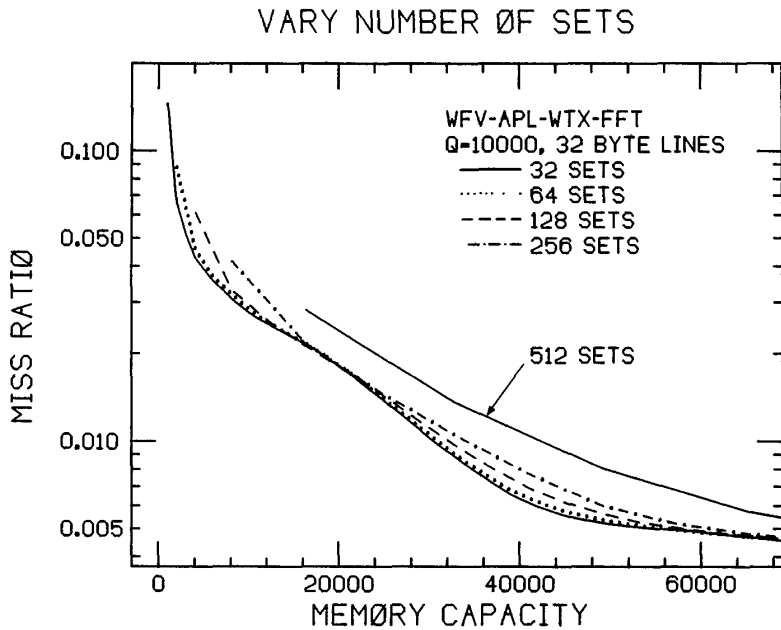
Figure 10. Miss ratios as a function of the number of sets and memory capacity.
