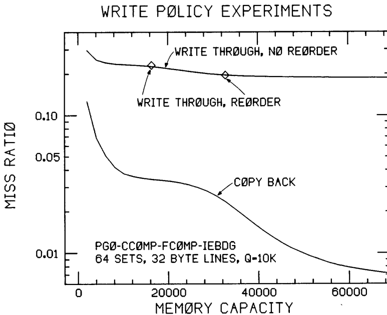
Figure 22. Miss ratio for copy-back and write-through. All writes counted as misses for write-through. No reorder implies replacement status not modified on write, reorder implies replacement status is updated on write.
