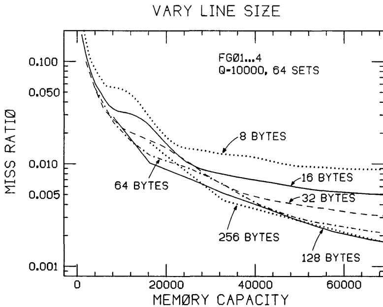
Figure 17. Miss ratios as a function of the line size and memory capacity.
