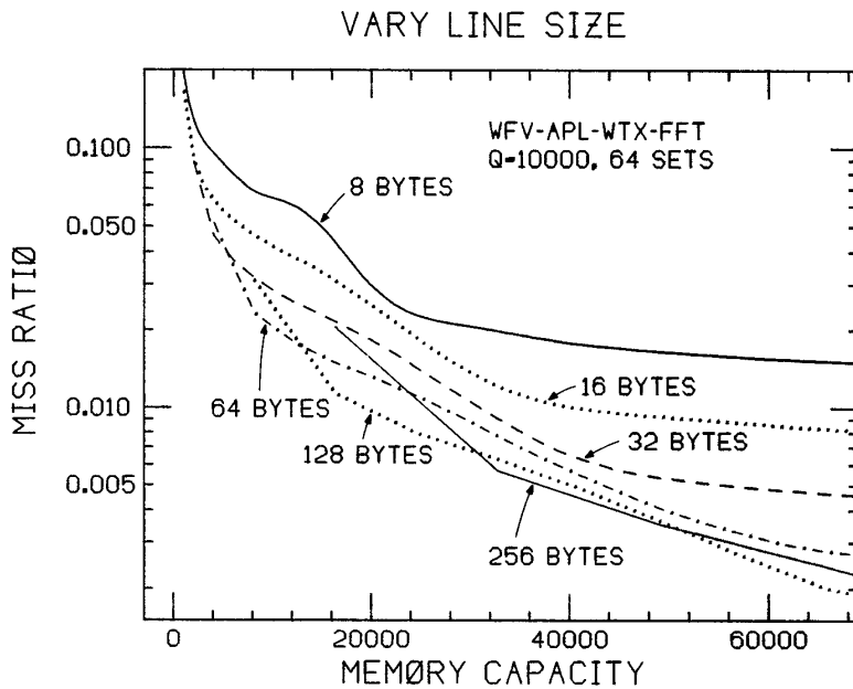
Figure 19. Miss ratios as a function of the line size and memory capacity.
