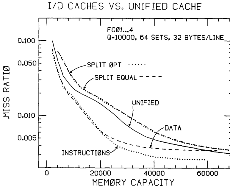
Figure 27. Miss ratio versus memory capacity for instruction/data cache and for unified cache.
