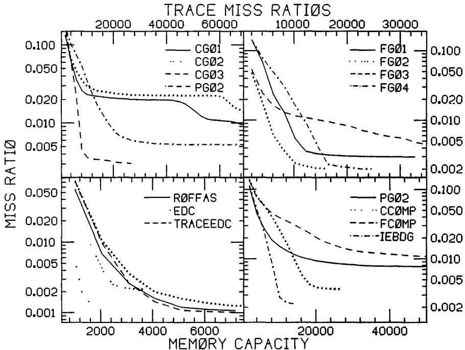
Figure 5. Individual trace miss ratios.
