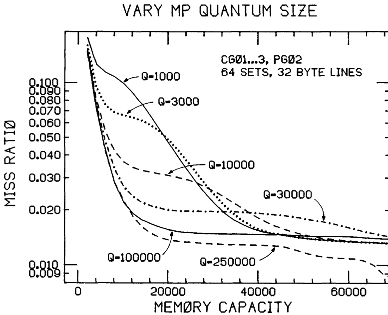
Figure 23. Miss ratio versus memory capacity for range of multiprogramming intervals Q .
