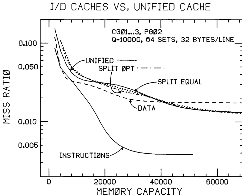
Figure 25. Miss ratio versus memory capacity for unified cache, cache split equally between instruction and data halves, cache split according to static optimum partition between instruction and data halves, and miss ratios individually for instruction and data halves.
