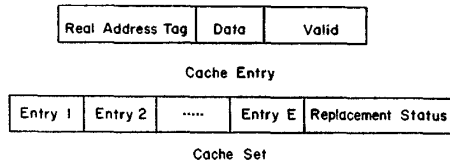
Figure 4. Structure of cache entry and cache set.
