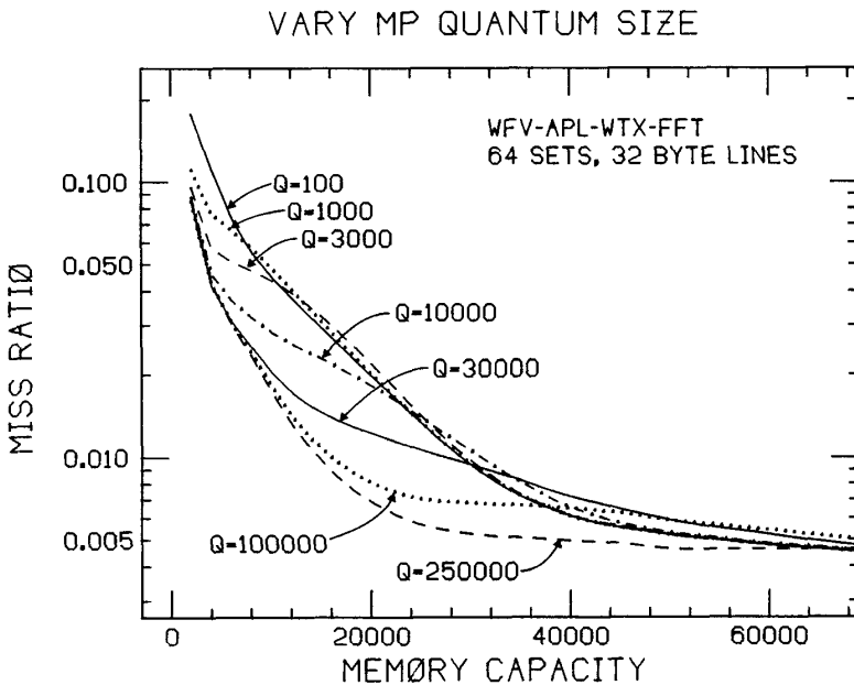
Figure 24. Miss ratio versus memory capacity for variety of multiprogramming intervals Q .
