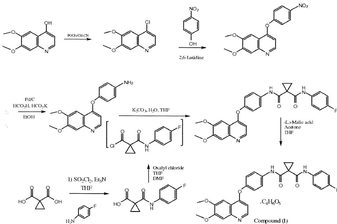
SCHEME 1
