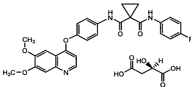
Compound I, L-Malate Salt
