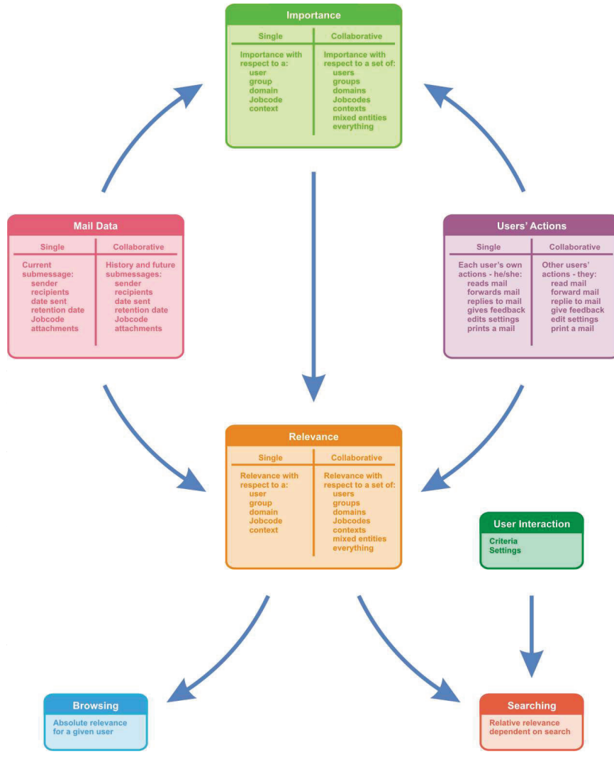
Figure 6 – Relevance overview
