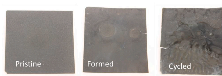
Fig. 4. Photographs of the delaminated pristine, formed, and cycled LCO cathodes (approximate size 2.5 cm × 2.5 cm) showing mechanical damage increase as the cell cycles.
