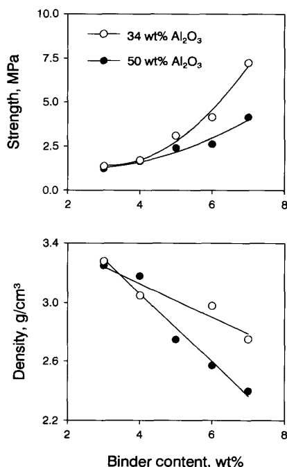
Fig. 6. Strength (top) and density (bottom) of alumina green tapes with different powder charges as a function of HEC wt.% [18].
