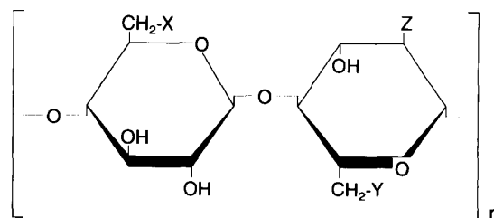
Fig. 3. Structural formula of cellulose derivatives.
