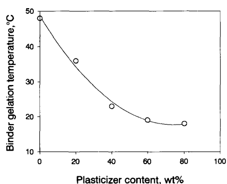
Fig. 8. Effect of the plasticizer content on the binder T_g [32]. Plasticizer is PEG, binder is PVA.
