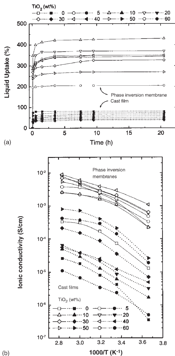
Fig. 4. (a) Liquid uptake and (b) Arrhenius plot for the ionic conductivities of PVdF-HFP/TiO 2 films, with varying TiO 2 content, prepared by casting (filled symbol) and phase inversion (hollow symbol) methods. The electrolyte solution used was 1 M LiPF 6 dissolved in EC/DMC (1:1 w/w).
