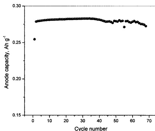
Fig. 9. Specific capacity upon discharge for the lithium-ion cell described in Fig. 8.
