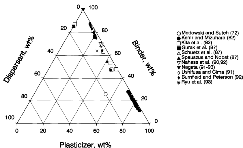
Fig. 2. Organic additive formulations used in aqueous slurries for tape casting.
