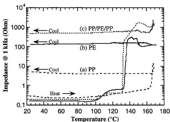
Fig. 3 Separator thermal shutdown [13]
