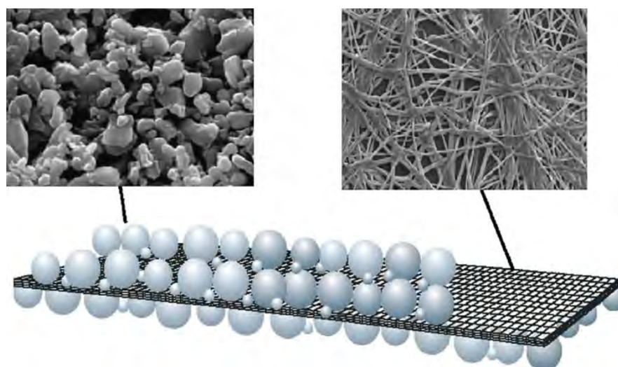
Fig. 5 Schematic of an Evonik–Degussa ceramic separator [8, 77]
