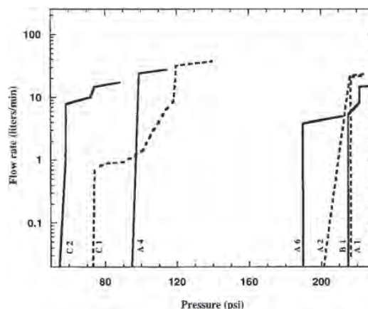
Fig. 2. Flow rate vs. pressure curves for commercial Li-ion battery separators.
