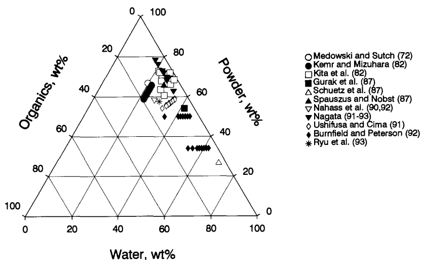
Fig. 1. Aqueous slurry formulations for tape casting. The ceramic powder is alumina, with the exception of Ushifusa and Cima [17], who used mullite.
