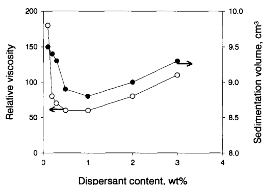
Fig. 9. Relative viscosity and sedimentation volume of an alumina/water suspension as a function of dispersant amount (adapted from Ref. [21]).
