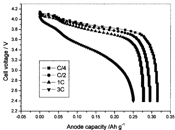
Fig. 10. Voltage profile for a lithium-ion cell cycled at different discharge rates. Discharge current densities: 0.42, 0.84, 1.65, and 4.97 mA cm -2 . The cell was charged at 1.65 mA cm -2 to 4.2 V and this voltage was applied until the current flow decreased at 1/10th of the charging current. The anode loading of graphite was 5.0 mg cm -2 .
