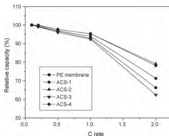
Fig. 6. Relative capacities of lithium-ion cells prepared with PE membrane or ceramic-coated separators as a function of C rate.
