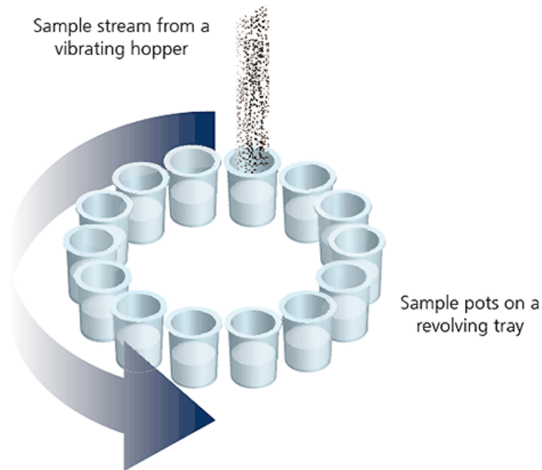
Figure 11: Illustration of a spinning riffler device.
