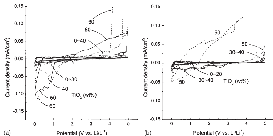
Fig. 5. Electrochemical window of PVdF-HFP/TiO 2 electrolyte films, with varying TiO 2 content, prepared by (a) casting and (b) phase inversion methods. The electrolyte solution used was 1 M LiPF 6 dissolved in EC/DMC (1:1 w/w).
