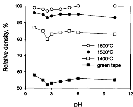
Fig. 10. Relative density as a function of slurry pH for green and sintered tapes of alumina [24].
