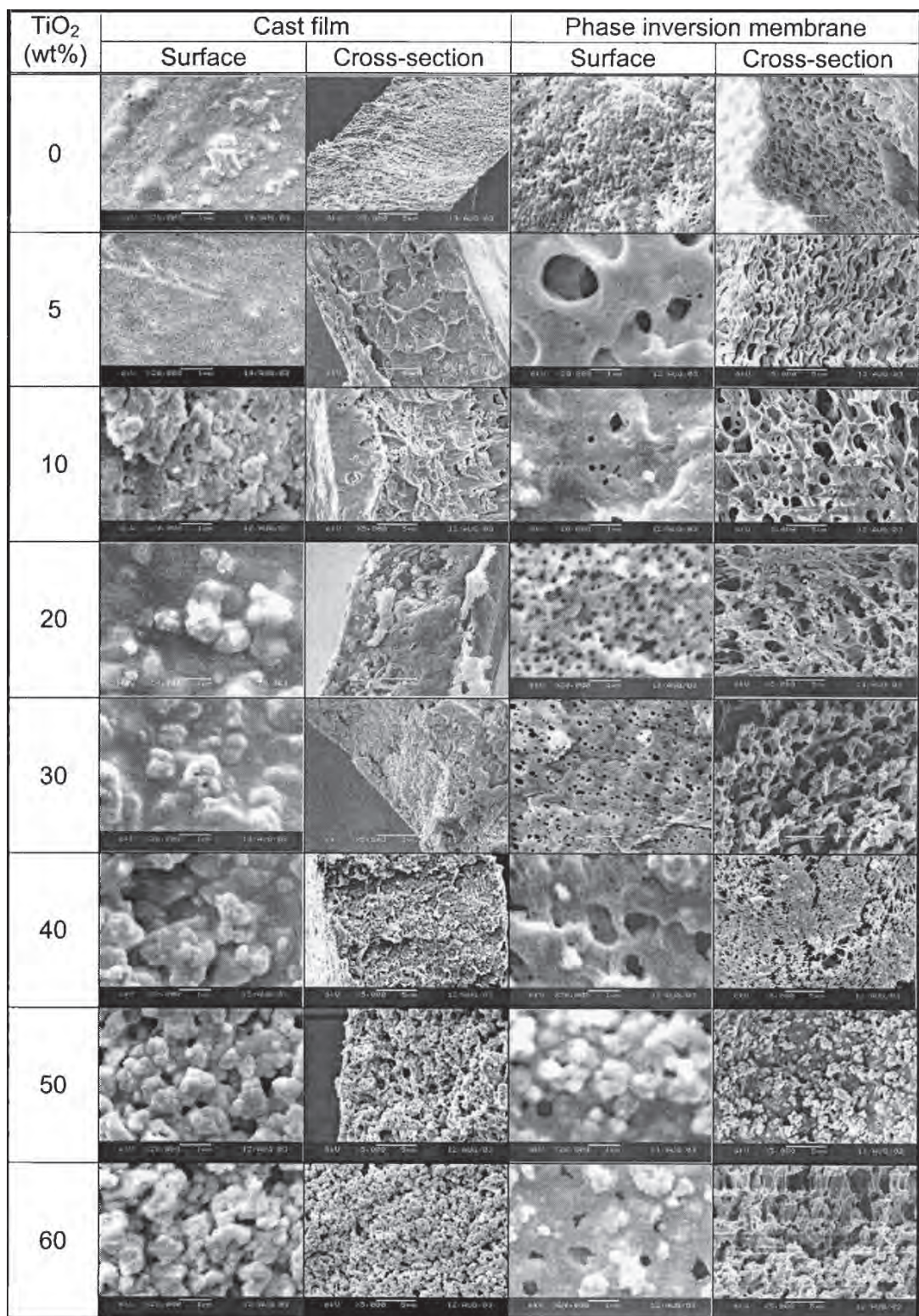
Fig. 1. Scanning electron microscope images of PVdF-HFP/TiO 2 films, with varying TiO 2 content, prepared by casting and phase inversion methods. Image magnifications were 20,000 \times and 5000 \times for surface and cross-sectional views, respectively.
