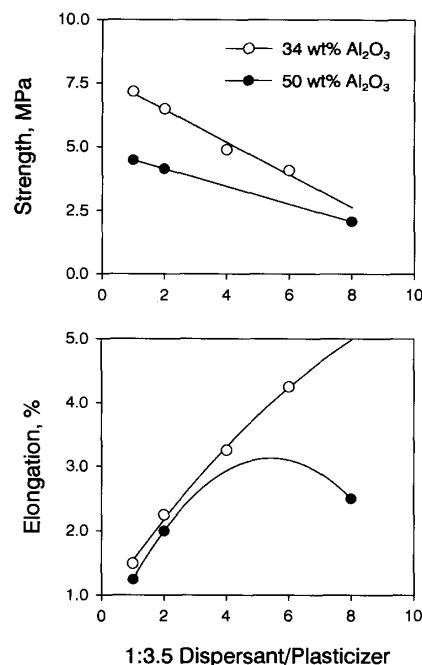
Fig. 7. Strength (top) and elongation (bottom) of alumina green tapes with different powder charges as a function of dispersant/plasticizer amount [18].
