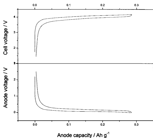
Fig. 8. Voltage profiles for a lithium-ion battery cell (top) and for the graphite anode measured against Li reference electrode (bottom). The cell was anode limited. The cell was charged at 0.5 \text{ mA cm}^{-2} for 1.5 h. The cell was discharged at the same current to 1.5 V. The anode loading of graphite was 2.7 \text{ mg cm}^{-2} .
