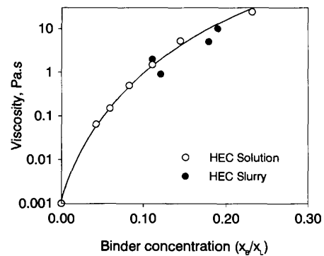
Fig. 11. Viscosity of aqueous HEC solutions and slurries at shear rate 20 \text{ s}^{-1} as a function of the binder concentration [30].
