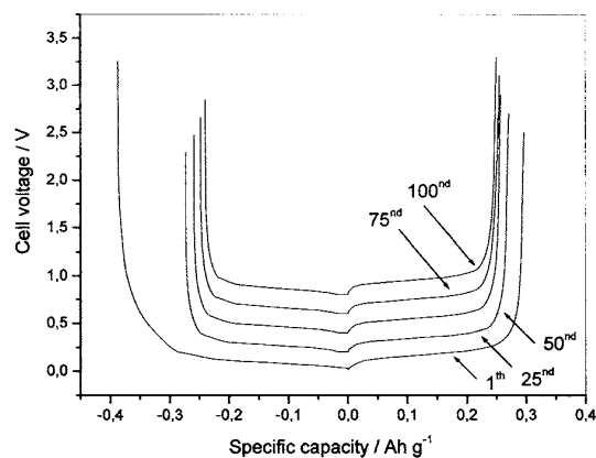
Fig. 5. Selected voltage profiles for a Li/fibre-glass/MgO-based separator/anode cell. Discharge current was 0.55 \text{ mA cm}^{-2} to 5 mV vs. Li, then the cell was left to equilibrate until the current density was less than 0.055 \text{ mA cm}^{-2} . Charge current density was 0.55 \text{ mA cm}^{-2} . The anode loading of graphite was 2.9 \text{ mg cm}^{-2} .
