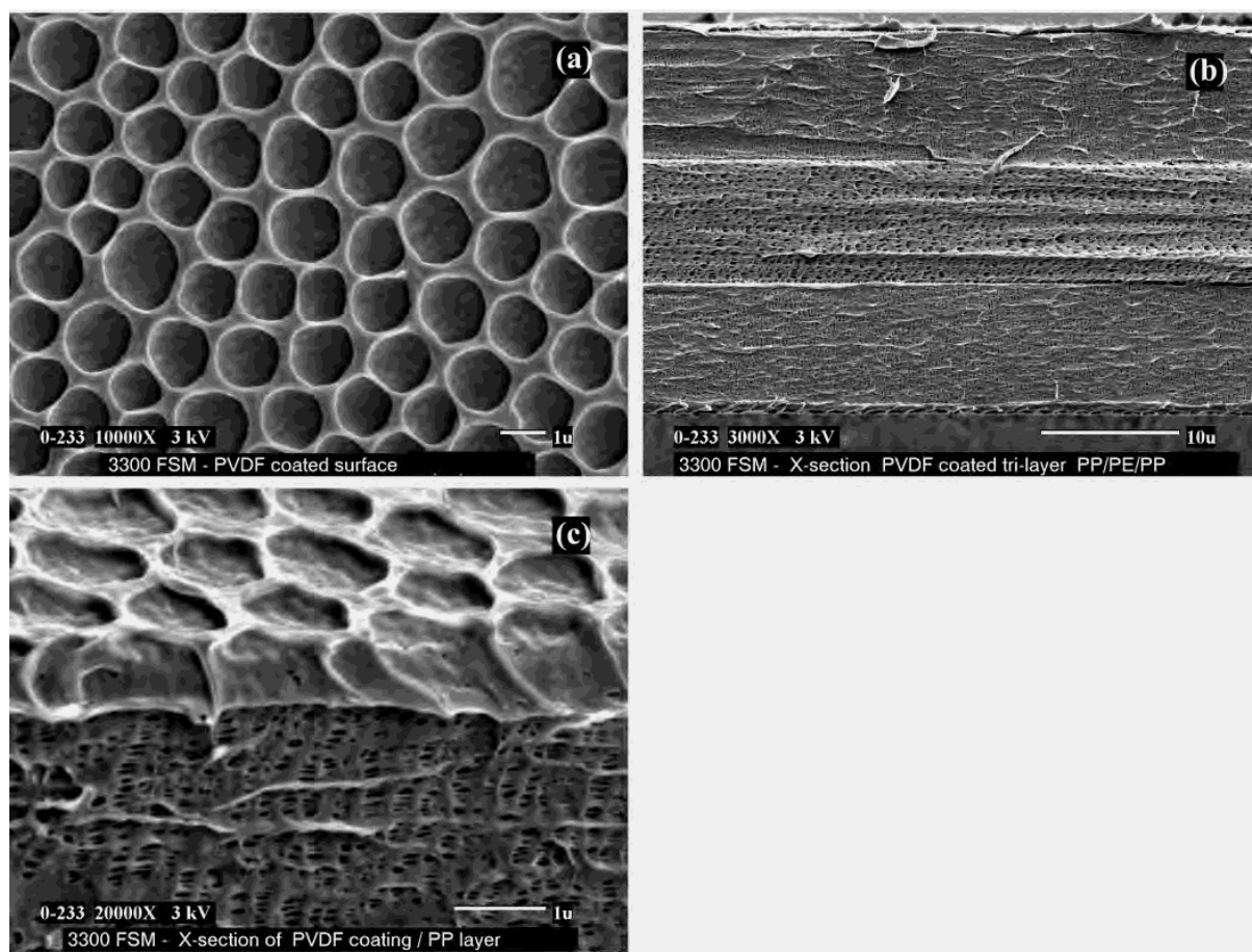
Figure 14. Scanning electron micrographs of Celgard PVdF coated separators used in lithium gel polymer batteries: (a) surface SEM, (b) cross-section SEM of coated trilayer, and (c) cross section of PVdF coating.
