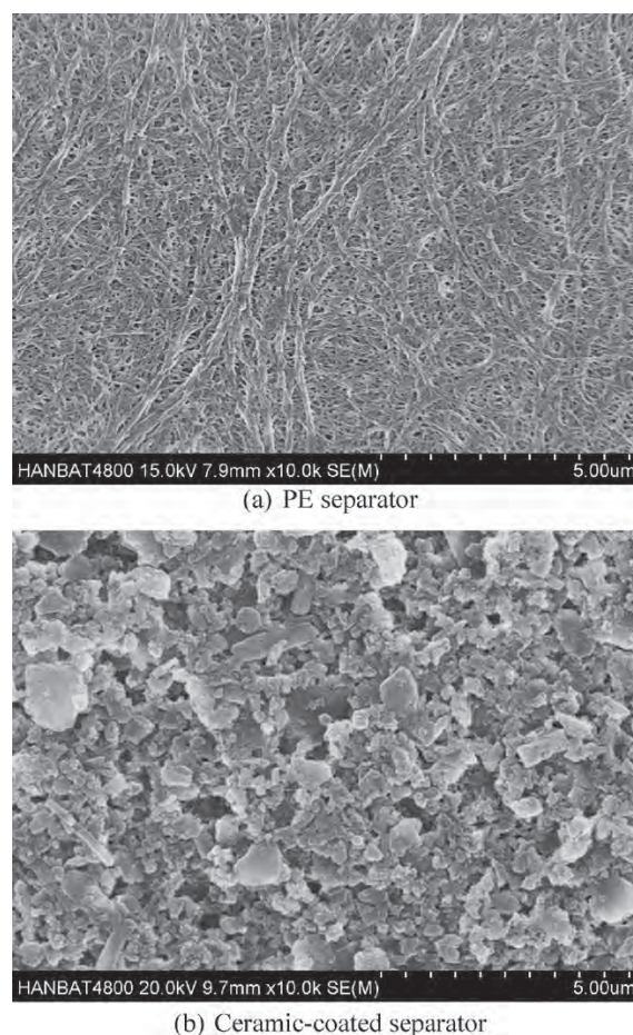
Fig. 1. Scanning electron micrographs of the surface of a porous PE membrane and ceramic-coated separator (ACS-3).
