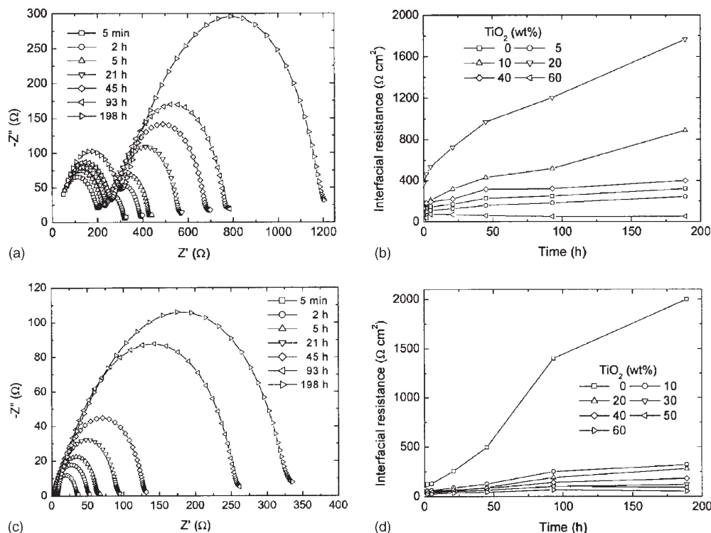
Fig. 6. Impedance spectra of PVdF-HFP/TiO 2 (10 wt.%) electrolytes on lithium electrodes as a function of time, which are prepared by (a) cast and (c) phase inversion techniques. Time evolutions of interfacial resistance between polymer electrolytes of (b) cast film and (d) phase inversion membrane, and lithium electrodes. The electrolyte solution used was 1 M LiPF 6 dissolved in EC/DMC (1:1 w/w).
