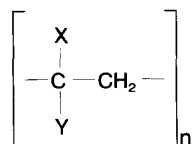
Fig. 4. General formula of vinyl and acrylic-type derivatives.
