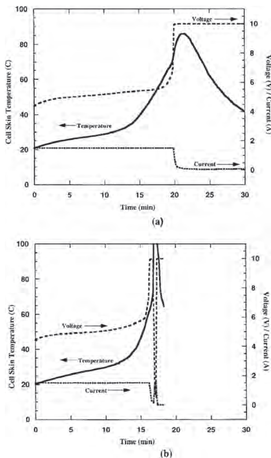
Fig. 8. (a) Overcharge test results for a cell containing a polypropylene/polyethylene/polypropylene trilayer separator. (b) Overcharge test results for a cell containing a polypropylene separator.
