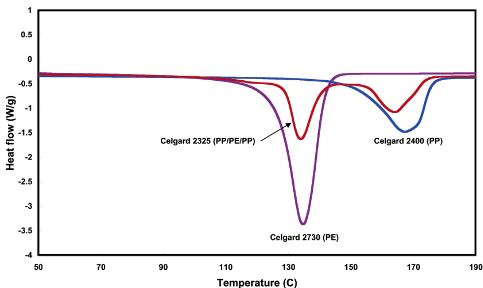
Figure 8. DSC of Celgard 2730 (PE), 2400 (PP), and 2325 (PP/PE/PP).
