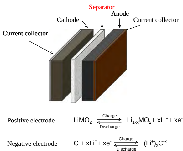
Fig. 1 Schematic of a liquid electrolyte Li-ion cell
