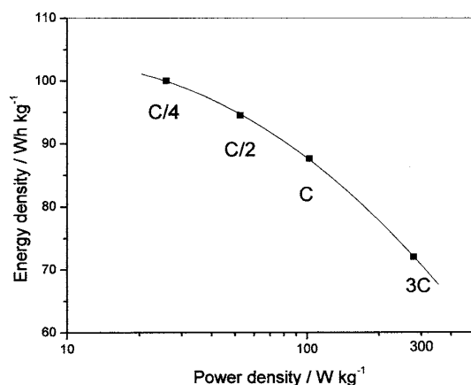
Fig. 11. Ragone plot for the lithium-ion cell described in Fig. 10. The energy and the power densities are based on the total weight of the cell, comprising the liquid electrolyte, without including the weight of the current collectors.
