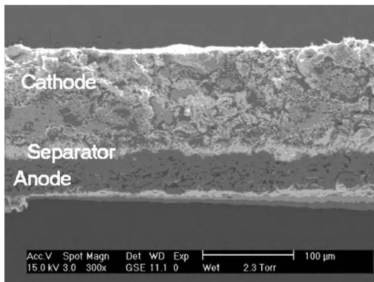
Fig. 7. SEM micrograph cross-section of an anode/MgO-based separator/cathode hot laminated cell.
