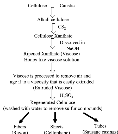
Figure 15. Viscous process for regenerated cellulose. 263
