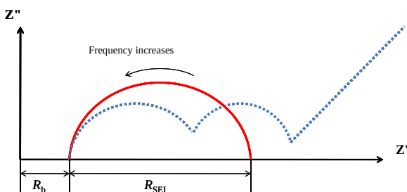
Fig. 2 Schematic of a simplified AC impedance spectrum
