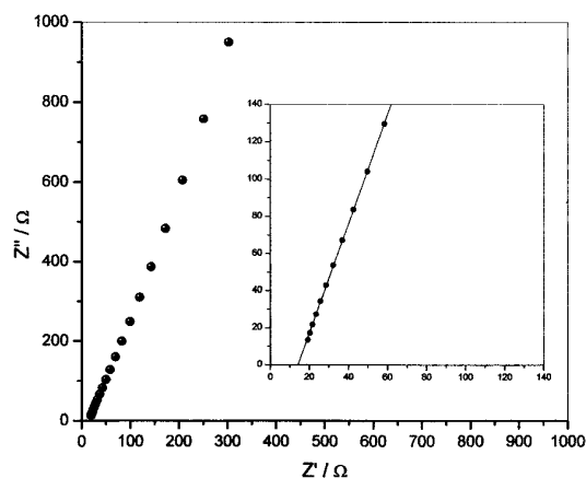
Fig. 6. Impedance spectra for a symmetrical SS/MgO-based separator/SS cell. The liquid electrolyte weight fraction in the separator was about 40%. Frequency range: 100 kHz–500 Hz. Electrode surface area: 0.785 \text{ cm}^2 . The insert shows the impedance spectra recorded in the frequency range from 100 kHz to 5000 Hz.
