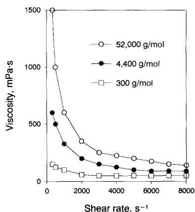
Fig. 5. Viscosity of a 2% aqueous solution of HEC with different molecular weights as a function of shear rate [31].
