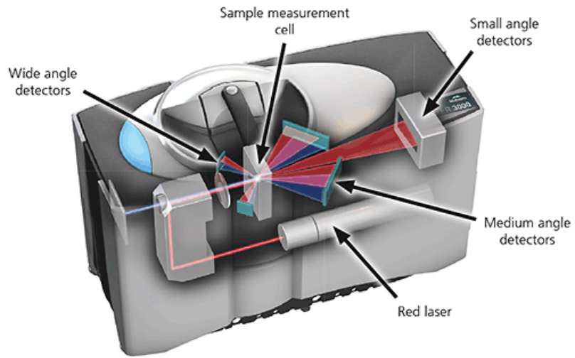
Figure 14: Optical layout of a state-of-the-art laser diffraction instrument.
