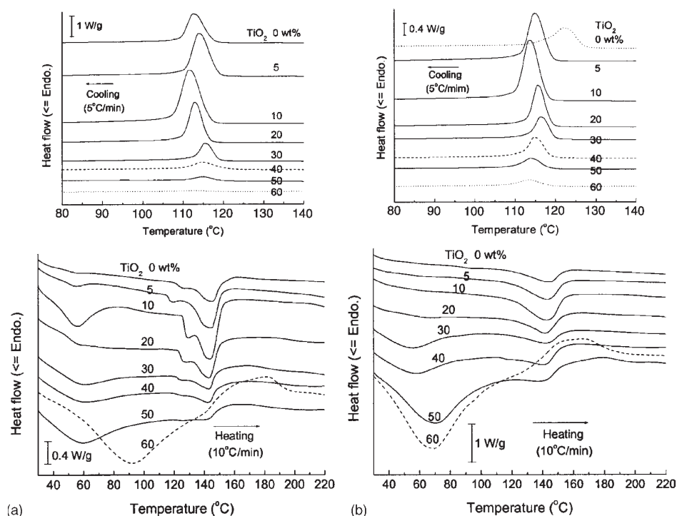
Fig. 2. Differential scanning calorimetric thermograms of PVdF-HFP/TiO 2 films, with varying TiO 2 content, prepared by (a) casting and (b) phase inversion methods. Small figures in upper part are the results of cooling run at -5^{\circ}\text{C min}^{-1} , examined after heating run from room temperature to 250^{\circ}\text{C} at 10^{\circ}\text{C min}^{-1} .
