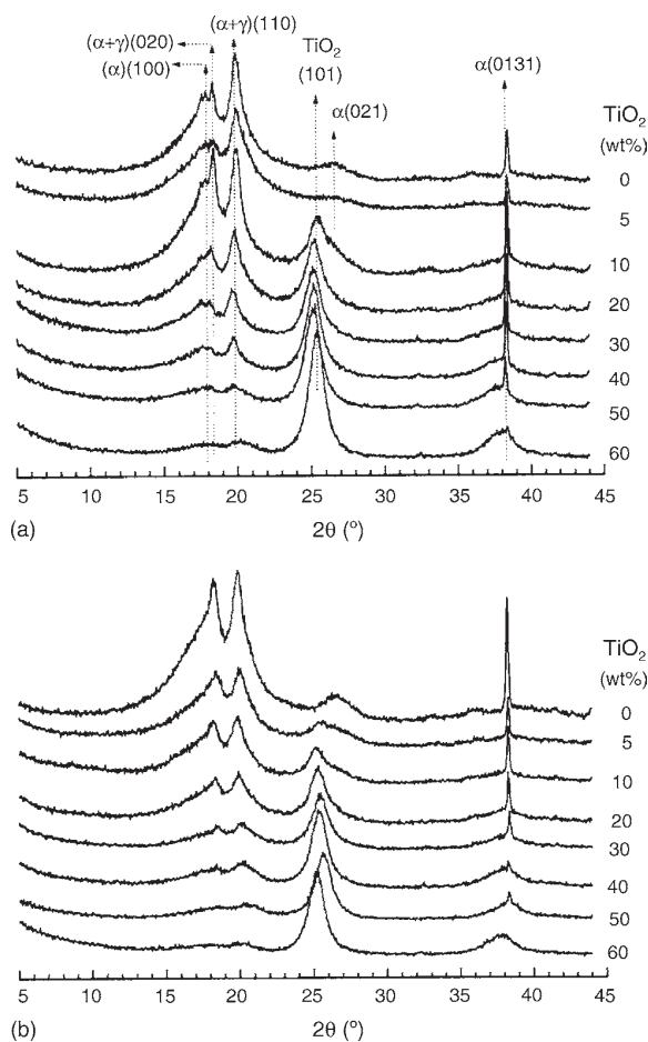
Fig. 3. X-ray diffraction spectra of PVdF-HFP/TiO 2 films, with varying TiO 2 content, prepared by (a) casting and (b) phase inversion methods.
