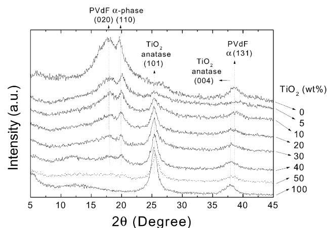
Fig. 3. Wide-angle X-ray diffraction spectra of the P(VdF-HFP)- \text{TiO}_2 films. As a reference, powder sample was only used for the \text{TiO}_2 100 wt%.
