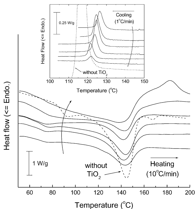
Fig. 2. Differential scanning calorimetric thermograms of the P(VdF-HFP)- \text{TiO}_2 films: results from heating run (rate 10 °C/min). The upper inset is from the cooling run (rate -1 °C/min). Arrows covering over the thermogram curves indicate 'increasing \text{TiO}_2 content' (5, 10, 20, 30, 40, 50 wt% in sequence).
