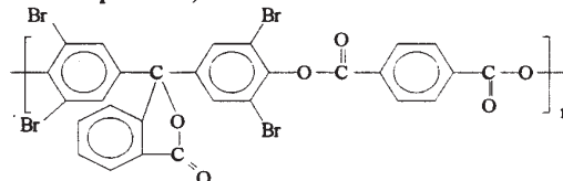
XXXVII Tetrabromo poly(phenol phthaleine phthalate)
