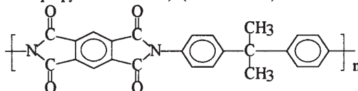
LIX Copoly(pyromellitic dianhydride - isopropylidene diamine) (PMDA-IPDA)
