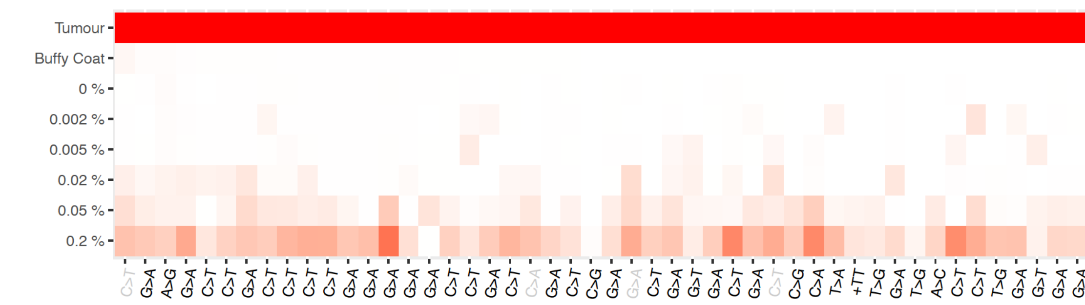
Figure 3: Initial variants chosen during the NeoGenomics RaDaR ® methodology were compared to sequencing of the tumor, buffy coat, and the sample plasma. Variants were removed from consideration if present in the normal control (Buffy Coat). The figure illustrates variant detection for one set of matrix samples (squamous lung) from the normal control to the highest tested VAF.
