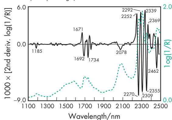
Figure 2: Near-infrared spectrum of alcohol (absolute) measured by transmittance (1 mm path-length).
