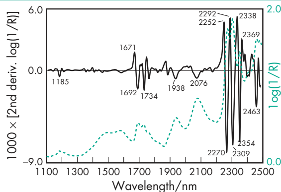
Figure 1: Near-infrared spectrum of alcohol (96%) measured by transmittance (1 mm path-length).
