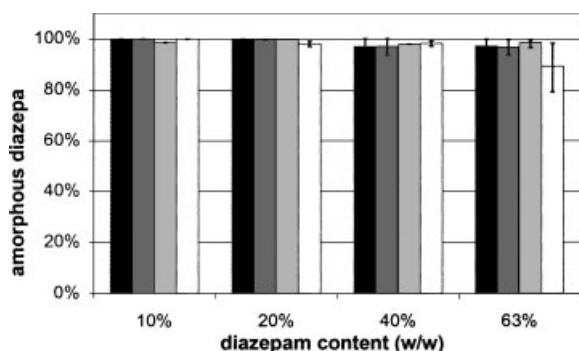
Figure 6. Fraction amorphous diazepam in solid dispersions after freeze drying (key: dark columns: inulin DP23; medium-dark columns: inulin DP11; shaded columns: trehalose; open columns: sucrose; average values; n=2-5 ; bars indicate lowest and highest values).
