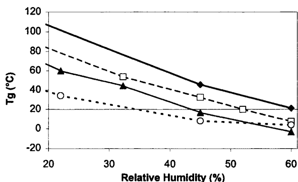
Figure 2. T_g s of the sugars used after conditioning at different RHs (key: \blacklozenge : inulin DP23; \square : inulin DP11; \blacktriangle : trehalose; \circ : sucrose).
