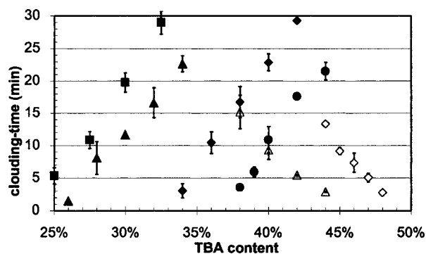
Figure 4. Clouding times of inulins and lipophilic drugs in different water/TBA solutions. (key: ■: diazepam 1.0% w/v; ▲: nifedipine 1.0% w/v; ◆: CSA 1.0% w/v; ●: THC 0.4% w/v; △: inulin DP23 9.0% w/v; ◇: inulin DP11 9.0% w/v; n = 8-12 ; error bars indicate standard deviation).
