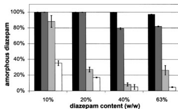
Figure 8. Fraction of amorphous diazepam after storage for 60 days at 20^{\circ}\text{C}/45\% \text{RH} (key: dark columns: inulin DP23; medium-dark columns: inulin DP11; shaded columns: trehalose; open columns: sucrose; average values, n = 2-3 ; bars indicate lowest and highest values).
