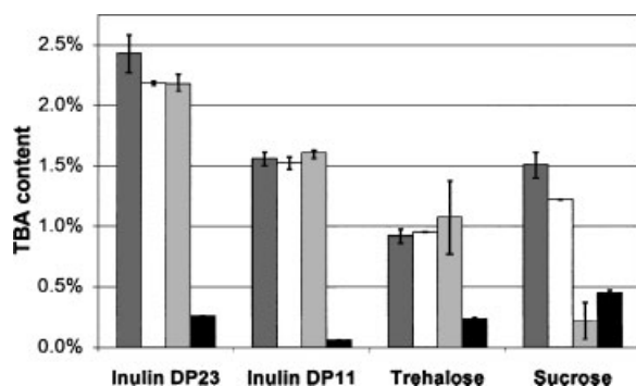
Figure 7. Content of TBA from freeze dried sugars before and after 7 days storage (key: medium-dark columns: before storage; open columns: 20°C/11% RH, shaded columns: 20°C/33% RH, dark columns: 20°C/45% RH; average values, n = 2-3 ; bars indicate lowest and highest values).
