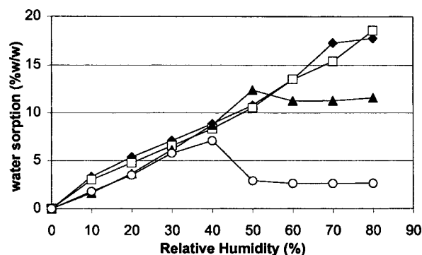
Figure 3. Water vapor sorption isotherms of lyophilized sugars at 24^{\circ}\text{C} (key: \blacklozenge : inulin DP23; \square : inulin DP11; \blacktriangle : trehalose; \circ : sucrose).
