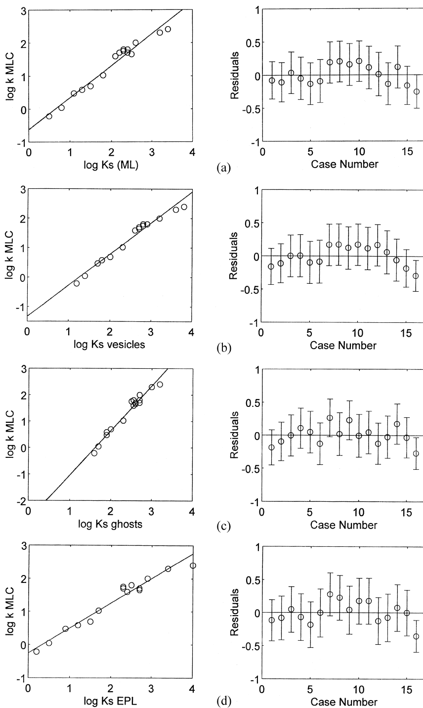
Fig. 1. Comparison between the retention data in MLC ( \log k_{\text{MLC}} ) for a heterogeneous set of compounds at 0.02 M Brij 35 mobile phase and retention data, \log K_s , on (a) red cell membrane lipid liposomes, (b) human red cell membranes vesicles, (c) native membranes of adsorbed red cells, ghosts and (d) egg phospholipids liposomes, EPLs; together their residuals plots.
