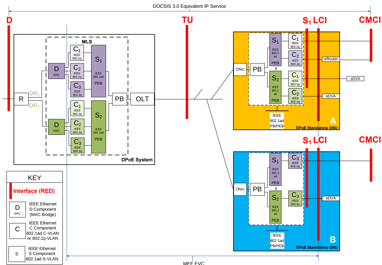
Figure 15 - IP(HSD) Implementation of MEF EVCs with MLS
