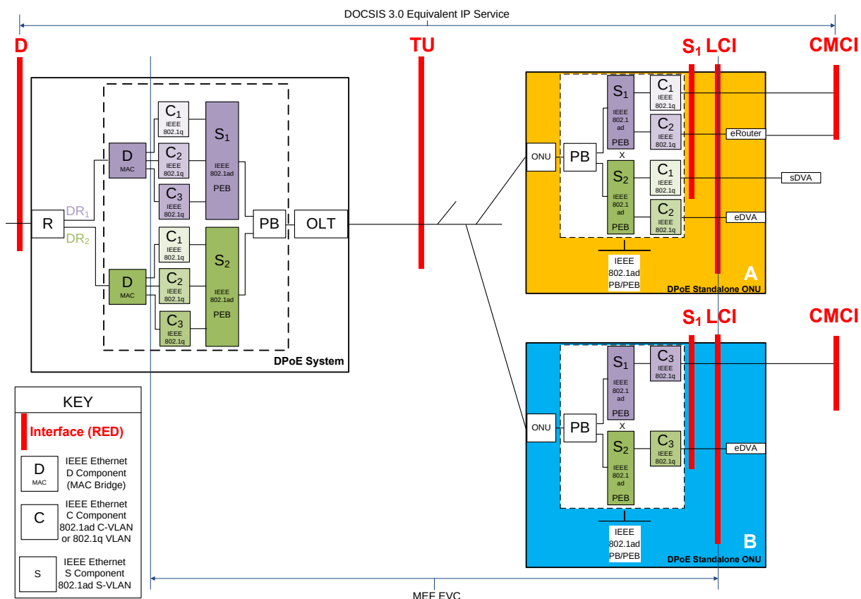
Figure 12 - IP(HSD) Implementation of MEF with [802.1ad]
