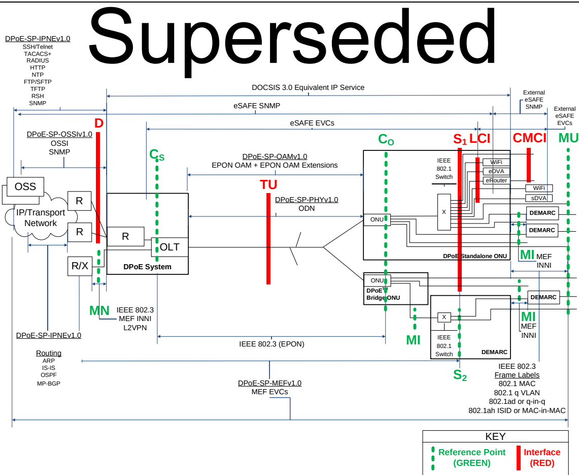
Figure 2 - DPoE Interfaces and Reference Points
