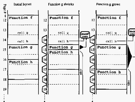
Fig. 1. Pure diff-based approach. Tabs indicate which pages are rewritten.
