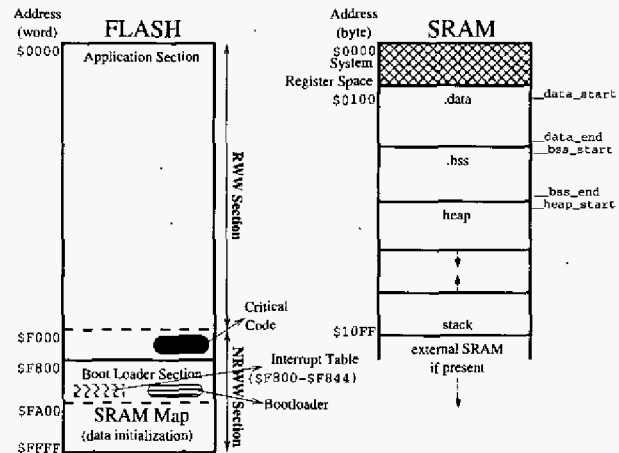
Fig. 3. ATMega128 memories.
