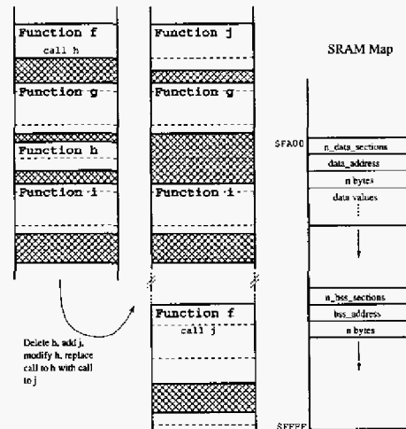
Fig. 4. Updating flash; data initialization region layout.
