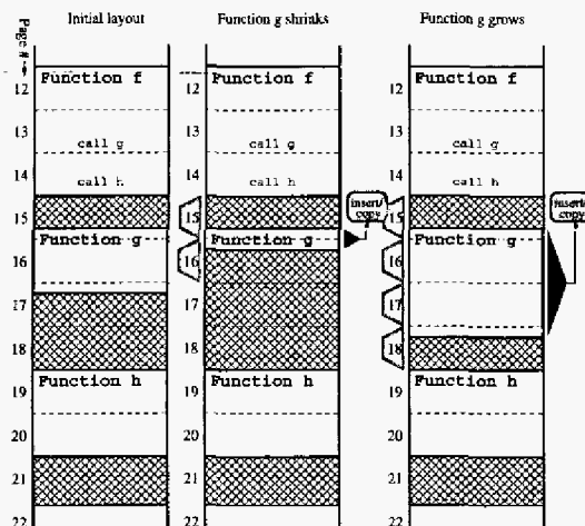
Fig. 2. Incremental linking approach. Slop space is hatched, and tabs indicate which pages are rewritten.
