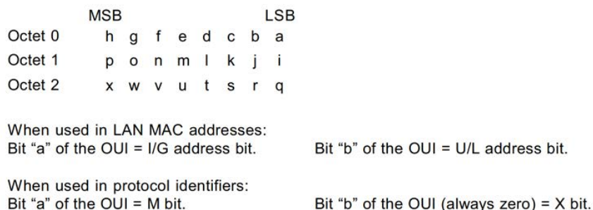
Figure 10—Bit significance of an OUI
