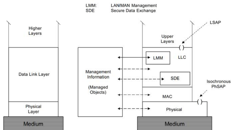
Figure 3—IEEE 802 RM with end-station management and security
