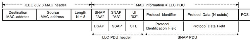
Figure 17—SNAP PDU in IEEE 802.3 MAC frame
