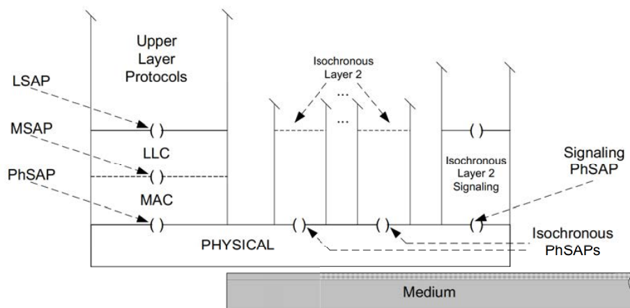
Figure 19—ISLAN RM (end station)
