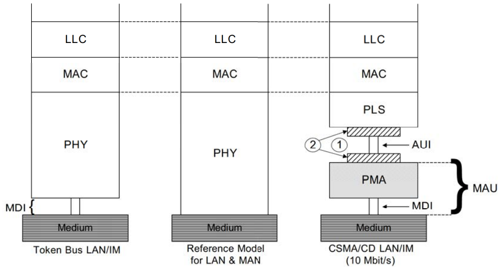
Figure 2—IEEE 802 RM and two examples of end-station implementation model
