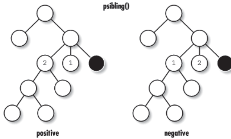
Figure 3.10, The path of psibling()
