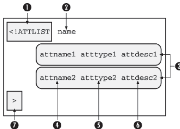
Figure 5.4, Attribute declaration list syntax
