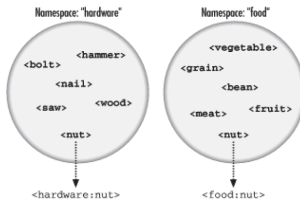
Figure 2.11, Qualifying an element's namespace with prefixes
