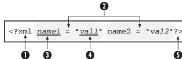
Figure 2.5, XML declaration syntax
