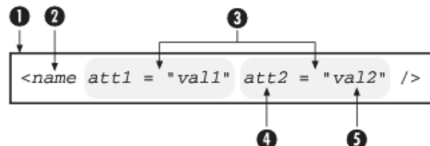
Figure 2.8, Empty element syntax
