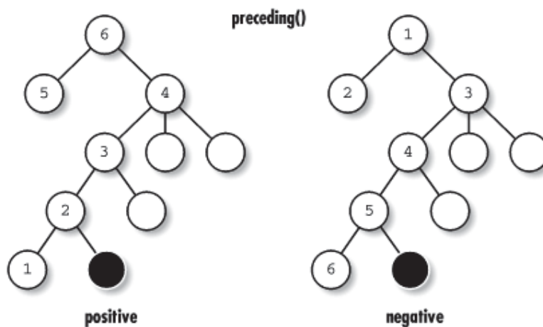
Figure 3.8, The path of preceding()
