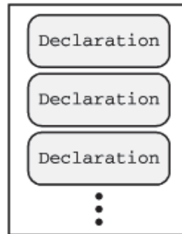
Figure 5.2, DTD syntax
