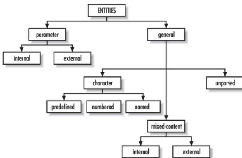
Figure 2.13, Taxonomy of entities
