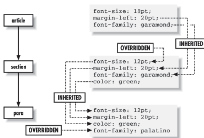
Figure 4.9, Element-inheriting properties
