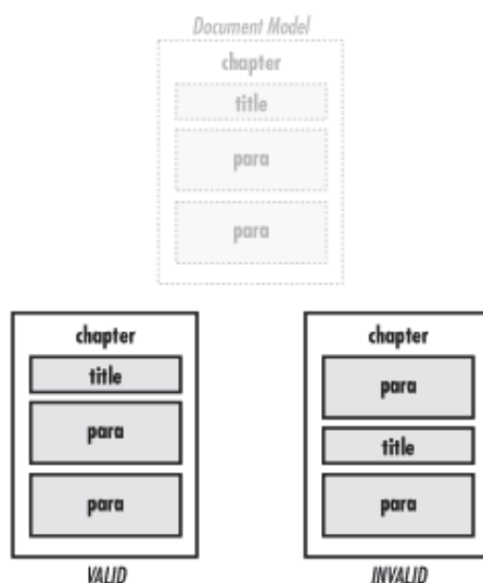
Figure 5.1, Comparing documents to a model
