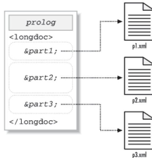
Figure 2.16, A compound document
