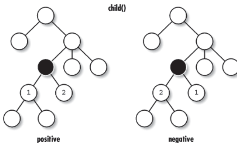
Figure 3.5, The path of child()
