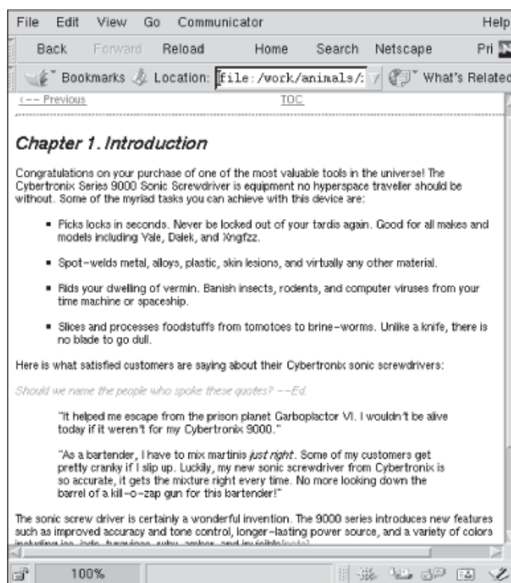
Figure 6.3, A page produced from the transformation
