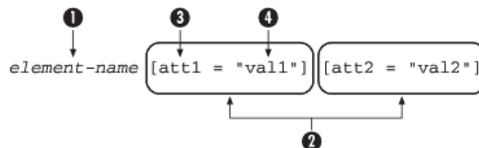
Figure 4.7, Syntax for a CSS selector
