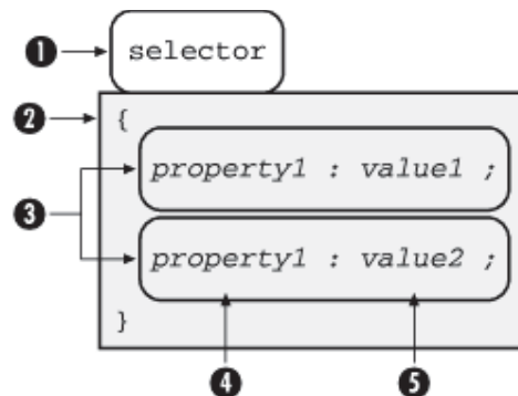
Figure 4.6, Syntax for a CSS rule
