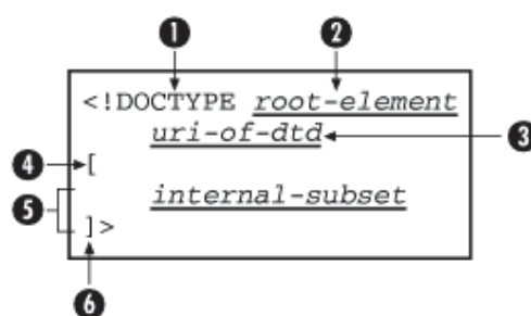
Figure 2.6, Document type declaration syntax
