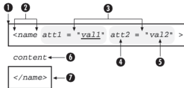
Figure 2.7, Container element syntax
