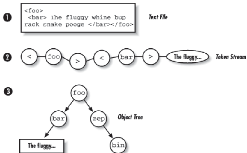
Figure 1.1, Three steps of parsing an XML document
