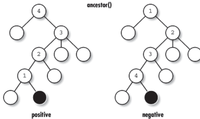
Figure 3.11, The path of ancestor()
