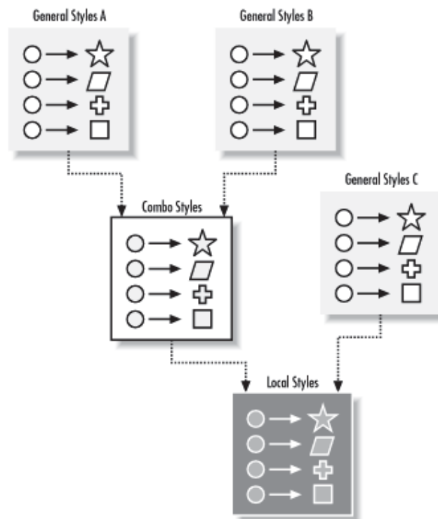
Figure 4.4, A cascade of stylesheets
