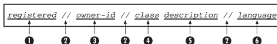
Figure 3.3, Formal public identifier syntax
