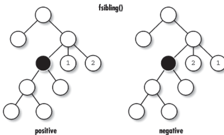
Figure 3.9, The path of fsibling()
