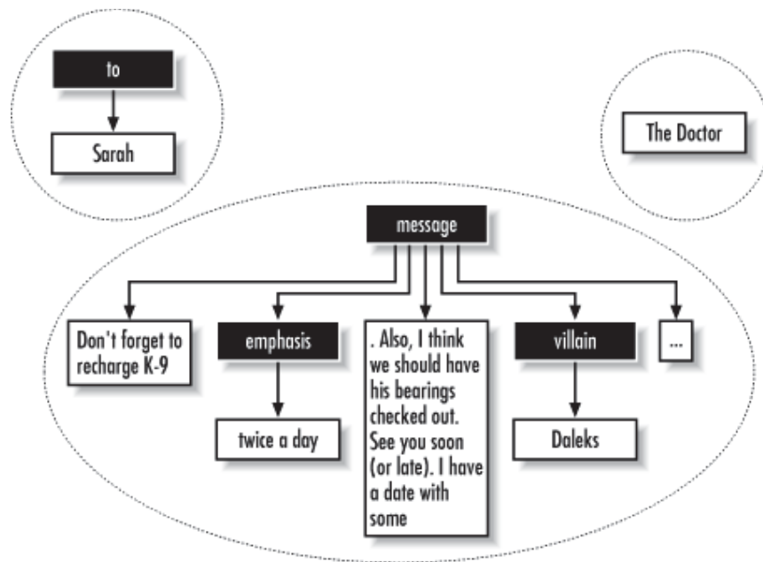
Figure 2.3, Some subtrees
