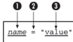
Figure 2.9, Attribute syntax
