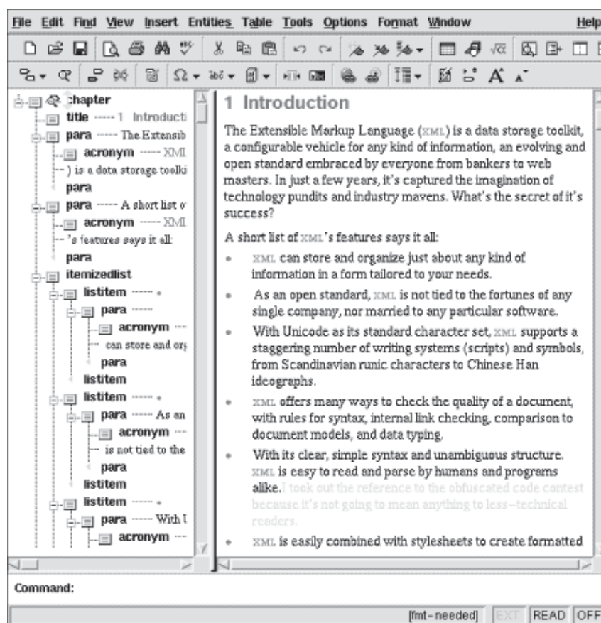
Figure 1.2, The Adept editor
