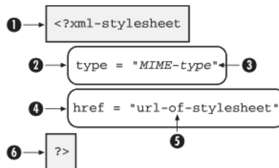
Figure 4.5, Syntax for a stylesheet declaration
