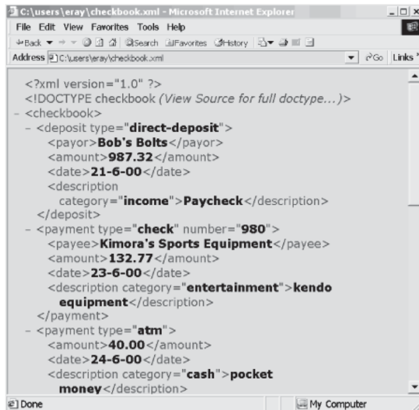
Figure 1.3, The outline view of Internet Explorer
