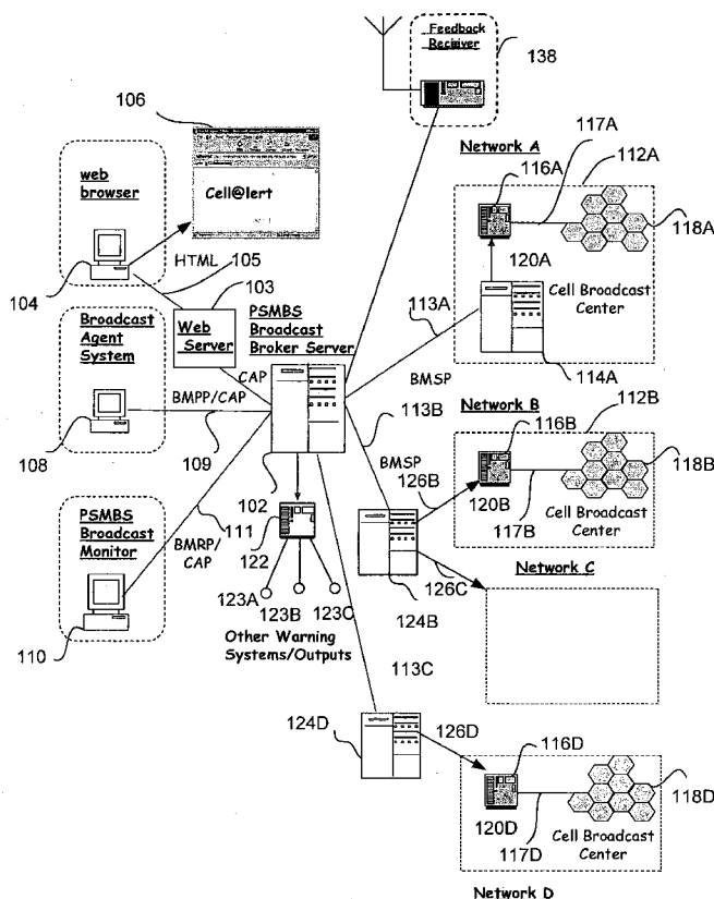
PSMBS System Components
