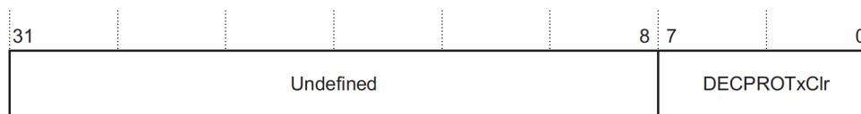
Figure 6 TZPCDECPROT0Clr Register bit assignments
