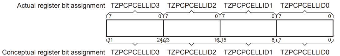
Figure 8 TZPC Identification Register bit assignments
