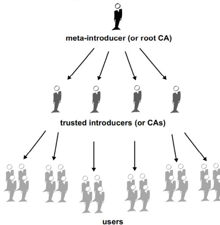
Figure 1-12. Hierarchical trust
