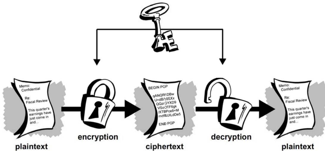
Figure 1-2. Conventional encryption
