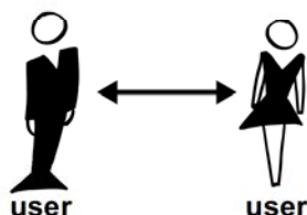
Figure 1-11. Direct trust
