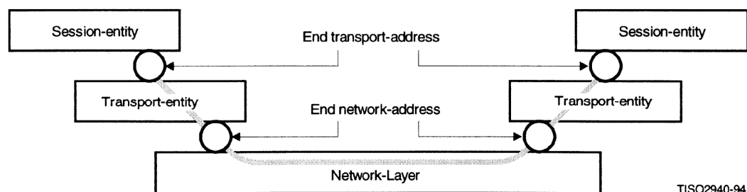
Figure 13 – Association of transport-addresses and network address
