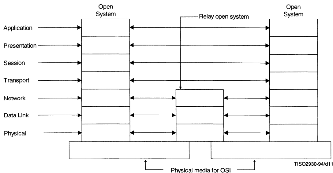
Figure 12 – Communication involving relay open systems
