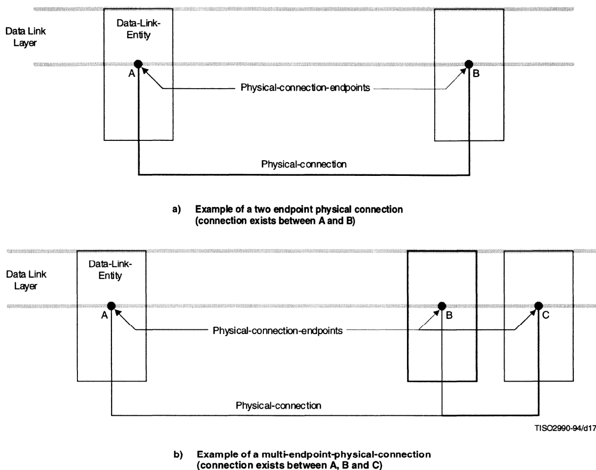
Figure 18 – Examples of physical connections
