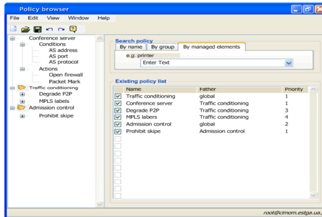
Figure 4 - Policy browser
