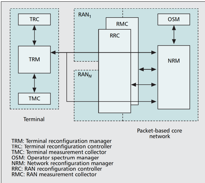
■ Figure 3. The P1900.4 system architecture.
