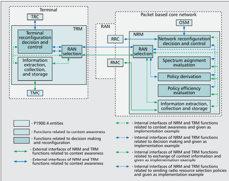
■ Figure 4. The P1900.4 functional architecture.
