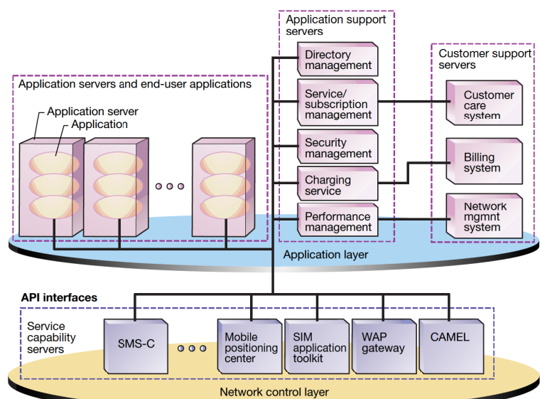
Figure 2 The structure of the application layer.
