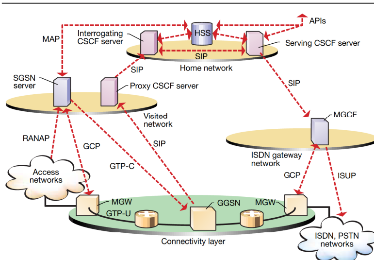
Figure 7 Example of a SIP call from a mobile terminal to the ISDN.
