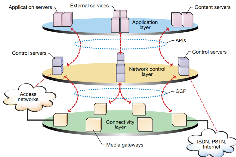
Figure 1 Horizontally layered network architecture.
