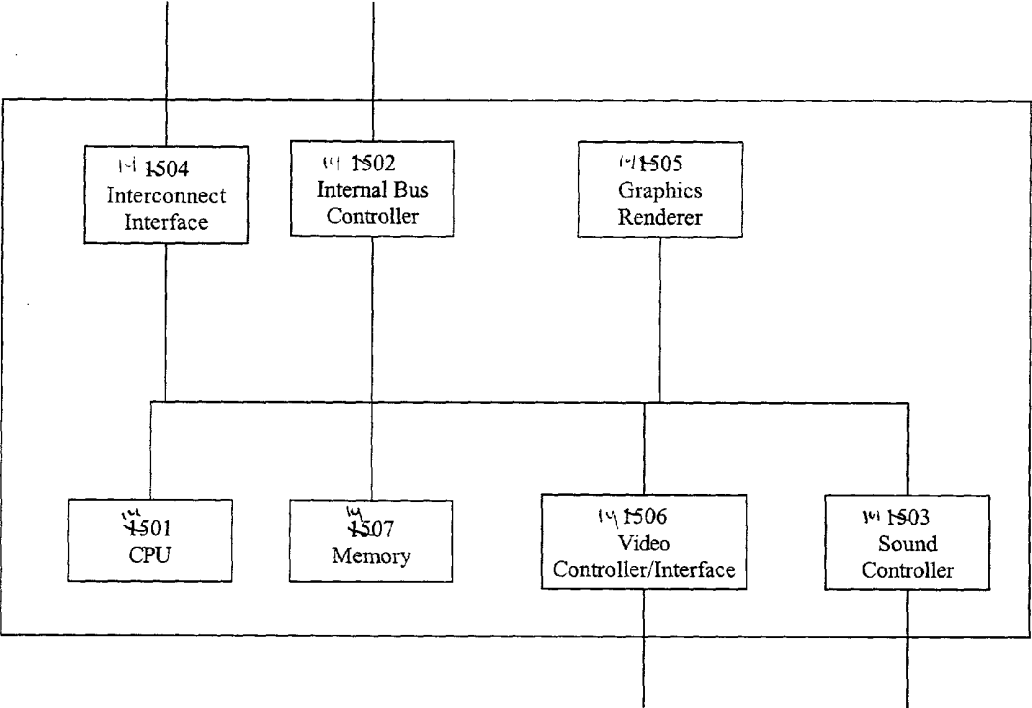
Figure 15: HID Single Chip Implementation
