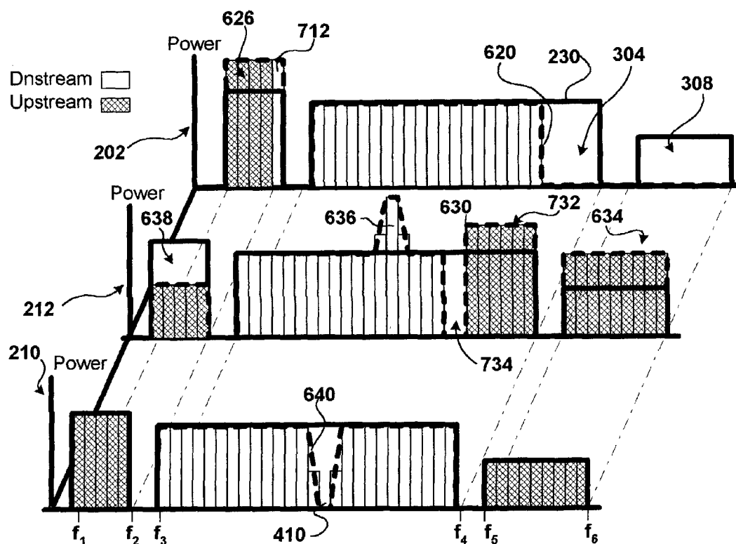
Alter PSD Masks and Bandplans
