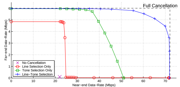
Fig. 3. Achievable Rate Regions of Different Algorithms ( c = 2 )
