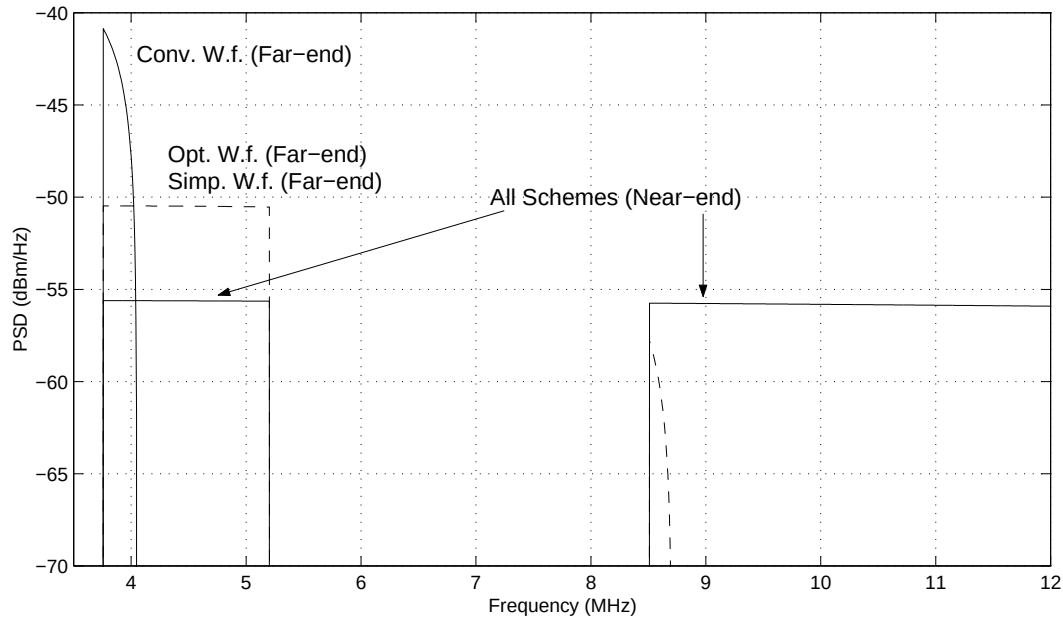
Fig. 1. PSDs of Different Power Allocation Schemes
