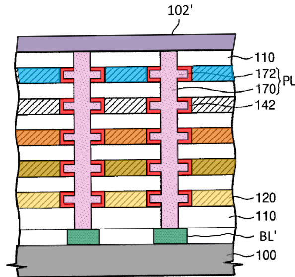
EX1003 — FIG. Z (Annotated and Modified FIG. 3 of Park)
