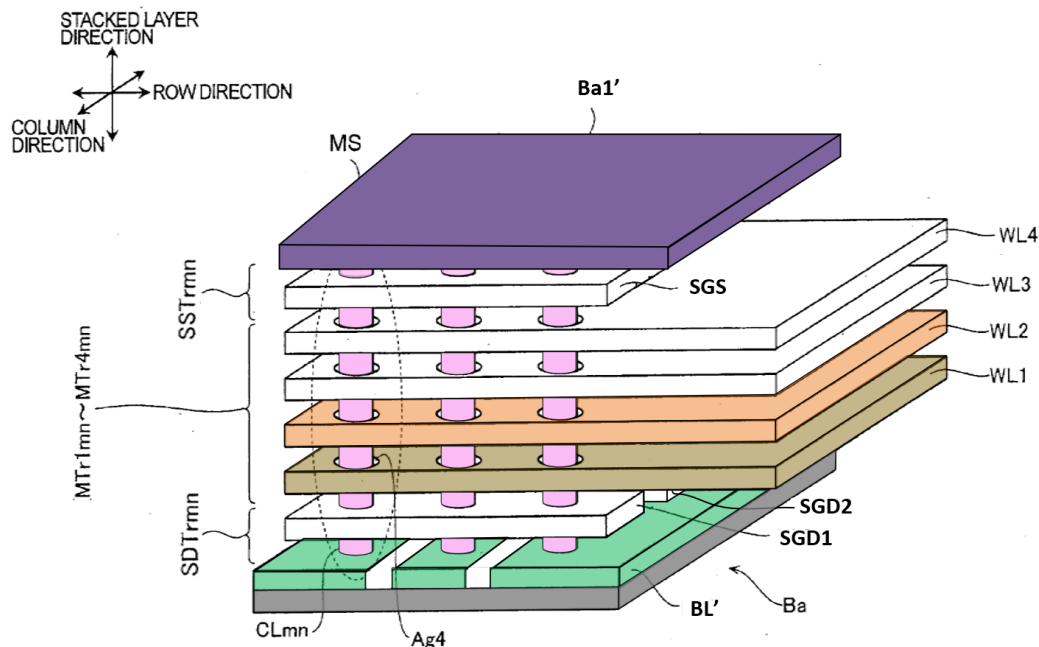
FIG. 2 EX1003 — FIG. AB (Annotated and Modified FIG. 2 of Fukuzumi)
