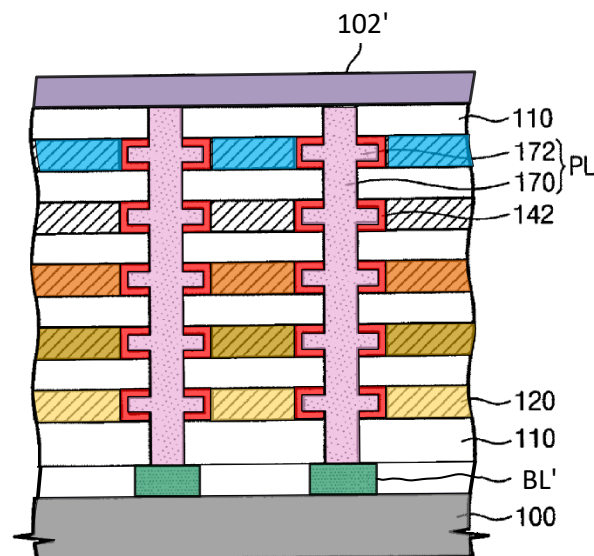
EX1003 — FIG. AA (Annotated and Modified FIG. 3 of Park)
