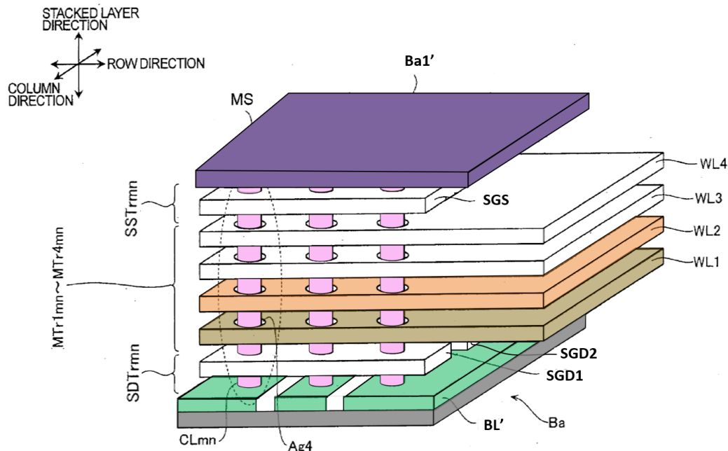
FIG. 2 EX1003 — FIG. AG (Annotated and Modified FIG. 2 of Fukuzumi)
