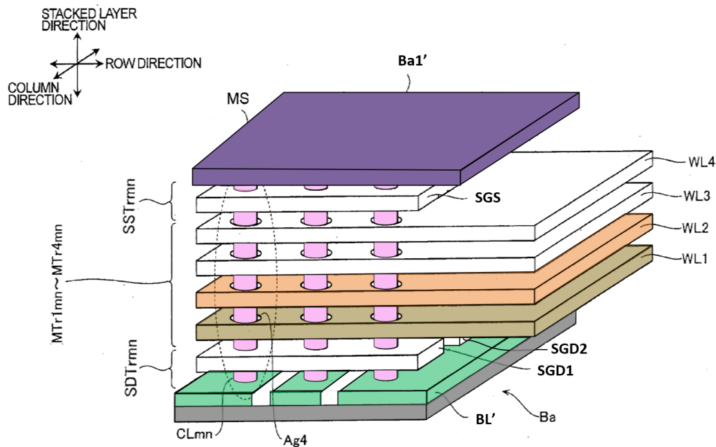
FIG. 2 EX1003 — FIG. AL (Annotated and Modified FIG. 2 of Fukuzumi)
