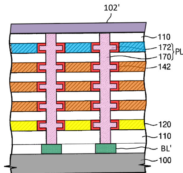
EX1003 — FIG. R (Annotated and Modified FIG. 3 of Park)
