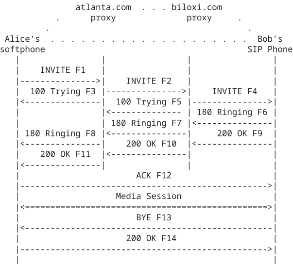
Figure 1: SIP session setup example with SIP trapezoid
