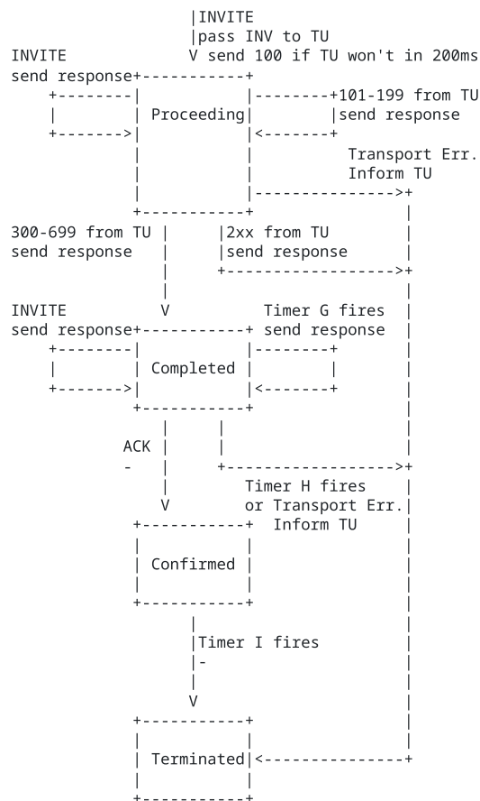
Figure 7: INVITE server transaction
