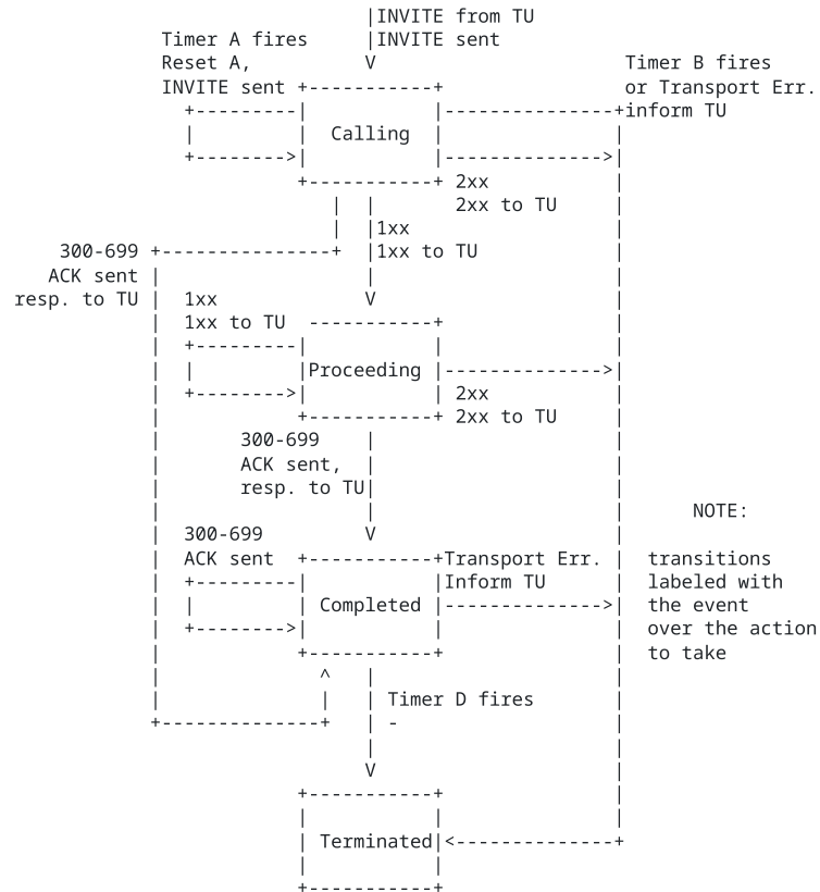
Figure 5: INVITE client transaction
