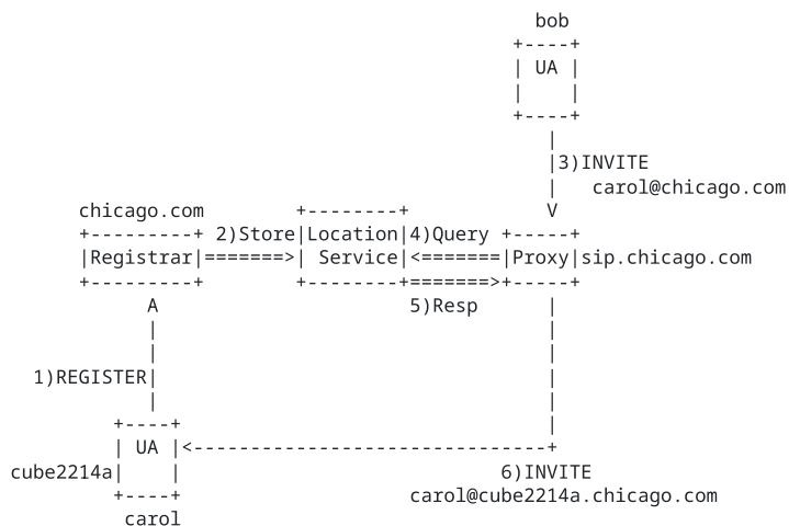
Figure 2: REGISTER example
