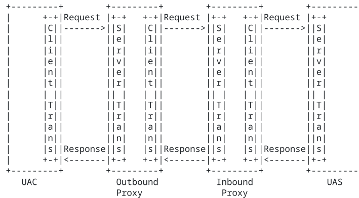
Figure 4: Transaction relationships
