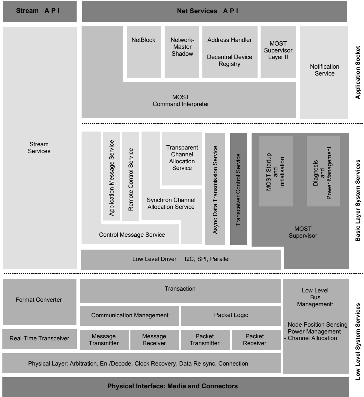
Block diagram of the MOST System Services
