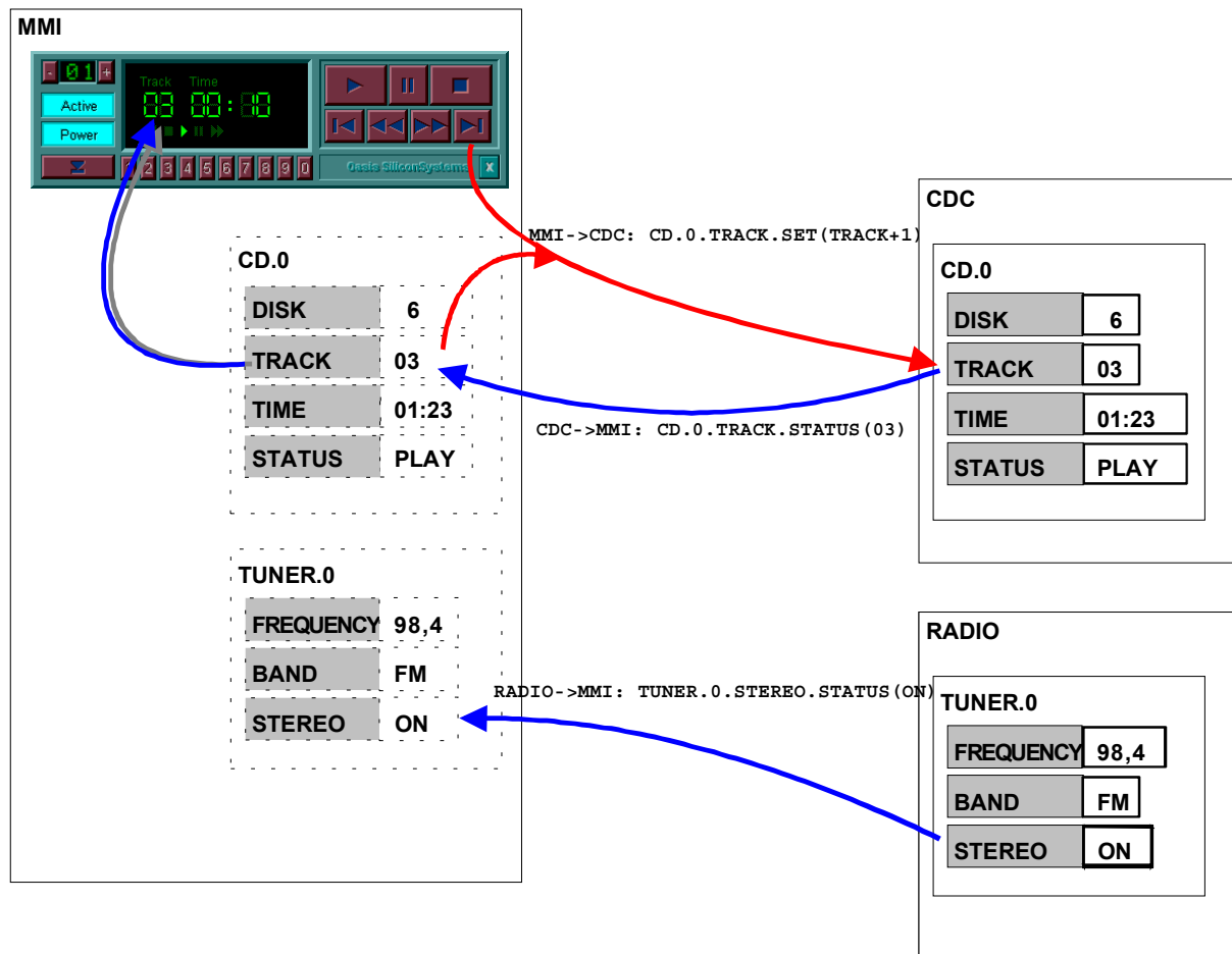
Figure 2-24: Controlling multiple devices.
