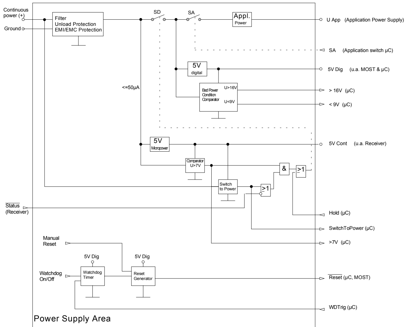
Figure 4-4: Block diagram of power supply area.
