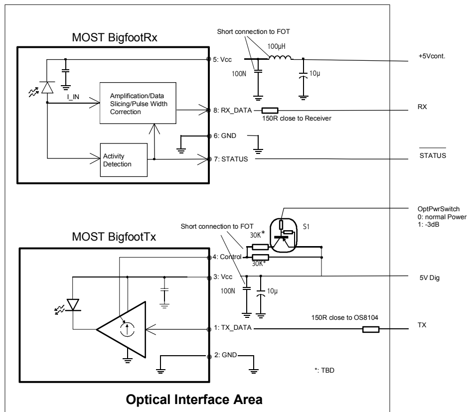
Figure 4-2: Optical interface area.
