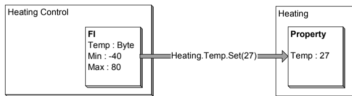
Figure 2-7: Example for a function interface (FI)
