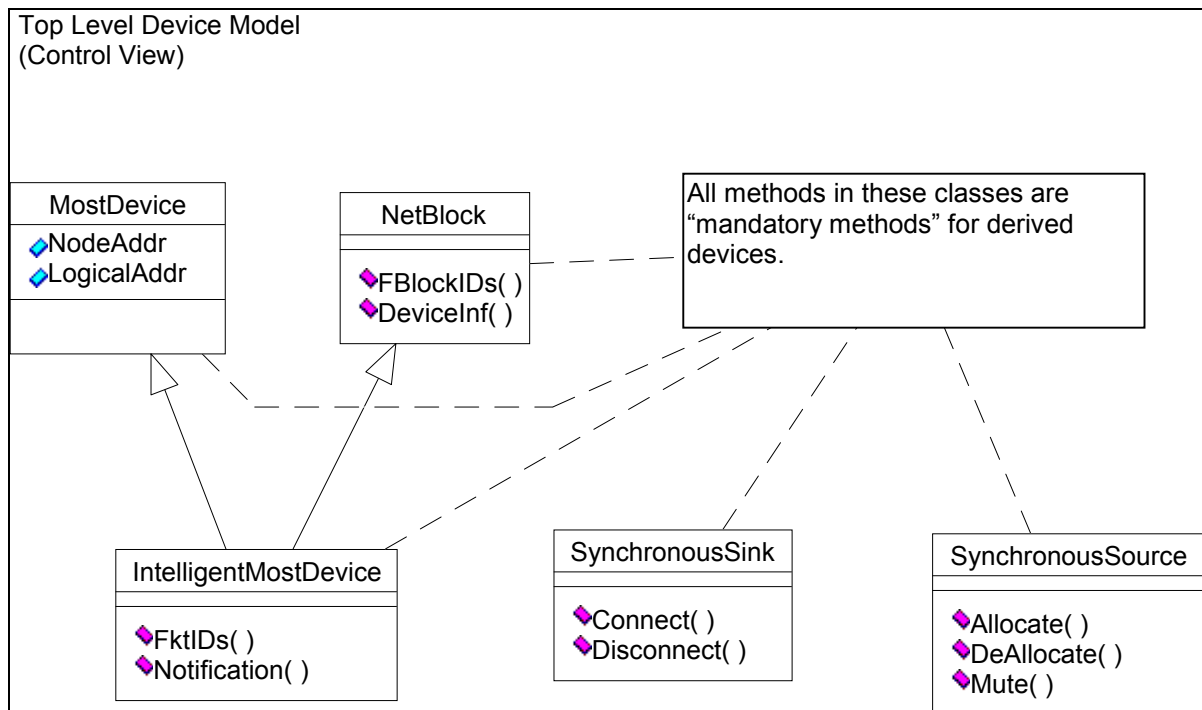
Figure 2-11: Highest layer of the device model
