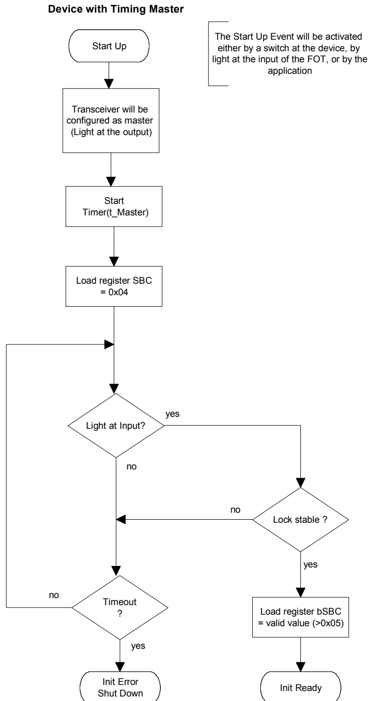
Figure 3-4: Behavior of a master device in state NetInterfaceInit .
