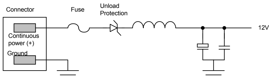
Figure 4-5: Input section of power supply area.
