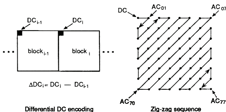
FIGURE 3. Preparation of Quantized Coefficients for Entropy Coding
