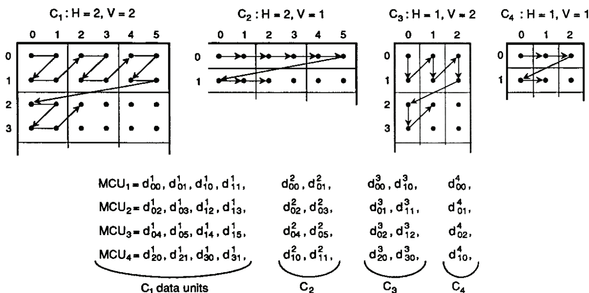
FIGURE 8. Generalized Interleaved Data Ordering Example
