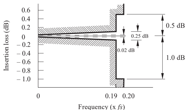
b) Passband ripple tolerance
