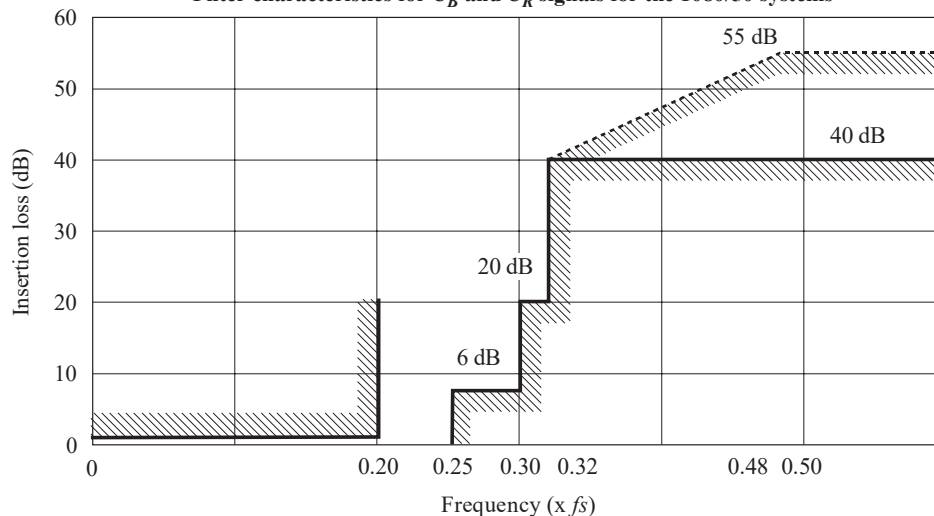
a) Template for insertion loss
