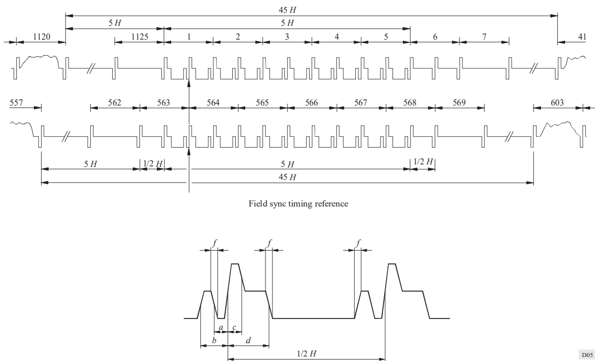
FIGURE 5 Field synchronizing signal waveform for the 1125/60/2:1 system
