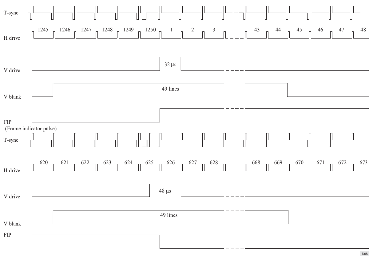
FIGURE 8 Timing of signals during the field-blanking interval for the 1250/50/2:1 system
