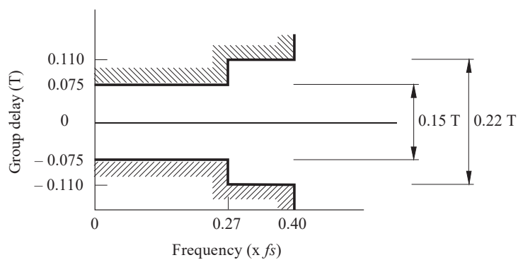
c) Passband group-delay
