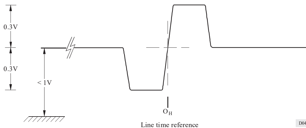
FIGURE 4 Line synchronizing signal waveform for the 1250/50/2:1 system
