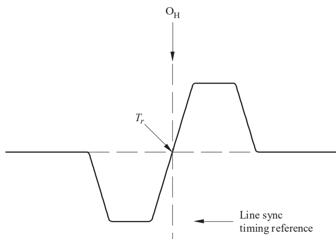
FIGURE 2 Form of synchronizing signal
