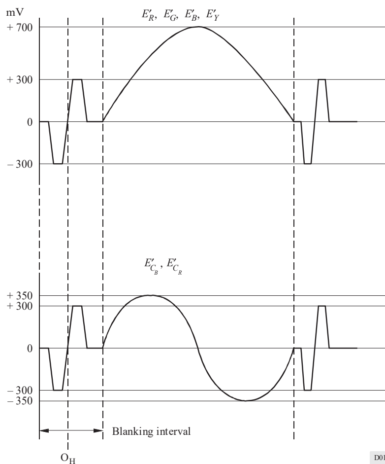
FIGURE 1 Sync level on component signals
