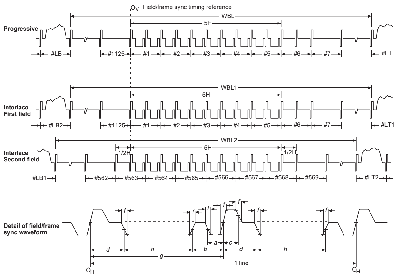
Field/frame synchronizing signal waveform for 1080/60(59) systems
