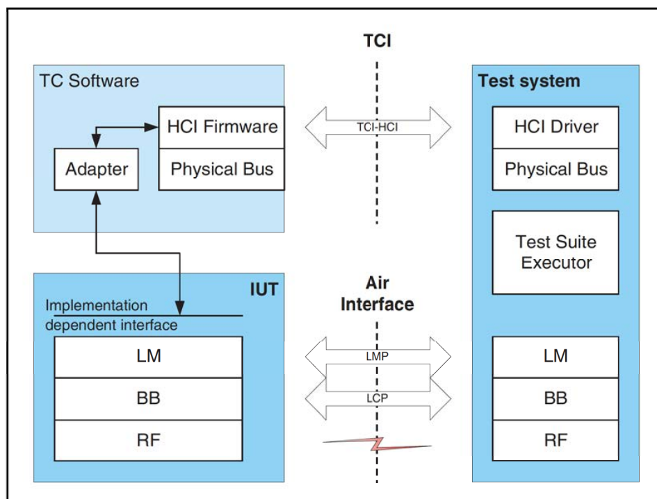
Figure 2.3: BB and LM qualification with TCI physical bearer
