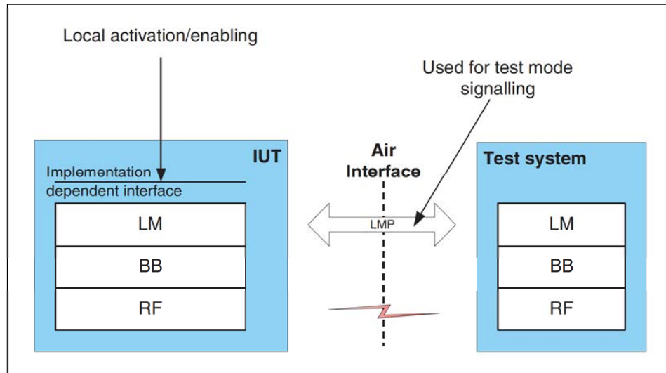
Figure 2.1: General test set-up for RF qualification
