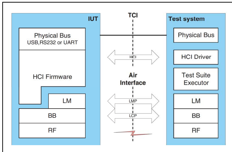
Figure 2.5: General test set-up for HCI qualification
