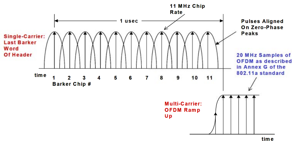
Figure 153Q—Single carrier to OFDM time alignment
