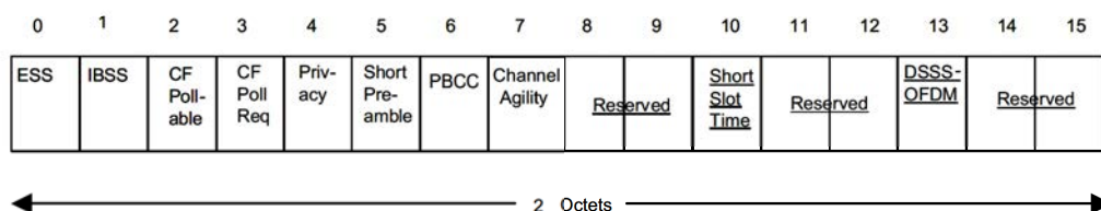
Figure 27—Capability Information fixed field
