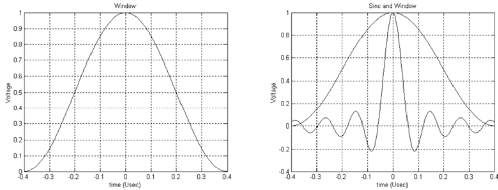
Figure 153L—The continuous time Hanning window
