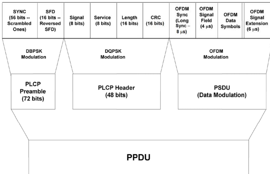
Figure 153B—Short preamble PDU format for DSSS-OFDM
