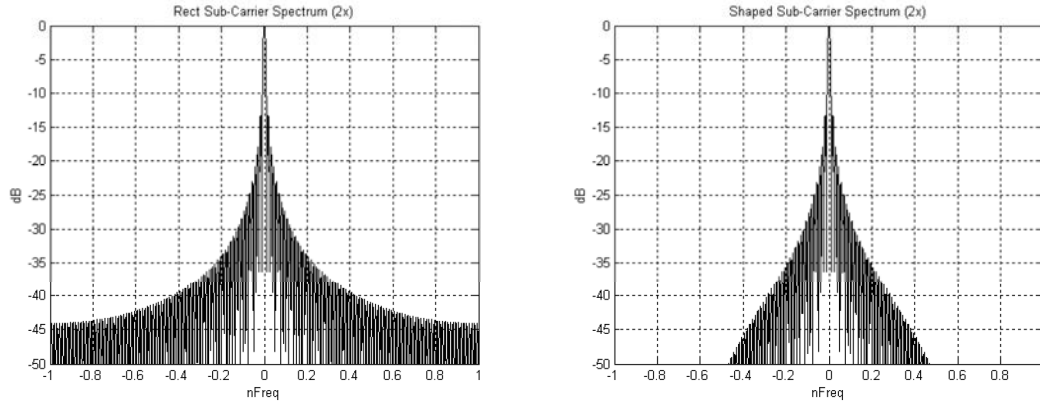
Figure 153J—Subcarrier spectrums for rectangular windowing and Clause 17 suggested windowing
