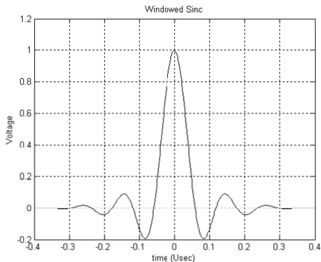
Figure 153M—The specified pulse
