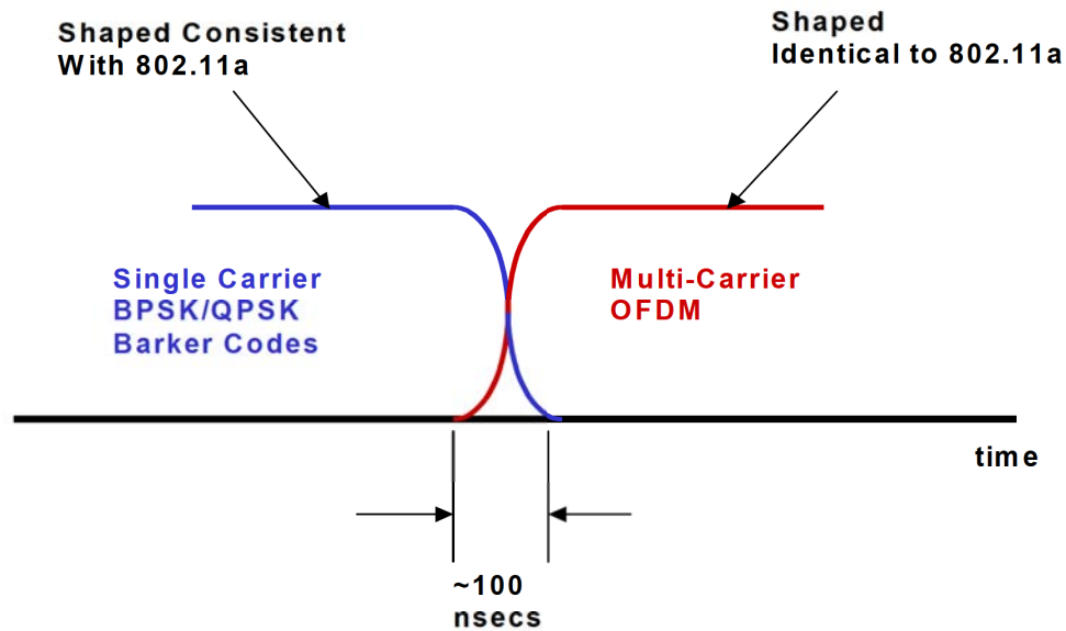
Figure 153R—Single carrier termination requirement
