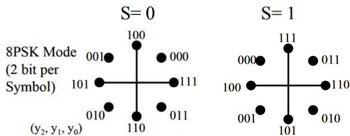
Figure 153D—ERP-PBCC-22 and ERP-PBCC-33 cover code mapping
