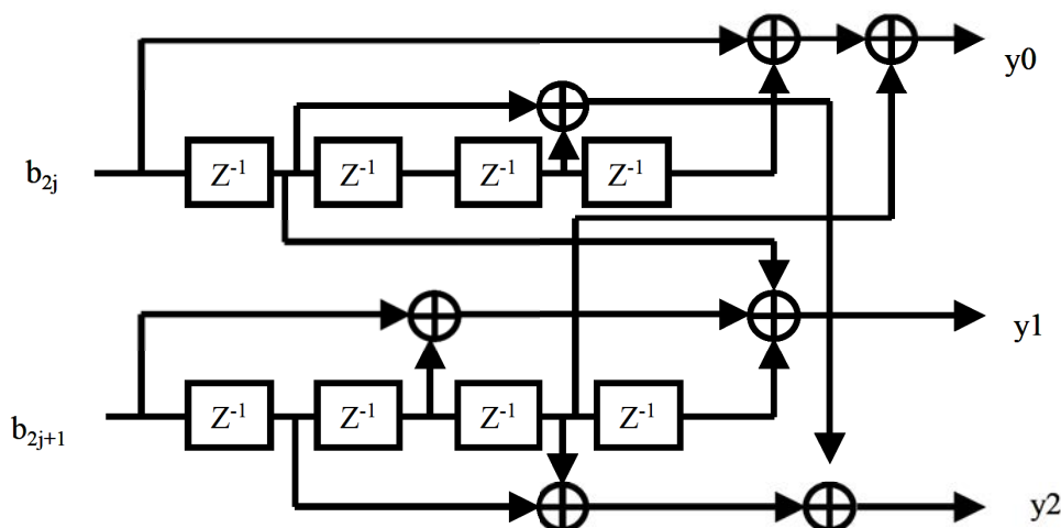
Figure 153C—22/33 Mbit/s ERP-PBCC convolutional encoder
