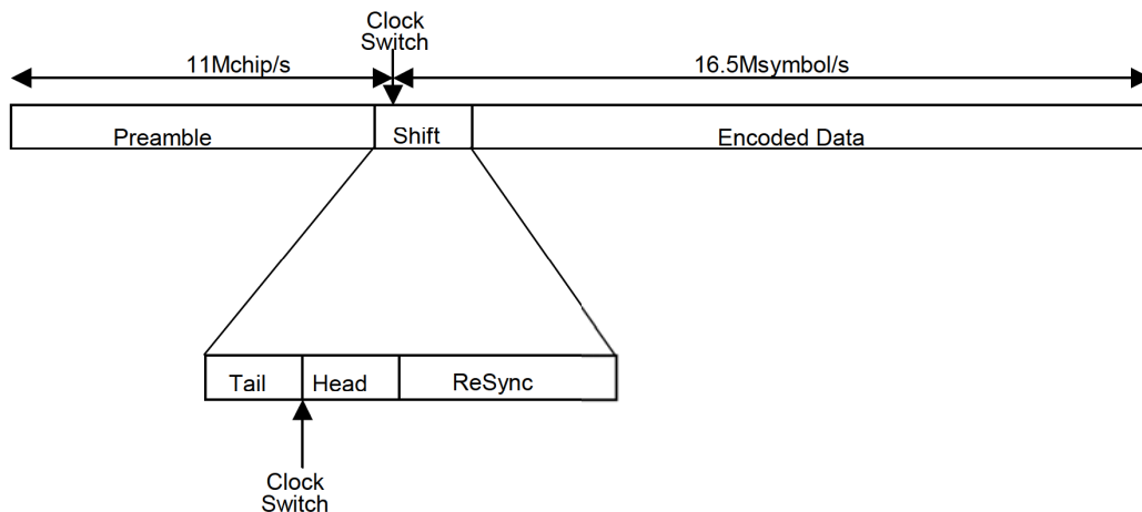
Figure 153E—33 Mbit/s clock switching
