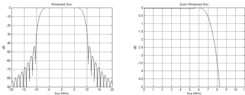
Figure 153N—The single carrier frequency response
