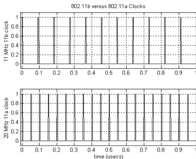
Figure 153P—Aligning the 11 MHz and 20 MHz clocks
