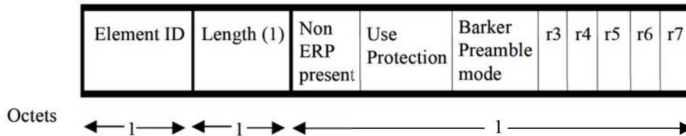
Figure 42E—ERP Information element
