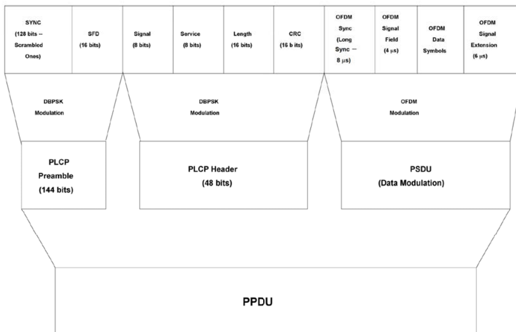
Figure 153A—Long preamble PPDU format for DSSS-OFDM
