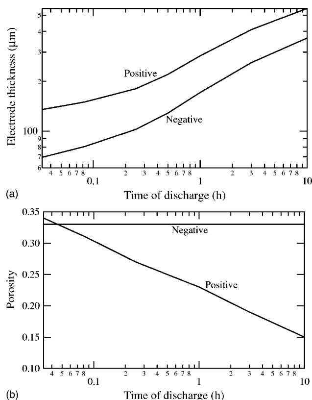
Figure 9. Optimized thickness and porosity corresponding to the envelope plot in Fig. 8. A cell fabricated with the design shown here would yield the maximum specific energy at that discharge time. The optimization was performed for the positive electrode thickness and porosity. The excess capacity ratio of the anode to cathode was held constant at 10% while the negative-electrode porosity was held constant at 0.33, and hence the negative-electrode thickness changes corresponding to the change in design of the positive electrode.
