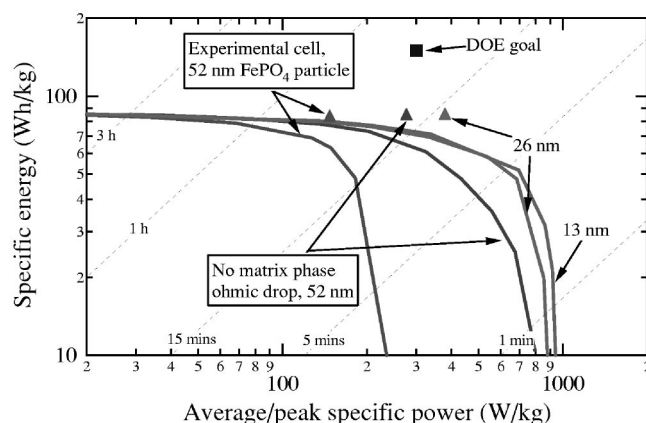
Figure 4. Simulated Ragone plot of the NG/LiFePO 4 cell for various designs. The lines represent the average specific power of the cell ( i.e. , specific energy divided by the discharge time) while the symbols represent the specific energy evaluated from a 3 h discharge and the peak specific power defined at 80% DOD for a 30 s pulse. The DOE technology assessment minimum goal for long-term commercialization is also shown.
