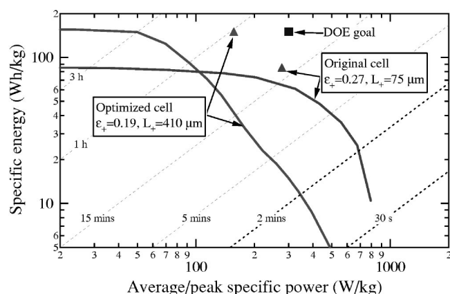
Figure 7. Comparison of the performance of the cell using the base-case design from Table I and the optimized design from Fig. 6 for a 3 h discharge. The plot shows a Ragone plot with both the average power and the peak power defined at 80% DOD for a 30 s pulse.
