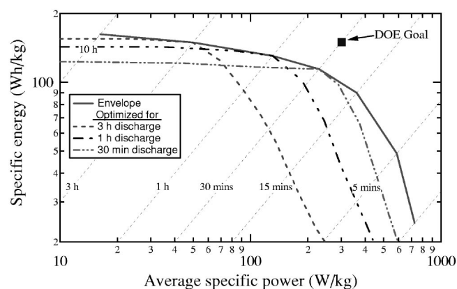
Figure 8. Ragone plot of the NG/LiFePO 4 cell with various optimized designs. The solid line is the envelope curve where every point is optimized for the corresponding discharge time. The design is shown in Fig. 9, and the optimum current in Fig. 10. The plot also shows the performance of three cells which are designed for one discharge time and used under other conditions. Compare with Fig. 10 in Ref. 4.
