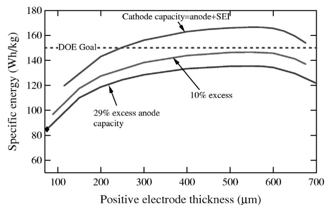
Figure 5. Illustration of the optimum in the positive electrode thickness for maximizing the specific energy for a constant porosity of 0.27 for the positive electrode. The plot also shows the effect of the anode-to-cathode capacity ratio. The DOE goal is shown for comparison. Each point is generated by finding the optimum current such that the cell discharges to 2.5 V in 3 h. Note that the negative electrode thickness is changed correspondingly. The symbol \blacklozenge represents the value taken from Fig. 4.
