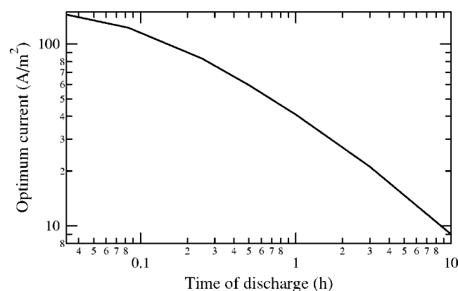
Figure 10. Optimized current density corresponding to the envelope curve in Fig. 8. The current density can be used to decide the area required to satisfy a specified load requirement.
