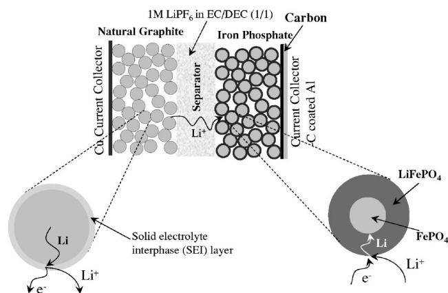
Figure 1. Schematic of the cell modeled in this study consisting of a natural graphite negative and an iron phosphate positive electrode with a separator between them. The whole cell is filled with 1 M \text{LiPF}_6 in EC/DEC (1:1). The processes on discharge are illustrated in the figure. Lithium transport via a diffusion mechanism and ohmic losses through the SEI are described for the negative electrode. The transport of lithium through the shell and the movement of the phase interface are described for the positive electrode.
