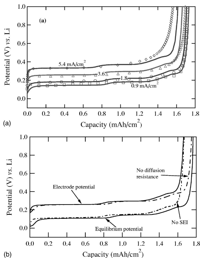
Figure 2. Model-experimental comparisons of the graphite half-cell at various currents (a) and the corresponding potential drops in the electrode at a current of 3.6 \text{ mA/cm}^2 (b). The SEI layer resistance is used as a fitting parameter in the figures, while the rest of the parameters are taken from the literature. Figure 3b shows the decomposition of the electrode potential curve by plotting the equilibrium potential, the electrode potential with no SEI layer and the electrode potential with no diffusion resistance.
