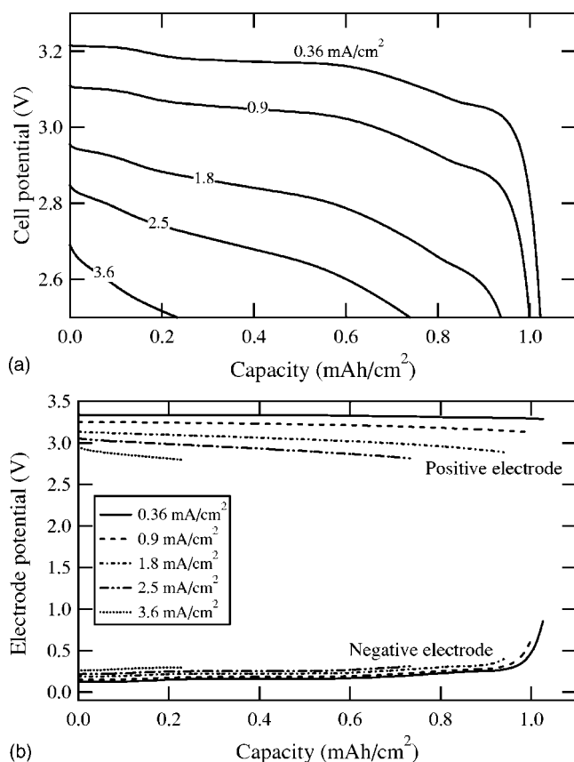
Figure 3. Simulated cell potential (a) and individual electrode potentials (b) at different current densities during discharge of a NG/LiFePO 4 cell. The curves were generated using the base-case parameters in Table I. The electrode potentials were generated by plotting the potential of the matrix at the current collector minus the potential of the solution at the midpoint of the separator. Note the significant drops in the potential of the positive electrode.
