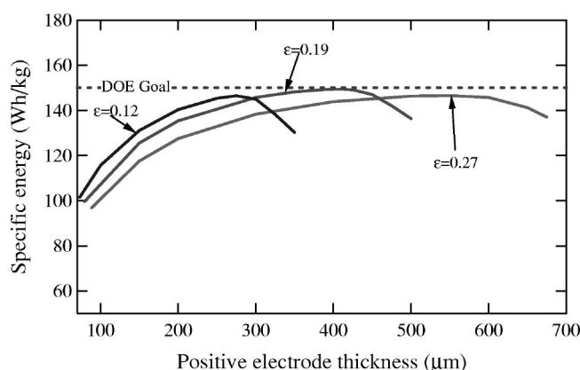
Figure 6. Illustration of the effect of porosity on the optimum thickness with the anode-to-cathode capacity ratio fixed at 10%. The curve at a porosity of 0.27 is same as that in Fig. 5. Each point is generated by finding the optimum current such that the cell discharges to 2.5 V in 3 h. Note that the negative electrode thickness is changed correspondingly. The optimum design occurs at \epsilon_+ = 0.19 and L_+ = 410 \mu\text{m} .
