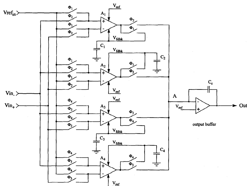
Fig. 1. Block diagram of the rail-to-rail ping-pong op-amp.
