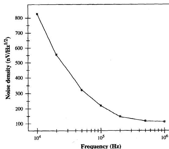
Fig. 8. Input referred noise floor versus clock frequency.
