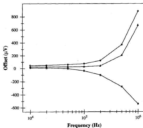
Fig. 7. Offset dependence on the clock frequency.
