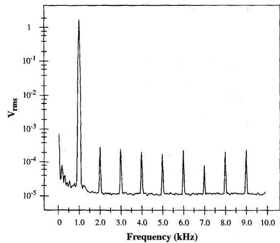
Fig. 10. Output spectrum for a 4.9 V_{pp}/1 \text{ kHz} sine input.
