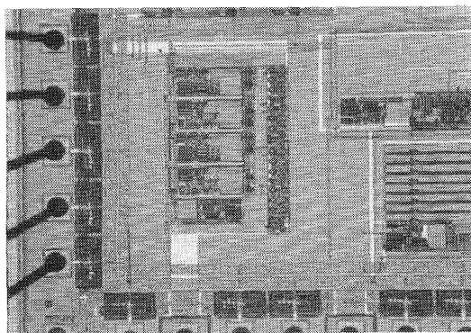
Fig. 6. Photomicrograph of the ping-pong op-amp.
