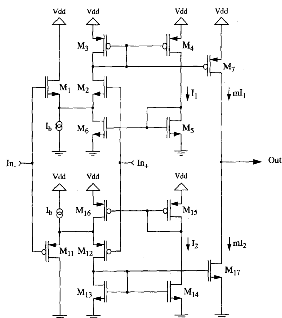
Fig. 5. Schematic diagram of the output buffer.
