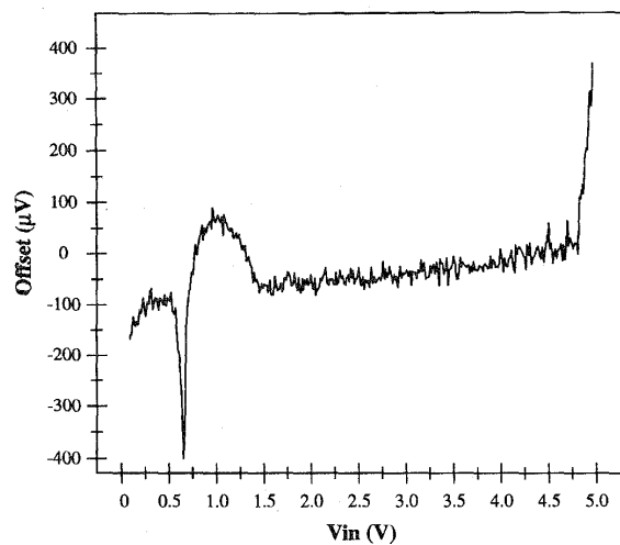
Fig. 9. Offset dependence on the input common mode voltage.
