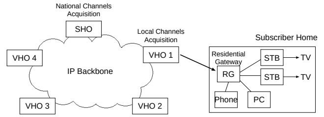
Figure 1: IPTV Architecture
