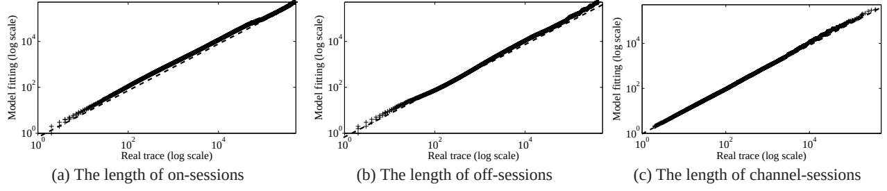
Figure 8: QQ plots comparing models and real traces
