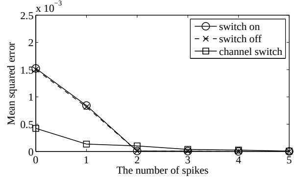
Figure 11: Find the optimal number of spikes
