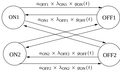
Figure 13: ON-OFF model
