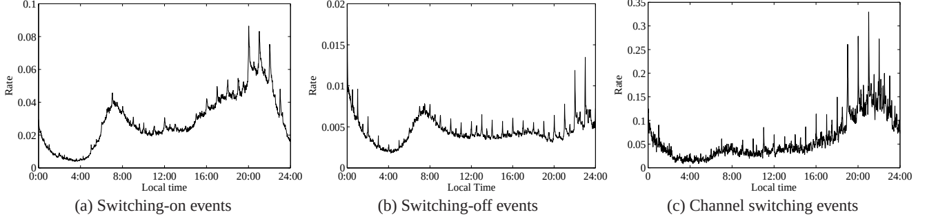
Figure 4: The normalized switching-on, switching-off, and channel switching events (one-minute granularity)
