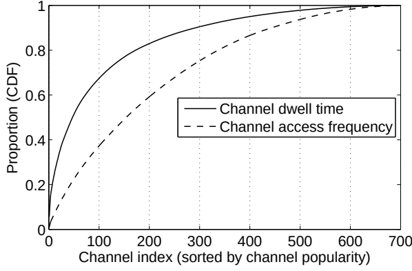
Figure 5: CDF of channels popularity
