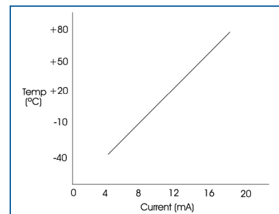
Figure 3 Calibration curve for a scaled transmitter.
