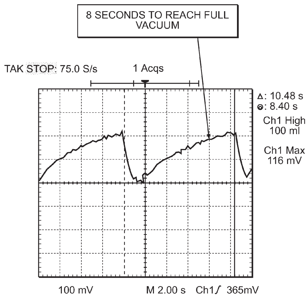
FIG. 23 PRIOR ART
