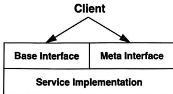
Figure 5 Meta-Object Protocol
