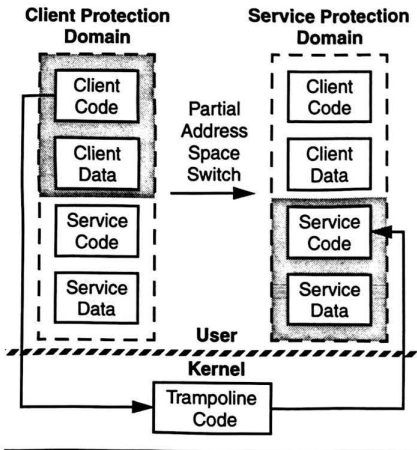
Figure 1 Protected Library
