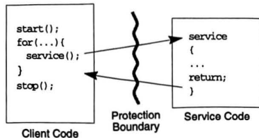
Figure 8 Client/Service Relationship
