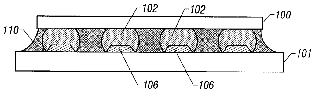
FIG. 9 (Prior Art)
