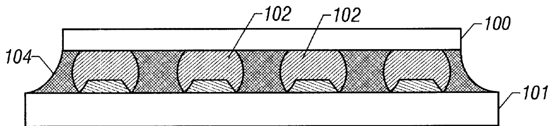
FIG. 4 (Prior Art)
