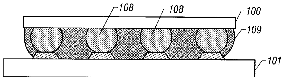
FIG. 8 (Prior Art)
