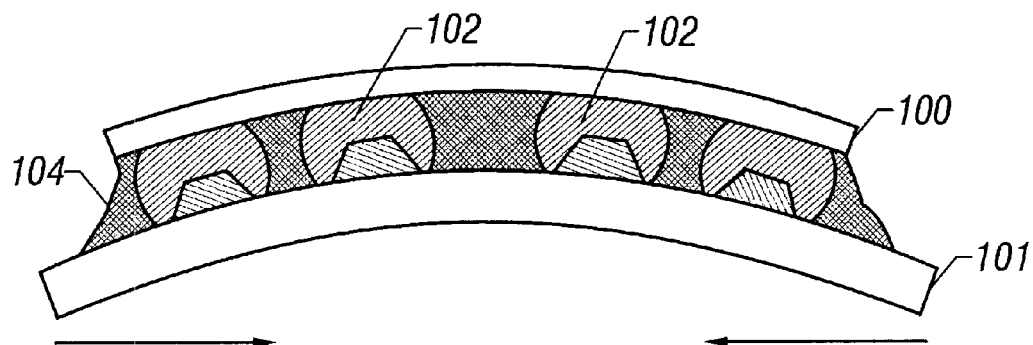
FIG. 6 (Prior Art)
