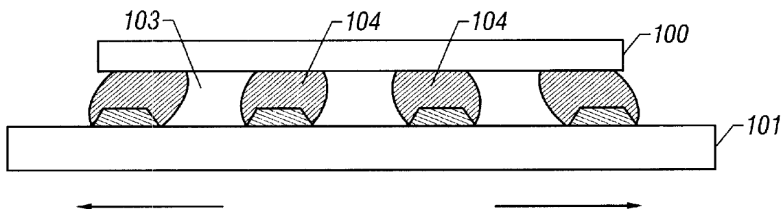
FIG. 2 (Prior Art)
