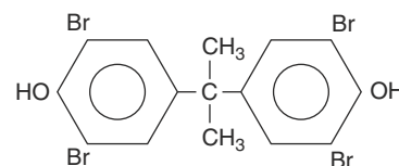
FIGURE 7.2 Tetrabromobisphenol-A (TBBPA).
