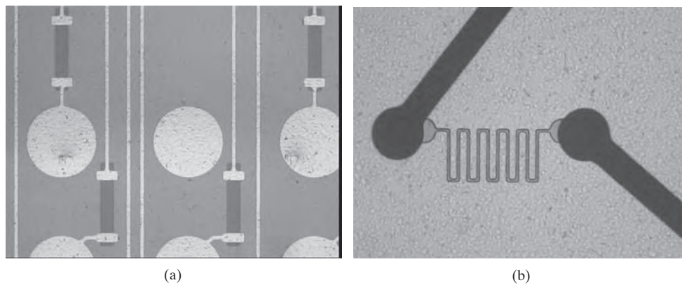
FIGURE 66.15 “Examples of functional flexible circuits (a): Embedded resistance (b): Small strain gage built on flexible substrate.” (Source: MicroConnex ).
