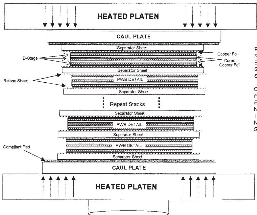
FIGURE 27.34 Typical ML-PWB stack-up for hydraulic lamination.
