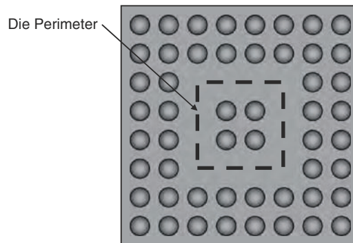
FIGURE 58.28 Depopulated array with no joints under the perimeter of the die. Solder ball locations are indicated by the array of circles. The die perimeter is indicated by the dashed rectangular outline. Note that the die edge falls in an area of depopulated solder balls.
