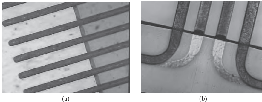
FIGURE 66.2 Typical fine flying leads construction (a) Single side, (b) Double side.
