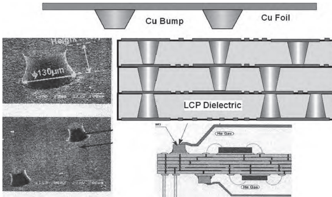
FIGURE 23.33 The Neo-Manhattan Bump Interconnect structure.
