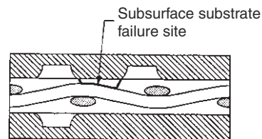
FIGURE 56.3 Subsurface substrate failure. 2 © 1976 IEEE
