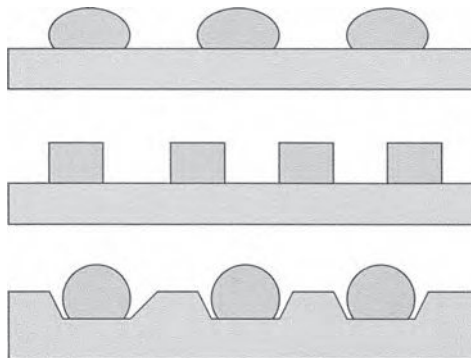
FIGURE 66.11 Microbump arrays on flexible circuits: examples of bump shapes.
