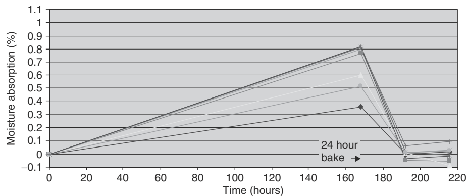
FIGURE 10.13 Percent weight change after seven days at 35°C/85 percent RH moisture test and 125°C bake.
