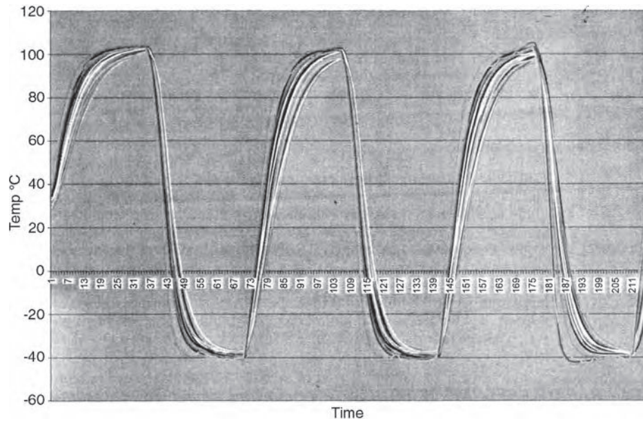
FIGURE 59.3 Typical thermal cycle profile. In this plot, T_{max} = 100^{\circ}\text{C} , T_{min} = -40^{\circ}\text{C} , and the cyclic frequency is 60 min.
