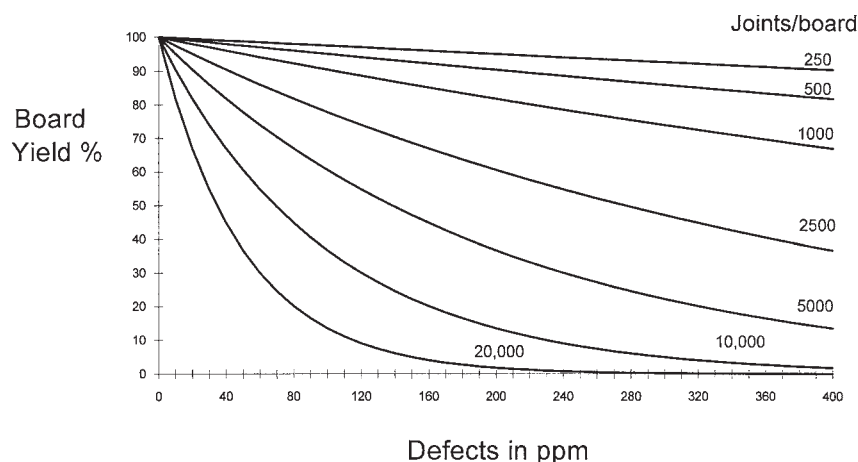
FIGURE 53.2 Printed circuit board yield decreases dramatically with increases in the number of solder joints per assembly if the defect rate per solder joint remains constant. For instance, at a 40 defects per million opportunities (DPMO) defect rate, the yield drops from 96 percent at 1,000 joints per assembly to 45 percent at 20,000 joints.
