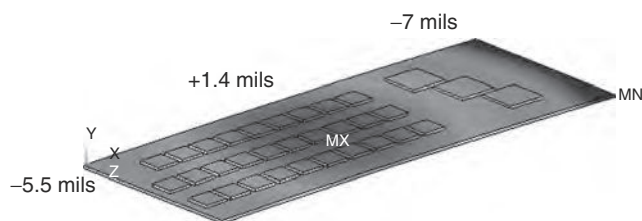
FIGURE 58.12 High-density placement of BGAs on top side of a PWB. This diagram illustrates the convex-type curvature of a PWB assembly where multiple BGA devices are all placed on one side of a board.
