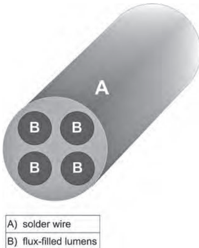
FIGURE 46.1 Solder wire for hand-soldering showing flux-filled lumens.
