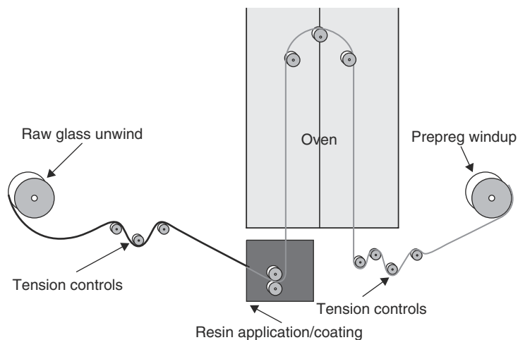
FIGURE 6.8 "Treating" fiberglass cloth with resin.
