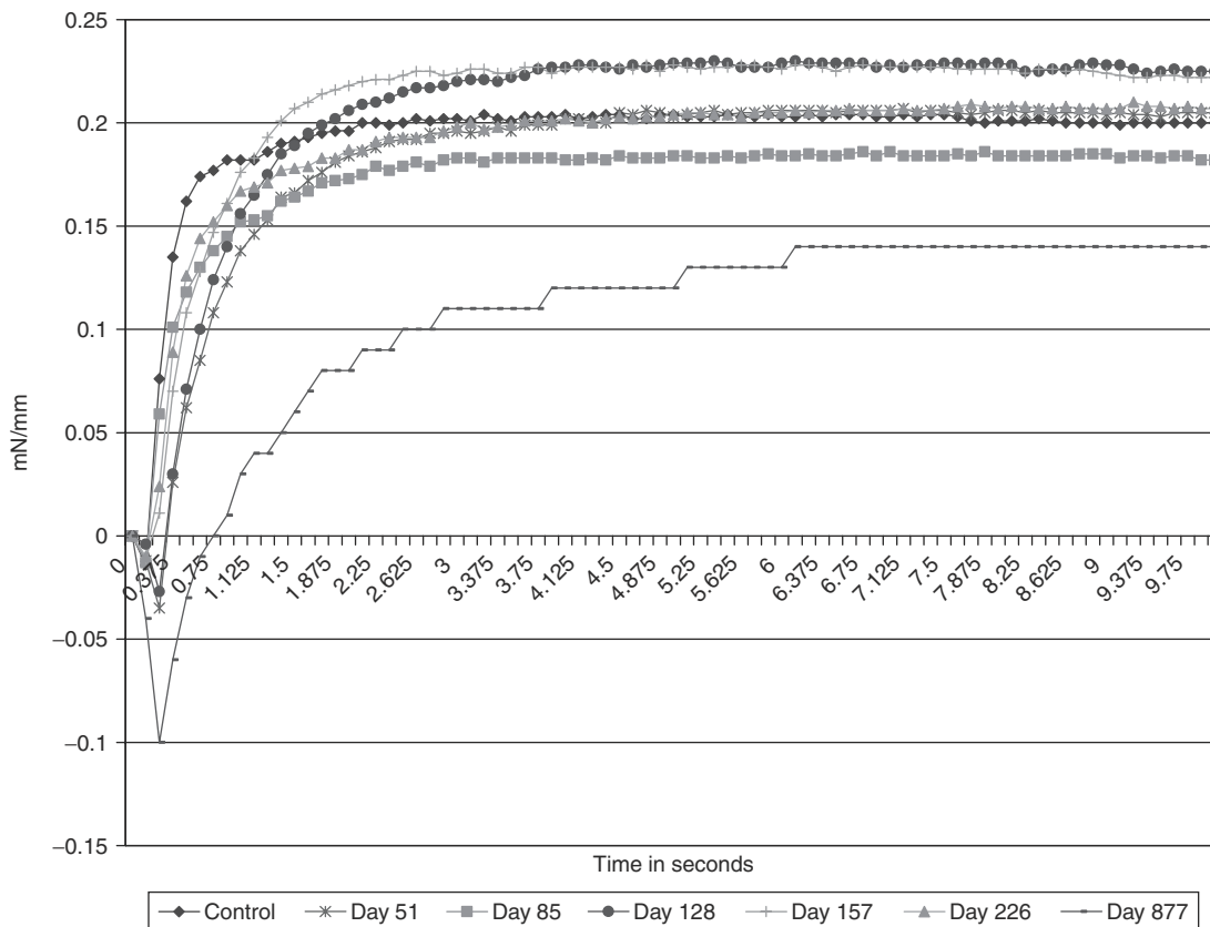
FIGURE 42.14 A gradual reduction of wetting forces as a function of copper migration through the Direct Immersion Gold (DIG) deposit after 877 days in storage.
