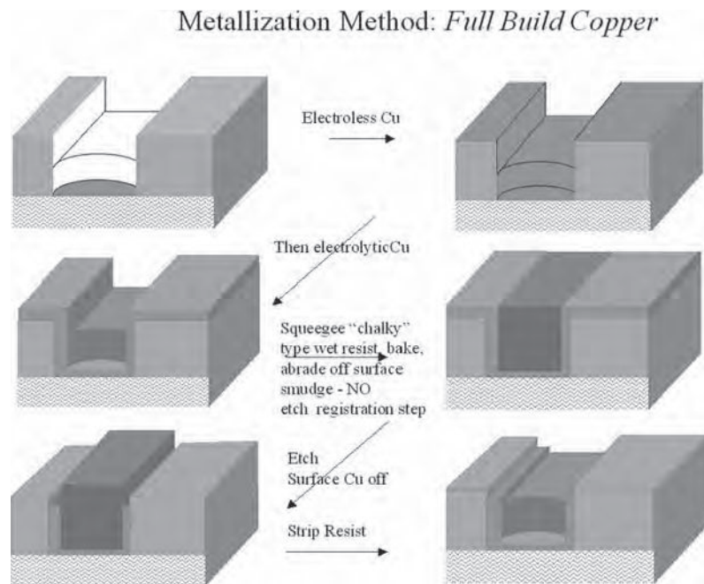
FIGURE 23.40 Methods of metallization using electroless plating, plugging, and etching. (Courtesy of Dimensional Circuits.)
