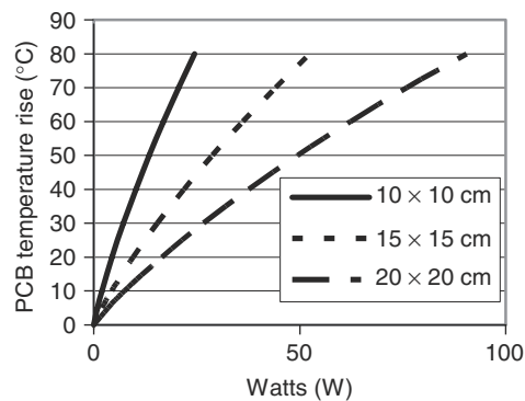
FIGURE 17.9 Temperature rise above 25^\circ\text{C} of a horizontal PCB in natural convection as a function of PCB size and power dissipation. Both convection and radiation are dissipating the power.
