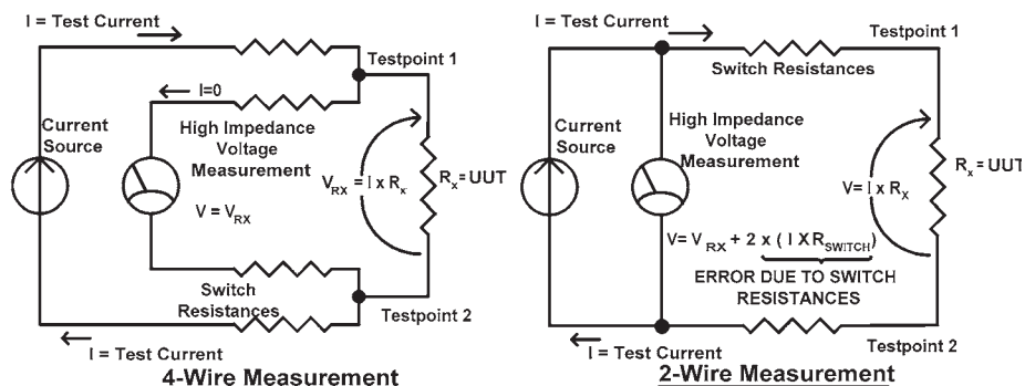
FIGURE 37.3 Continuity measurement circuits.
