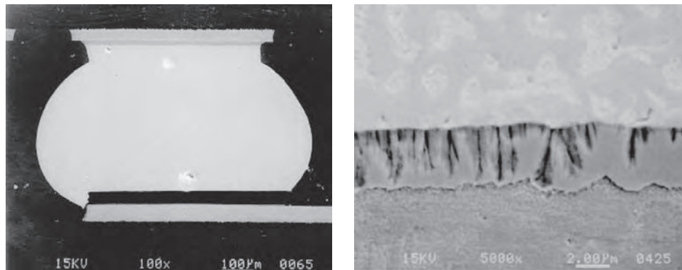
FIGURE 32.7 The result of black-pad and the microstructure of a black-pad nickel interface.
