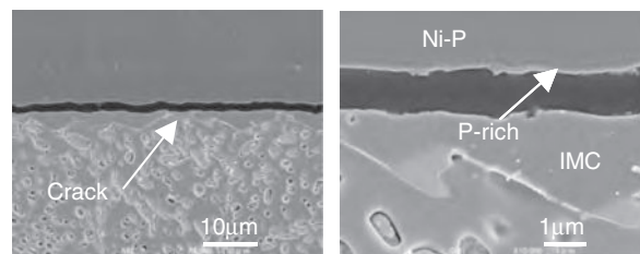
FIGURE 58.19 Brittle Solder Joint Failure. 19 A clear separation between the P-rich phase and IMC on the package side is shown. (Reprinted with permission from Renesas Technology Corp./© [2003] IEEE ECTC.)
