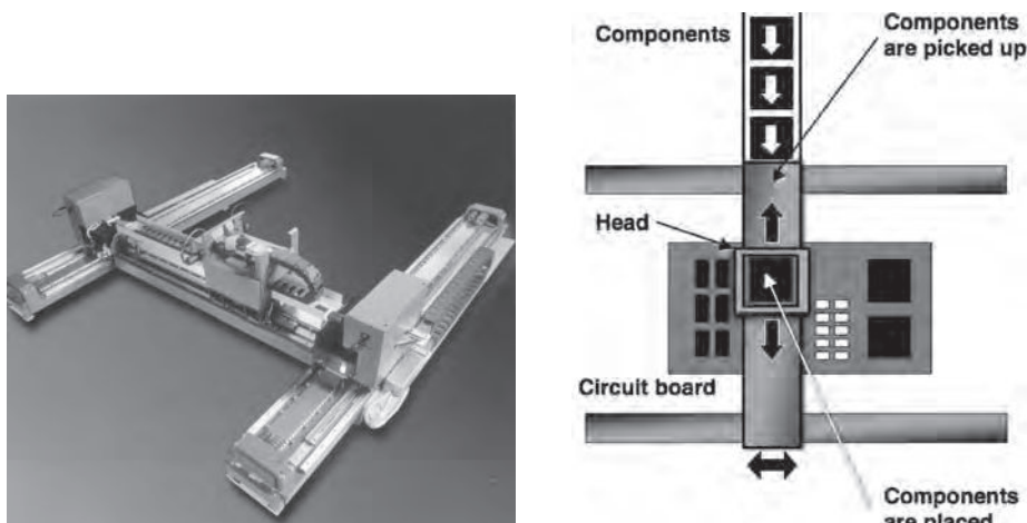
FIGURE 40.21 Gantry architecture used for placing larger components such as SOICs, PLCCs, and area-array packages. (Photo courtesy of Universal Instruments.)
