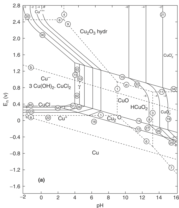
FIGURE 56.7 Pourbaix diagram of the copper-chlorine-water system.
