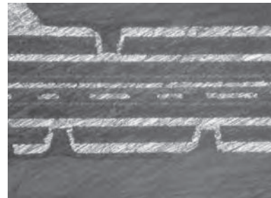
FIGURE 65.13 Micro blind vias on two sides of a multilayer rigid/flexible circuit.
