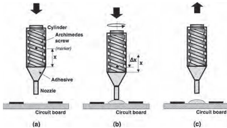
FIGURE 40.18 Archimedes screw pump dispensing technique: (a) The dispenser is lowered to above the circuit board surface; (b) the Archimedes screw is turned a set rotation ( \Delta x ), pushing adhesive out of the nozzle; (c) the dispenser is lifted from the circuit board.
