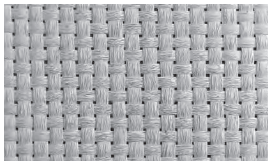
(b) 2116 Cloth
