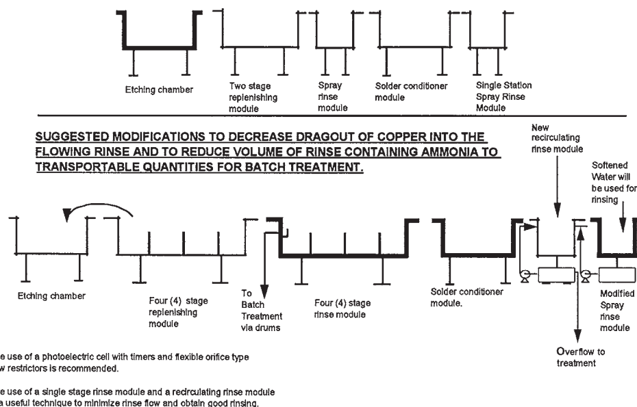
FIGURE 60.3 Suggested modifications to inner/outerlayer etching equipment.
