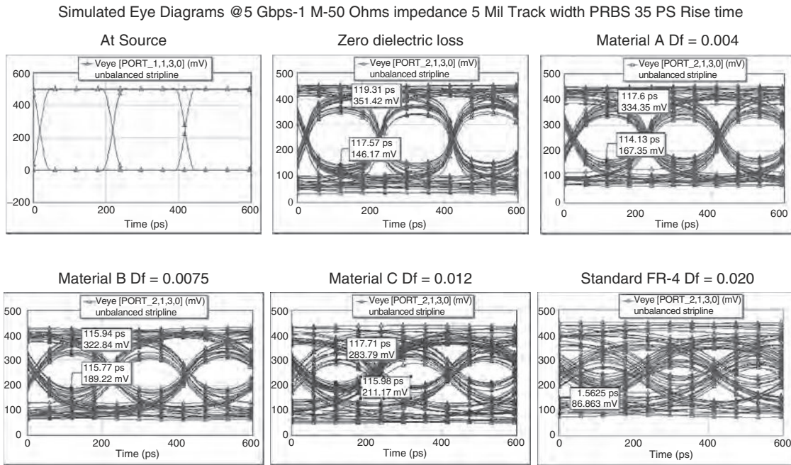
FIGURE 9.24 Simulated eye diagrams at 5 Gbps, 1 M, 50 ohms impedance, 5 mil track width.
