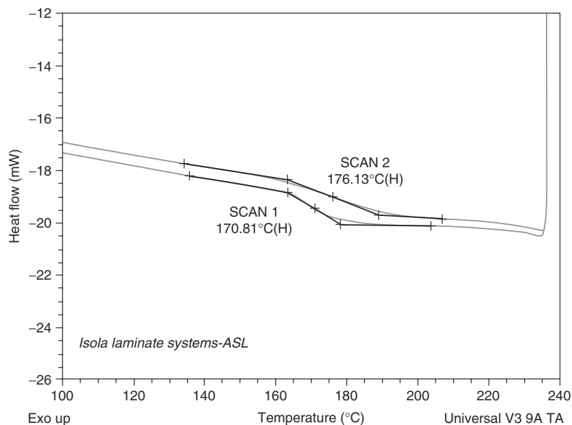
FIGURE 8.2 Measurements of T_g by DSC.
