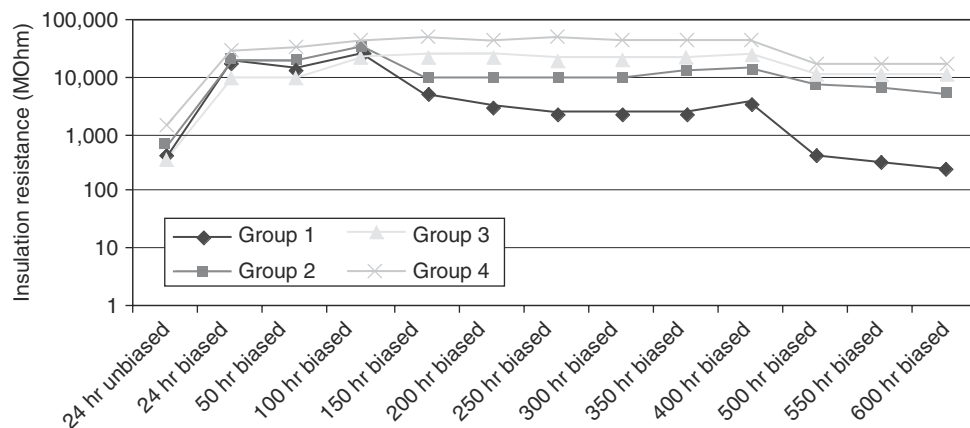
FIGURE 9.20 Results for CAF test example #3.
