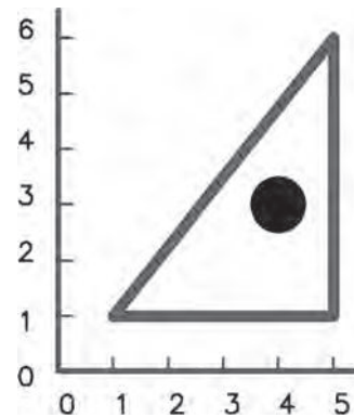
FIGURE 20.2 Datum identification examples.
