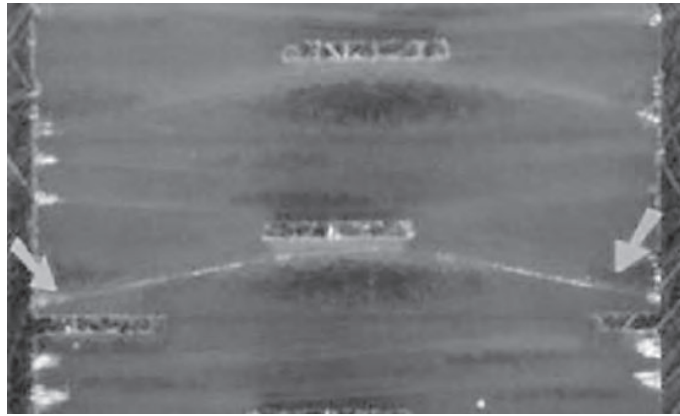
FIGURE 9.13 An example of CAF between two plated through holes.
