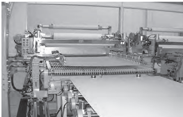
FIGURE 6.10 Sheeting of rolls of copper foil.
