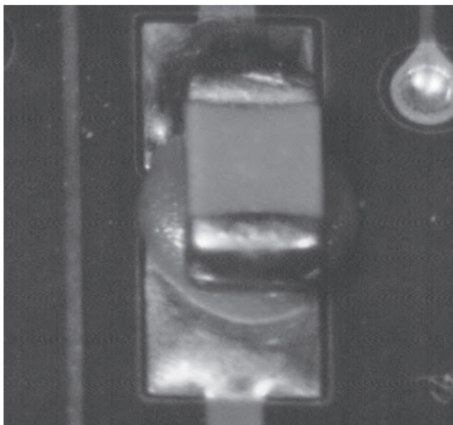
FIGURE 52.20 Adhesive visibly extended from under the component and visible in the terminal area. (IPC)
