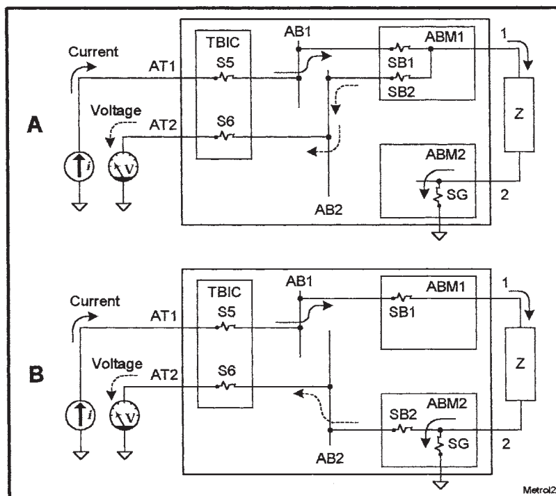
FIGURE 54.10 Two measurements (a) and (b) can be used to measure the voltage across Z for a known current.
