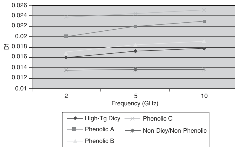
FIGURE 9.30 D_f versus frequency for lead-free compatible FR-4 materials.
