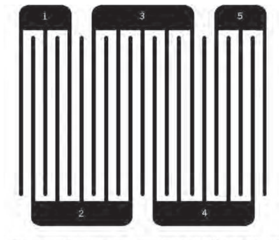
Basic Surface Insulation Resistance (SIR) Test Pattern
