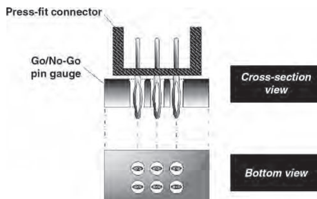
FIGURE 49.14 Gauge for checking connector pin position prior to pressing. This is best used for high lead count, fine-pitch pin press-fit connectors.
