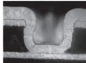
FIGURE 29.12 Example of a blind via that is 5.0 mil in diameter and 3.0 mil deep, plated with chemically mediated bath.
