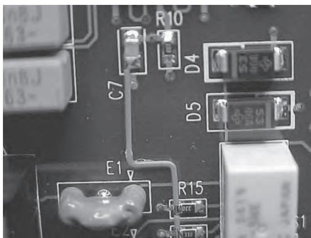
FIGURE 52.39 Example of X-Y routing of jumper wires. (IPC)
