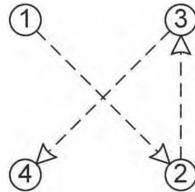
FIGURE 50.7 Manual torque pattern for even fastening of the LGA. Each fastener should receive the same number of turns or partial turns to ensure even seating of the LGA stack.
