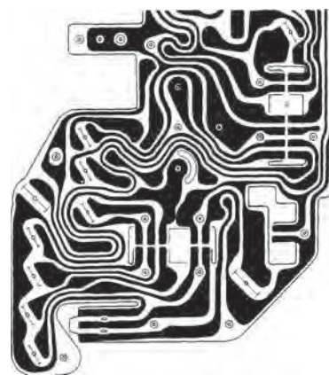
FIGURE 62.22 “Conductor pattern designed for the instrument panel of an automobile.”
