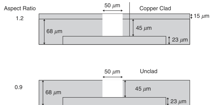
FIGURE 22.9 Impact of 1.2 oz. base copper on the aspect ratio of a 50\text{ }\mu\text{m} via. (Courtesy of Vantico.)
