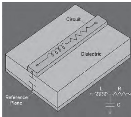
FIGURE 51.17 Impedance diagram of a PCB. (Courtesy of Microtek Laboratories.)
