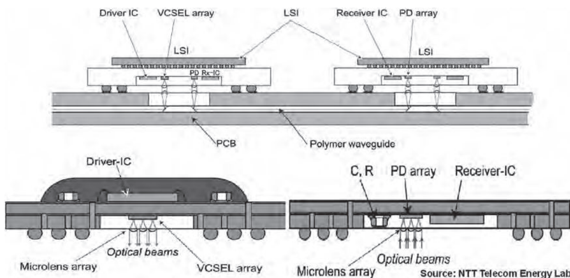
FIGURE 23.42 NTT waveguide-on-board concept with OptoBump packages. (Courtesy of NTT-Lab.)
