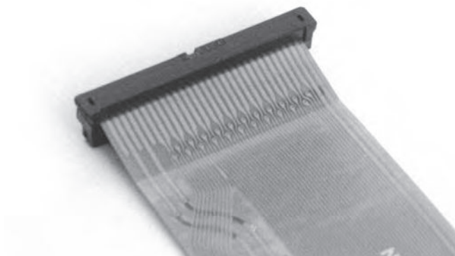
FIGURE 64.18 Clamp type connector for flexible circuits.
