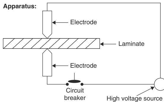
FIGURE 8.17 Dielectric strength.
