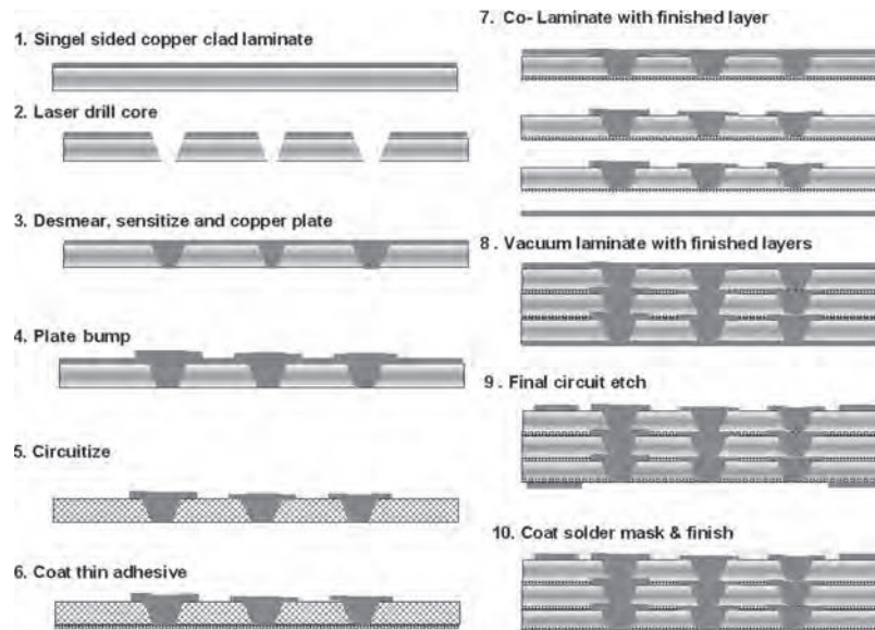
FIGURE 23.15 The typical manufacturing process for SSP boards.
