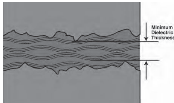
FIGURE 51.24 Layer-to-layer spacing, minimum dielectric thickness, vertical microsection. (Courtesy of IPC.)
