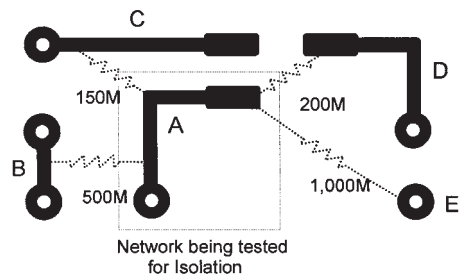
FIGURE 37.6 Parallel leakage detection.
