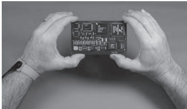
FIGURE 52.2 Appropriate method of handling board to avoid contamination and electrostatic discharge damage. Note position of fingers and the use of a grounding wrist strap.
