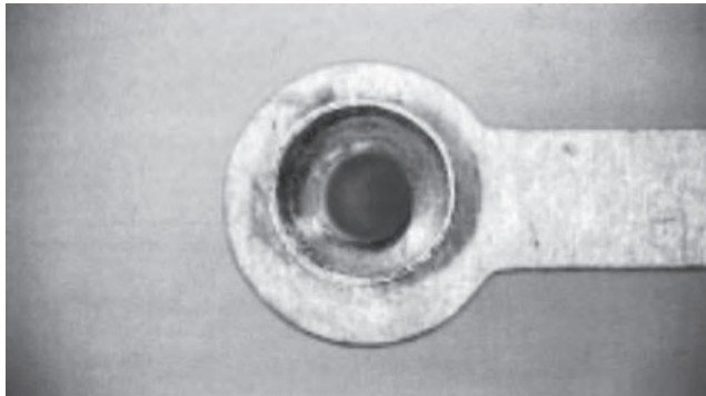
FIGURE 52.8 Flared flange. Acceptable for all Classes.
