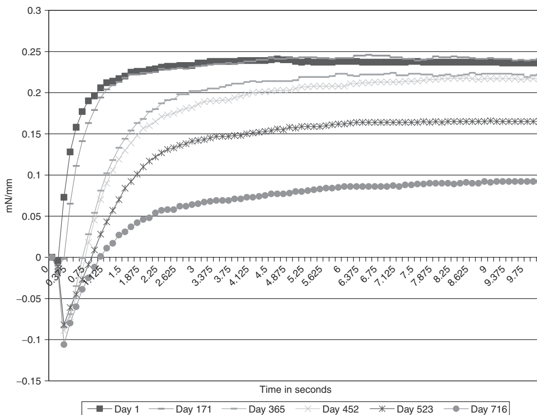
FIGURE 42.13 An excellent example of a good I Sn deposit's gradual decline in solderability performance as a function of intermetallic growth over 716 days. The wetting times increase slightly, which is also as a function of SnO growth on the surface of the deposit.
