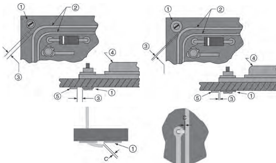
FIGURE 52.10 Examples of acceptable and unacceptable electrical clearance-hardware. (a) Acceptable where: (1) Metallic hardware; (2) Conductor pattern; (3) Specified minimum electrical clearance; (4) Mounted component; (5) Conductor; (b) Unacceptable where hardware reduces clearances to less than specified electrical clearance; (1) Metallic hardware; (2) Conductor pattern; (3) Spacing less than minimum electrical requirements; (4) Mounted component; (5) Conductor; (c) Unacceptable as lead is clinched toward a noncommon electrical conductor (1) and violates clearance; (C) requirement.
