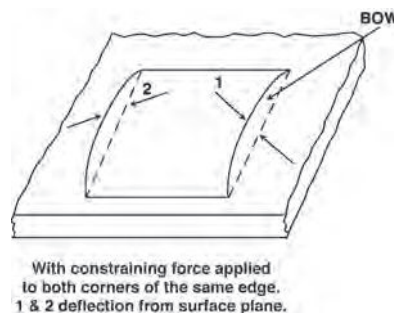
FIGURE 51.13 Bow measurement of PCB. (Courtesy of IPC.)
