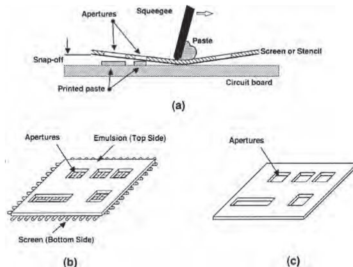
FIGURE 40.16 Screen and stencil printing: (a) the squeegee movement used to print adhesive or paste through a screen or stencil; the construction of a screen (b) and stencil (c) used for printing.
