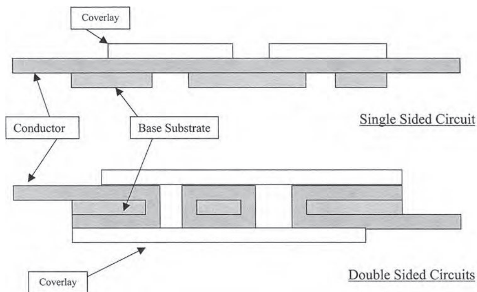
FIGURE 66.1 Basic constructions for Flying-leads for flexible circuits.
