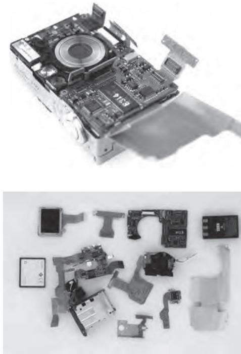
FIGURE 61.3 Flexible circuits applied for digital camera. (Courtesy of Canon).
