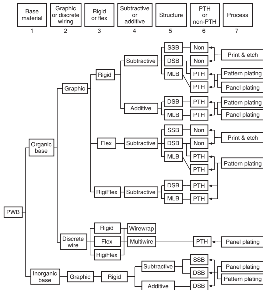
FIGURE 5.1 Classification of printed wiring boards.
