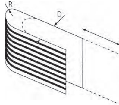
FIGURE 62.16 “Typical dynamic flexing mode of flexible circuit specified by IPC-TM-650.”
