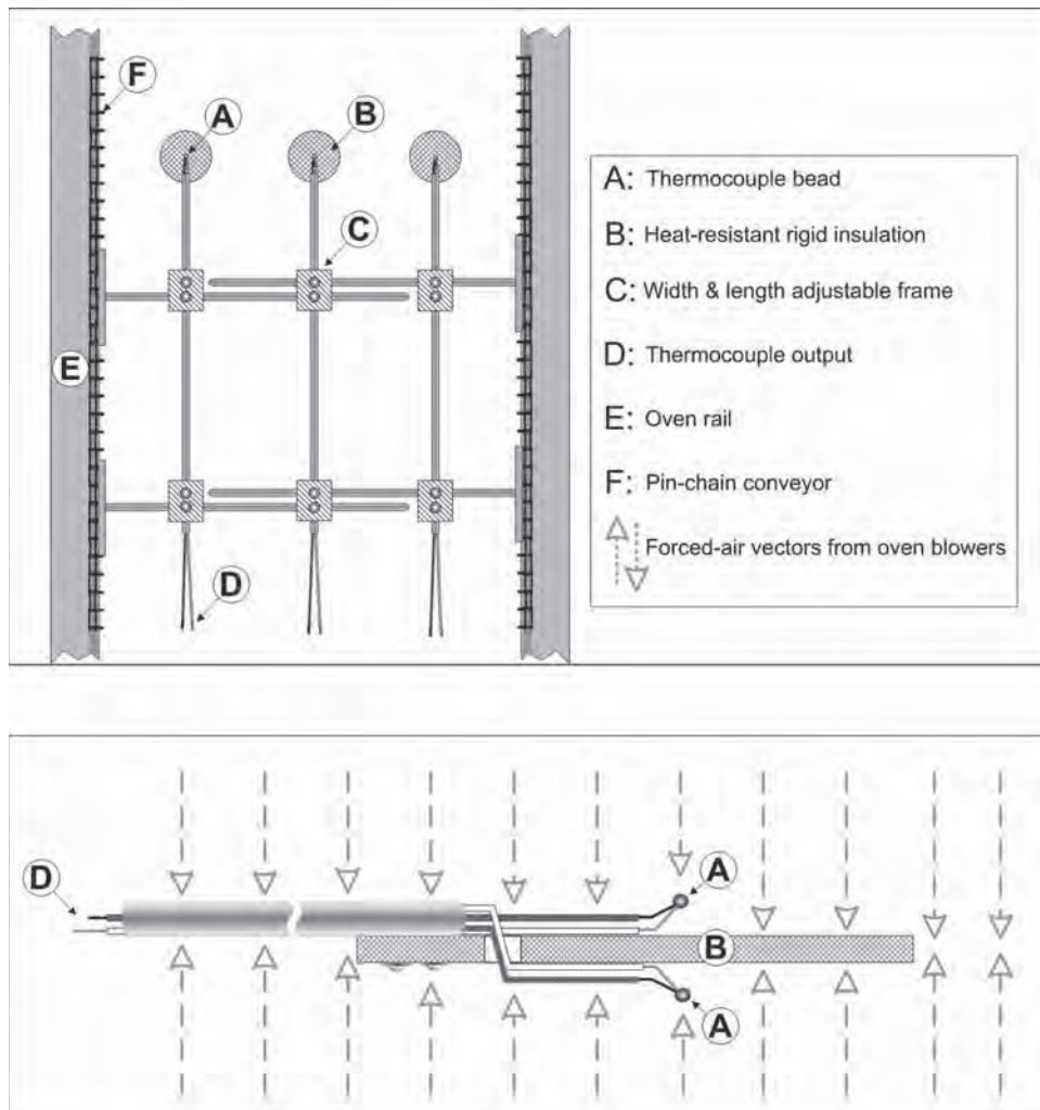
FIGURE 47.9 Schematic plan view and detailed side view of an adjustable oven characterization fixture (oven diagnostic tool) composed of pairs of thermocouples, shielded from one another by a rigid, heat-resistant insulator. The thermocouple positions are adjustable in width and length for investigating temperature distribution along the tunnel width.
