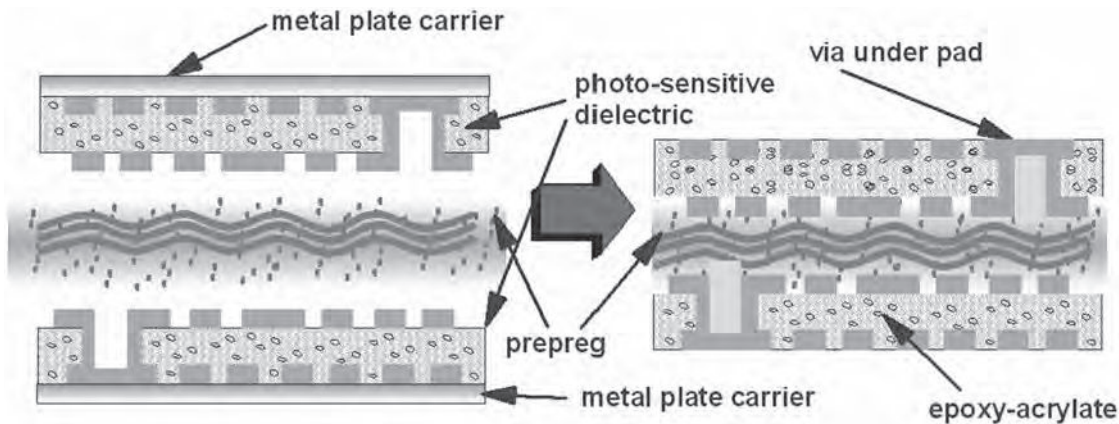
FIGURE 23.11 The carrier-formed circuit multilayer structure.
