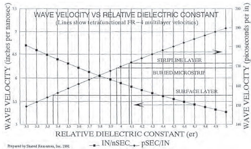
FIGURE 13.3 Signal velocity as a function of dielectric constant. (Prepared by Shared Resources, Inc., 1991.)
