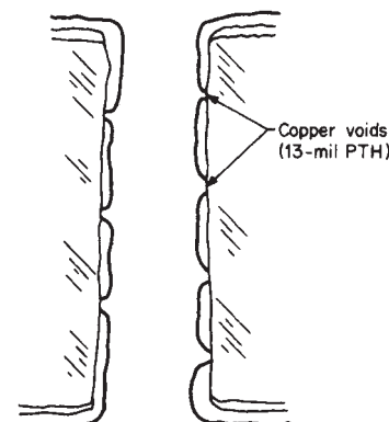
FIGURE 29.19 PTH vertical cross section illustrating copper voids.
