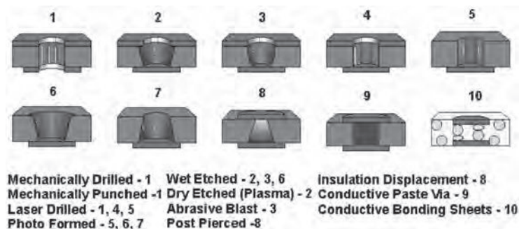
FIGURE 22.3 Representative microvia profiles and the processes that produce them.
