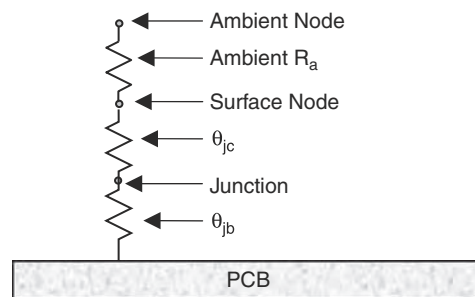
FIGURE 17.13 Thermal conduction representation of an electrical component by two thermal resistances, \theta_{jc} and \theta_{jb} . The resistance to ambient ( R_a ) is the result of convective and radiative heat loss.
