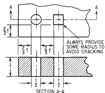
FIGURE 35.1 Illustration of the proper sizing and locating of pierced holes with respect to one another and to the edge of paper laminates. Minimum dimensions are given as multiples of laminate thickness t .
