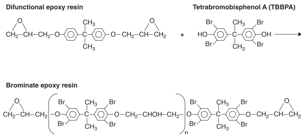
FIGURE 7.3 Brominated difunctional epoxy resin.
