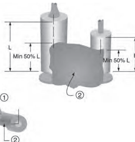
FIGURE 52.22 Adhesive on vertically mounted components. (1) Top view, (2) Adhesive. (IPC)
