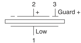
FIGURE 8.15 Circuit for volume resistance.
