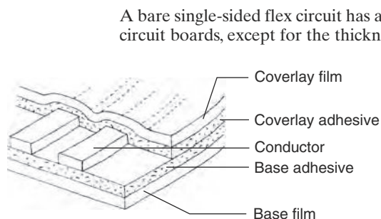
FIGURE 62.3 Basic structure of single-sided flexible circuit.
