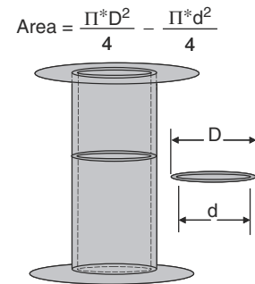
FIGURE 16.14 Via cross-sectional area.
