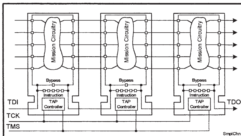
FIGURE 54.4 A collection (chain) of boundary scan devices can be used to test interconnections between ICs.
