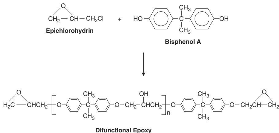
FIGURE 7.1 Reaction to form difunctional epoxy resin.
