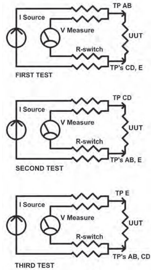
FIGURE 37.5 Measurement sequence for three isolations.
