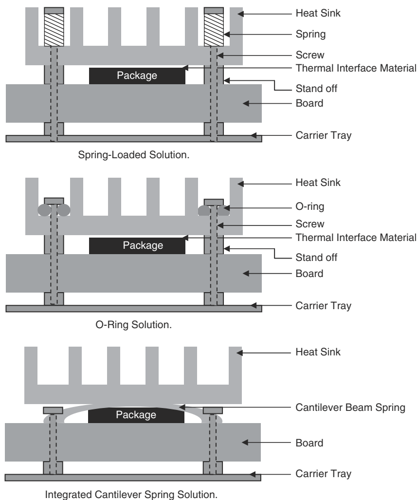
FIGURE 58.17 Heatsink attachment methods.
