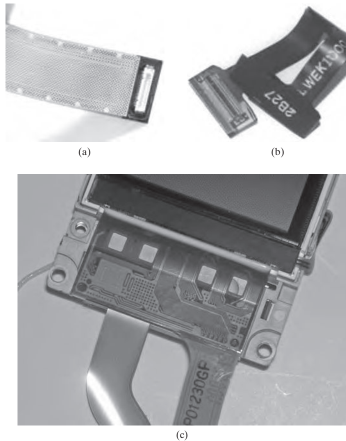
FIGURE 66.14 Shielding of the flexible cables (a): Screen-printing of silver paste (b): Screen-printing of carbon paste (c): Lamination of thin aluminum foil.
