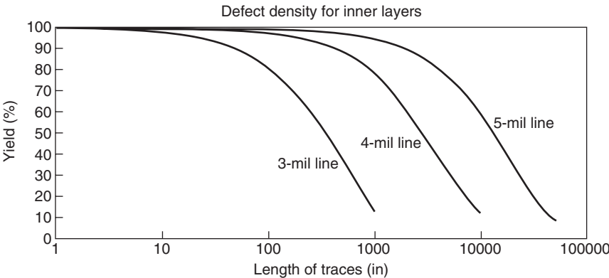
FIGURE 2.10 Board yields vs. conductor width.
