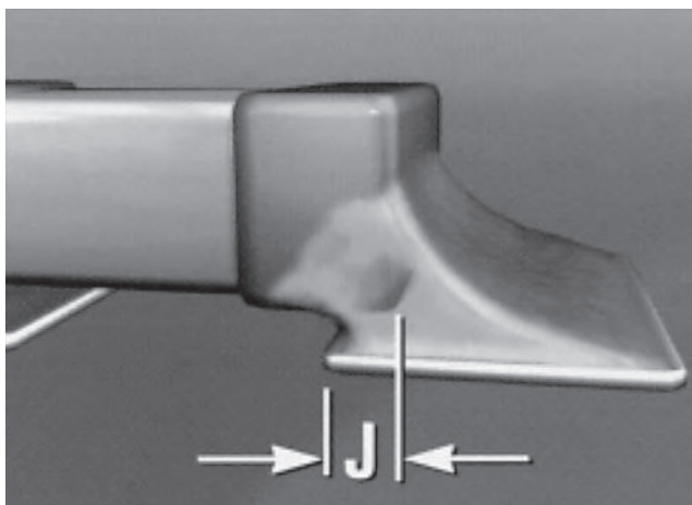
FIGURE 52.17 Example placement and solder fillet for surface mount chip component. Evidence of overlap of contact (J) between the component termination and the land is required. (IPC)
