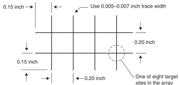
FIGURE 25.6 Fiducial target.
