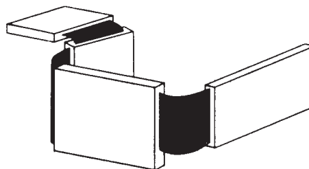
FIGURE 65.3 Folding type rigid/flexible circuit.
