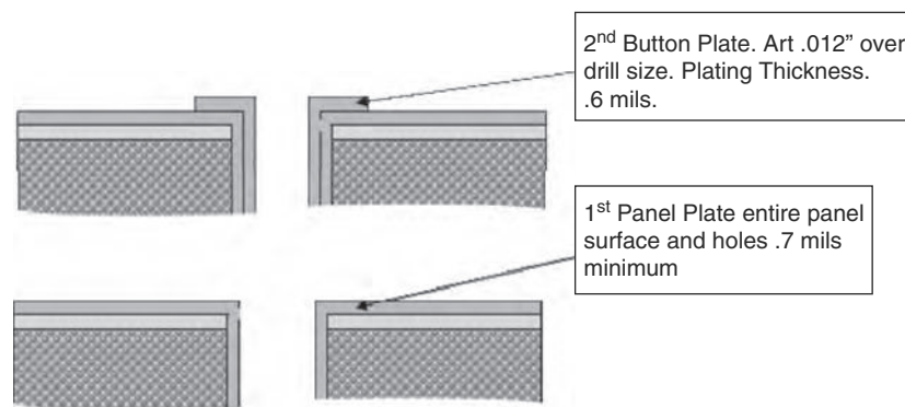
FIGURE 27.27 Pre-hole-fill plating.
