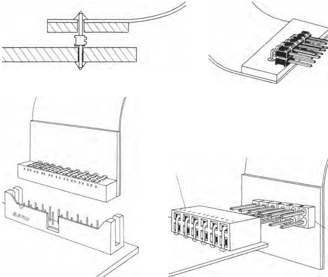
FIGURE 64.16 Examples of soldering lead-type connection in flexible circuits.
