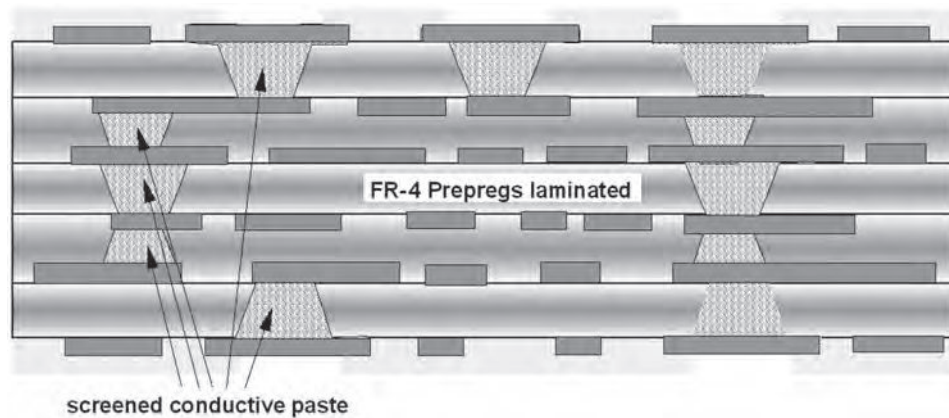
FIGURE 23.26 The VIL manufacturing sequence for a multilayer substrate.
