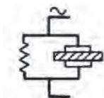
FIGURE 12.9 Dissipation factor test.
