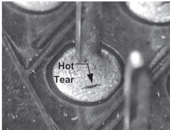
FIGURE 47.30 Hot tear (shrink hole) on an SAC wave-soldered PTH joint. (Courtesy of Hewlett-Packard).
