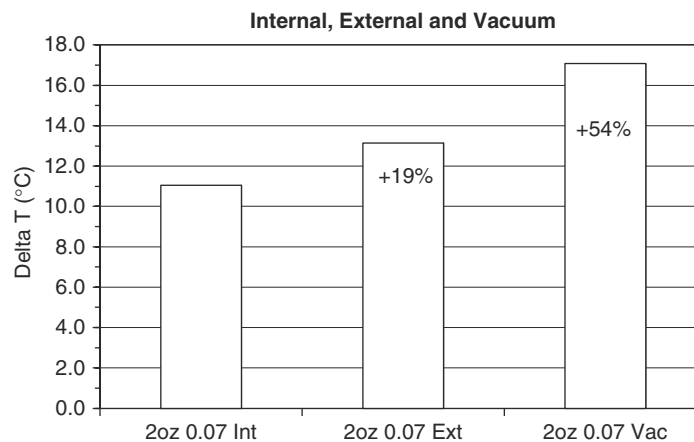
FIGURE 16.13 Vacuum versus baseline environments.
