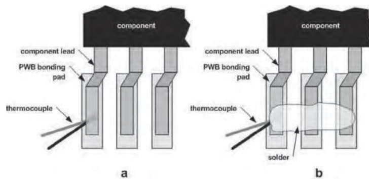
FIGURE 47.12 Checking the quality of the thermocoupling: (a) A good thermocouple deployment. The bead is secured beneath a single lead and held in place with high-temperature solder. (b) The thermocouple is held in place by high-temperature solder but the solder has bridged to multiple leads. Temperature indicated will be that of the entire thermal mass of leads and solder rather than a single lead as in (a).
