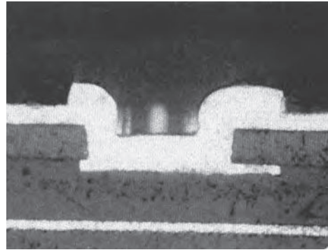
FIGURE 65.11 Micro blind via hole on a multilayer rigid/flexible circuit made by a build-up process using resin-coated foil. The hole diameter is 150 micrometer. (Source: Photo Machining.)
