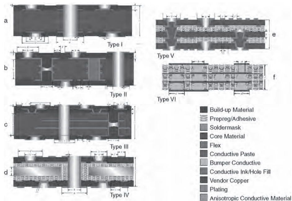
FIGURE 22.4 IPC-2226 microvia structures from Type I to Type VI.
