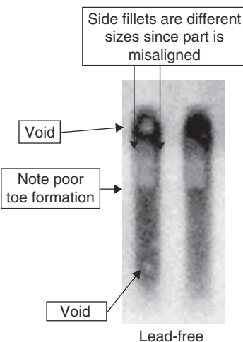
FIGURE 53.6 An x-ray image of a lead-free example.
