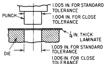
FIGURE 35.2 Example of proper tolerance of a punch and die.
