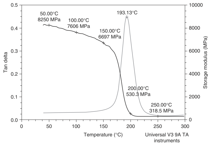
FIGURE 8.3 Measurement of T_g by DMA.
