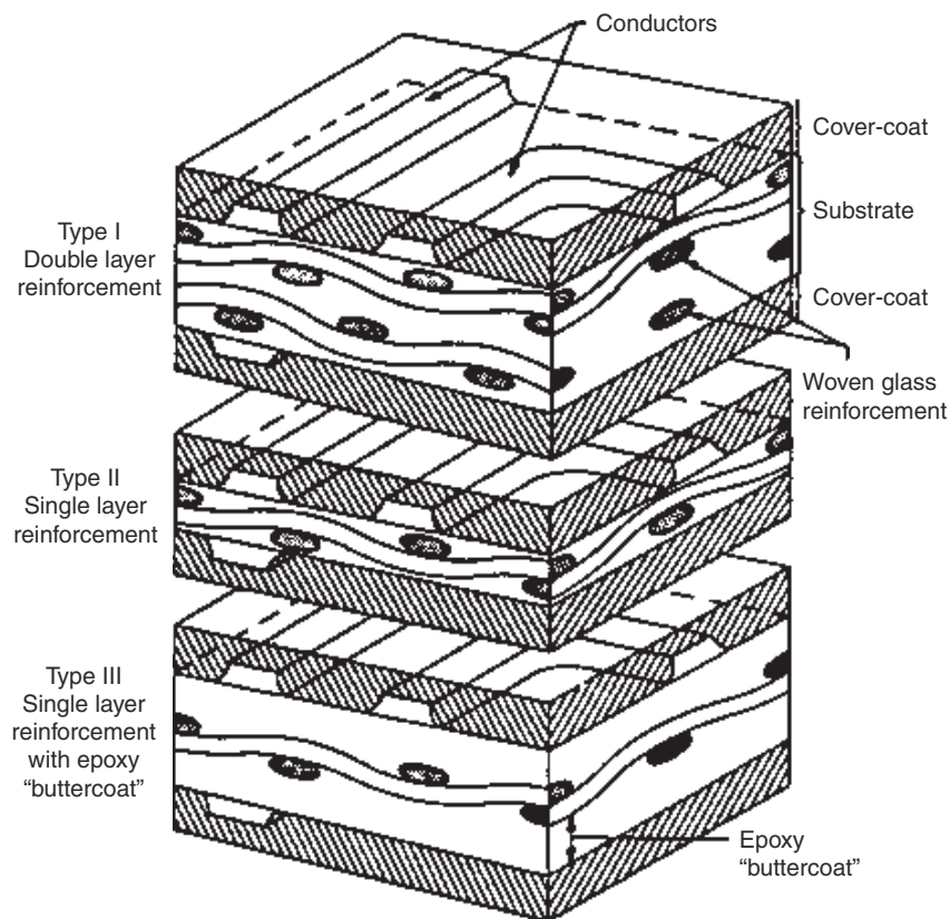
FIGURE 56.1 AT&T test vehicle compared: (a) double-layer glass reinforcement; (b) single-layer glass reinforcement; (c) single-layer glass reinforcement with extra "buttercoat." 2 © 1976 IEEE
