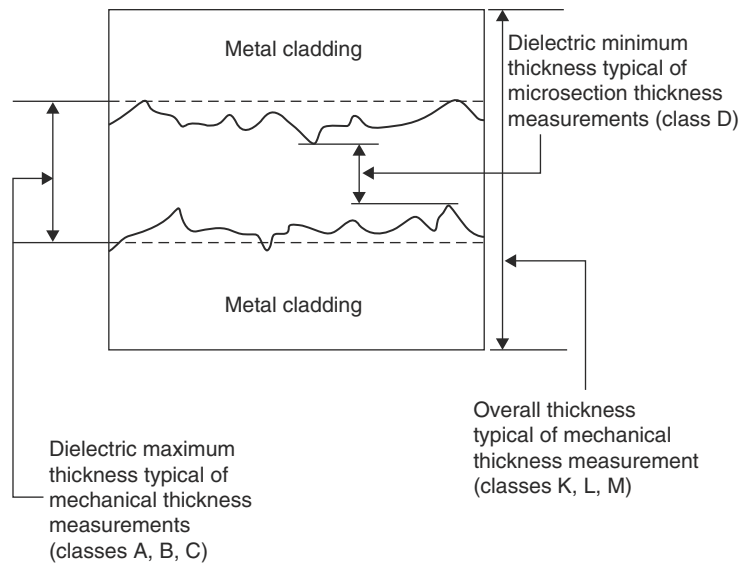
FIGURE 6.5 Dielectric minimum thickness measurements by microsection. (from IPC-4101)
