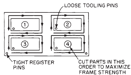
FIGURE 35.13 Single-pin method.
