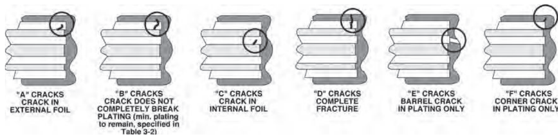
FIGURE 51.27 Types of cracks in the PTH, vertical microsection. (Courtesy of IPC.)
