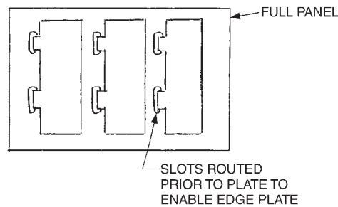
FIGURE 35.7 Multiple-image palletization.
