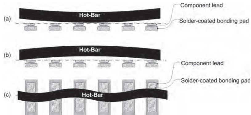
FIGURE 47.39 If not constructed properly, the hot-bar can develop a “smiling” profile (a), a “frowning” profile (b), or may warp along its length (c). (a) and (b) are front views whereas (c) is a top view. The dashed line in (a) and (b) shows the desired seating plane.
