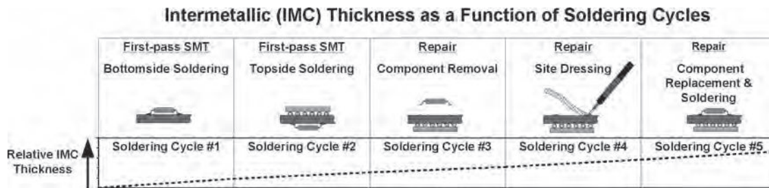
FIGURE 48.2 Soldering steps required for first-pass soldering of a bottomside component on a PWB and success reflow steps encountered during first-pass soldering and repair. Note that the intermetallic compound formation thickness is not truly linear with each step. Thickness depends on materials of the soldering system, time above solder alloy liquidus, peak temperature, etc. The illustration is meant to show that with each reflow cycle, there is increased intermetallic layer thickness.
