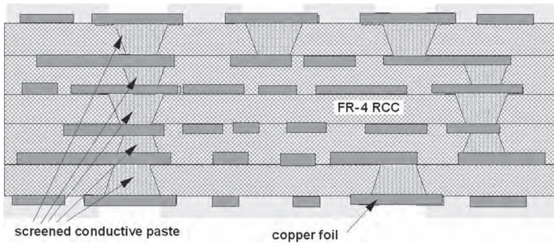
FIGURE 23.24 The MSF manufacturing sequence for a multilayer substrate.
