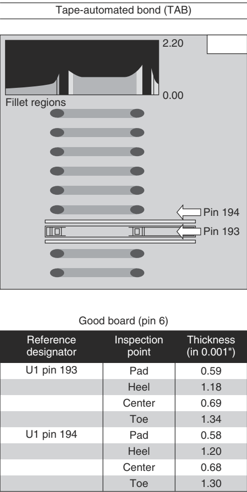
FIGURE 53.13 Cross-sectional x-ray image of TAB solder joints. Image-processing software converts the grayscale readings of the image for pin 193 into the side profile of solder thickness shown above the image. The actual calibrated measurements of average solder thickness across the pad, heel fillet height, center thickness, and toe fillet height processed from the images of pins 193 and 194 are shown in the table below the x-ray image. These measurements indicate that both of these solder joints are good.
