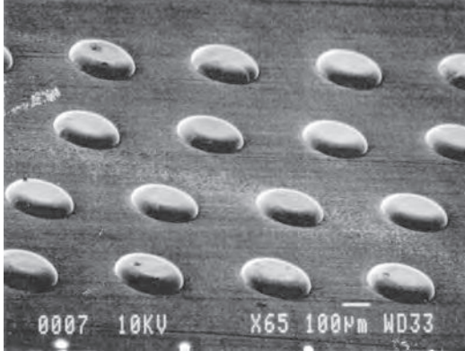
FIGURE 64.22 Flat disk-shaped microbump array on flexible circuit fir area contacts. Contact metal is copper-nickle-gold at 0.5 mm pitch. (Source: Asahi Fine Technology.)
