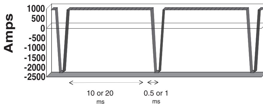
FIGURE 29.14 Periodic pulse reverse rectifier output wave.
