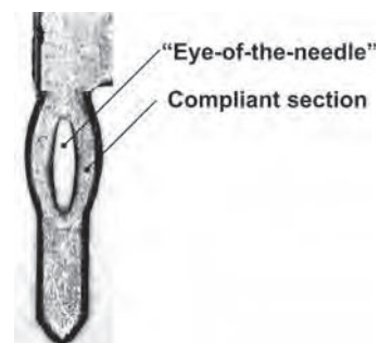
FIGURE 49.4 “Eye-of-the-needle” configuration press-fit pin, shown before compression.
