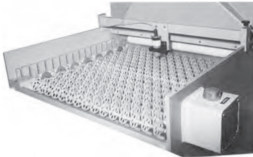
FIGURE 63.12 Special wheel conveyor system for thin, flexible materials showing high density and smooth wheels. (Source: Camellia.)
