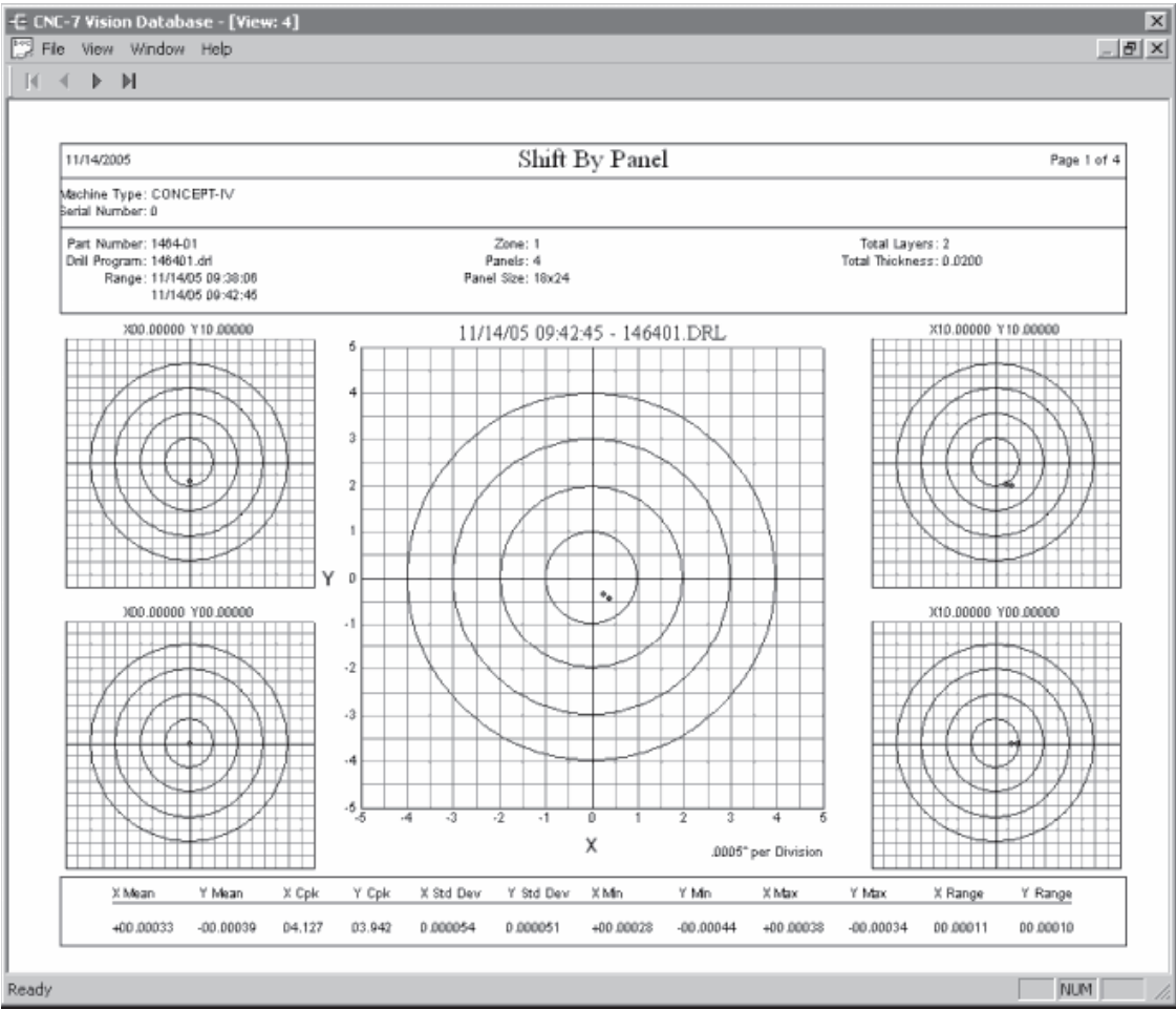
FIGURE 25.15 Report view.
