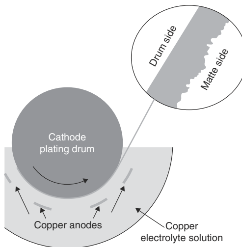
FIGURE 7.21 Electroplating copper foil.
