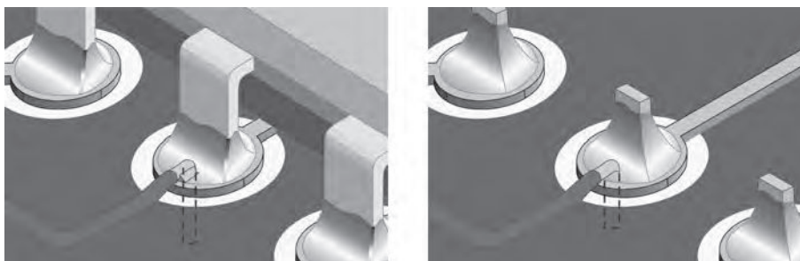
FIGURE 52.40b Example of wire connected to a via hole with a lead installed.
