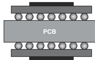
FIGURE 58.7 Double-sided BGA in mirror configuration. Note that the PCA is an exact mirror about the center line of the PWB. In some instances the top- and bottom-side packages share common vias.
