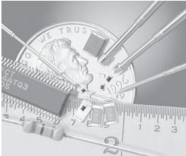
FIGURE 55.1 A US penny shows the size of some common PC board components, some older, some recent. The small black devices near Lincoln's bow tie are 04-02 ( 40 \times 20 mils) surface-mount resistors. (Now 02-01 [ 20 \times 10 mils] devices are being used.) Some 100-, 75-, and 50-mil test probes are shown for comparison. Note the lettering on the penny is done with 10-mil lines and the width of the circular part of the 9 is 35 mils, a common probe target size. (Photograph courtesy of Agilent Technologies.)
