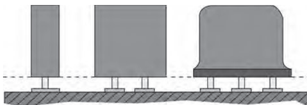
FIGURE 52.16 Radial leaded components spacing. Component is perpendicular and base is parallel to board. Acceptable clearance varies with Class. (IPC)
