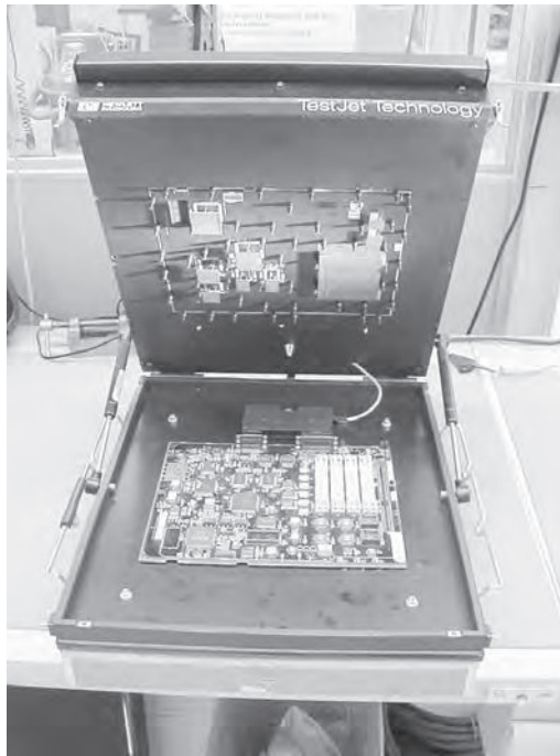
FIGURE 55.14 A test fixture with board on a bed of nails, with clamshell top fixture containing capacitive sensor plates. Notice eight closely spaced sensor plates (right) that test for opens in eight (white) connectors on the board.
