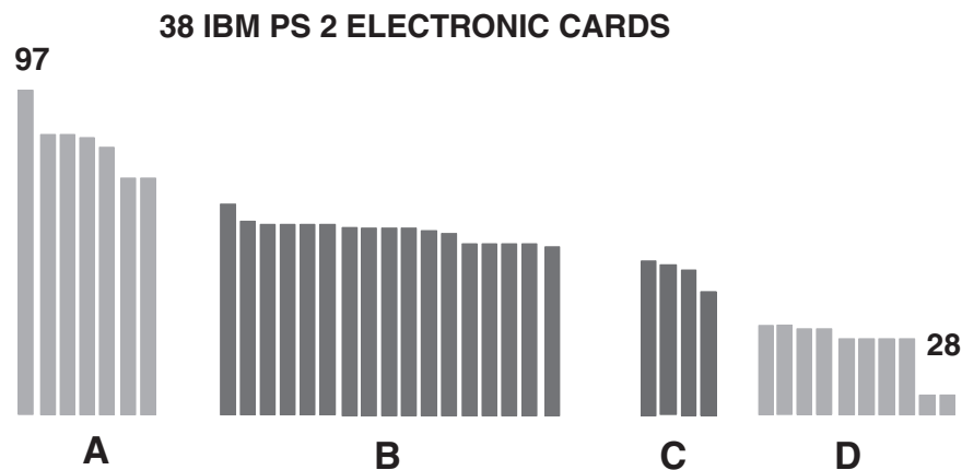
FIGURE 19.17 Improvement in producibility scores as a result of the Assembly Report Card.
