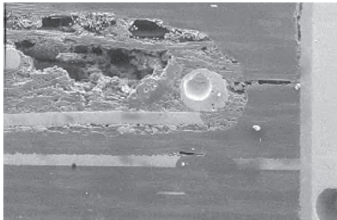
FIGURE 56.9 Catastrophic field failure of military hardware. The conductive filament grew from the +20 V ground plane to the -20 V ground pin. Flux residues enhanced this failure rate. 16
