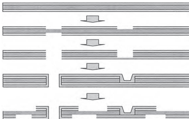
FIGURE 63.4 Basic high density circuit generation process by subtractive process.
