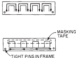
FIGURE 35.12 No-internal-pin method. Step 1: Cut three sides (a). Step 2: Apply masking tape (b). Step 3: Cut parts away.
