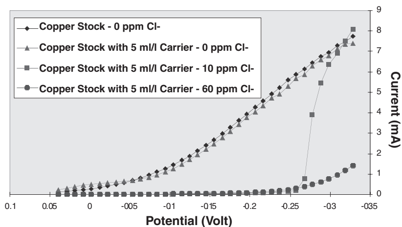
FIGURE 29.8 Effect of chloride concentration in a copper stock solution with carrier.
