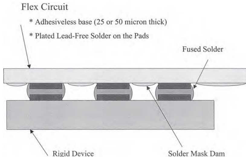
FIGURE 64.4 Flexible termination by solder fusing.
