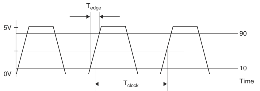
FIGURE 9.21 Digital communication.
