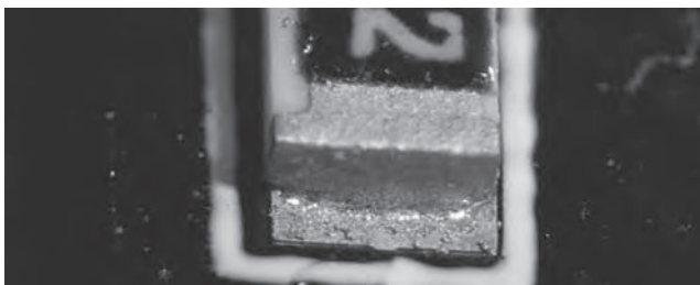
FIGURE 52.26 Example of non wetting. (IPC)
