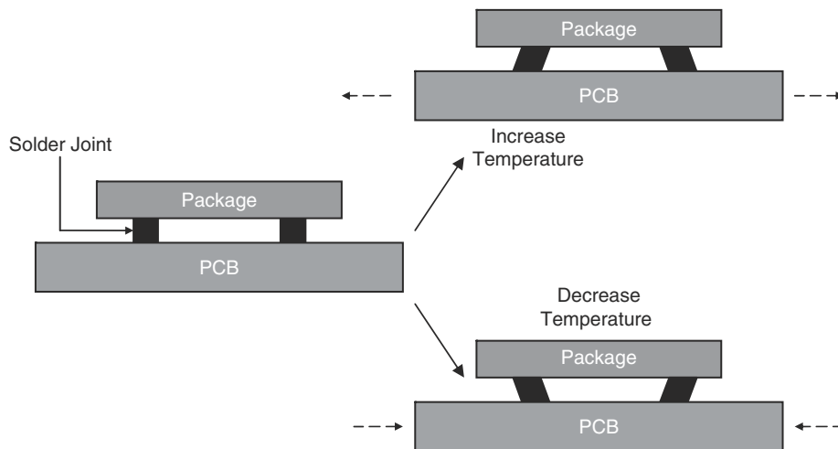
FIGURE 58.31 Simplified CTE mismatch effects. As the temperature increases, the PWB expands at a higher rate than the package due to the package having a lower effective CTE. As the temperature decreases, the opposite effect is observed.
