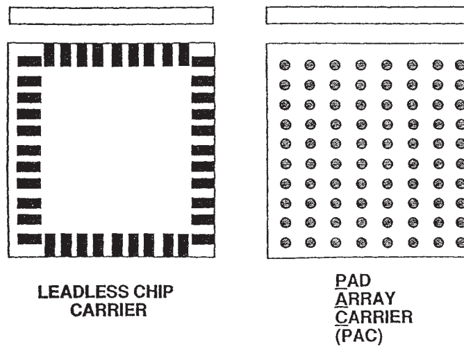
FIGURE 3.9 Perimeter I/O package vs. area array package.
