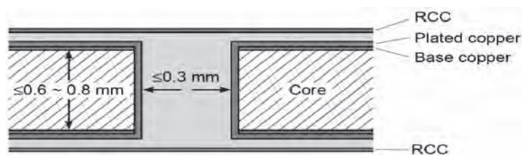
FIGURE 22.15 Conditions under which the through hole can be filled with resin by RCC lamination.
