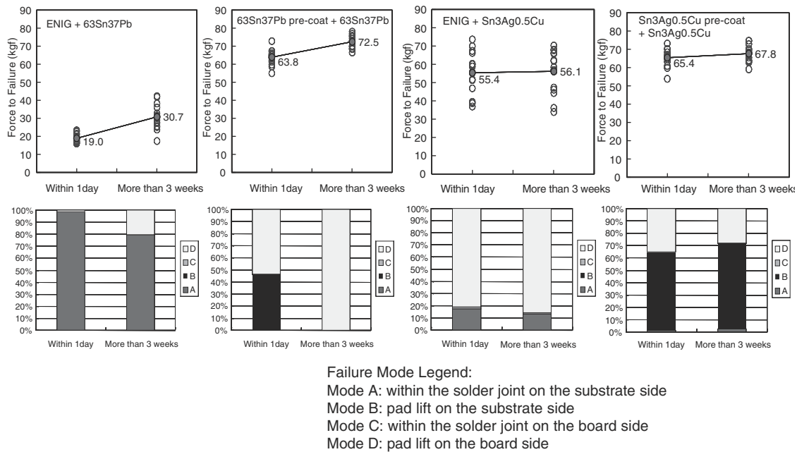
FIGURE 59.14 Data set comparing the force-to-failure value of Pb/Sn and Sn/Ag/Cu assemblies for two different surface finishes (ENIG and SOP) as a function of time after reflow. The histograms show a comparison of the different failure modes obtained in the bend tests. (Reprinted with permission from Kyocera SLC Technologies. /© [2005] IEEE.)
