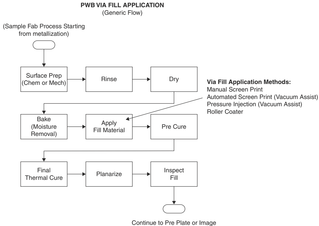
FIGURE 27.28 Generic via fill application flow.
