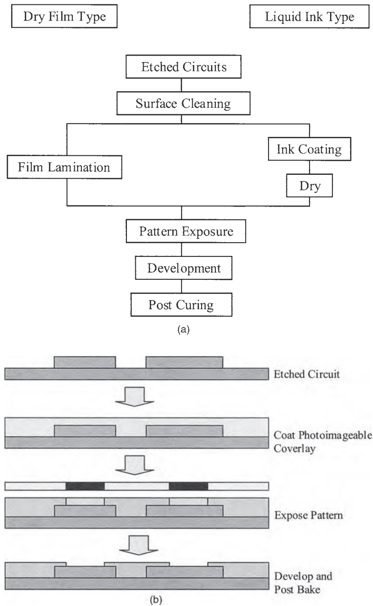
FIGURE 63.28 An example of a manufacturing process for photoimageable coverlay (a) A schematic flowchart of a generic process using either dry film or liquid resist, (b) A graphic flowchart starting with the etched circuit, showing the manufacturing process for a photoimageable coverlay.
