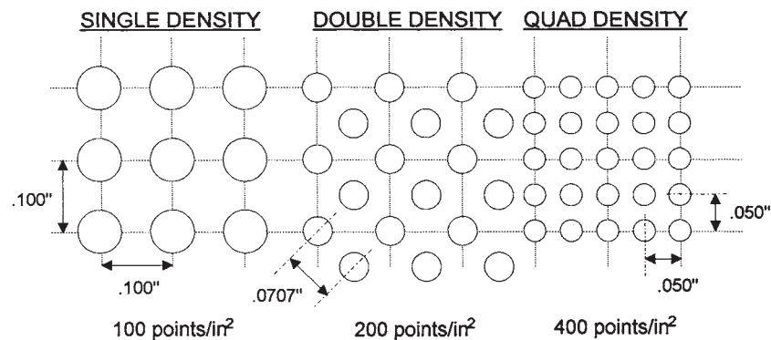
FIGURE 37.11 Single-, double-, and quad-density universal grid patterns.
