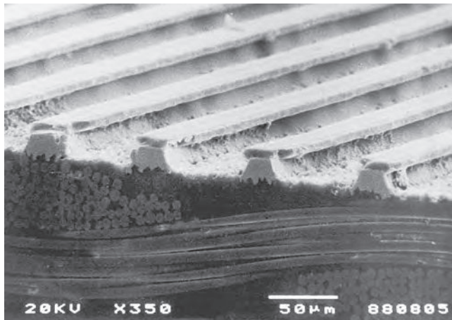
FIGURE 31.6 Formation of fineline conductors by etching process results in undesirable, nonrectangular conductor cross section. (Photo courtesy of Ividen Co., Ltd.)
