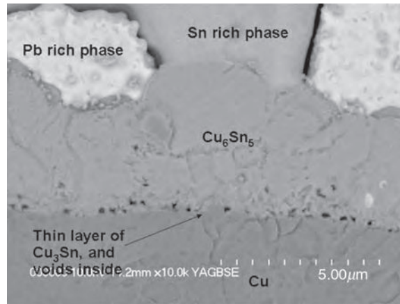
FIGURE 58.22 SEM Backscattering Electron Image of Tested Sample with Solder-On-Pad Surface finish – Package/Ball Interface. The image shows the intermetallics formed at the joint/package interface. These intermetallics include a thick layer of \text{Cu}_6\text{Sn}_5 and a thinner layer of \text{Cu}_3\text{Sn} . Small voids are seen at the \text{Cu}_6\text{Sn}_5 and \text{Cu}_3\text{Sn} interface. 24 (Reprinted with permission from IEEE © [2005].)
