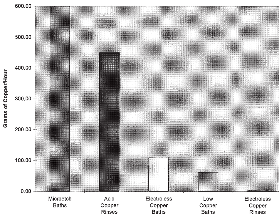
FIGURE 60.2 Major sources of copper expressed in grams per hour discharged. Inner- and outerlayer etching is excluded from this figure since it is so large in relation to the other contributors.
