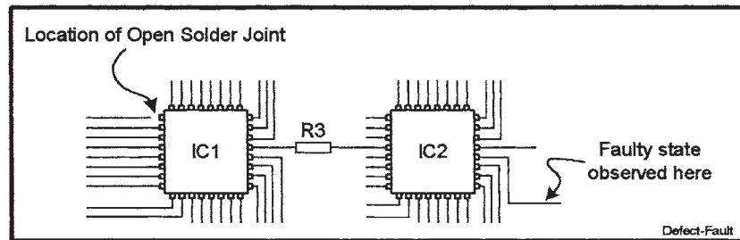
FIGURE 55.2 A defective solder joint on an input pin to IC1 causes a fault on an output of IC2. Note that IC1, R3, and IC2 are suspect, as well as six solder joints, two IC input buffers, two IC output buffers, and four IC bond wires.
