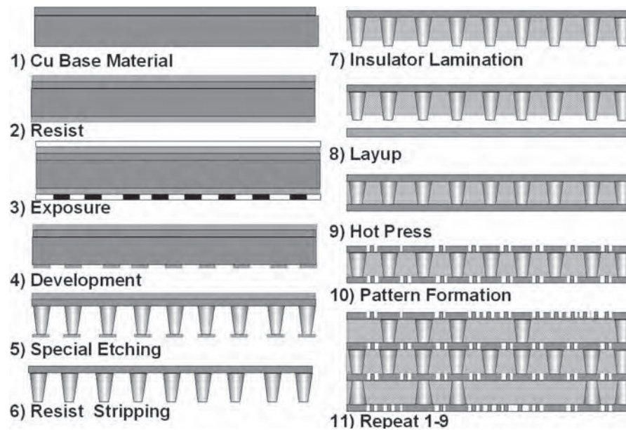
FIGURE 23.34 The manufacturing process for the NMBI substrates.
