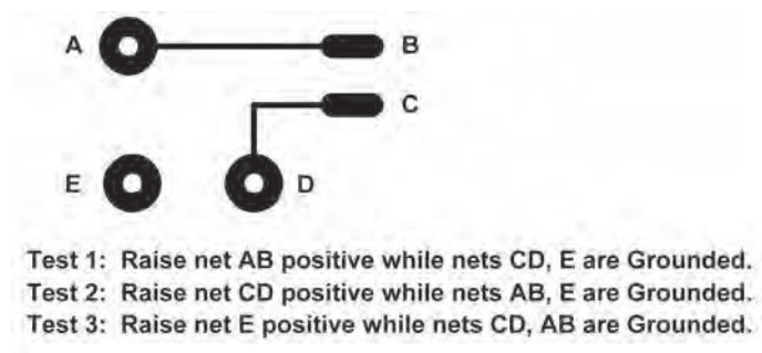
FIGURE 37.4 True isolation test of three-network board.
