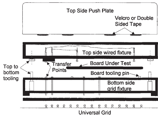
FIGURE 38.17 Transfer point clamshell fixture for dual-side access.
