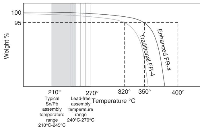
FIGURE 6.4 Illustration of decomposition curves.
