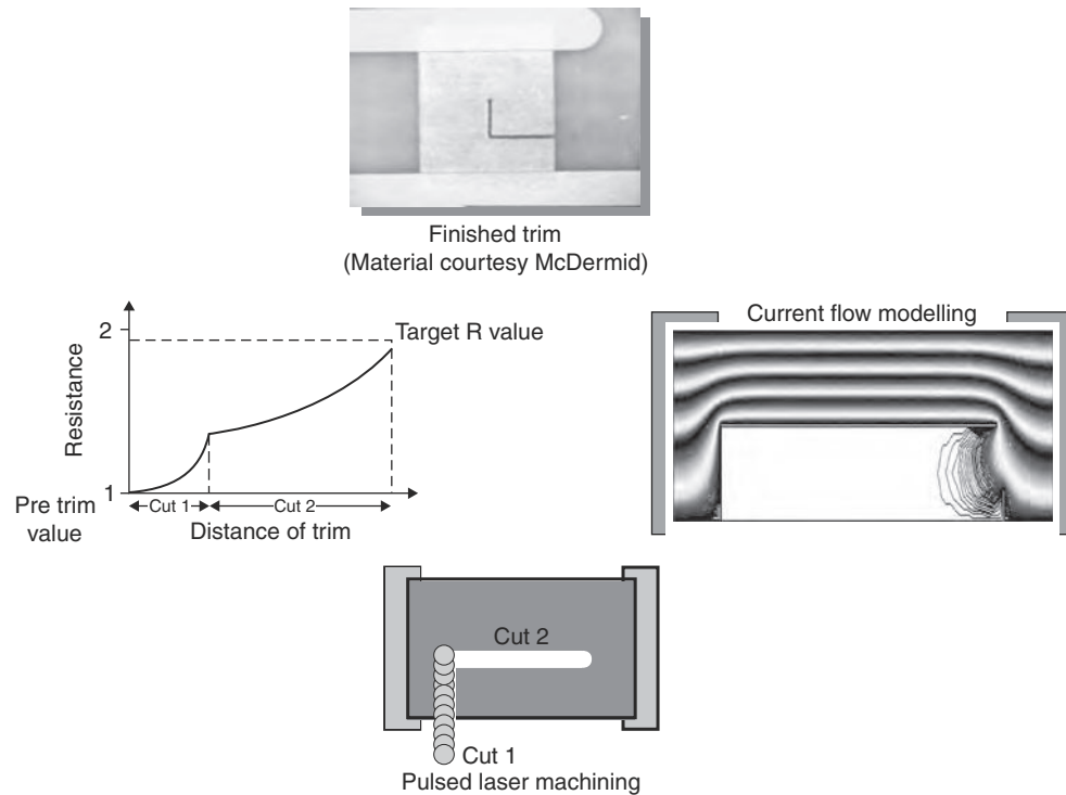
FIGURE 21.4 Resistor trimming.
