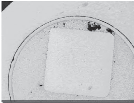
FIGURE 51.19 Example of interconnection separation in a horizontal microsection. (Courtesy of Microtek Laboratories.)
