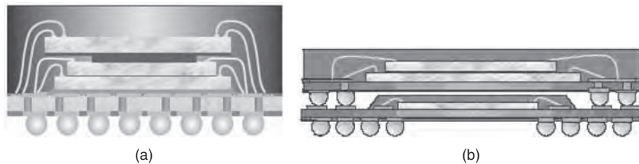
FIGURE 58.6 (a) Stacked-die package. Several dies are stacked within a single package and wirebonded to a single substrate. (b) Stacked package. Several wirebonded packages are stacked on top of each other with solder balls. (Courtesy of Amkor Technology, Inc.)
