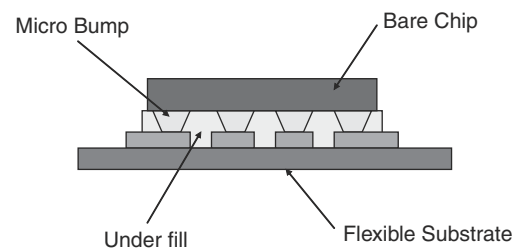
FIGURE 64.10 Flip chip mounting of bare chip.
