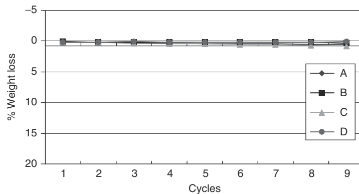
FIGURE 10.7 Decomposition through multiple cycles to 235°C.
