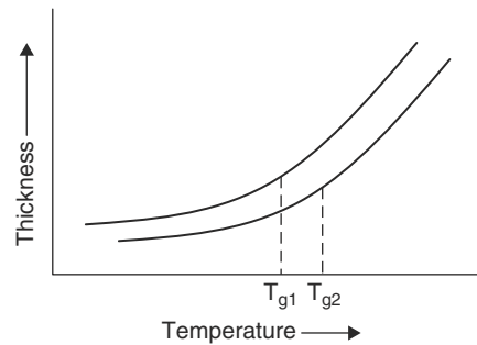
FIGURE 6.2 Measuring the degree of cure by measuring T_g values.
