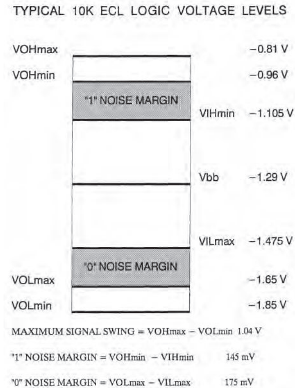
FIGURE 13.8 Noise-band chart for ECL. (Prepared by Ritch Tech, 1992.)
