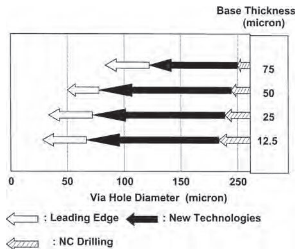
FIGURE 62.8 Microvia capabilities shown by base thickness and hole diameter. Also shown is the range of technologies from HDI to mechanical drilling required to create the vias.
