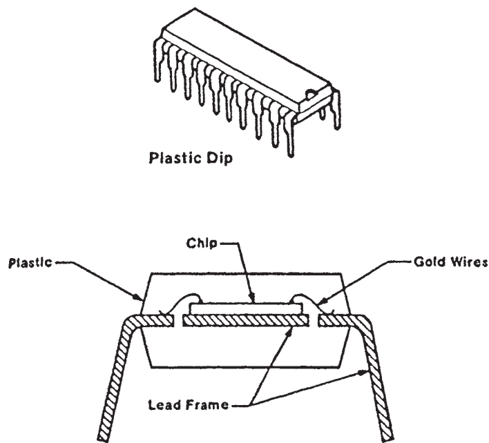
FIGURE 3.5 Dual inline package.
