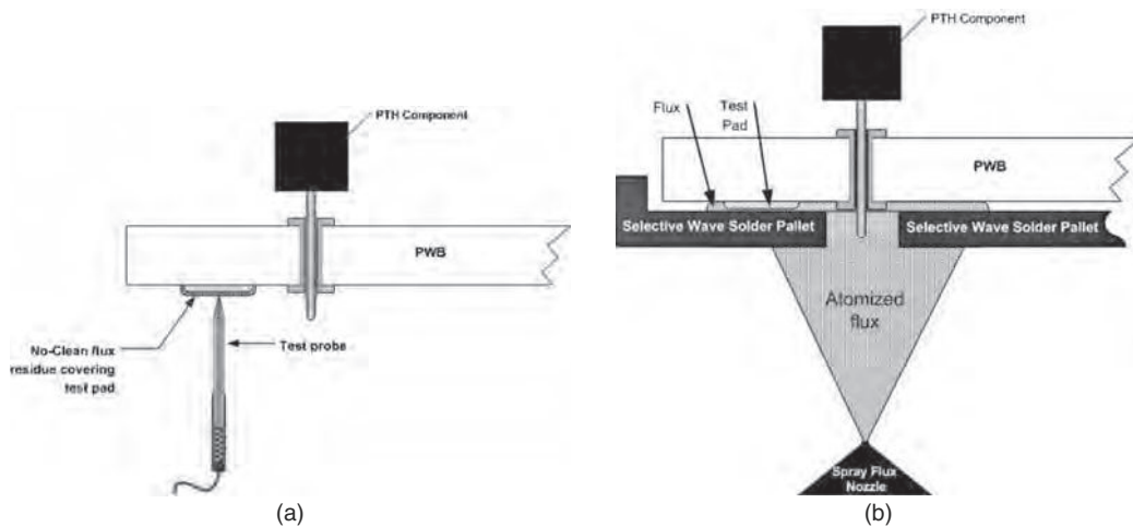
FIGURE 46.5 ICT probe noncontact: (a) If there is flux on a test pad, it will harden after soldering and may prevent the test probe from making electrical contact to the test pad. The test result may be interpreted as an “open” circuit. (b) As the board is fluxed in preparation for the wave solder process, the liquid flux may be drawn by capillary action between the wave solder pallet and the PWB. When this occurs, the in-circuit test pad (the target for bed-of-nails testing) may become fouled with solder flux. The flux residue inhibits probe contact.
