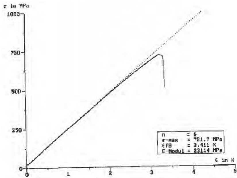
FIGURE 12.4 Typical flexural strength measurement curve.
