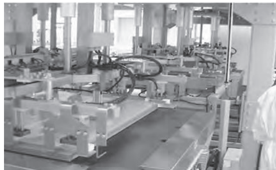
FIGURE 6.12 Automated build-up of copper and prepreg.
