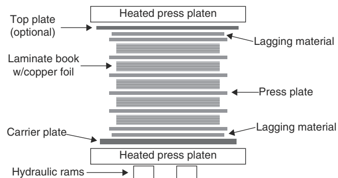
FIGURE 6.13 Laminate pressing.
