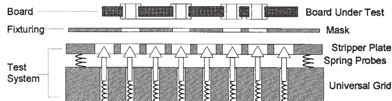
FIGURE 38.5 Exclusion mask fixture.
