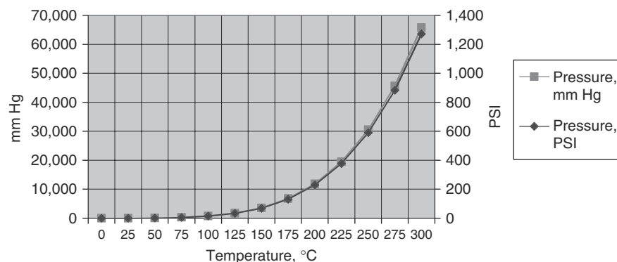
FIGURE 11.1 Vapor pressure of water versus temperature.
