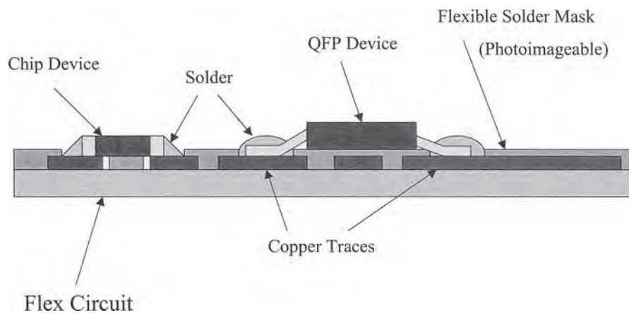
FIGURE 64.2 SMT soldering of high density flexible circuits.
