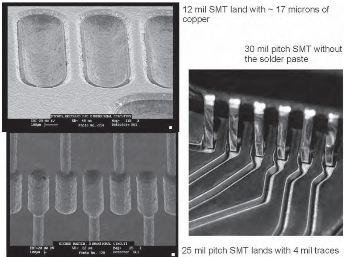
FIGURE 23.36 Various views of SEMs of imprinted circuit liquids and traces. (Courtesy of Dimensional Circuits.)
