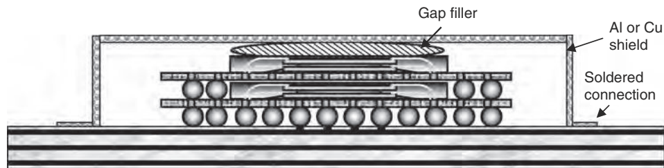
FIGURE 17.11 A stacked package configuration on a PCB with a perforated RF shield that is being used to spread heat from the top package. Thermal gap filler material such as thermal grease is used to conduct the heat from the top package into the RF shield.
