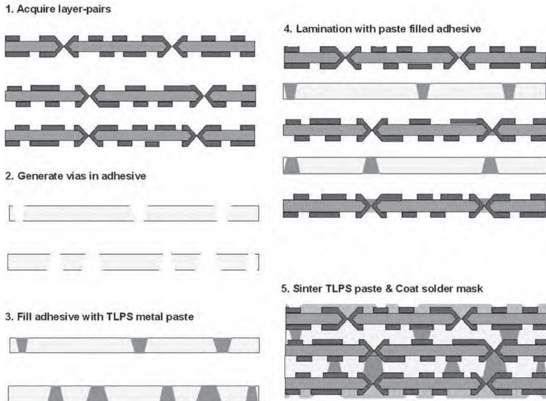
FIGURE 23.20 The OrmaLink multilayer substrate fabrication process.
