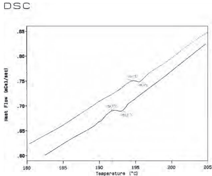
FIGURE 12.6 Example of a DSC result.
