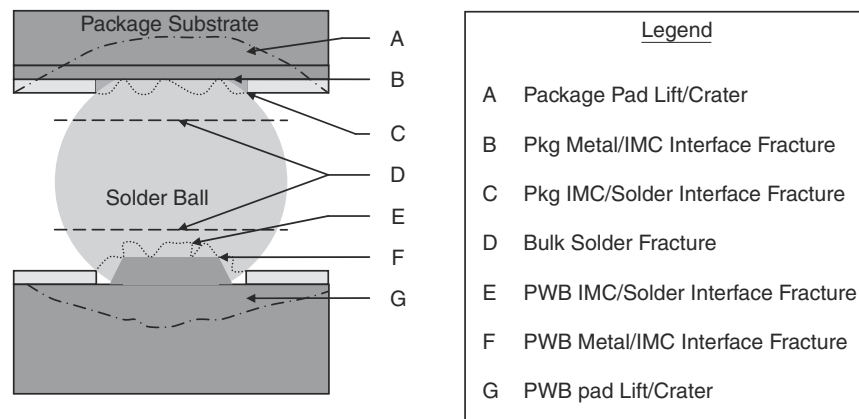
FIGURE 59.10 Different interconnect failure modes.
