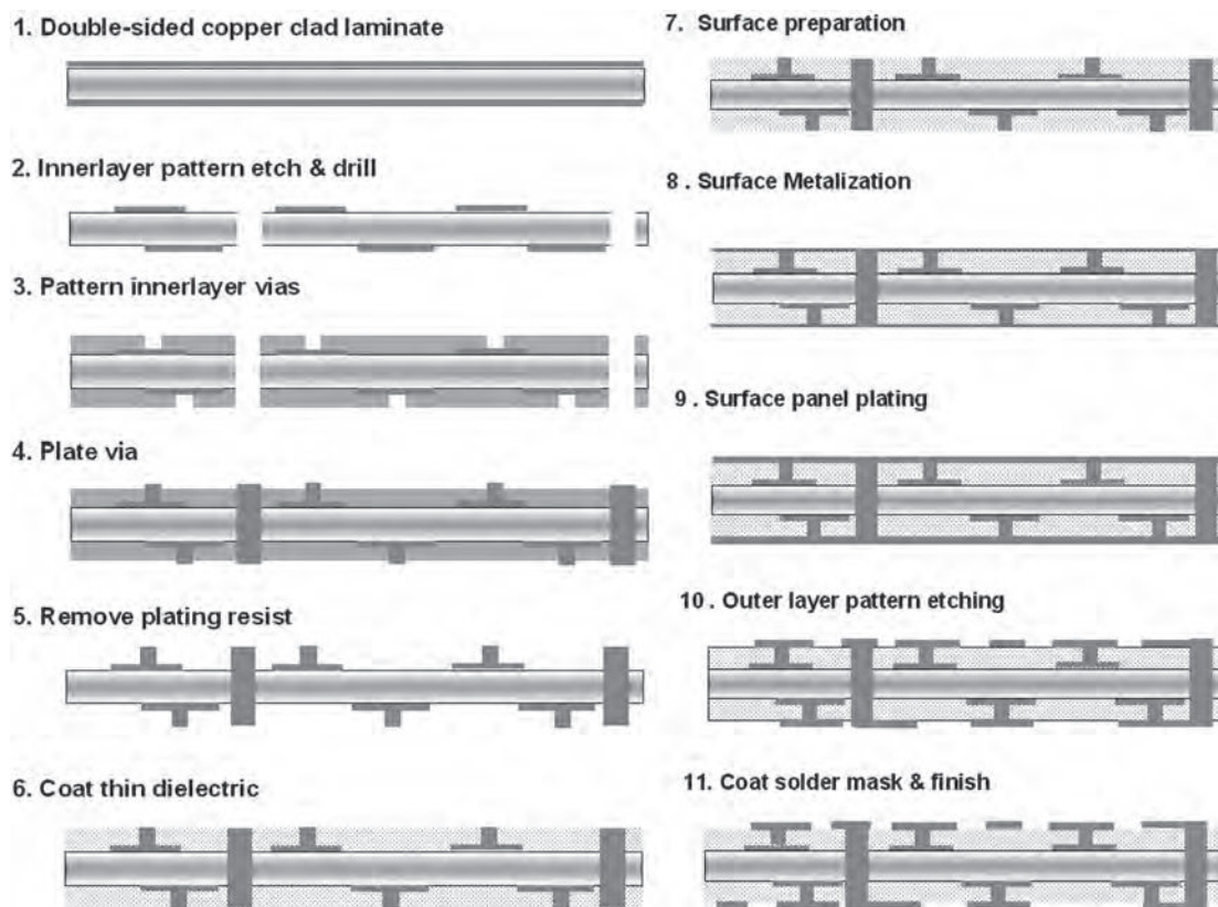
FIGURE 23.16 The typical manufacturing process for FACT-EV boards.
