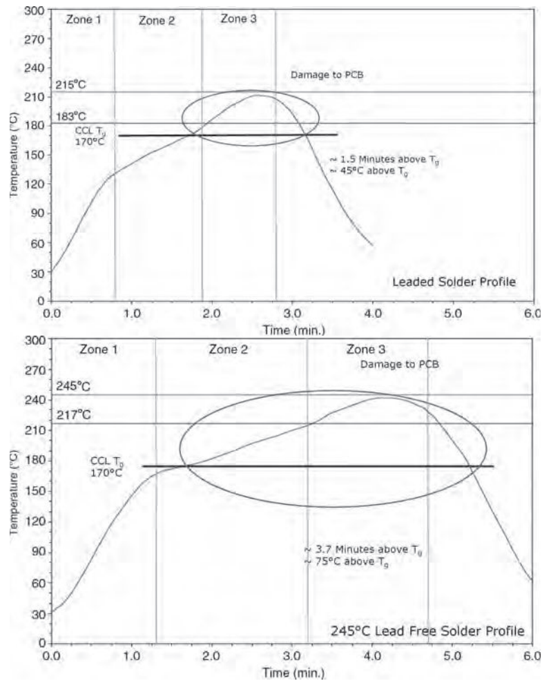
FIGURE 51.2 Damage done to PCBs during typical leaded and lead-free solder cycles. (Courtesy of Microtek Laboratories.)
