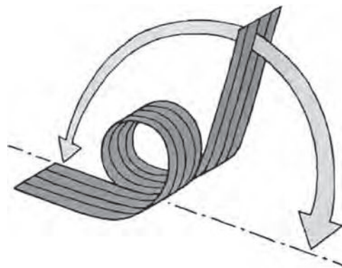
FIGURE 67.5 Flexing endurance test for spiral wiring.
