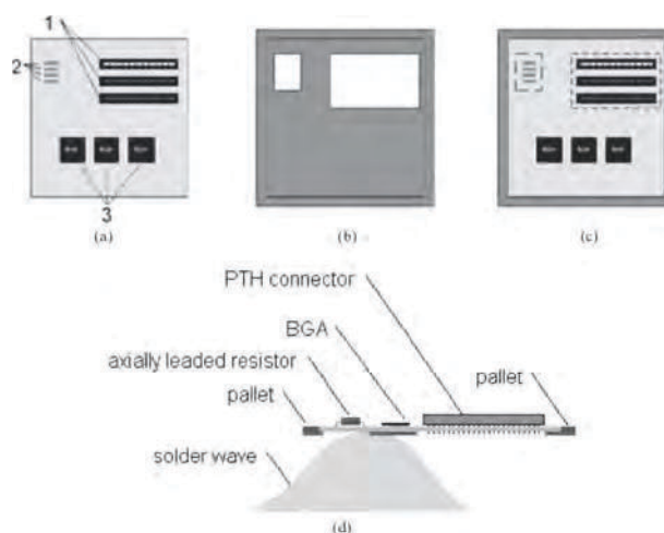
FIGURE 47.25 (a) A wave-solder pallet: (1) a PWB with PTH connectors; (2) PTH axially leaded resistors; (3) BGAs. (b) A pallet with cutouts for PTH components. It also shields BGA via pattern and other components and features on the bottom side of the PWB. (c) A PWB nested in a pallet. Dashed lines indicate areas in the pallet that were cut out to expose the bottom side of the board to the wave. (d) A masked board passing over the solder wave, showing open and shielded areas.
