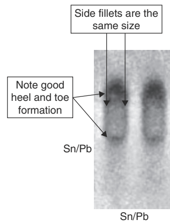
FIGURE 53.5 An x-ray image of a tin-lead example.
