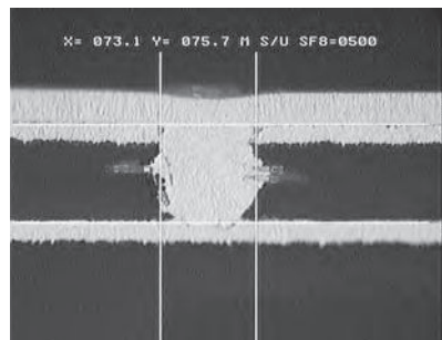
FIGURE 29.2 Example of a plated filled blind microvia.
