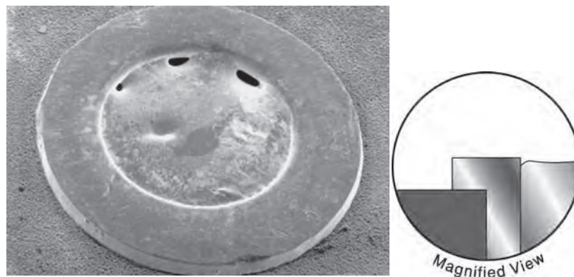
FIGURE 51.16 Non-“wetted” solder joint. (Courtesy of IPC.)
