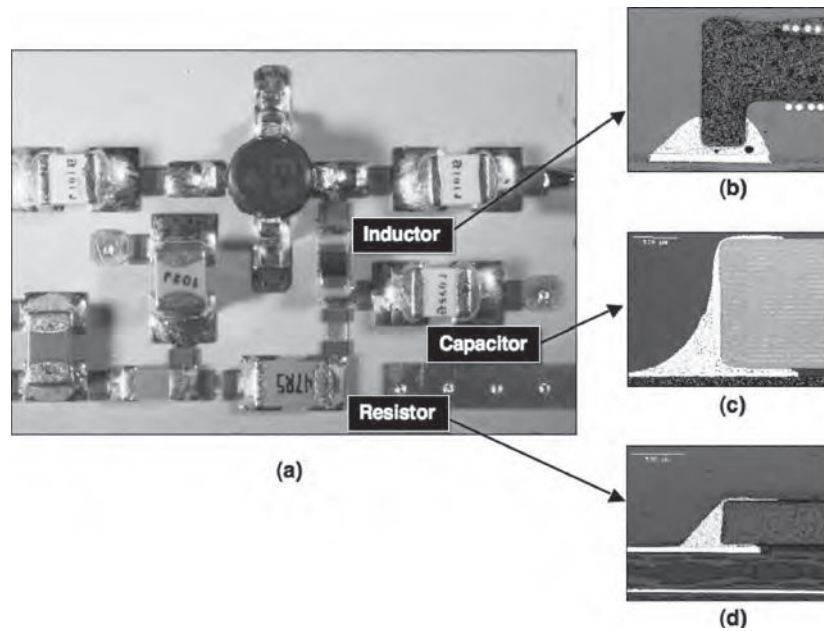
FIGURE 40.12 (a) Stereo photograph showing surface-mount passive (chip) devices: inductor, capacitor, and resistor; (b–d) cross sections of their respective solder joints. (Courtesy of Sandia National Laboratories.)
