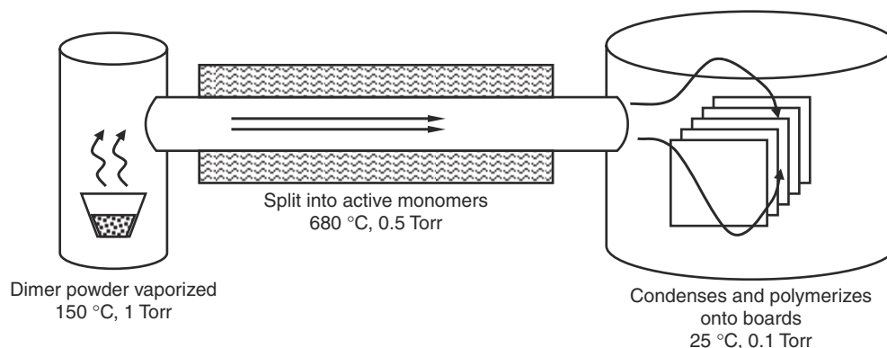
FIGURE 41.5 Para-xylene vapor deposition process.
