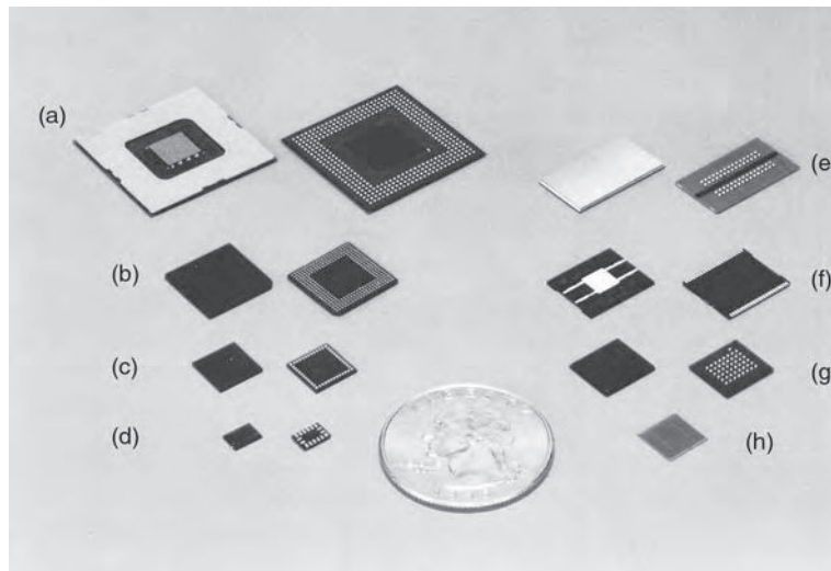
FIGURE 4.7 Photograph of several chip-size packages. On the left are logic CSPs: Row 1: 352-pin TAB-BGA (0.80 mm pitch) Row 2: 288-pin FBGA (0.5 mm pitch) Row 3: 48-pin BCC (0.5 mm pitch) Row 4: 16-pin BCC (0.65 mm pitch) On the right are memory CSPs: Row 1: 60-pin \mu BGA (0.8 mm pitch) Row 2: 46-pin SON (0.5 mm pitch) Row 3: 48-pin FBGA (0.8 mm pitch) Row 4: 16 M bit flash memory chip (Photograph provided courtesy of Fujitsu Microelectronics, Inc.)
