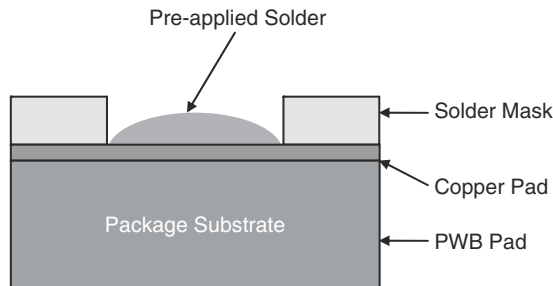
FIGURE 58.21 Solder-on-pad schematic.
