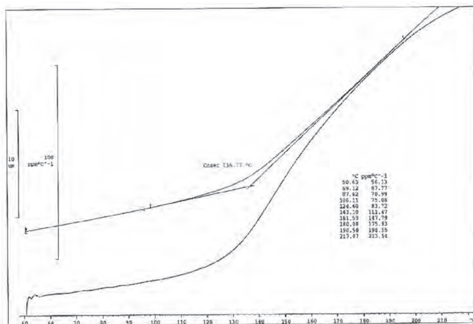
FIGURE 12.5 Typical TMA scan.
