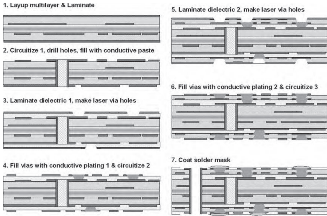
FIGURE 23.14 The typical manufacturing process for CLLAVIS boards.
