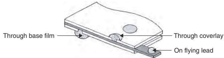
FIGURE 62.12 Locations of microbumps.
