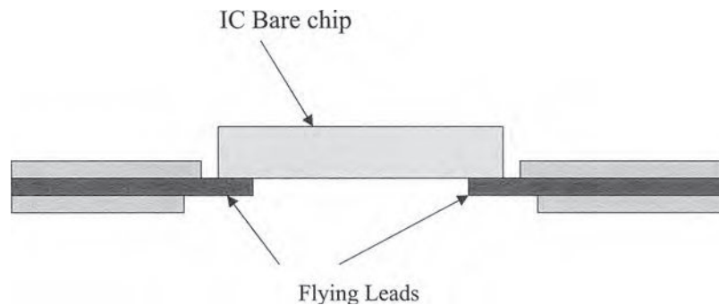
FIGURE 64.7 Direct bonding of flying leads.
