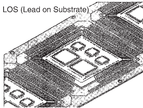
FIGURE 3.18 LOS printed circuit MCP.
