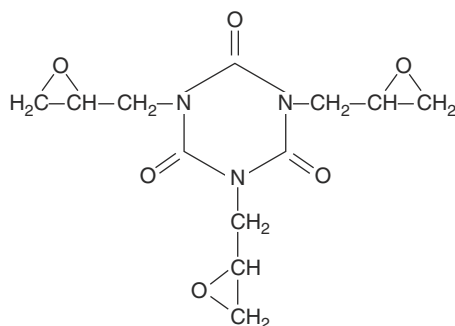
FIGURE 7.8 Epoxy isocyanurate.
