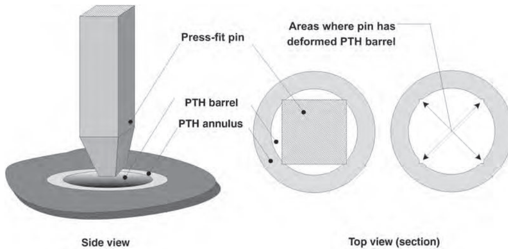
FIGURE 49.2 A square or rectangular pin forced into round hole. This is the most primitive of press-fit techniques.
