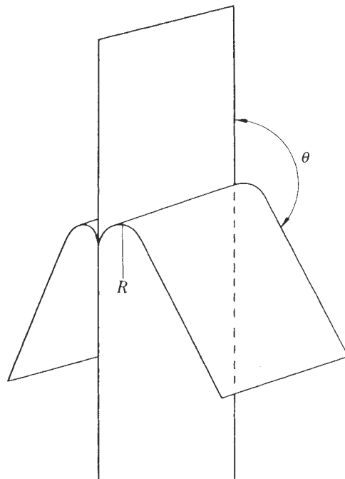
FIGURE 67.4 JIS-C5016 MIT test method for flexing endurance. R is the radius of the bend during the test symbol for “theta” is the angle from vertical.
