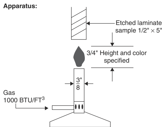
FIGURE 1.12 Flammability testing.
