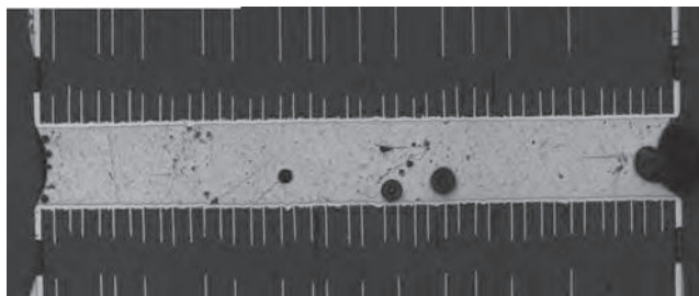
FIGURE 29.1 A 15:1 aspect ratio plated with MacDermid PPR 100.
