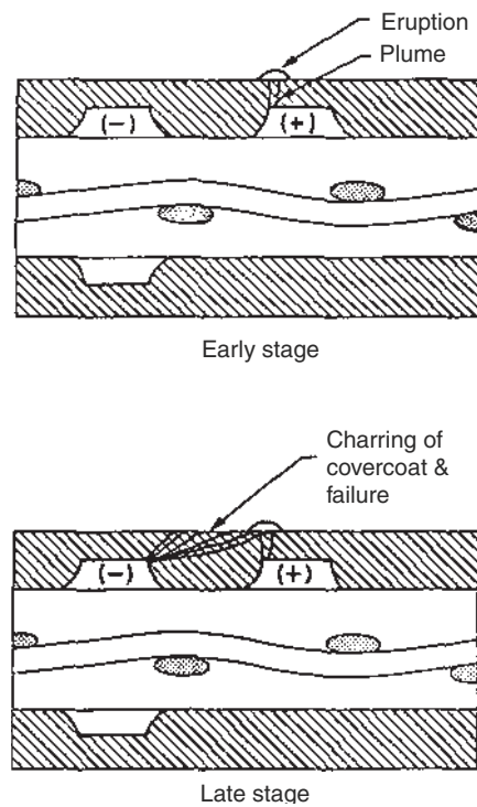
FIGURE 56.4 Anodic eruption failure mode. 2 © 1976 IEEE
