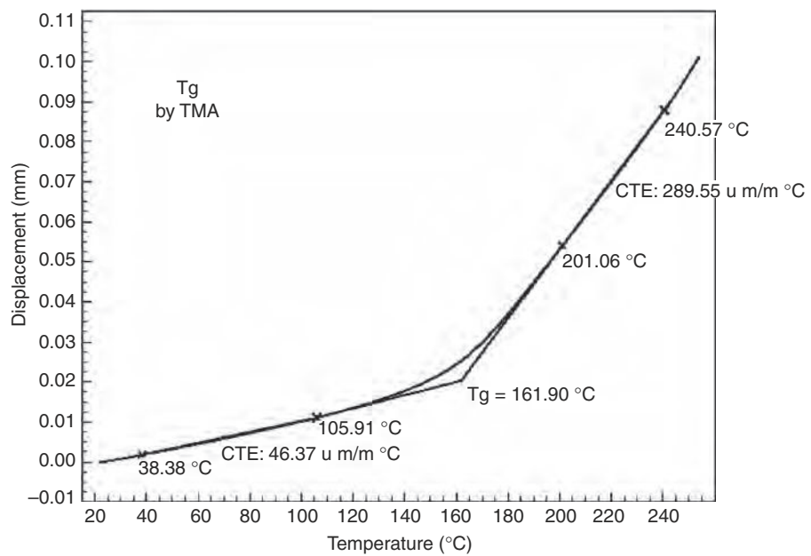
FIGURE 27.3 TMA plot: T_g and CTE.
