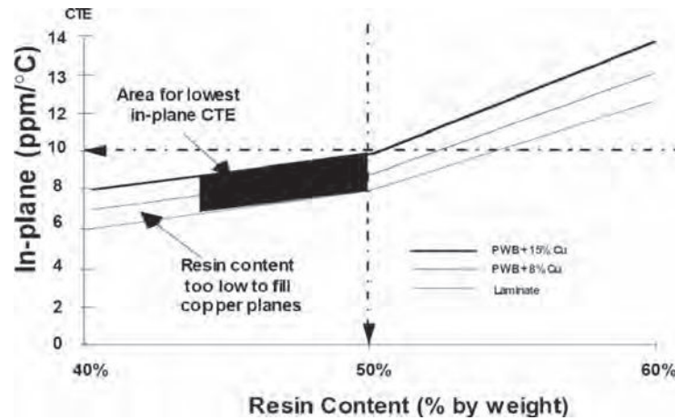
FIGURE 22.13 Impact of copper and resin content on in-plane CTE. (Source: DuPont.)
