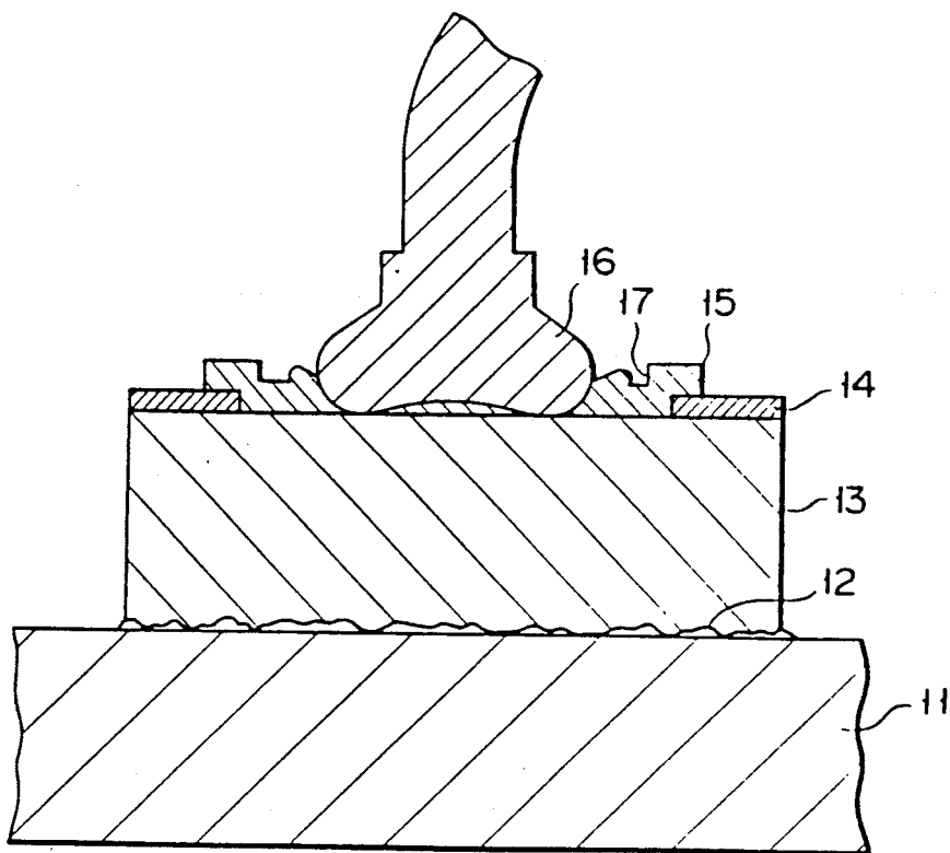
FIG. 2 (PRIOR ART)
